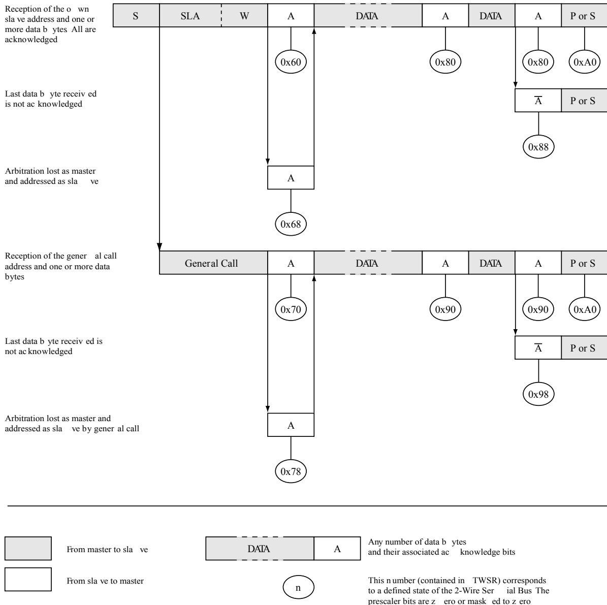
Figure 25-18. Formats and States in the Slave Receiver Mode
