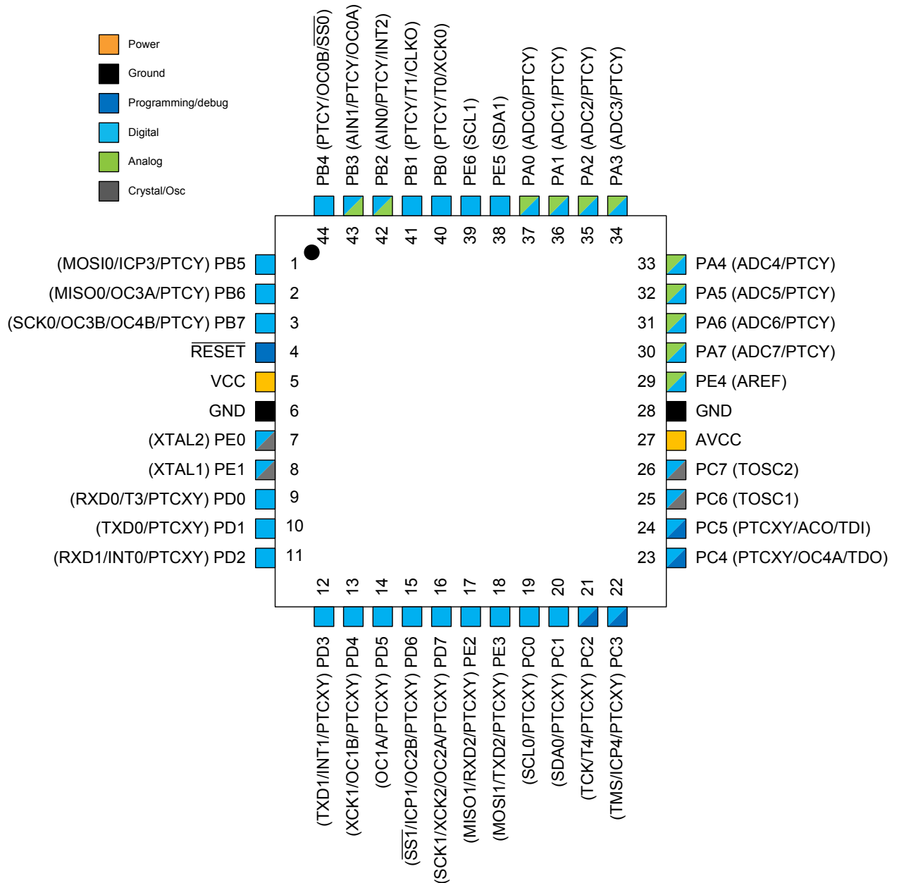
Figure 5-1. Pinout ATmega324PB
