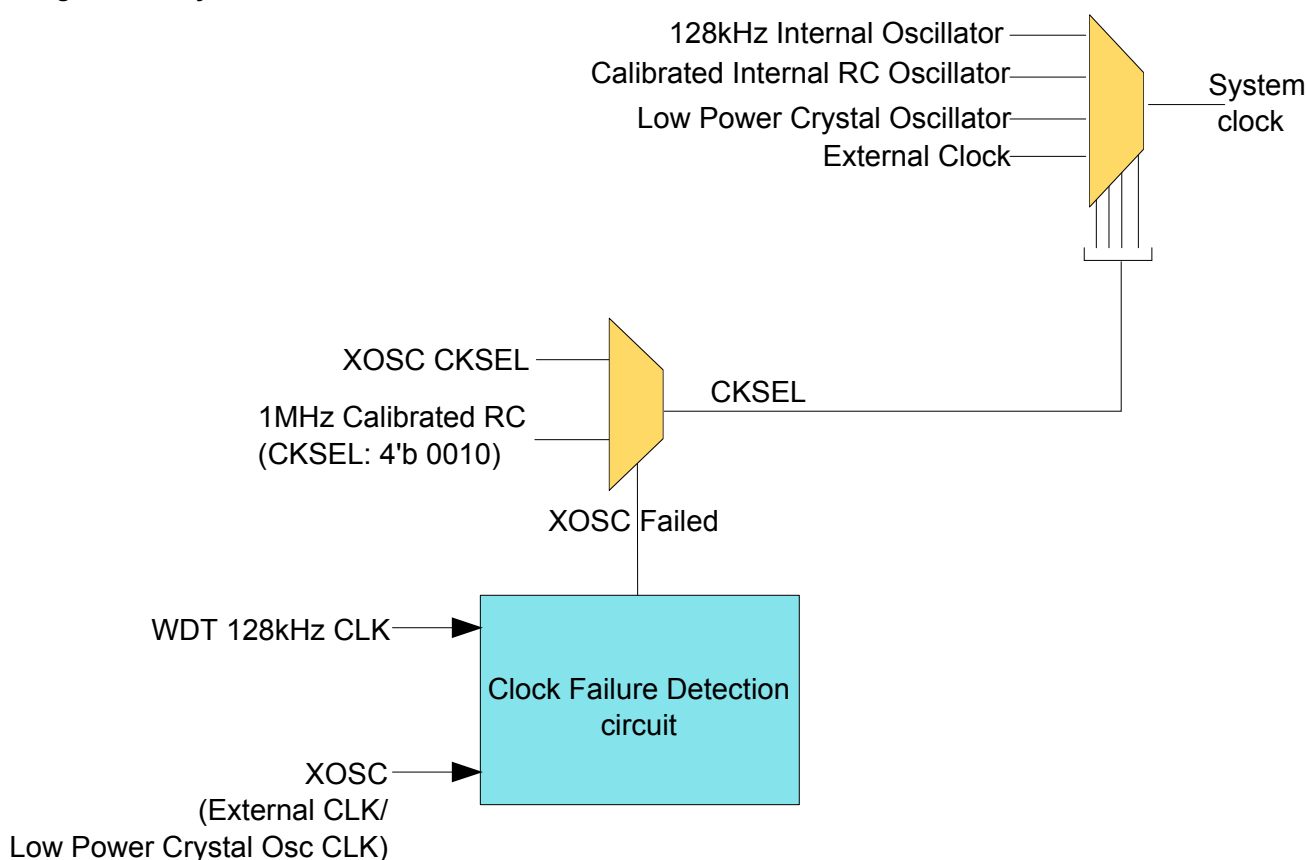
Figure 11-1. System Clock Generation with CFD Mechanism
