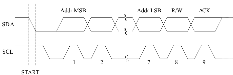
Figure 24-5 Address Packet Format
