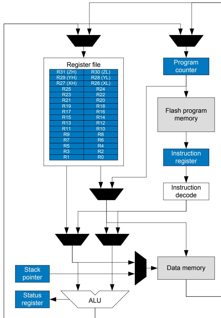
Figure 10-1 Block Diagram of the AVR MCU Architecture
