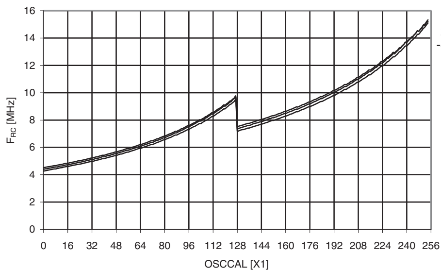
Figure 30-40. Atmel ATmega164A: Calibrated 8MHz RC oscillator vs. OSCCAL value.
