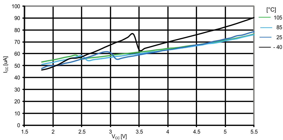
Figure 31-36. Atmel ATmega164PA: Analog comparator current vs. V_{CC} .
