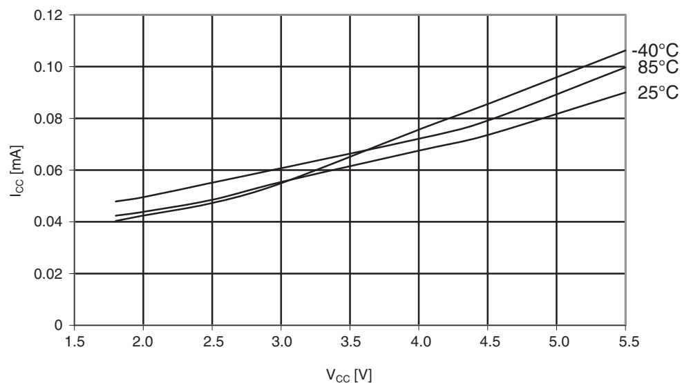
Figure 30-354. Atmel ATmega1284P: Idle supply current vs. V_{CC} (internal RC oscillator, 128kHz).
