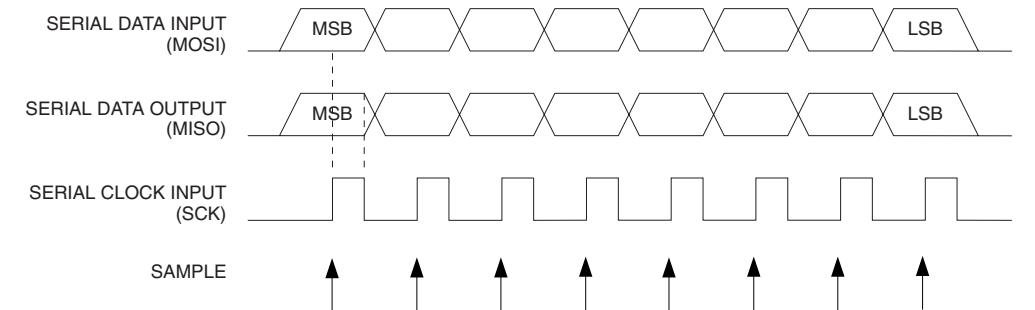
Figure 148. SPI Serial Programming Waveforms
