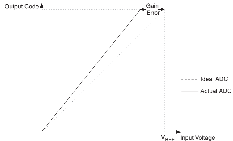
Figure 118. Gain Error
