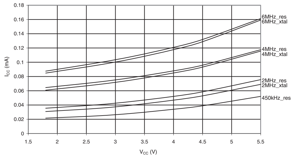
Figure 30-60. Standby Supply Current vs. Vcc (Watchdog Timer Disabled).
