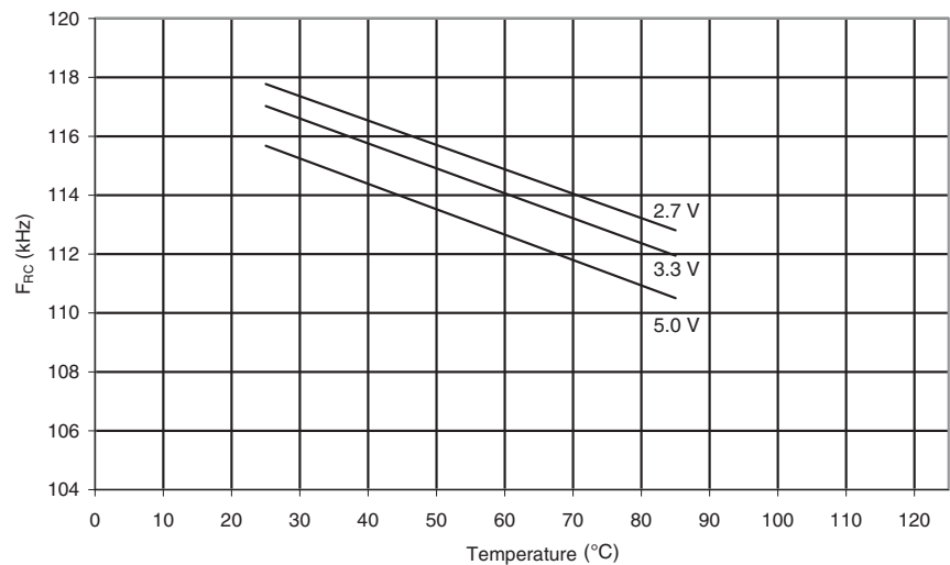
Figure 30-126. Watchdog Oscillator Frequency vs. Temperature.
