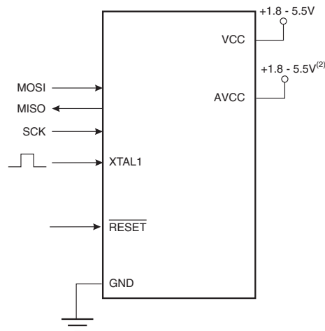
Figure 28-7. Serial Programming and Verify (1)
