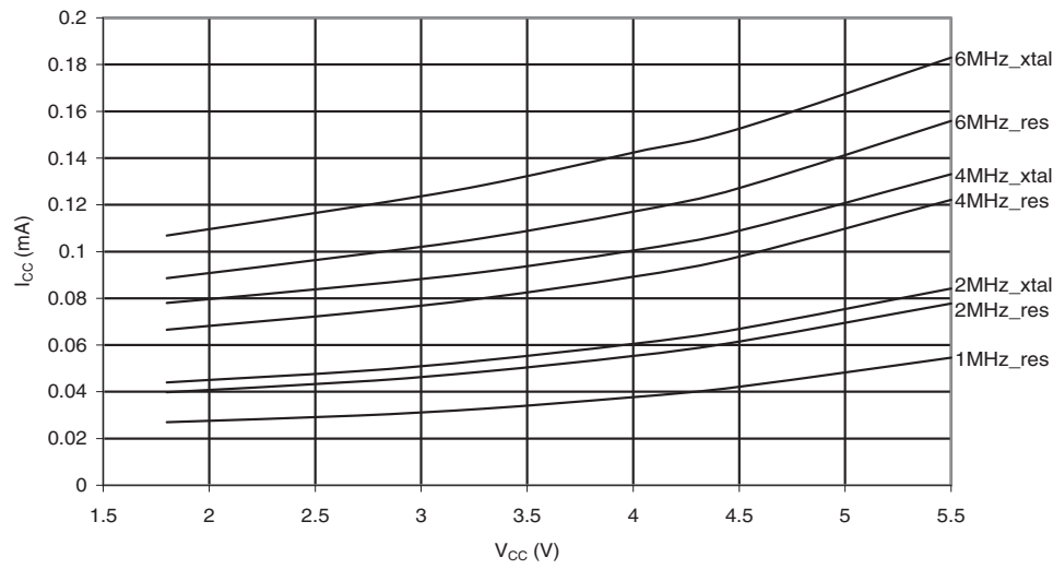
Figure 30-106. Standby Supply Current vs. Vcc (Watchdog Timer Disabled).
