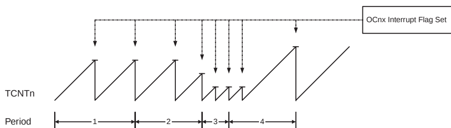
Figure 17-3. CTC Mode, Timing Diagram
