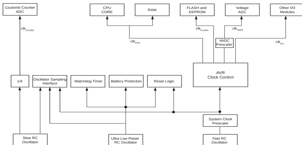
Figure 9-1. Clock Distribution
