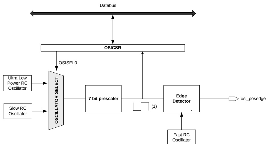
Figure 9-2. Oscillator Sampling Interface Block Diagram
