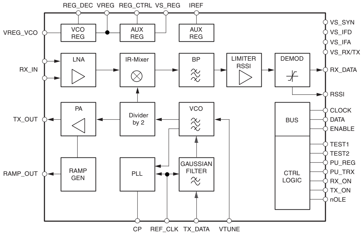
Figure 1-1. Block Diagram
