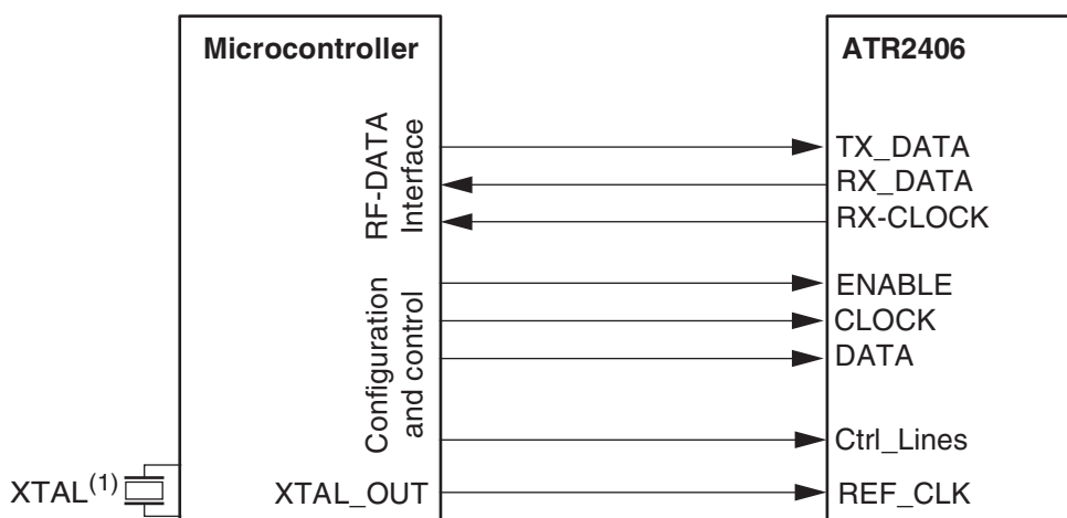
Figure 8-1. Microcontroller Interfacing with General Purpose MCU, Pin Connections between Microcontroller and ATR2406
