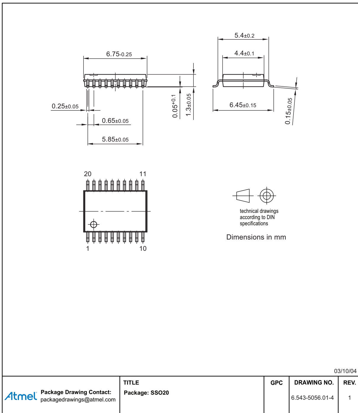
Figure 12-1. SSO20
