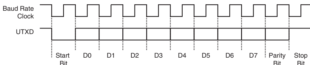
Figure 29-9. Character Transmission
