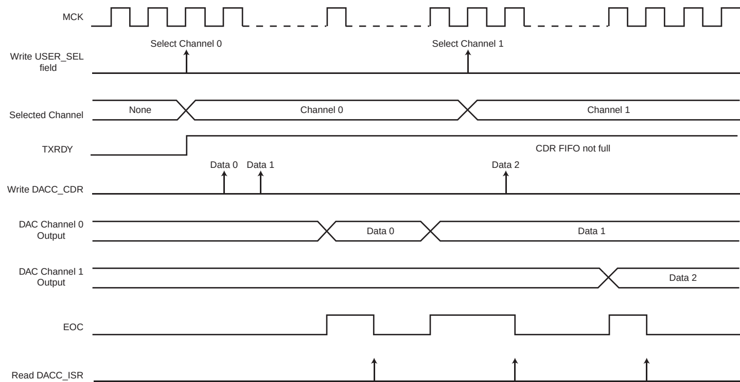
Figure 40-2. Conversion Sequence
