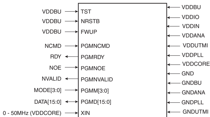
Figure 22-1. Parallel Programming Interface
