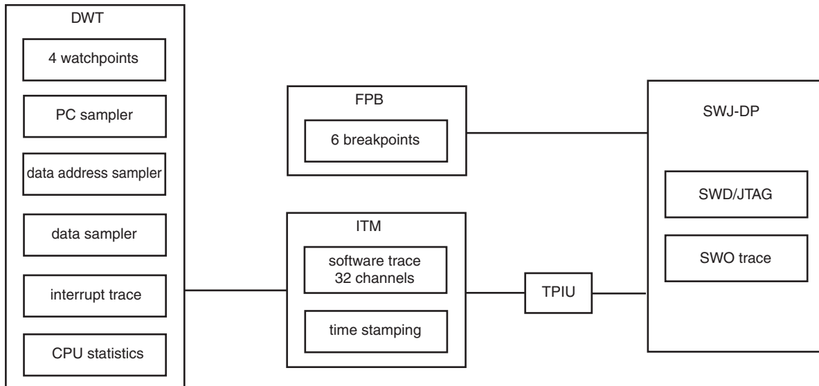
Figure 14-4. Debug Architecture
