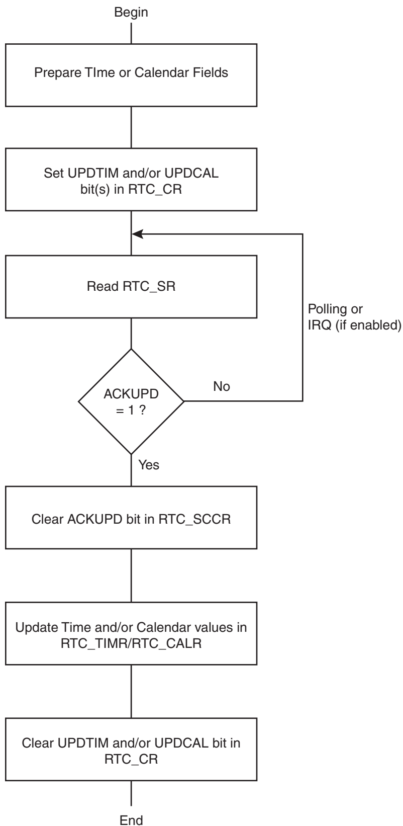
Figure 18-2. Update Sequence
