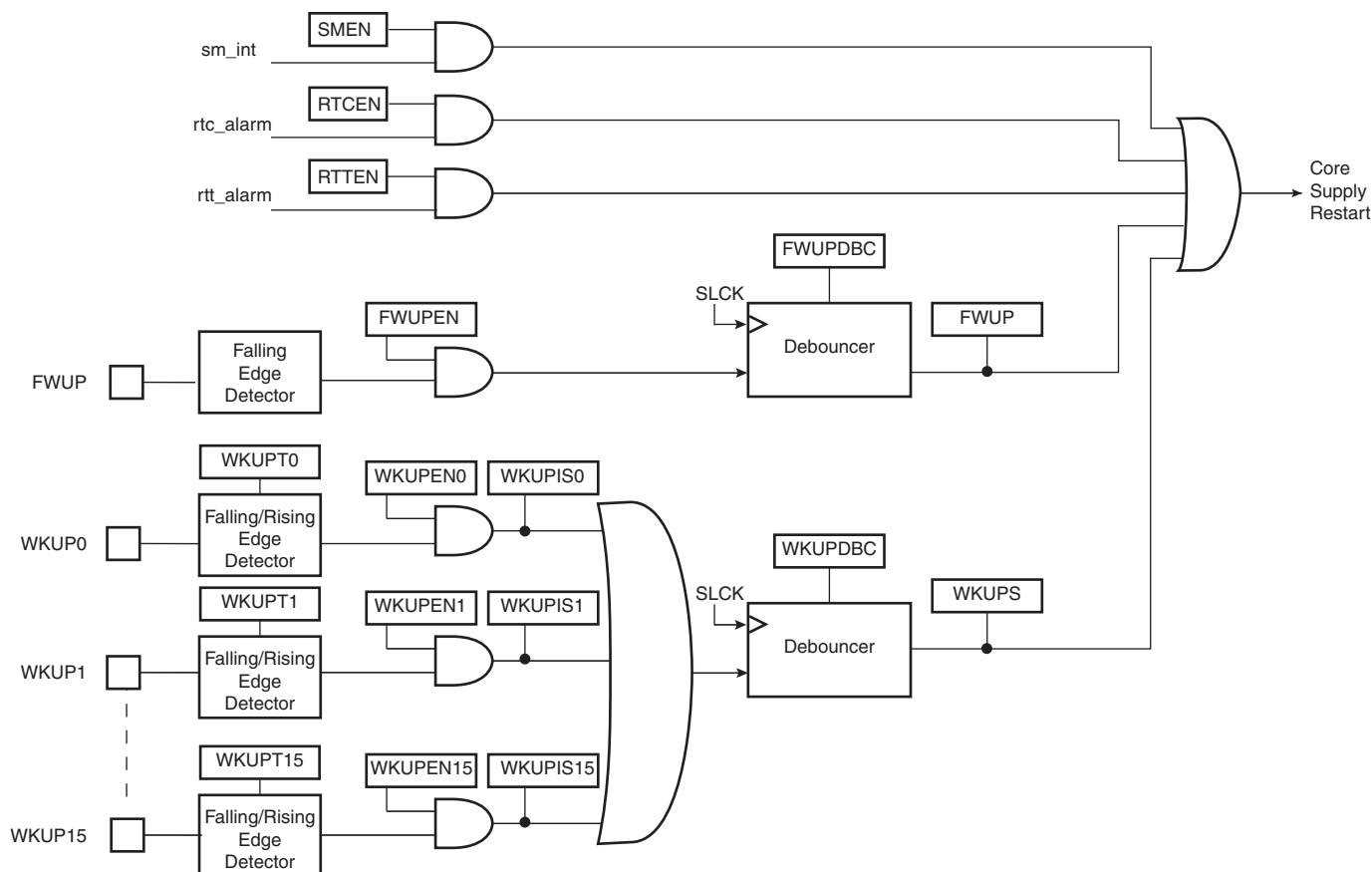
Figure 19-7. Wake Up Sources
