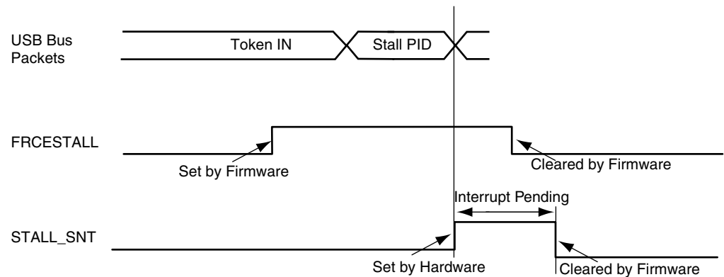
Figure 39-17. Stall Handshake Data IN Transfer
