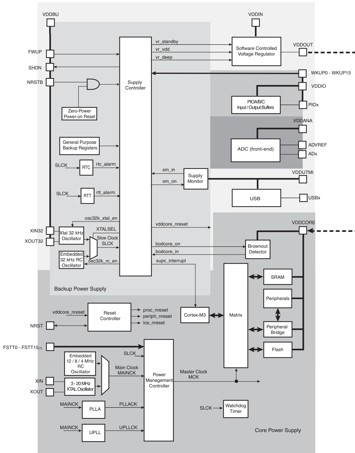
Figure 19-1. Supply Controller Block Diagram
