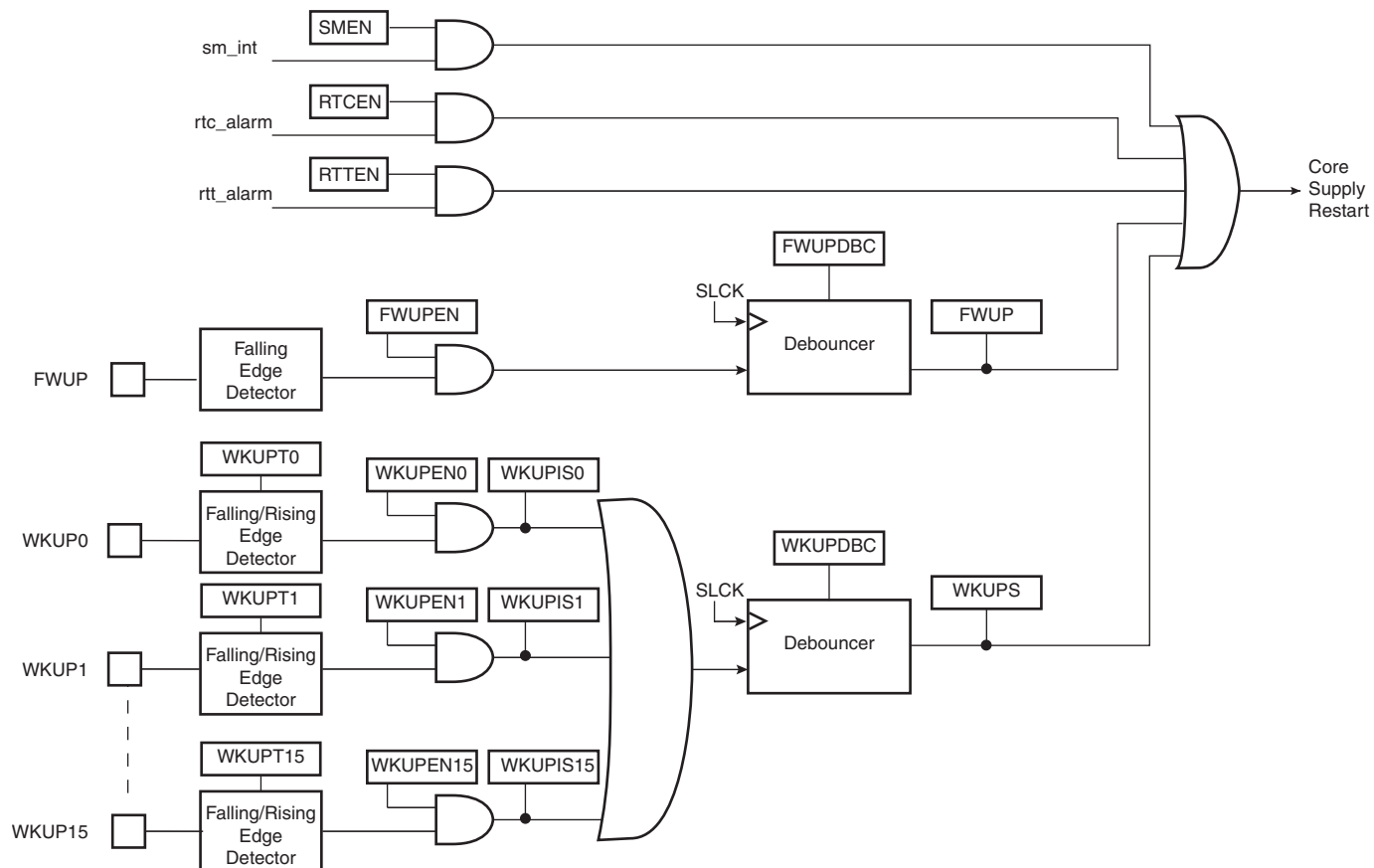
Figure 5-4. Wake-up Source
