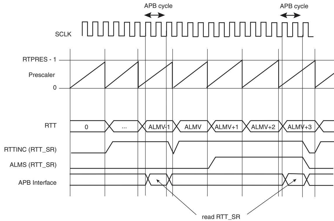
Figure 17-2. RTT Counting
