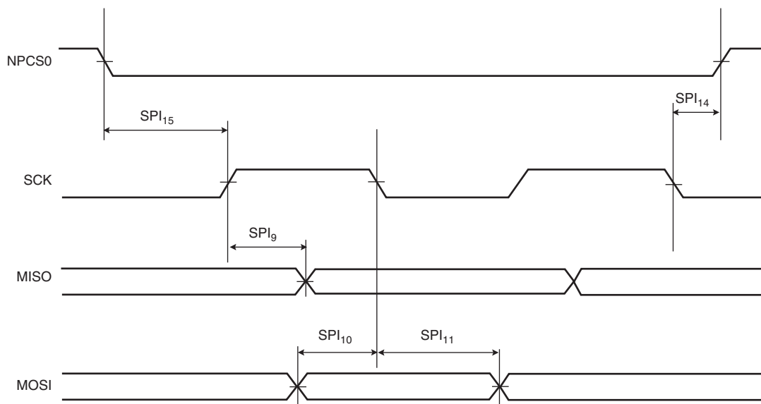
Figure 43-29. USART SPI Slave mode (Mode 0 or 3)
