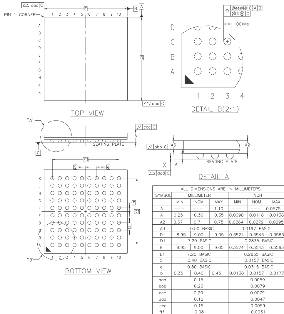
Figure 44-2. 100-ball TFBGA Package Drawing
