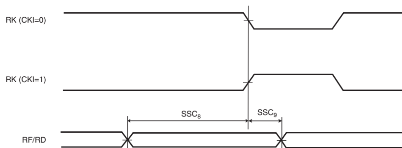
Figure 43-20. SSC Receiver RK and RF as input
