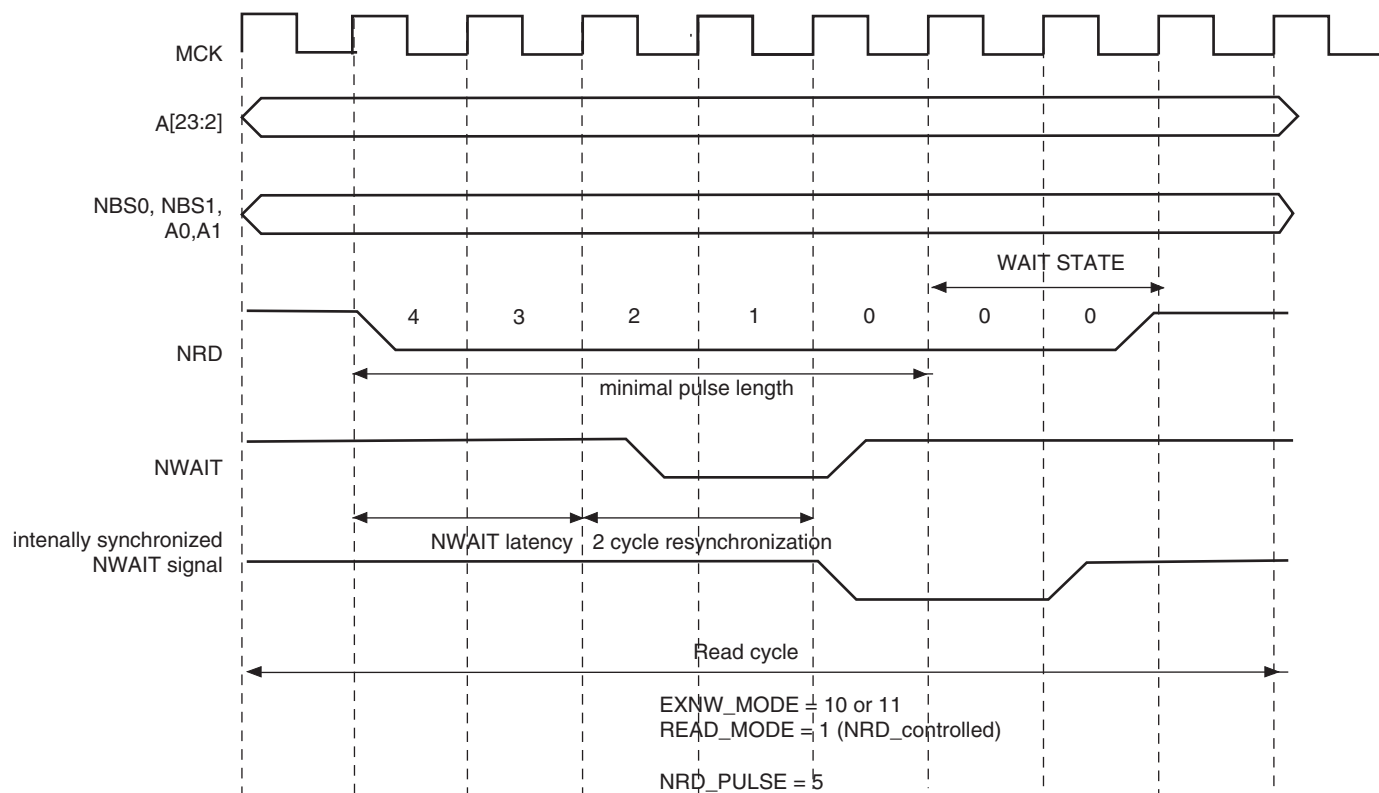
Figure 25-27. NWAIT Latency
