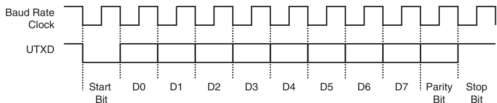
Figure 34-9. Character Transmission
