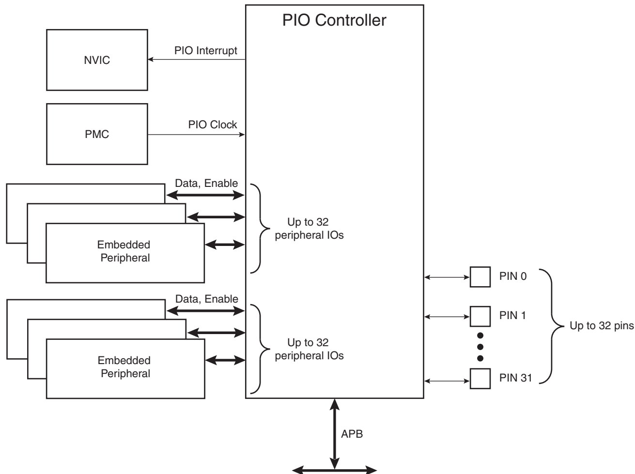
Figure 30-1. Block Diagram
