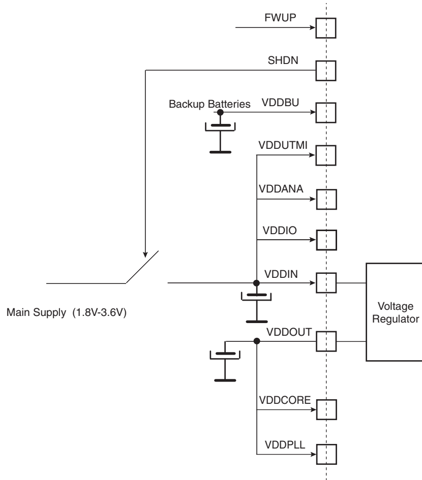
Figure 19-2. Separated Backup Supply Powering Scheme
