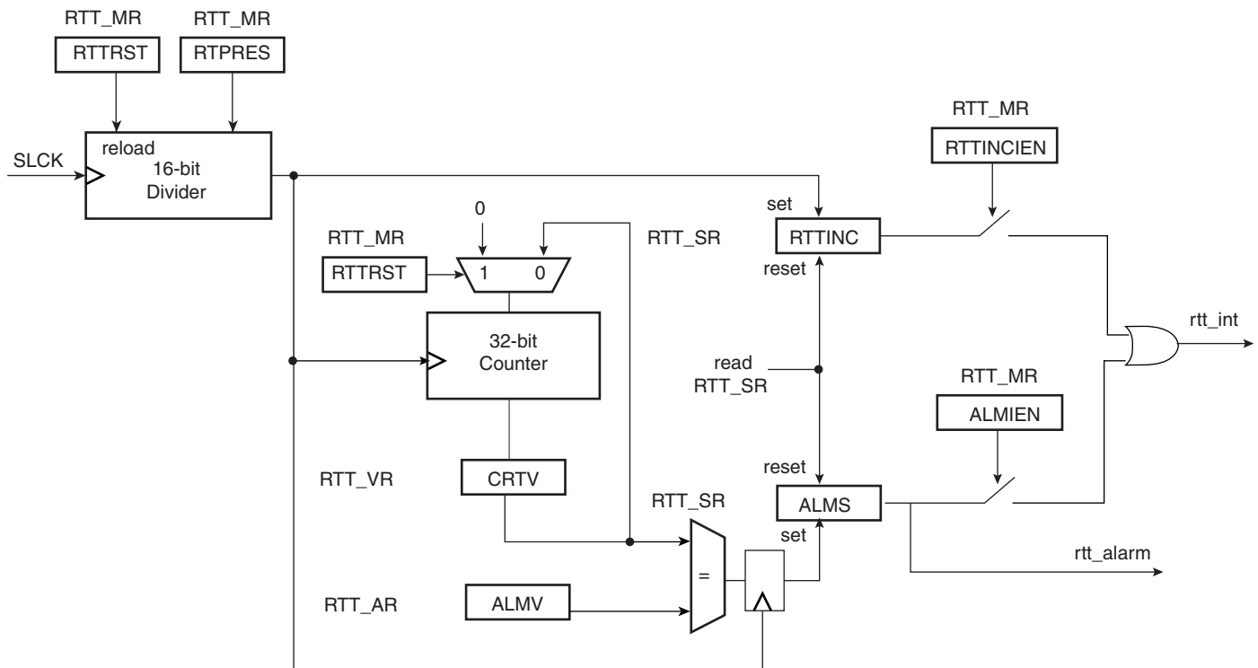
Figure 17-1. Real-time Timer
