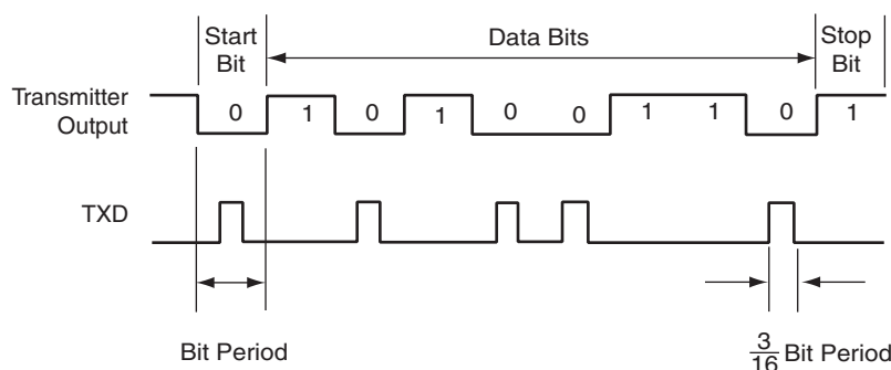
Figure 35-34. IrDA Modulation
