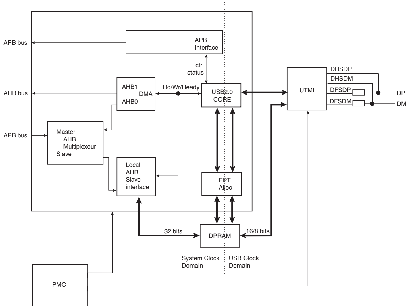
Figure 39-1. Block Diagram
