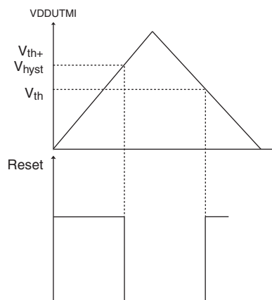
Figure 43-2. VDDUTMI Supply Monitor
