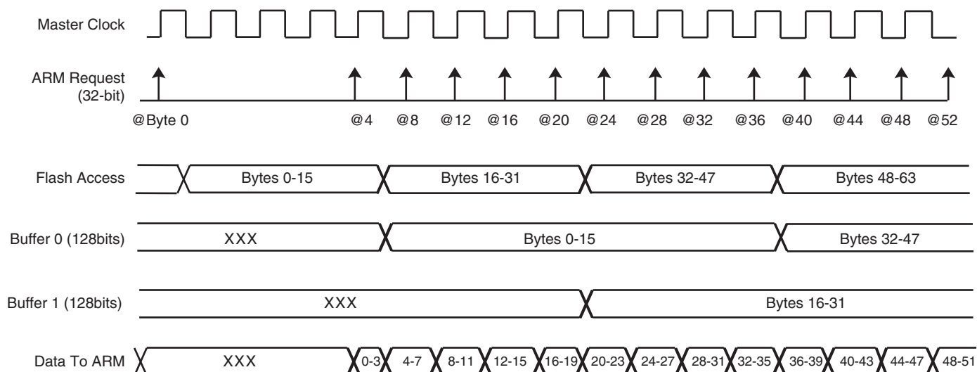
Figure 21-3. Code Read Optimization for FWS = 3
