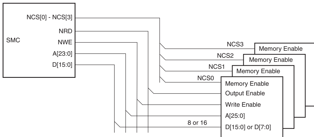
Figure 25-3. Memory Connections for External Devices
