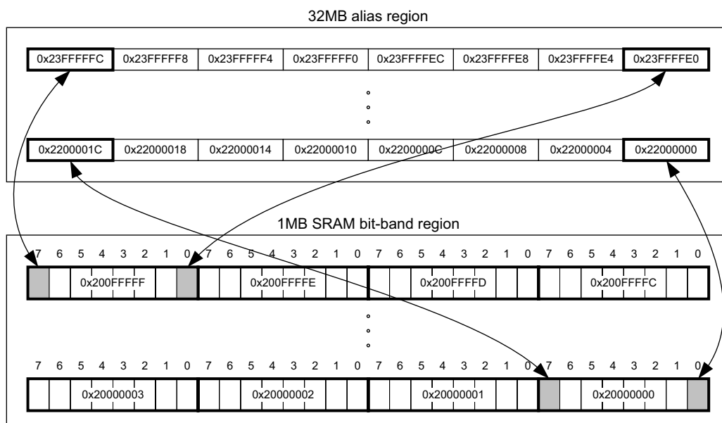
Figure 13-2. Bit-band mapping
