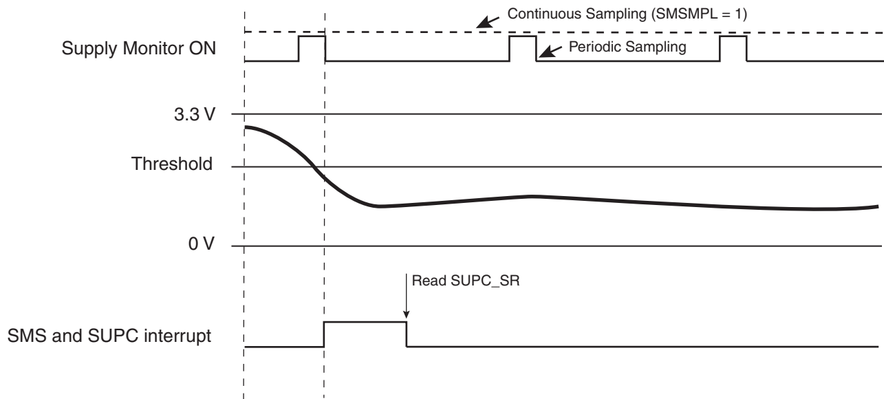
Figure 19-4. Supply Monitor Status Bit and Associated Interrupt
