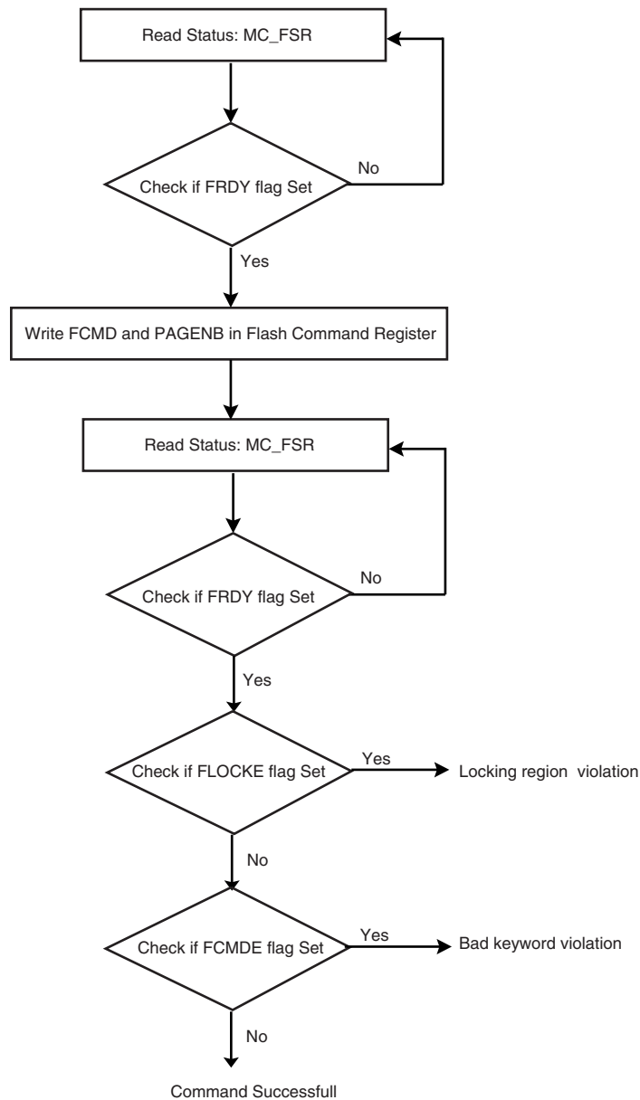
Figure 21-5. Command State Chart
