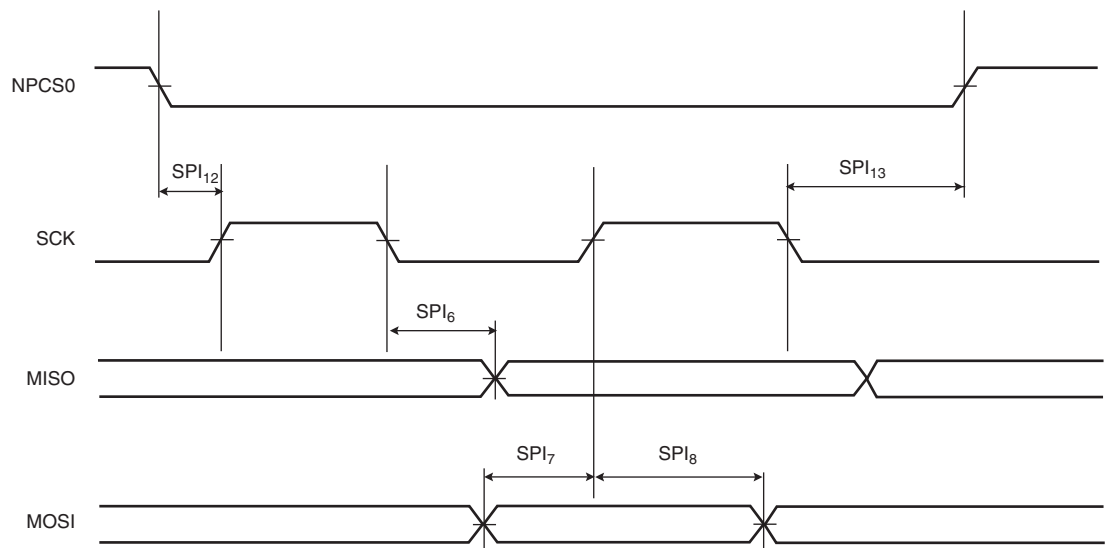
Figure 43-28. USART SPI Slave mode (Mode 1 or 2)
