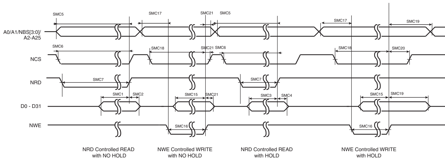
Figure 43-26. SMC Timings - NRD Controlled Read and NWE Controlled Write
