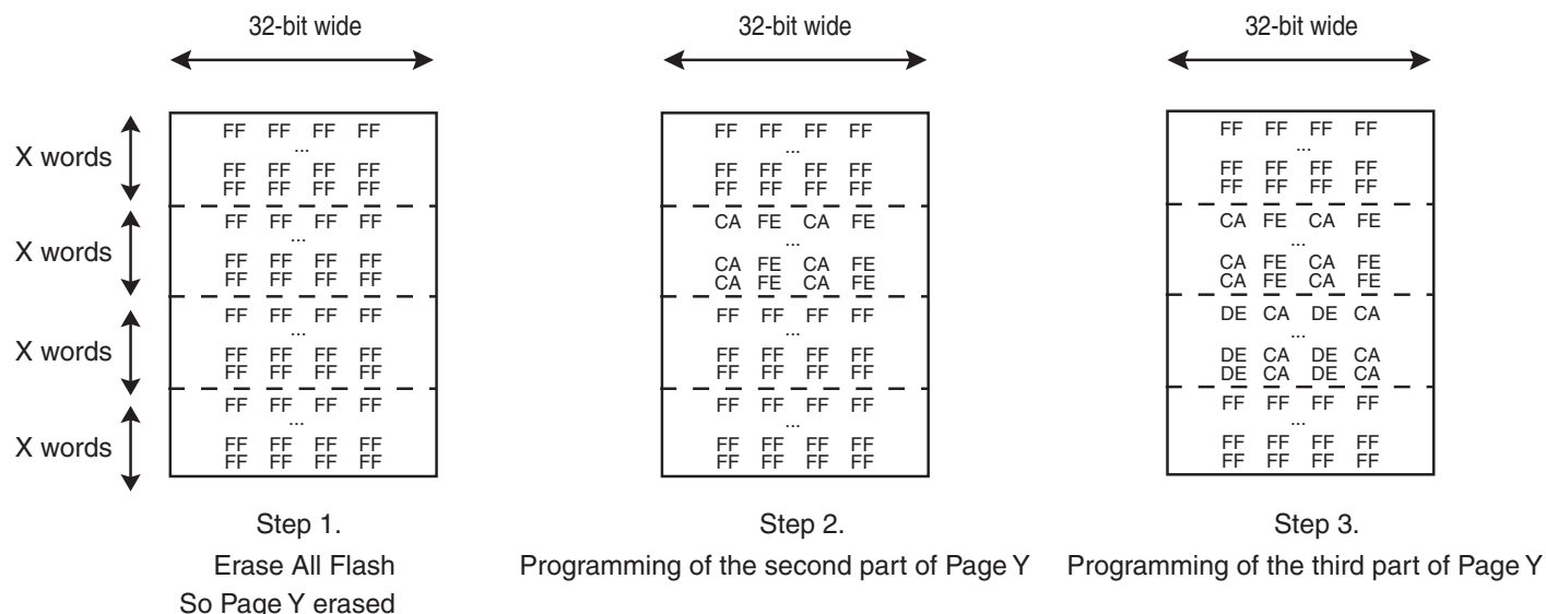
Figure 21-6. Example of Partial Page Programming
