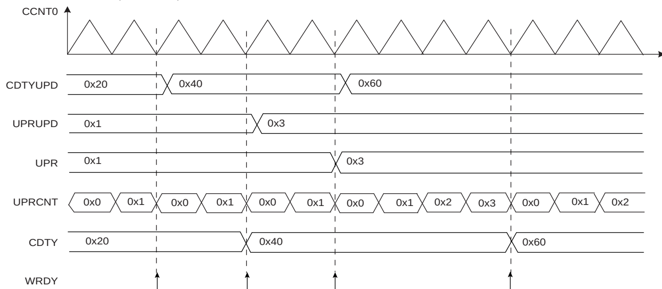
Figure 38-10. Method 2 (UPDM=1)
