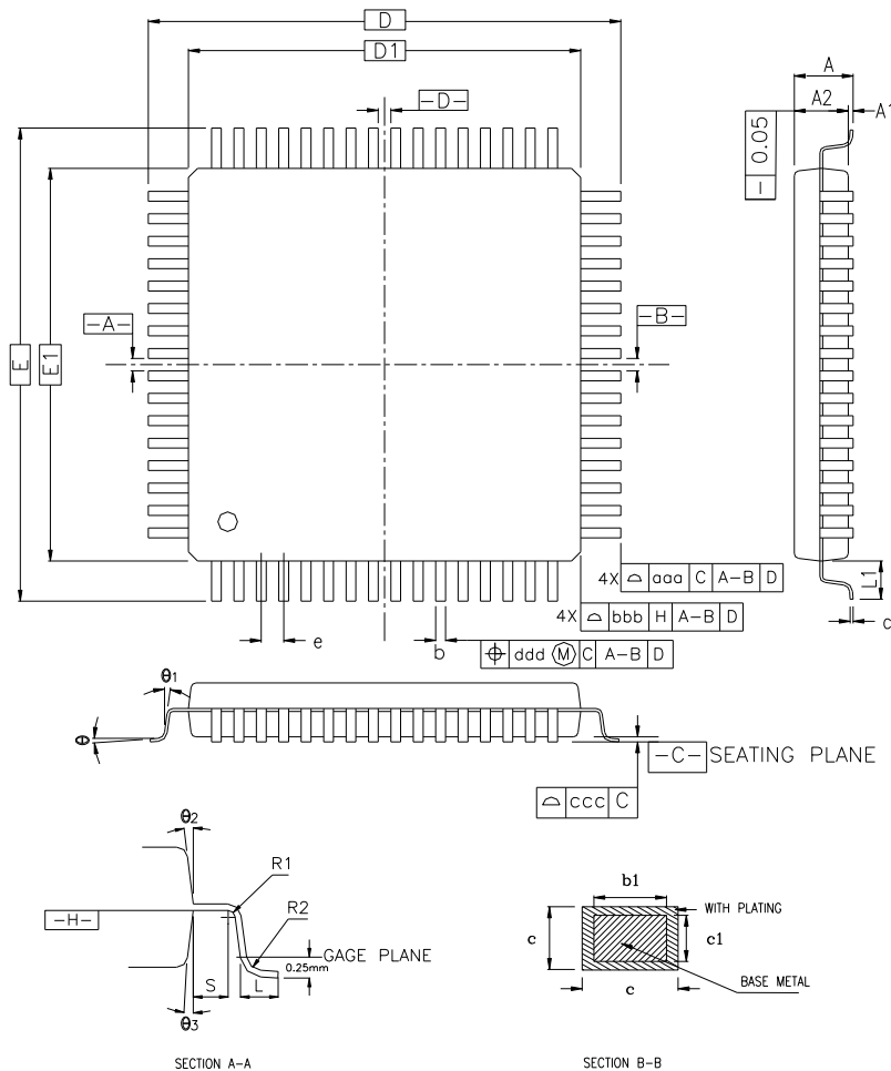
Figure 44-1. 100-lead LQFP Package Drawing
