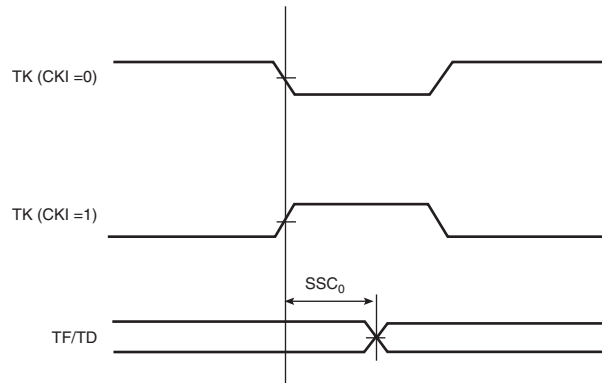
Figure 43-16. SSC Transmitter, TK and TF as output
