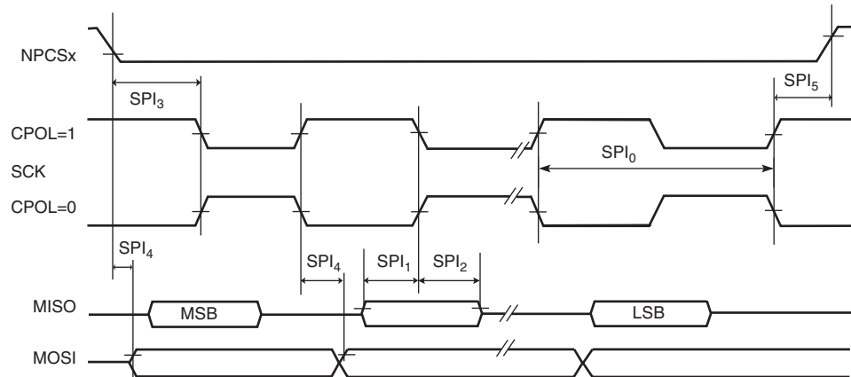
Figure 43-27. USART SPI Master Mode
