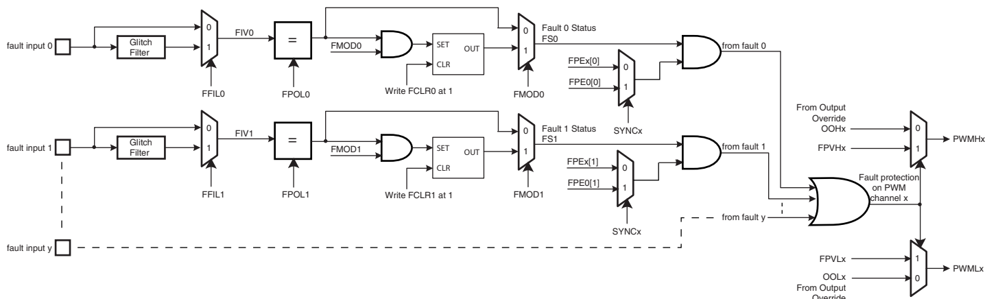
Figure 38-8. Fault Protection
