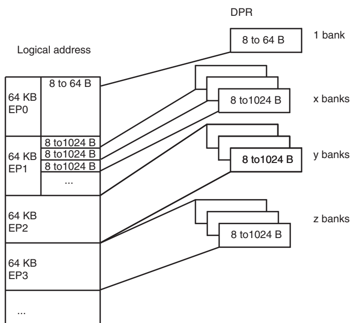
Figure 39-4. Logical Address Space for DPR Access
