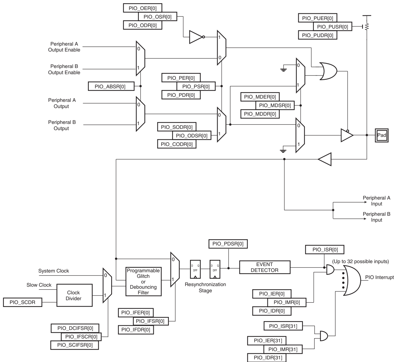
Figure 30-3. I/O Line Control Logic
