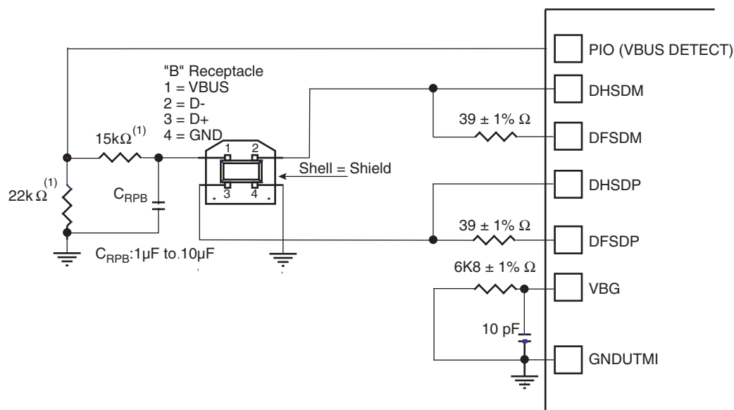
Figure 39-2. Board Schematic
