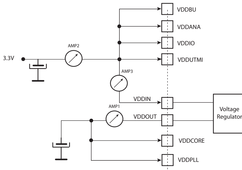
Figure 43-8. Measurement Setup for Wait Mode
