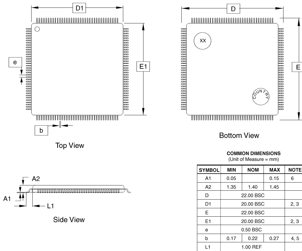
Figure 44-3. 144-lead LQFP Package Drawing
