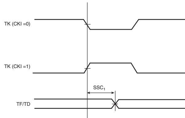
Figure 43-17. SSC Transmitter, TK as input and TF as output
