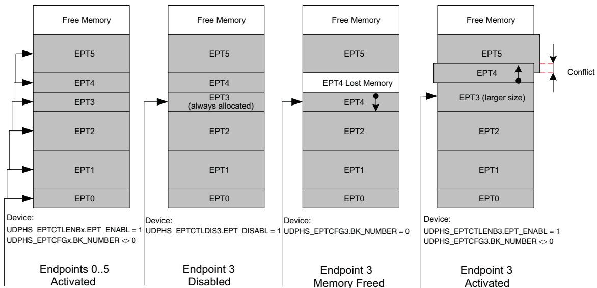
Figure 39-5. Allocation and Reorganization of the DPRAM
