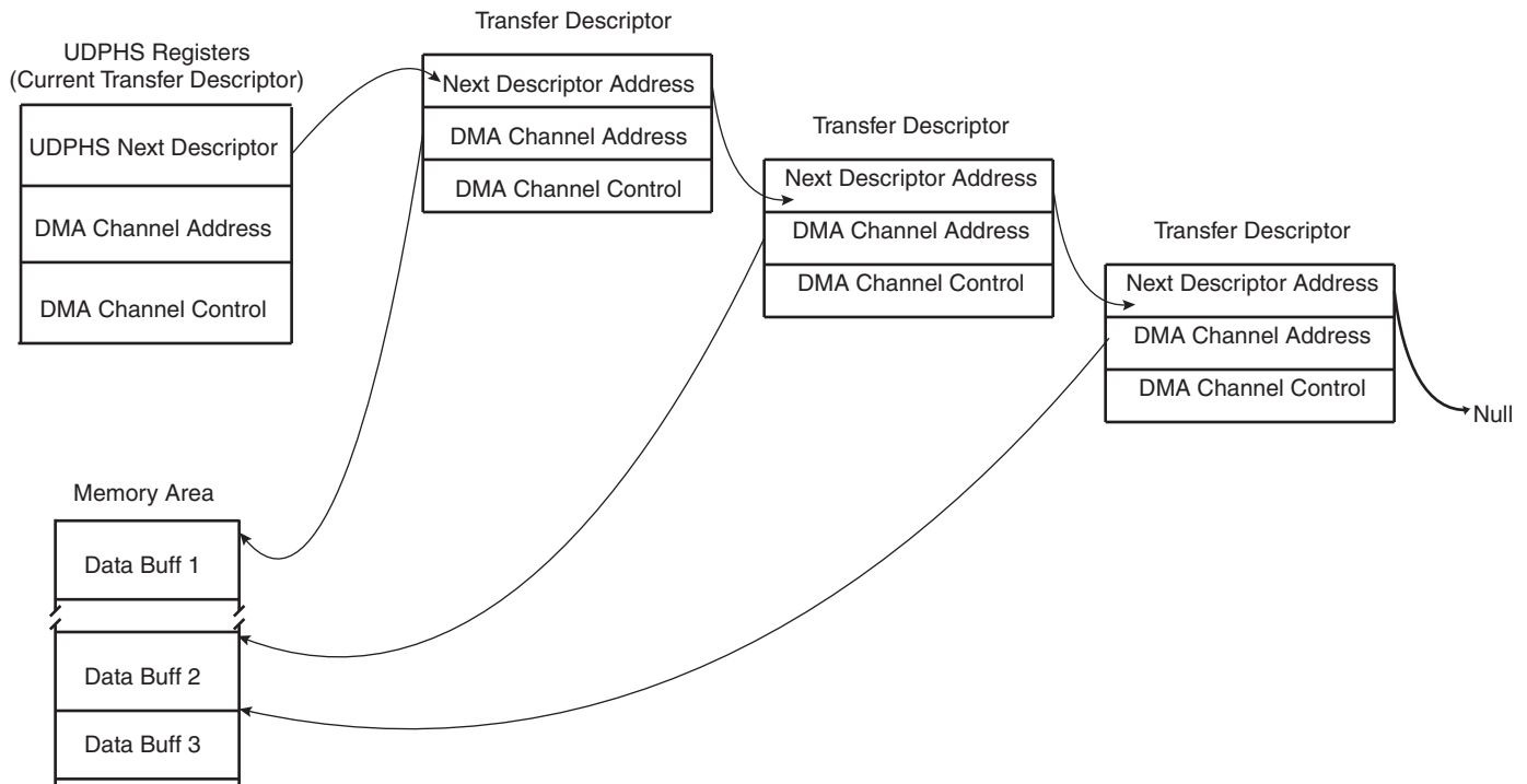
Figure 39-6. Example of DMA Chained List
