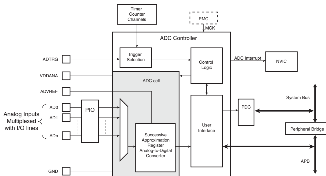
Figure 42-1. Analog-to-Digital Converter Block Diagram
