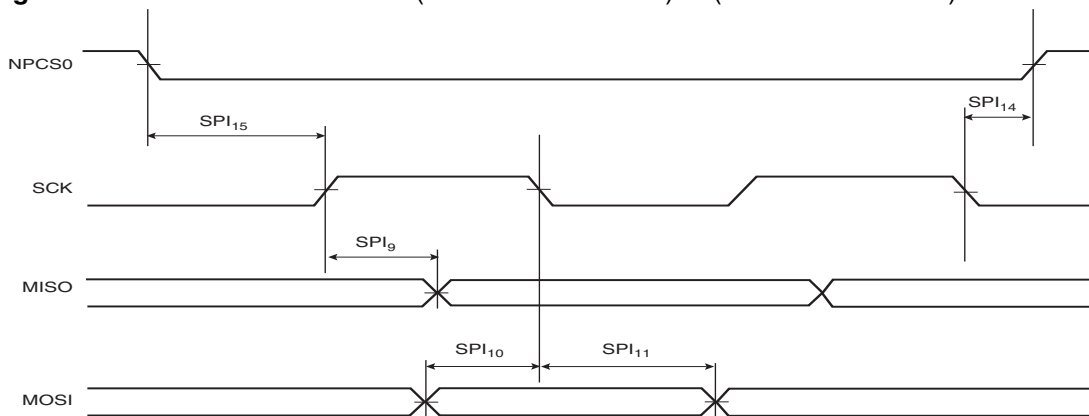
Figure 43-15. SPI Slave Mode with (CPOL = NCPHA = 0) or (CPOL= NCPHA= 1)
