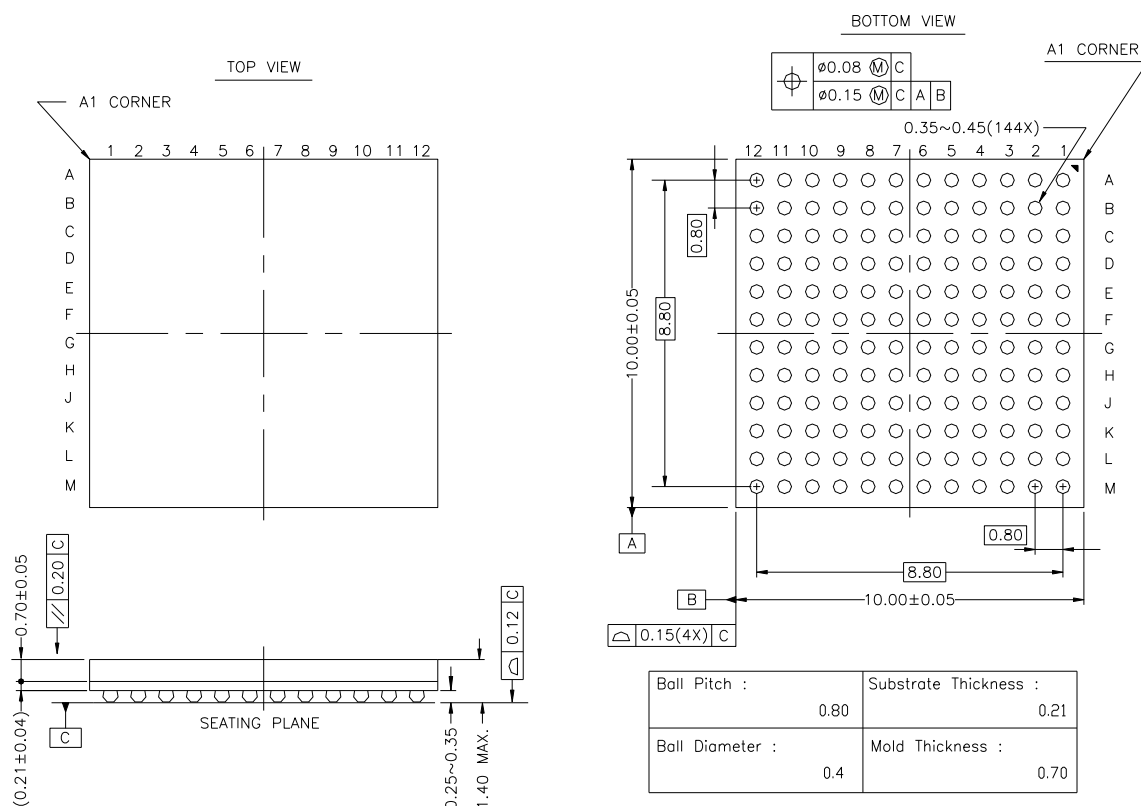
Figure 44-4. 144-ball LFBGA Package Drawing
