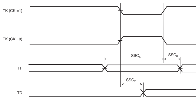
Figure 43-19. SSC Transmitter, TK and TF as input
