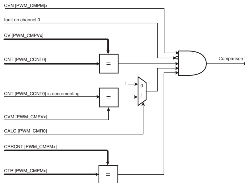
Figure 38-13. Comparison Unit Block Diagram
