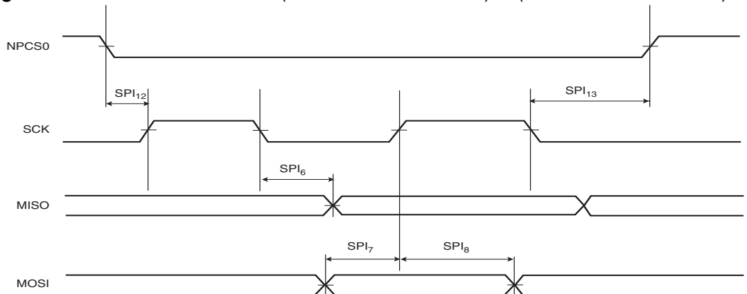
Figure 43-14. SPI Slave Mode with (CPOL=0 and NCPHA=1) or (CPOL=1 and NCPHA=0)
