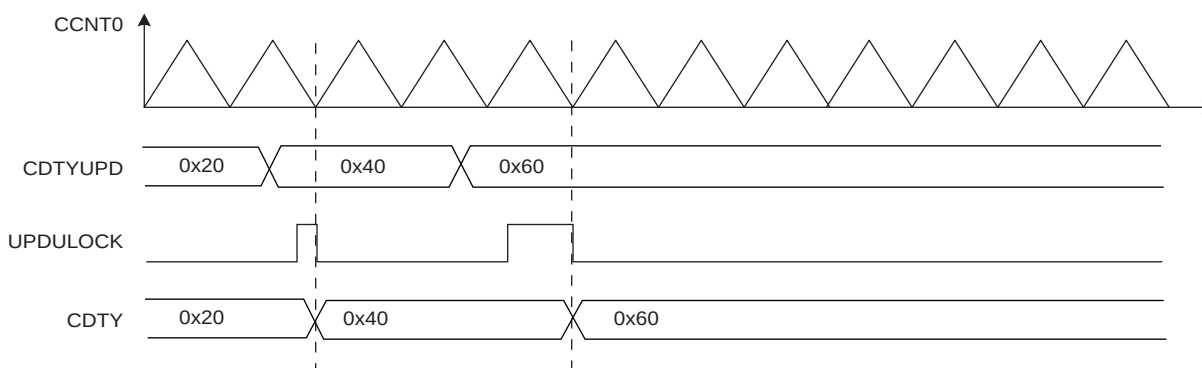
Figure 38-9. Method 1 (UPDM = 0)
