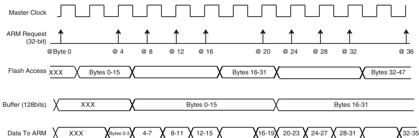
Figure 21-4. Data Read Optimization for FWS = 1
