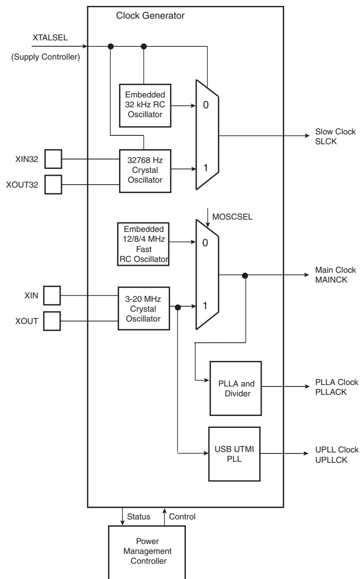
Figure 27-1. Clock Generator Block Diagram
