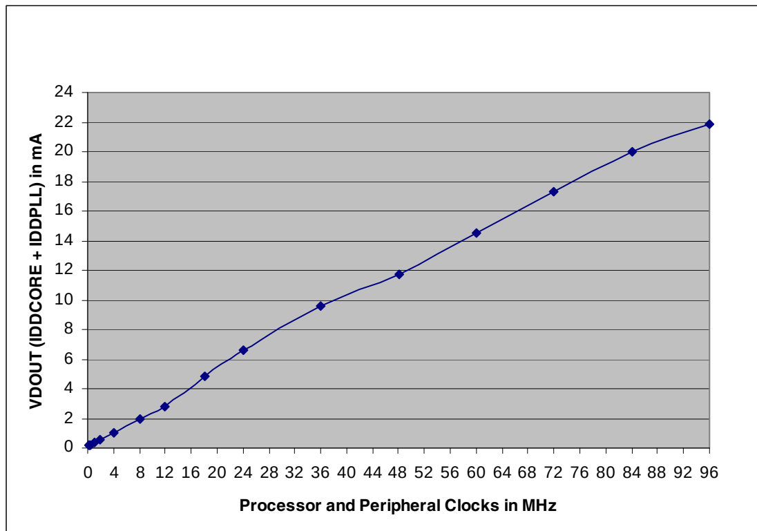
Figure 43-7. Current Consumption in Sleep Mode (AMP1) versus Master Clock ranges (Condition from Table 43-10 )
