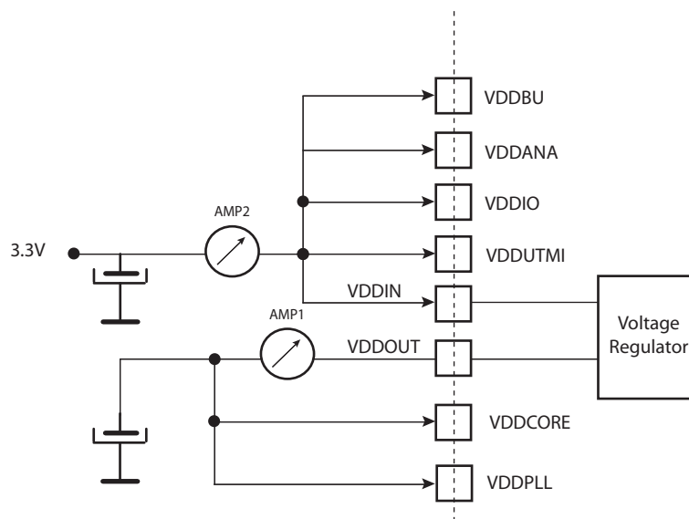
Figure 43-6. Measurement Setup for Sleep Mode
