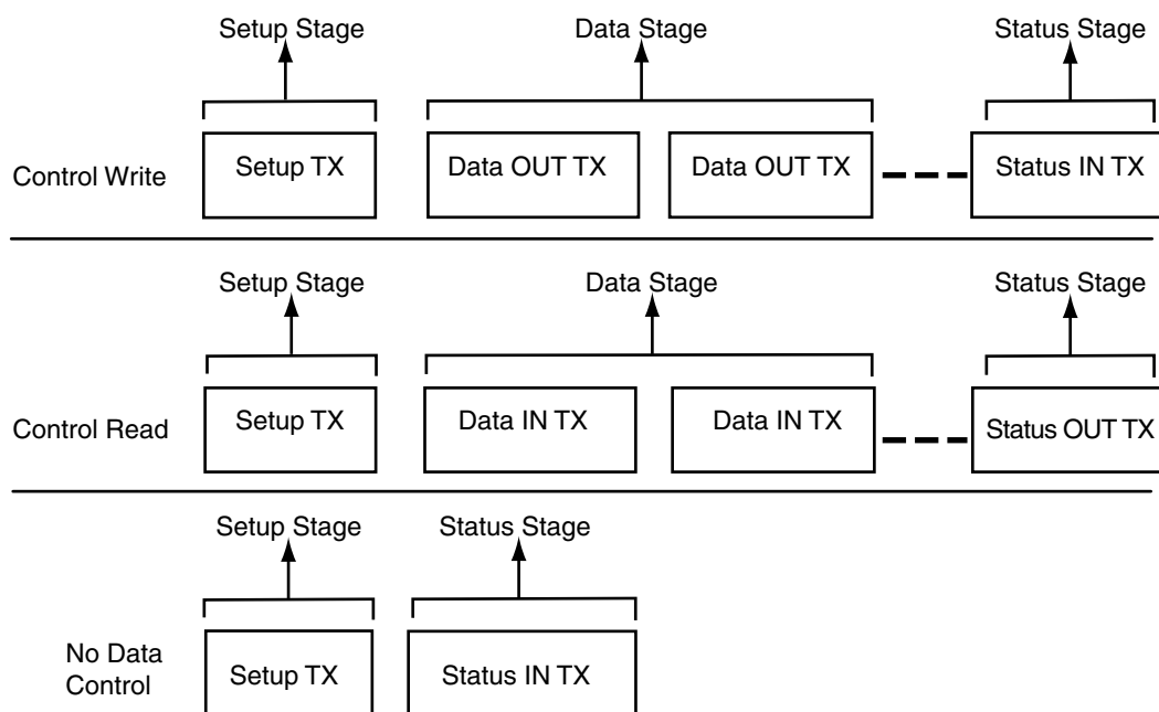
Figure 39-3. Control Read and Write Sequences
