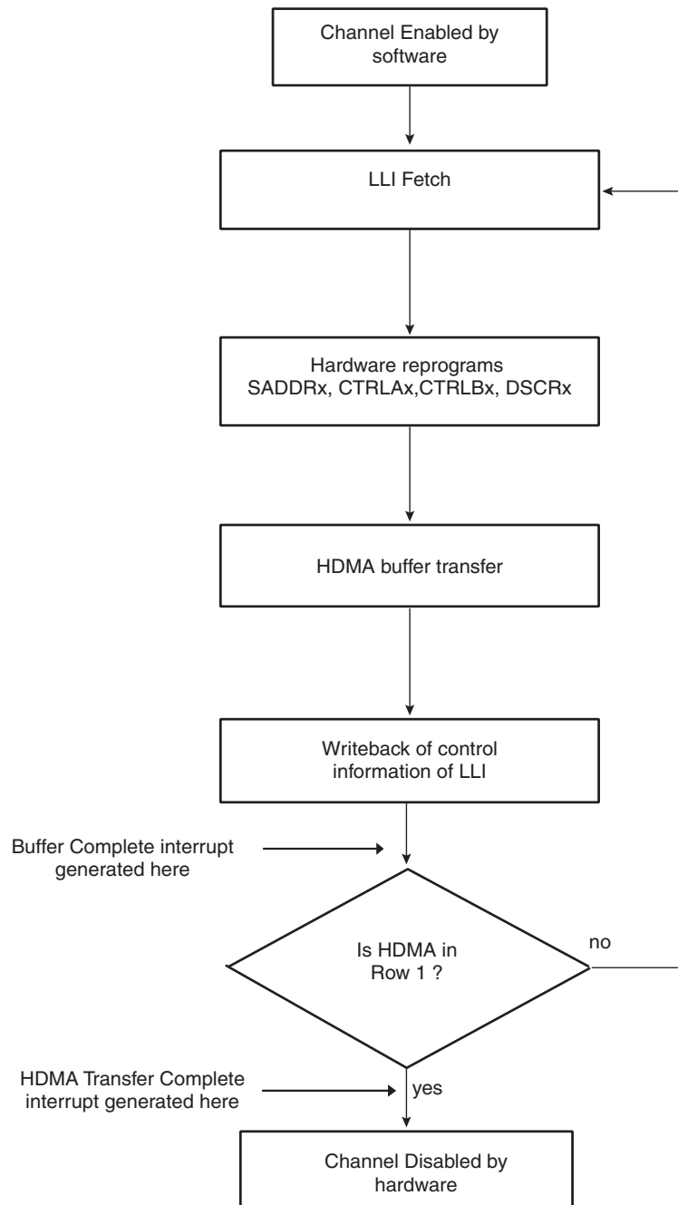
Figure 40-9. DMAC Transfer Flow for Linked List Source Address and Contiguous Destination Address
