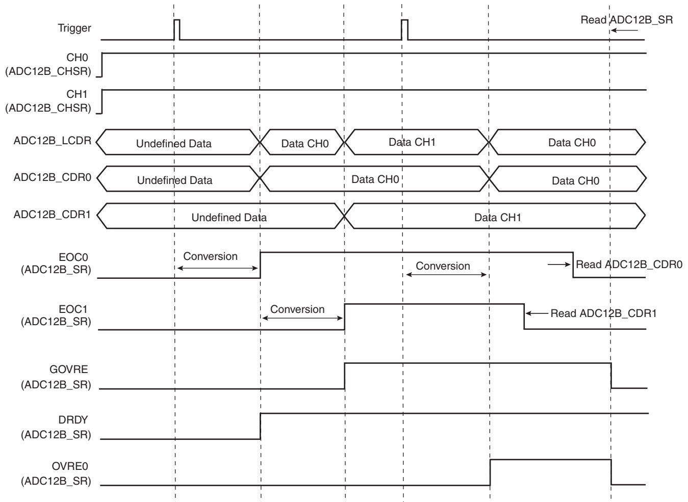
Figure 41-4. GOVRE and OVREx Flag Behavior
