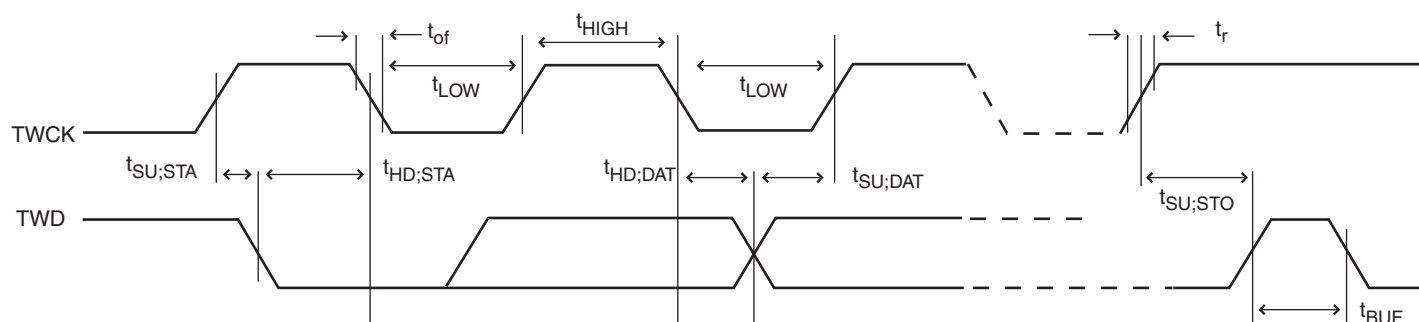
Figure 43-30. Two-wire Serial Bus Timing
