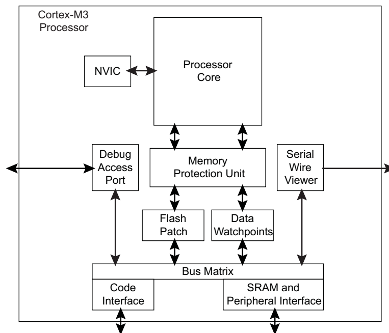
Figure 13-1. Typical Cortex-M3 implementation
