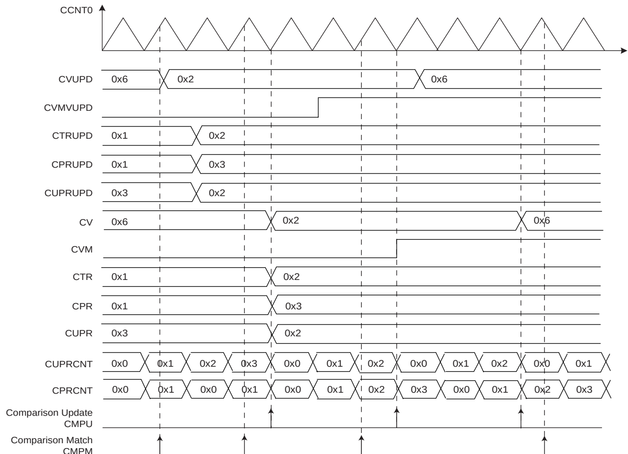
Figure 38-14. Comparison Waveform
