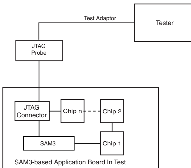
Figure 14-3. Application Test Environment Example
