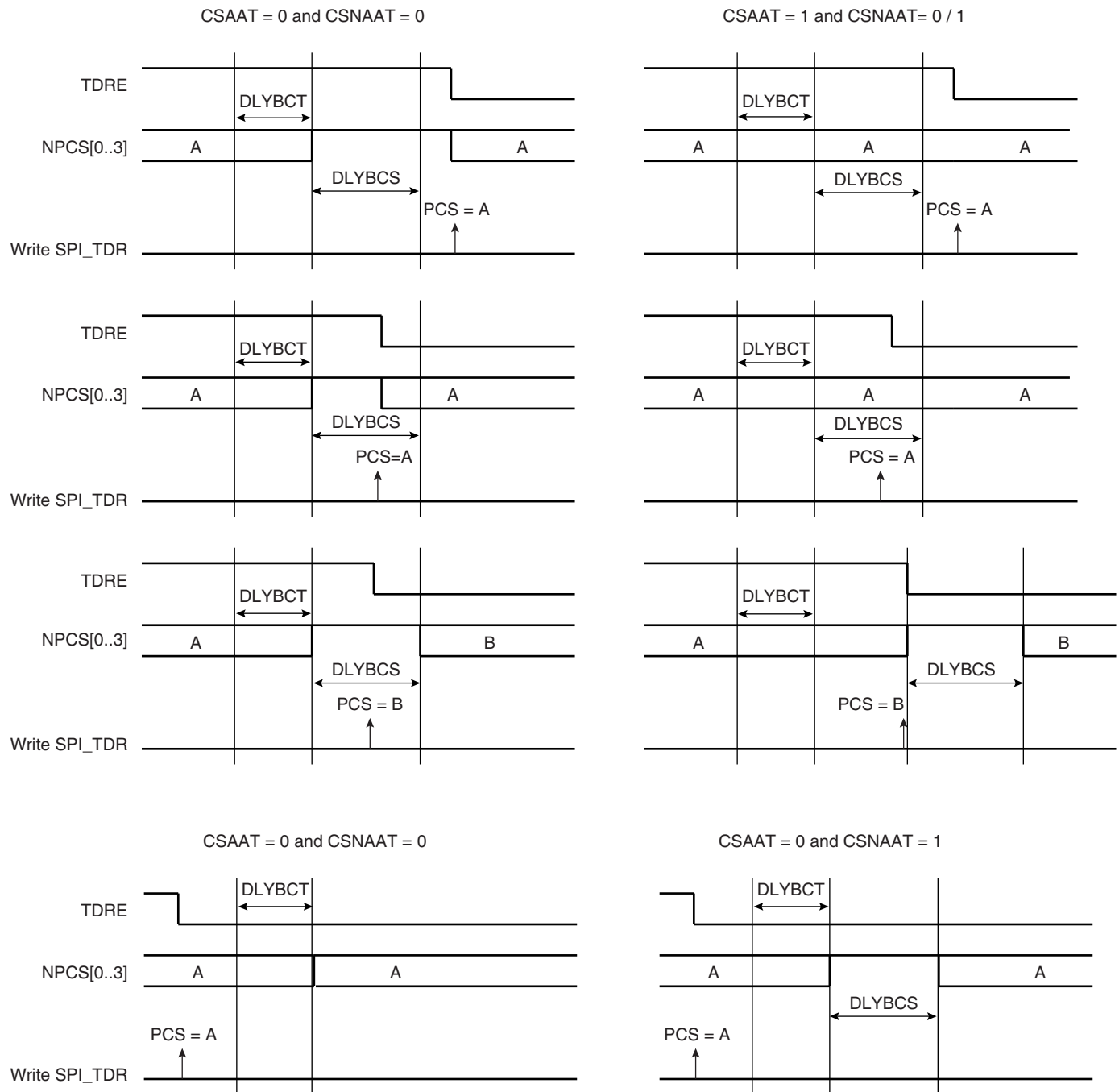
Figure 32-10. Peripheral Deselection
