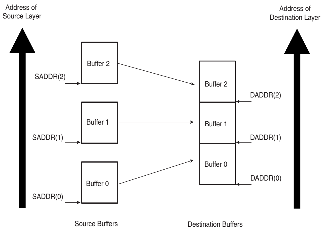
Figure 40-8. DMAC Transfer with Linked List Source Address and Contiguous Destination Address
