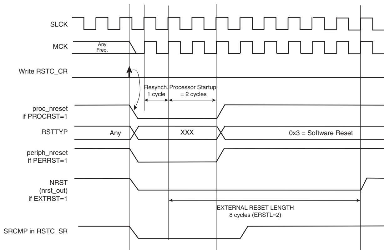
Figure 16-5. Software Reset
