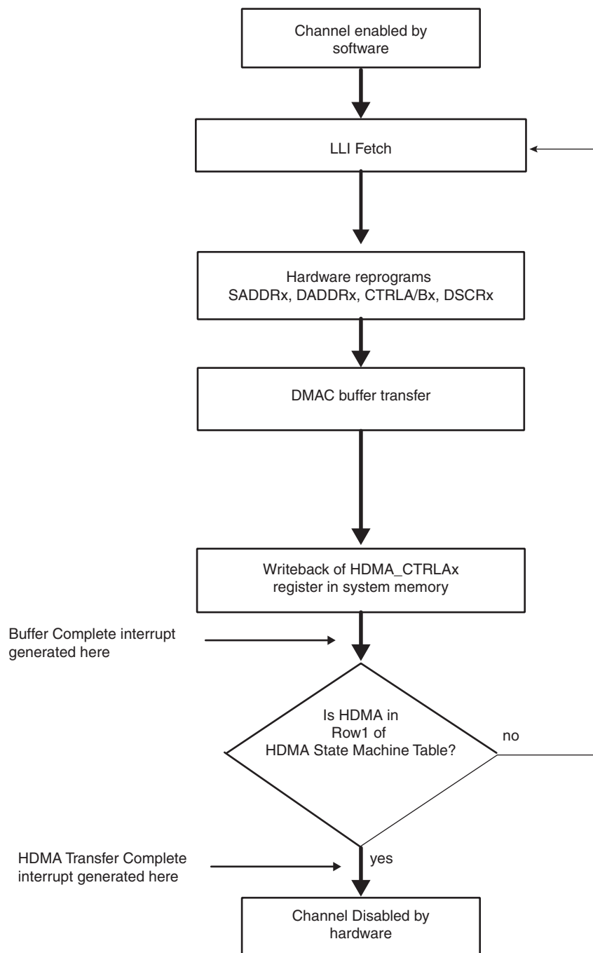
Figure 40-7. DMAC Transfer Flow for Source and Destination Linked List Address
