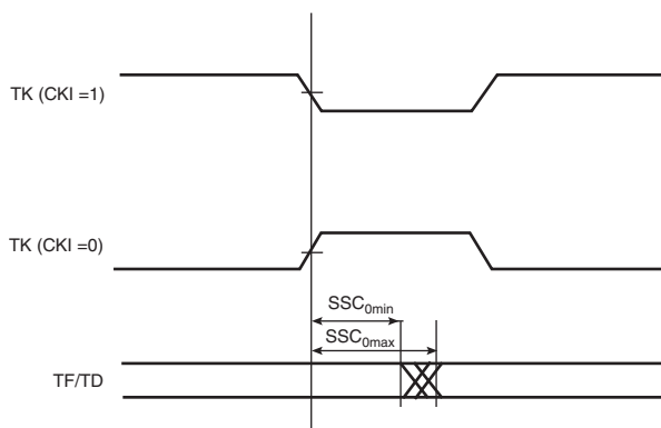
Figure 43-24. Min and Max Access Time of Output Signals
