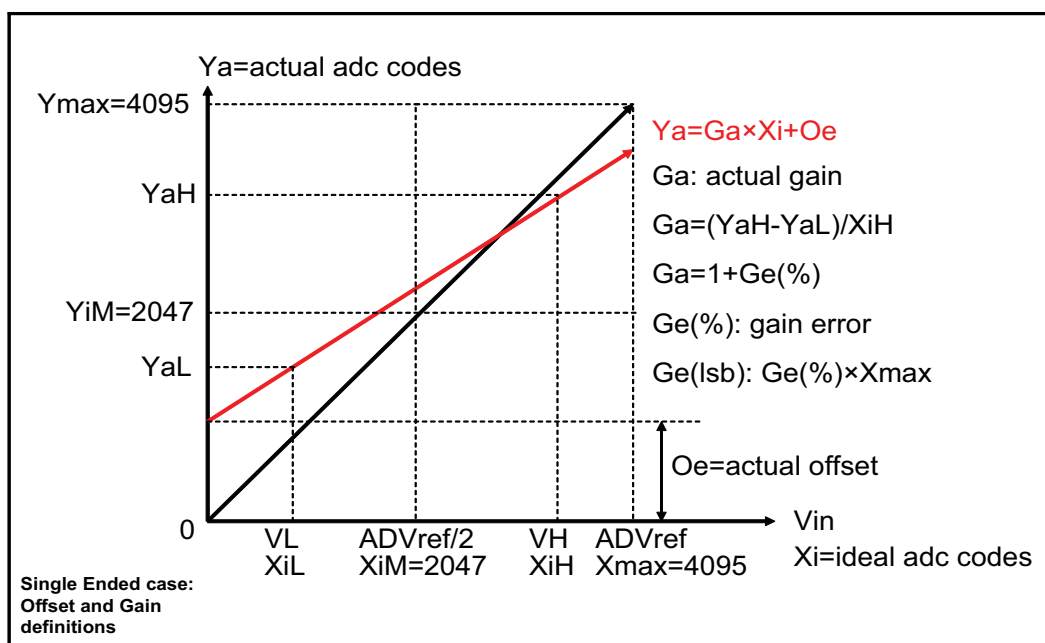
Figure 43-10. Offset and Gain Definitions
