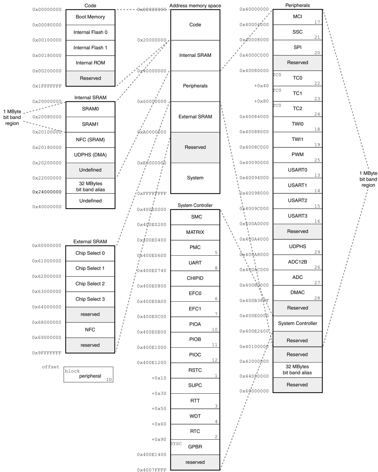
Figure 8-1. ATSAM3U4/2/1 Memory Mapping
