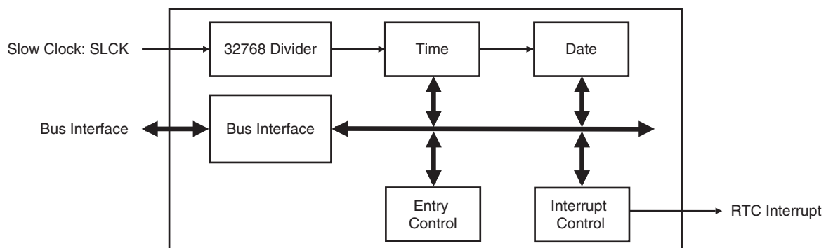
Figure 18-1. RTC Block Diagram
