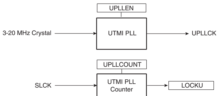
Figure 27-5. UTMI PLL Block Diagram
