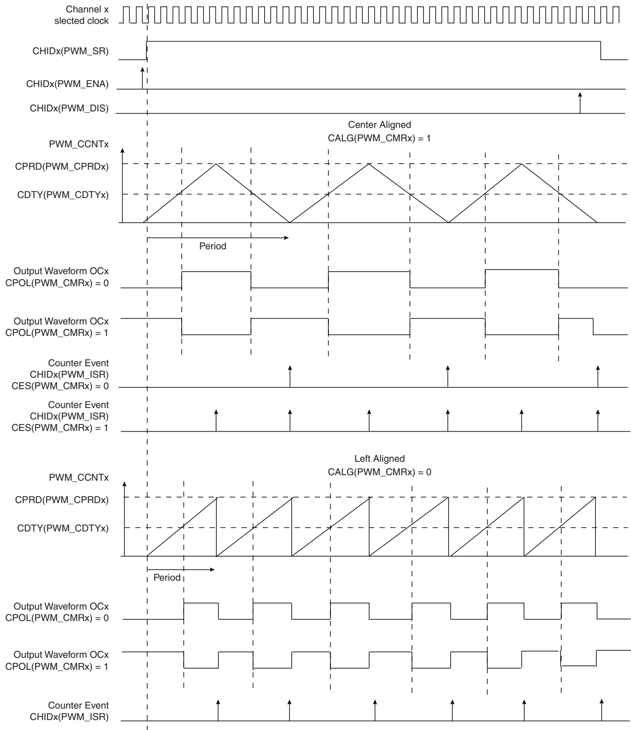
Figure 38-5. Waveform Properties
