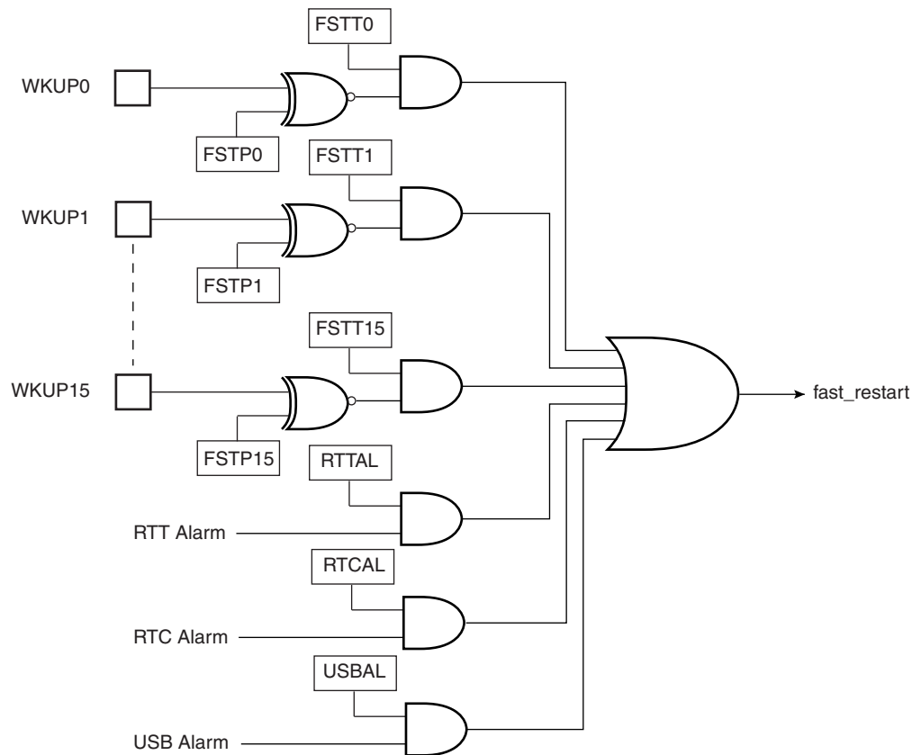
Figure 28-3. Fast Startup Circuitry
