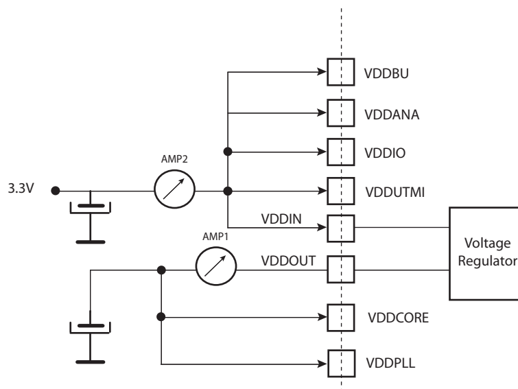
Figure 43-9. Active Mode Measurement Setup
