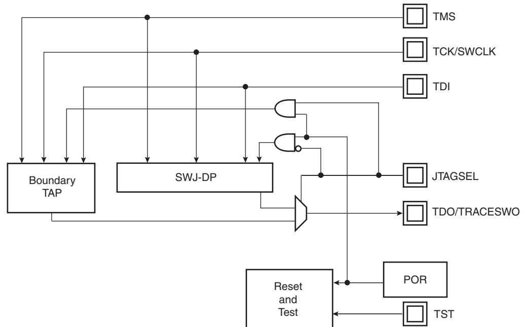
Figure 14-1. Debug and Test Block Diagram
