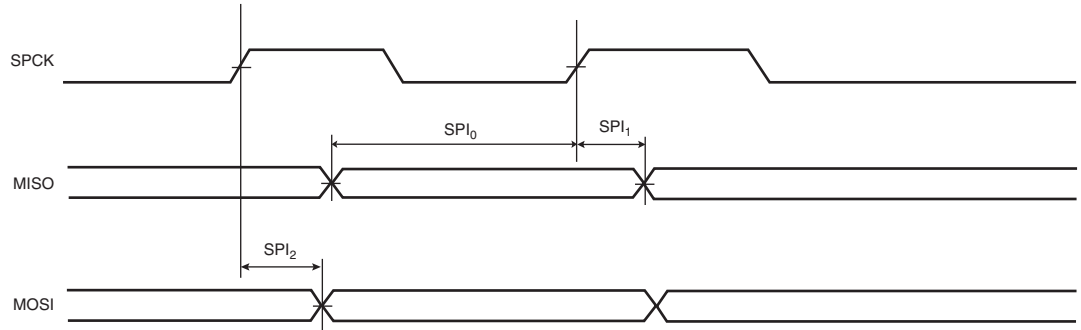
Figure 43-12. SPI Master Mode with (CPOL= NCPHA = 0) or (CPOL= NCPHA= 1)
