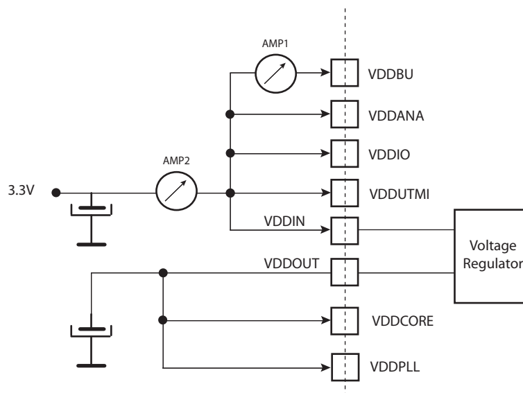
Figure 43-5. Measurement Setup
