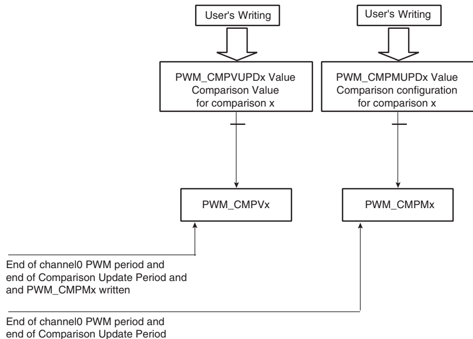
Figure 38-18. Synchronized Update of Comparison Values and Configurations
