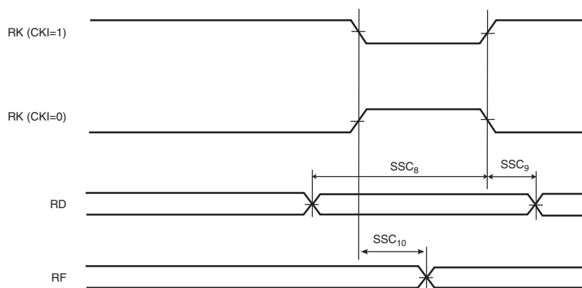
Figure 43-21. SSC Receiver, RK as input and RF as output
