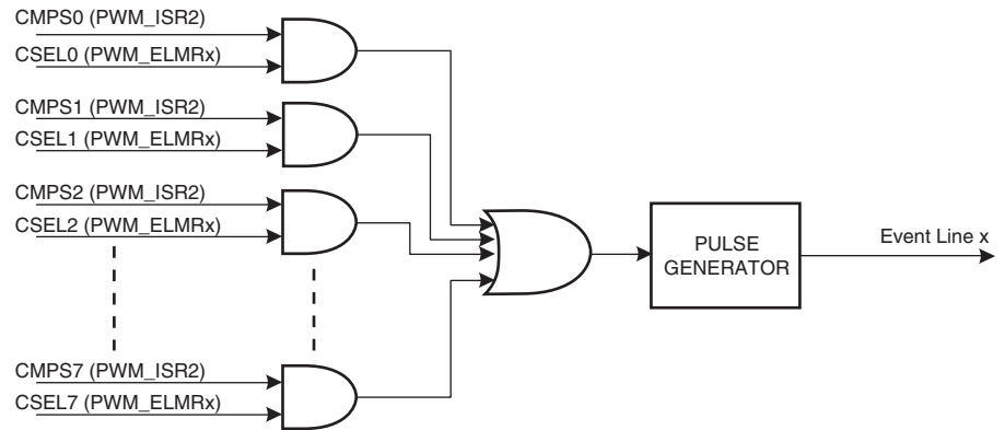
Figure 38-15. Event Line Block Diagram
