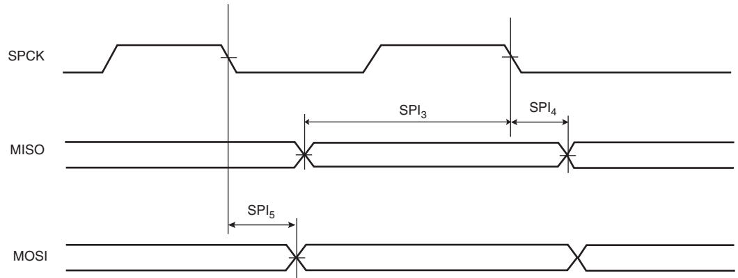
Figure 43-13. SPI Master Mode with (CPOL = 0 and NCPHA=1) or (CPOL=1 and NCPHA= 0)
