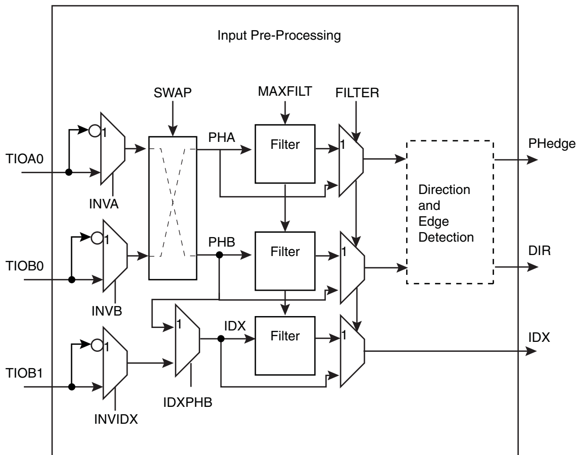
Figure 36-16. Input Stage
