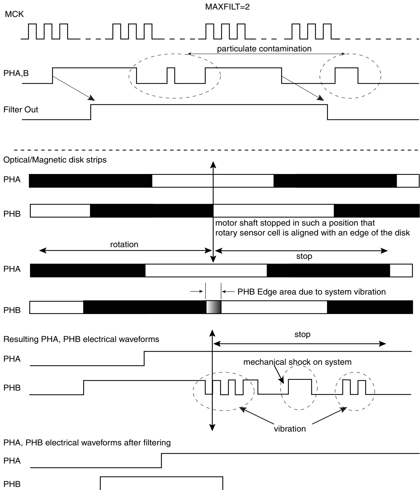
Figure 36-17. Filtering Examples
