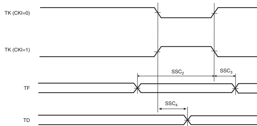
Figure 43-18. SSC Transmitter, TK as output and TF as input
