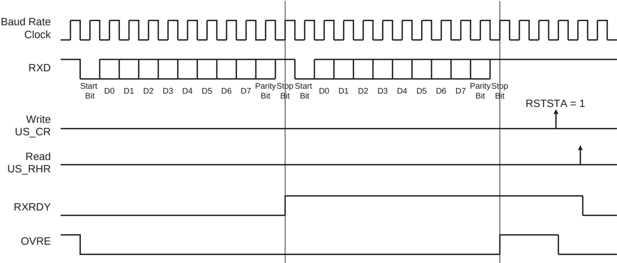
Figure 36-20. Receiver Status
