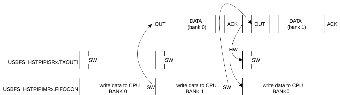
Figure 45-26. Example of an OUT Pipe with two Data Banks and a Bank Switching Delay
