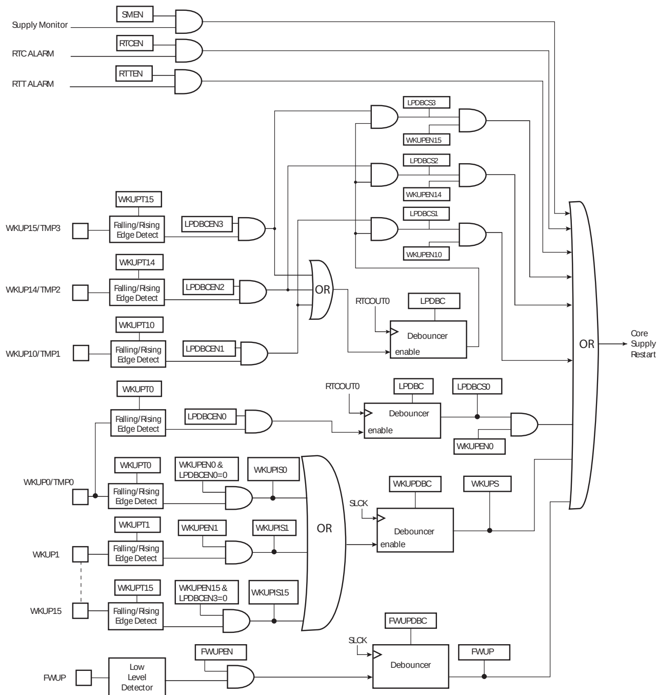
Figure 20-4. SAM4C16/8/4 Wake-up Sources
