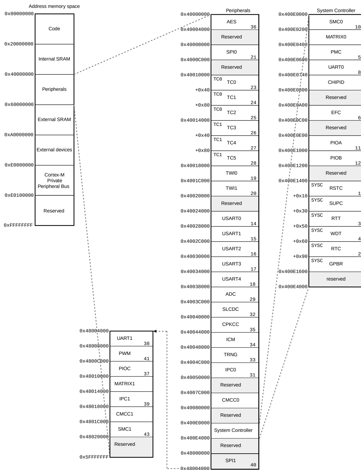
Figure 7-4. SAM4C16/8/4 Memory Mapping of the Peripherals Area
