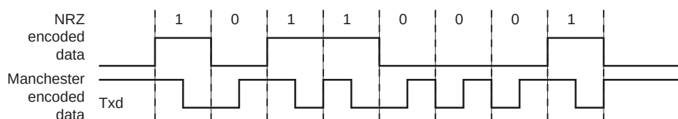
Figure 36-7. NRZ to Manchester Encoding
