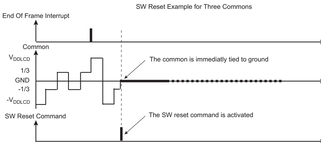
Figure 39-11. Software Reset
