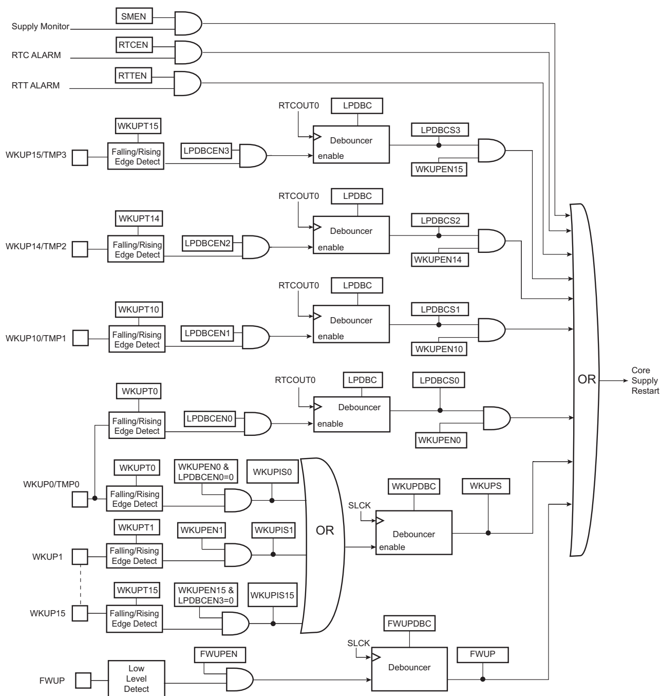
Figure 20-5. SAM4C32 Wake-up Sources
