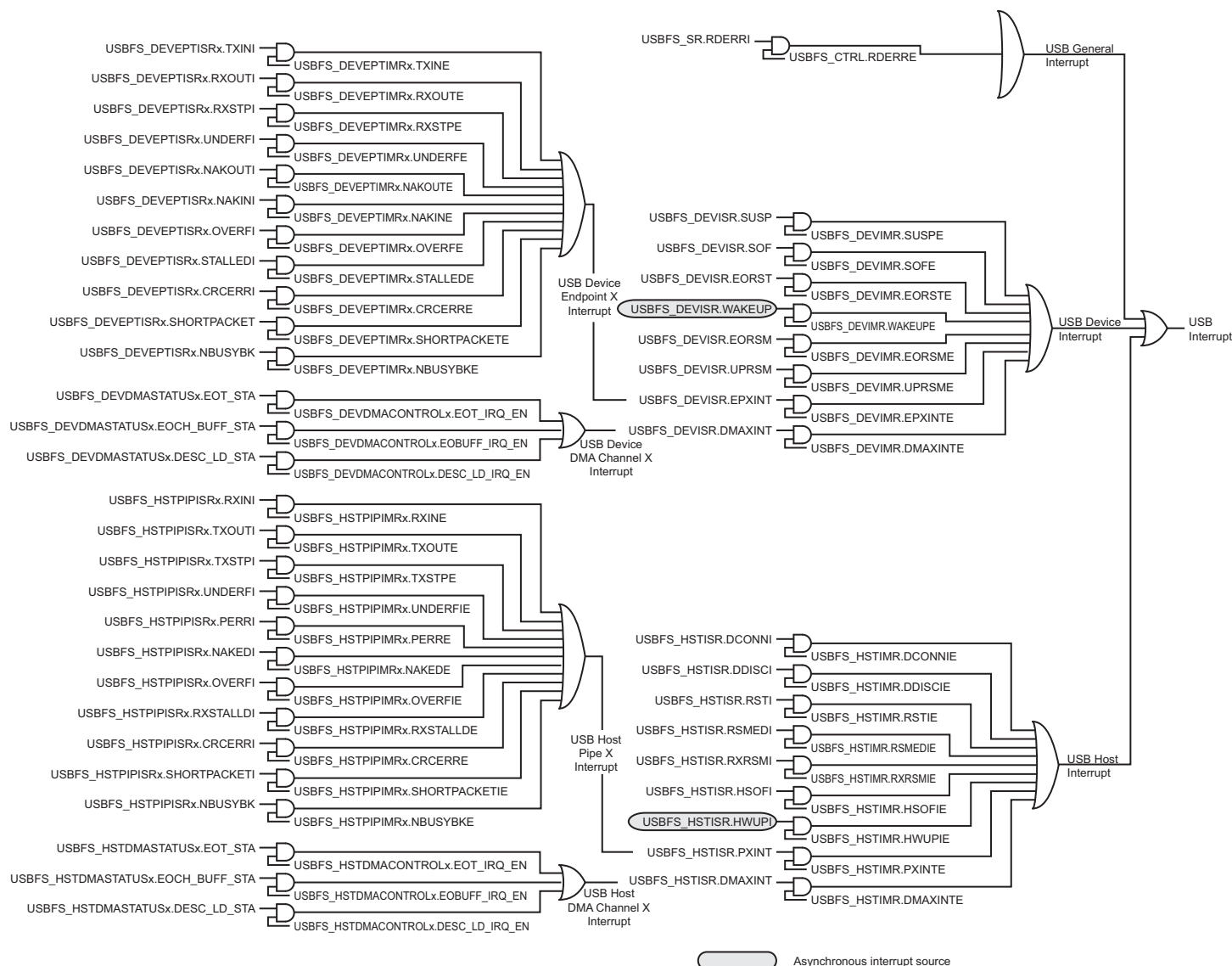
Figure 45-6. Interrupt System
