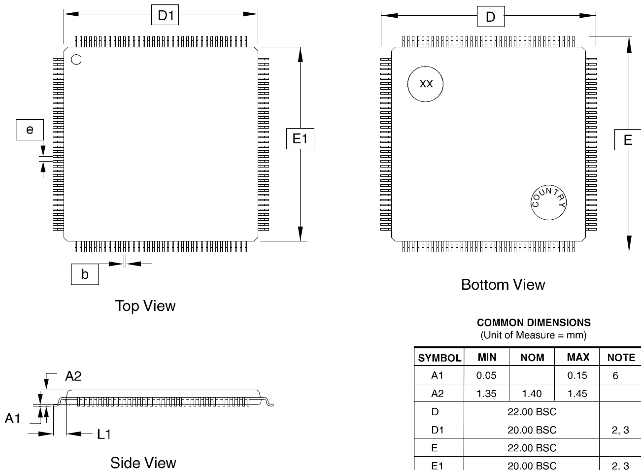
Figure 47-2. 144-lead LQFP Package Mechanical Drawing
