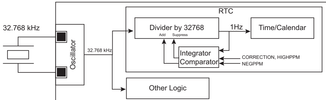
Figure 17-3. Calibration Circuitry
