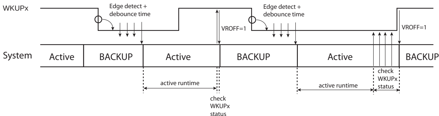
Figure 20-6. Entering and Exiting Backup Mode with a WKUP pin
