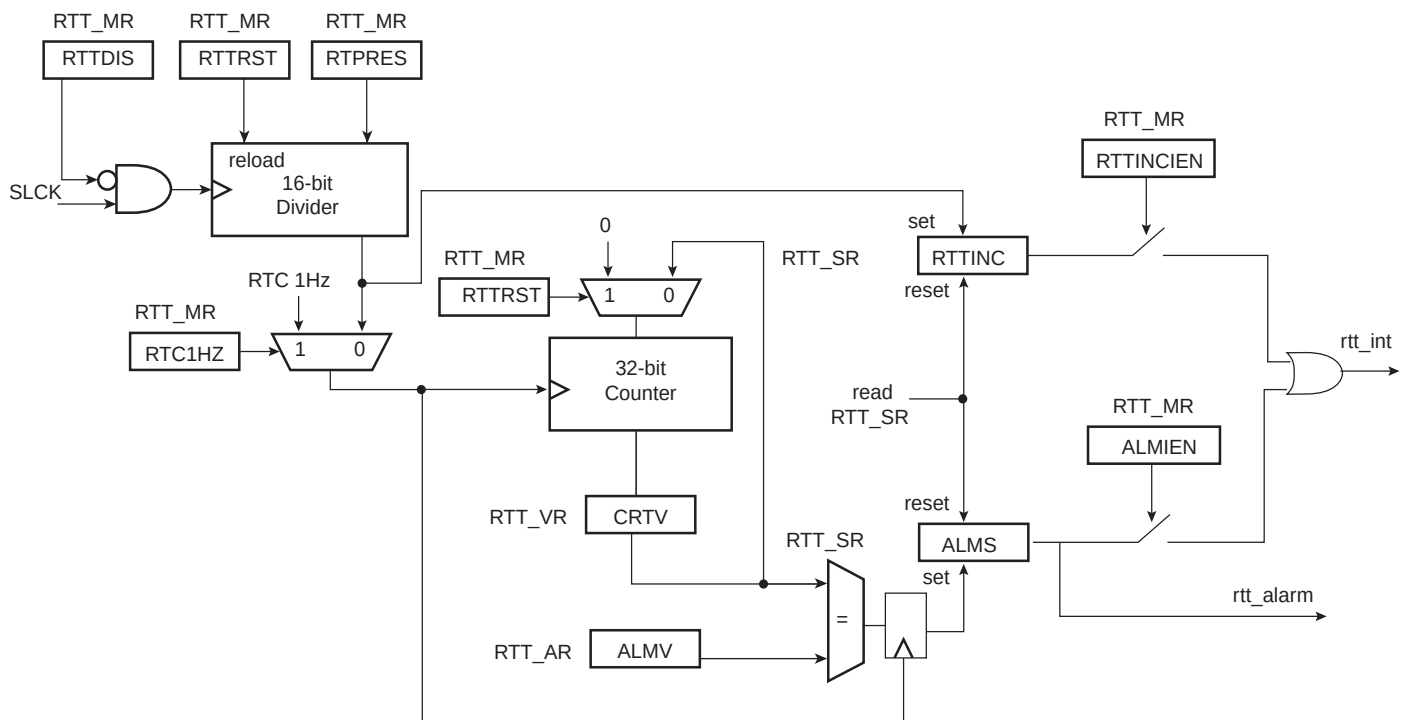
Figure 16-1. Real-time Timer
