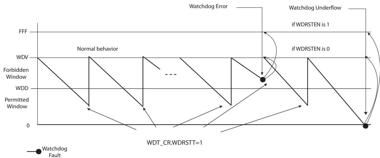
Figure 18-2. Watchdog Behavior
