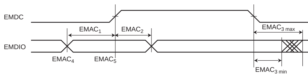
Figure 46-26. Min and Max Access Time of EMAC Output Signals
