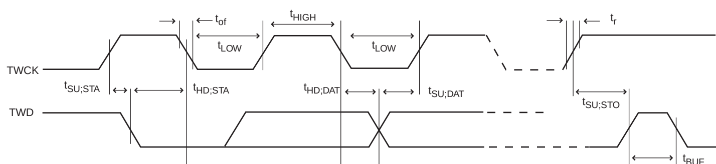
Figure 46-25. Two-wire Serial Bus Timing
