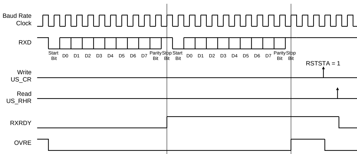
Figure 37-21. Receiver Status
