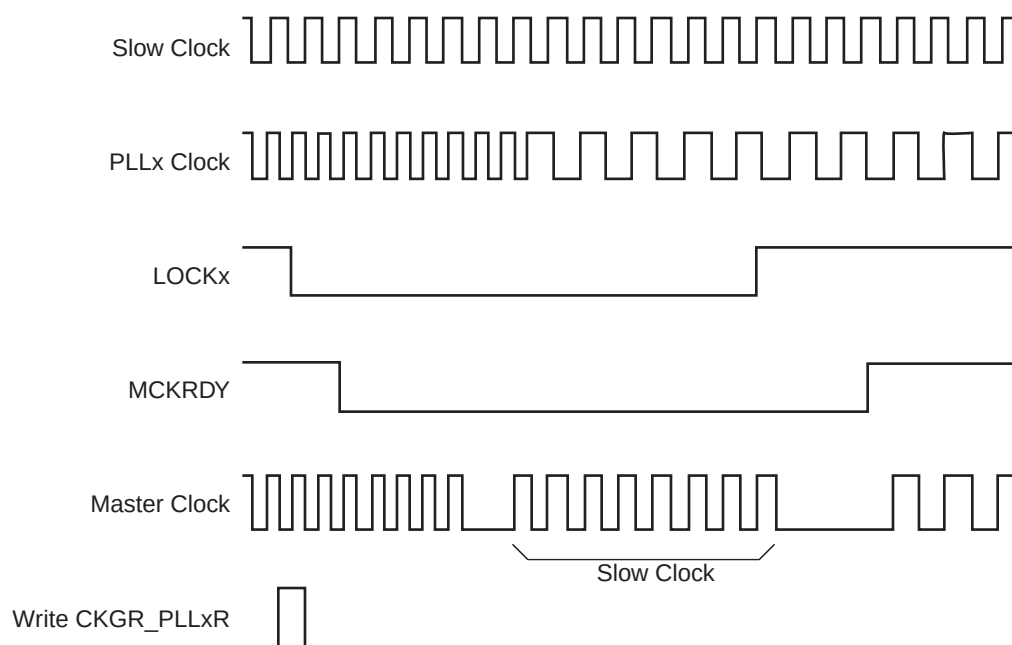
Figure 30-11. Change PLLx Programming
