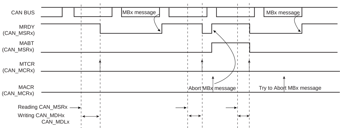
Figure 32-15. Transmitting Messages
