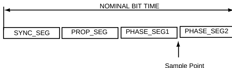
Figure 32-4. Partition of the CAN Bit Time
