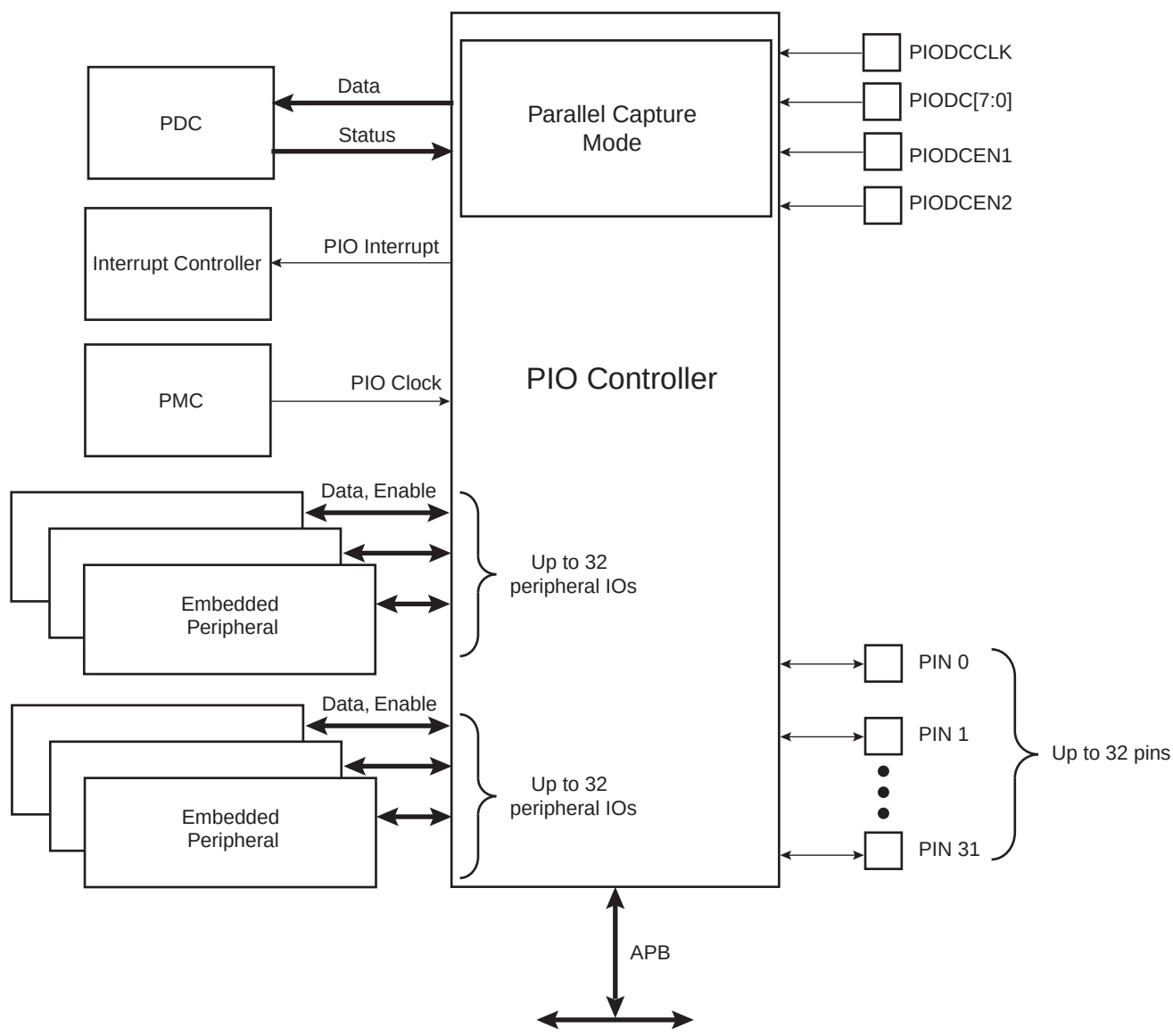
Figure 33-1. Block Diagram
