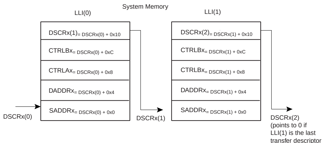
Figure 26-4. Multi Buffer Transfer Using Linked List
