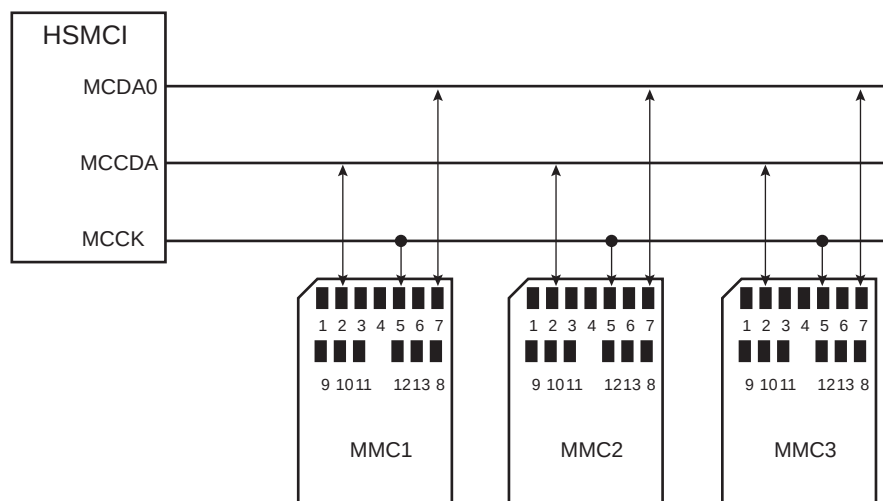
Figure 41-4. MMC Bus Connections (One Slot)
