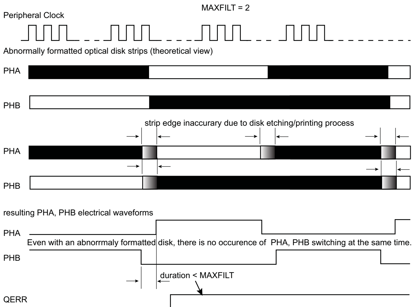
Figure 39-21. Quadrature Error Detection
