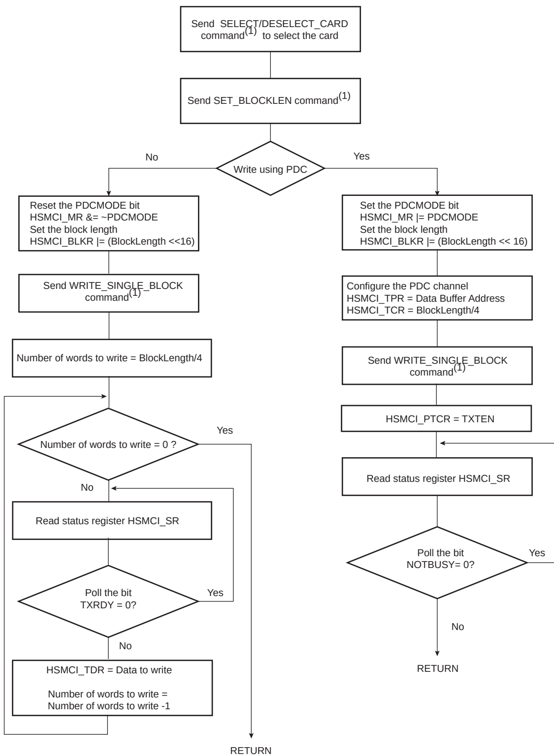
Figure 41-9. Write Functional Flow Diagram
