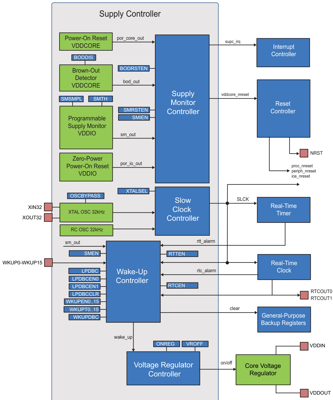
Figure 19-1. Supply Controller Block Diagram
