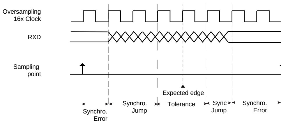
Figure 38-11. Bit Resynchronization
