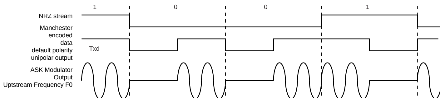
Figure 38-18. ASK Modulator Output
