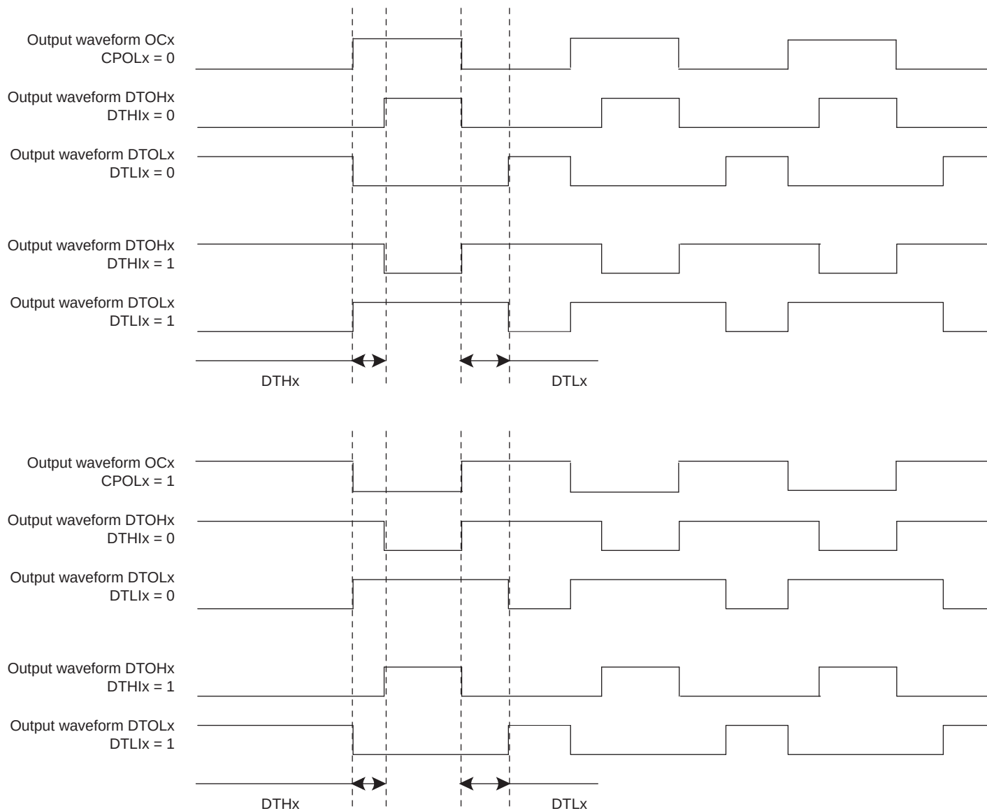
Figure 40-7. Complementary Output Waveforms
