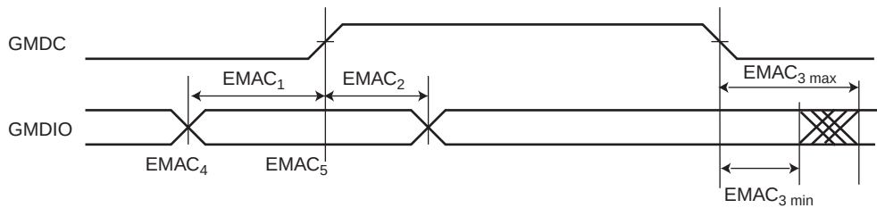
Figure 47-29. Min and Max Access Time of EMAC Output Signals
