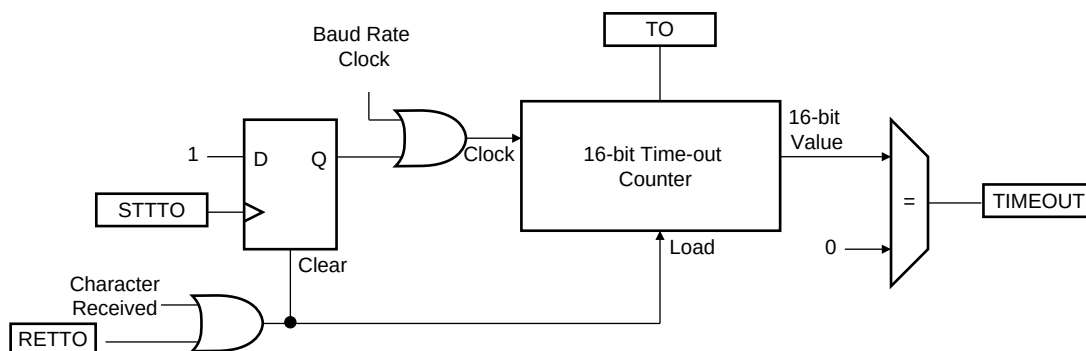
Figure 38-24. Receiver Time-out Block Diagram
