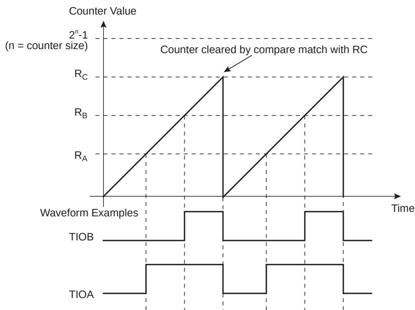
Figure 39-10. WAVSEL = 10 without Trigger
