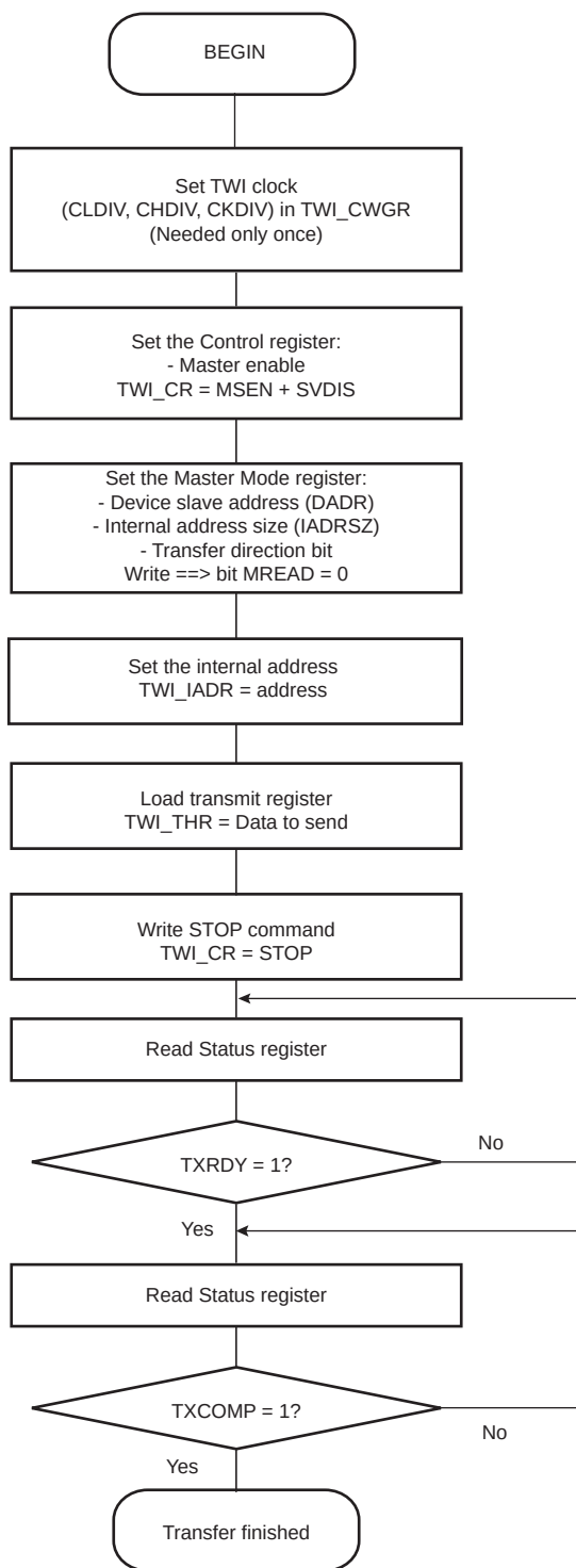
Figure 36-17. TWI Write Operation with Single Data Byte and Internal Address
