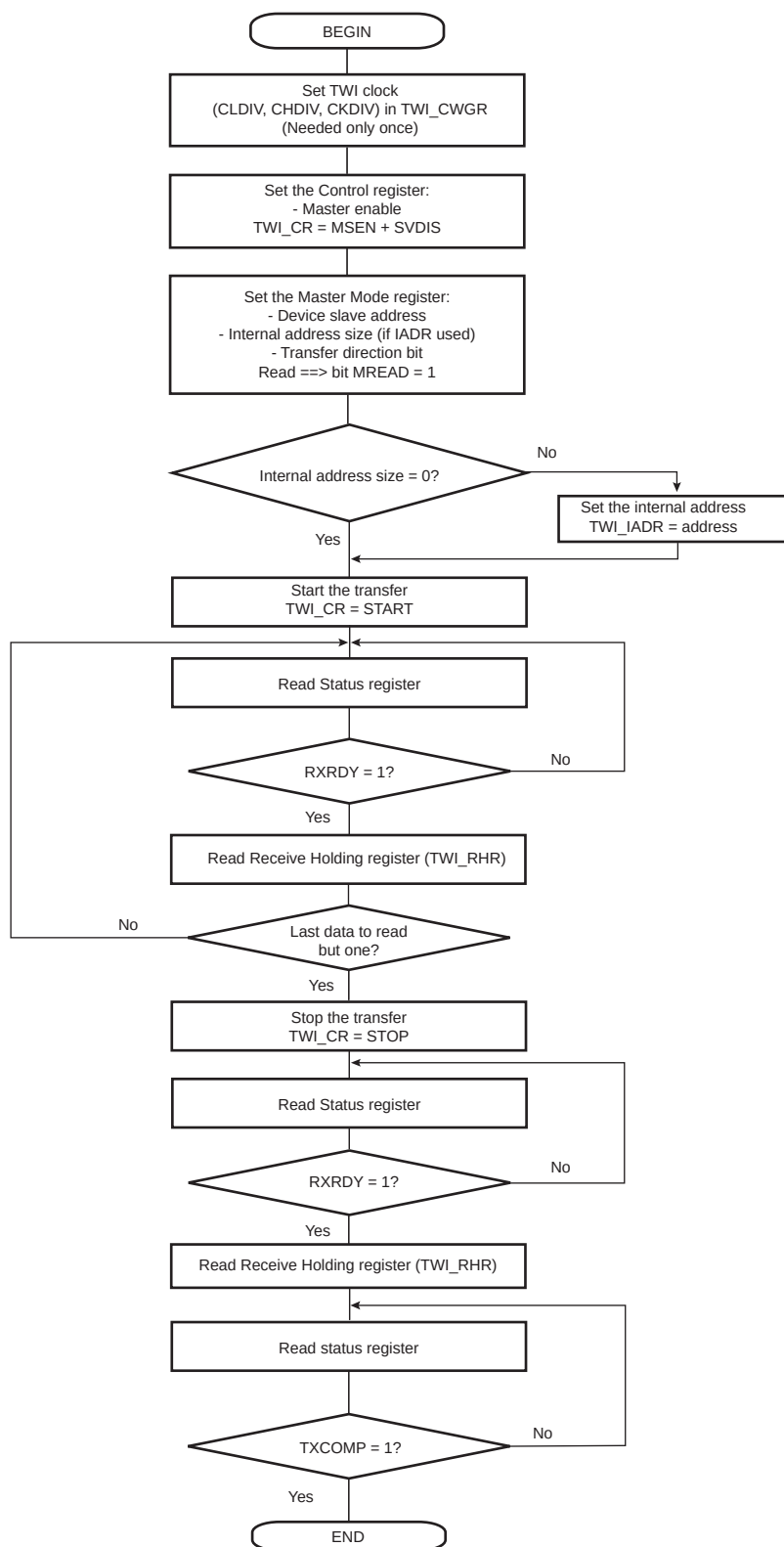
Figure 36-21. TWI Read Operation with Multiple Data Bytes with or without Internal Address
