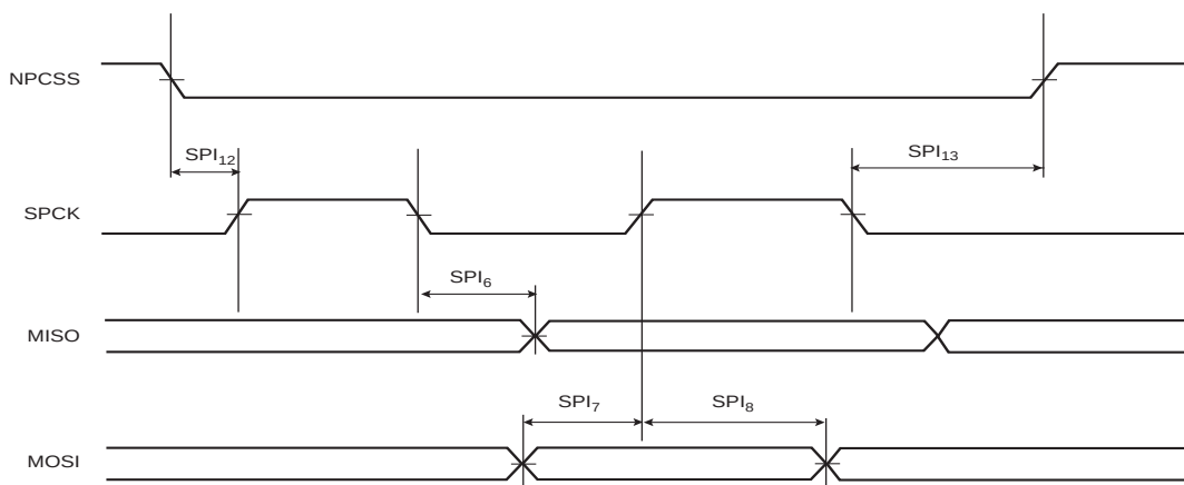
Figure 47-21. SPI Slave Mode with (CPOL=0 and NCPHA=1) or (CPOL=1 and NCPHA=0)
