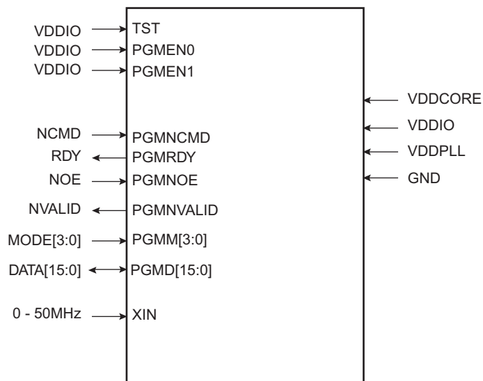
Figure 22-1. SAM4ExE Parallel Programming Interface
