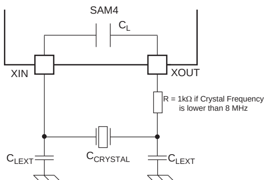
Figure 47-12. 3 to 20 MHz Crystal Oscillator Schematics
