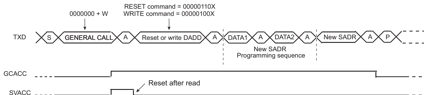
Figure 36-28. Master Performs a General Call
