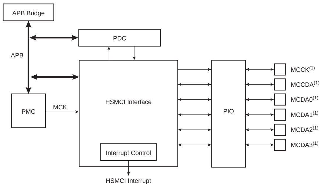
Figure 41-1. Block Diagram (4-bit configuration)
