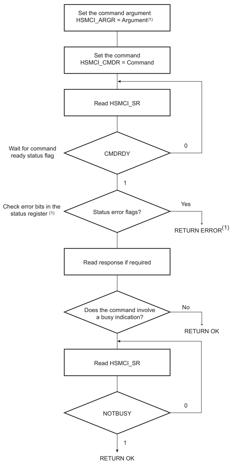
Figure 41-7. Command/Response Functional Flow Diagram
