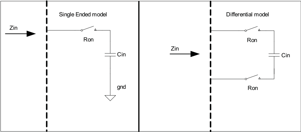
Figure 47-17. Input Channel Model
