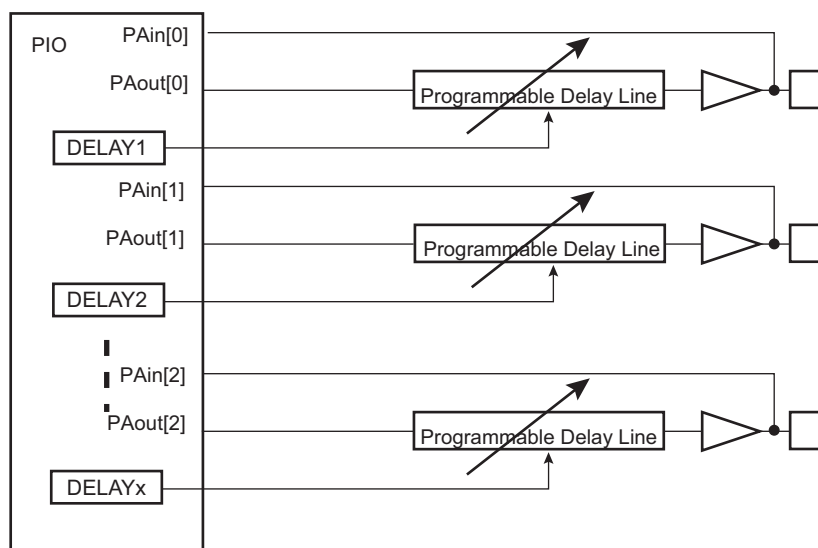
Figure 34-9. Programmable I/O Delays
