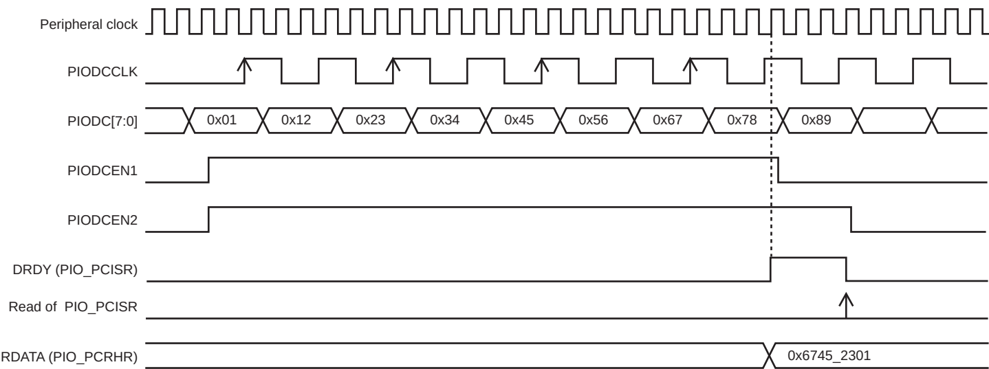
Figure 34-13. Parallel Capture Mode Waveforms (DSIZE = 2, ALWAYS = 0, HALFS = 1, FRSTS = 0)
