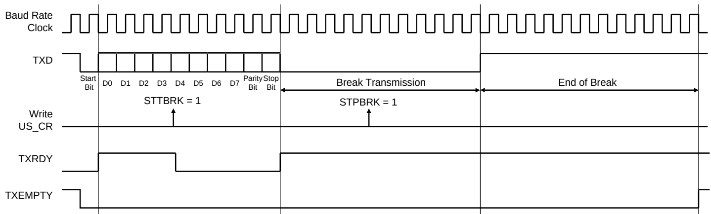
Figure 38-26. Break Transmission
