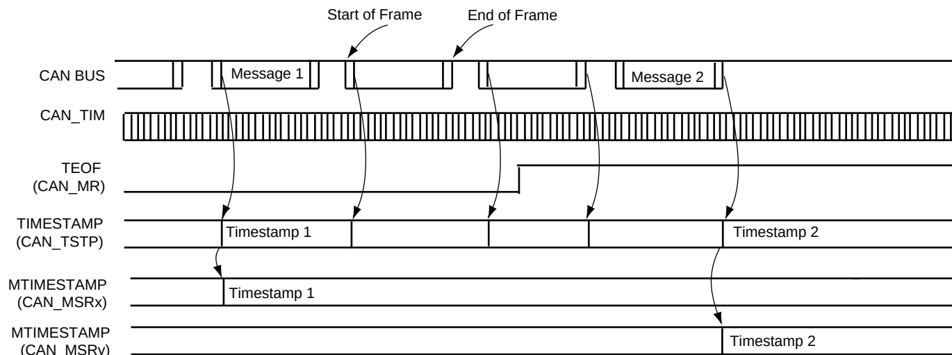
Figure 33-19. Mailbox Timestamp
