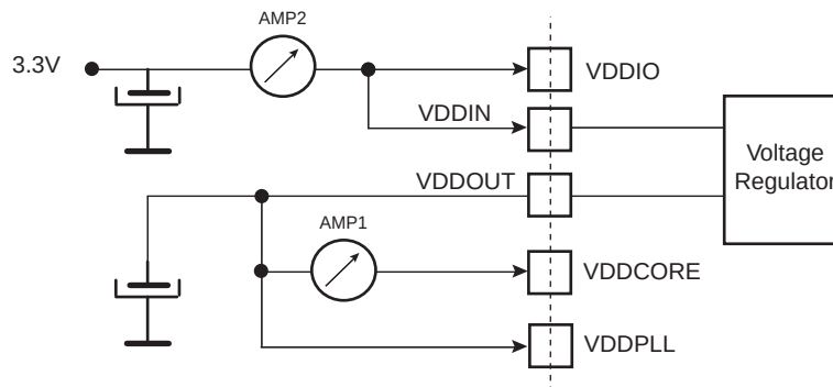
Figure 47-5. Measurement Setup for Sleep Mode
