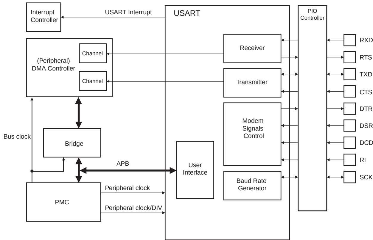
Figure 38-1. USART Block Diagram
