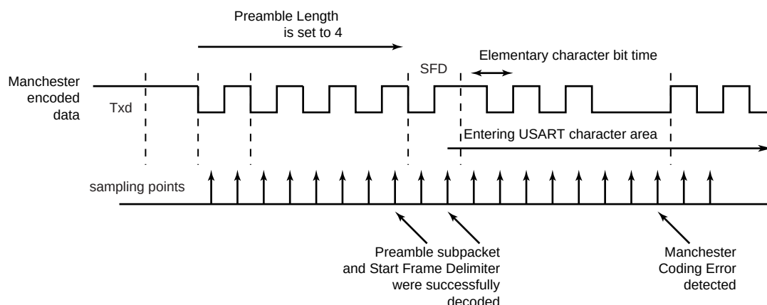
Figure 38-16. Manchester Error Flag
