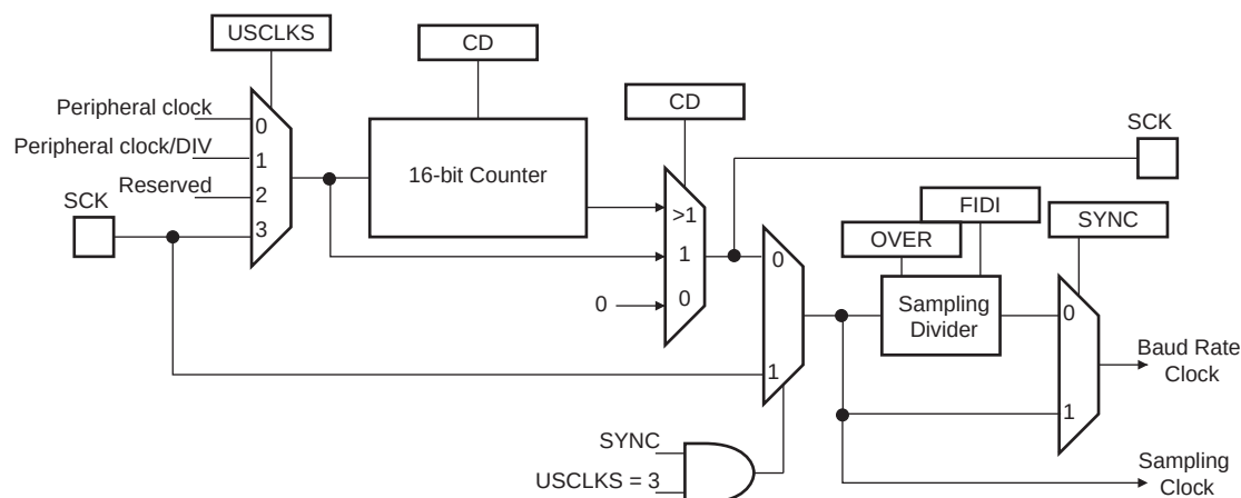
Figure 38-3. Baud Rate Generator
