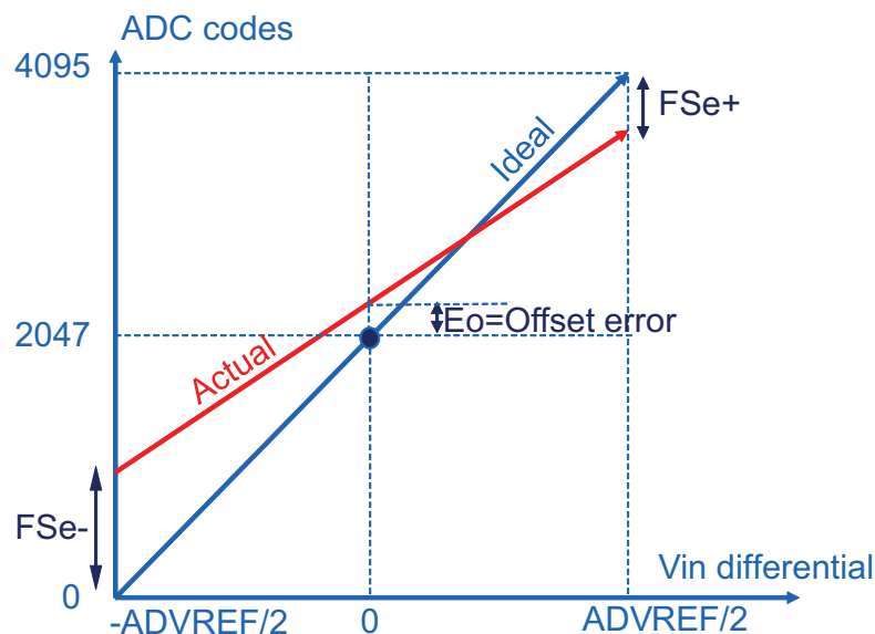
Figure 47-15. Gain and Offset Errors in Differential Mode
