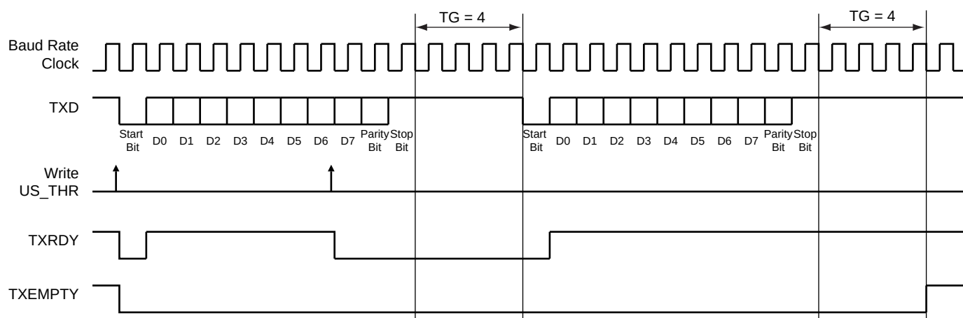
Figure 38-23. Timeguard Operations
