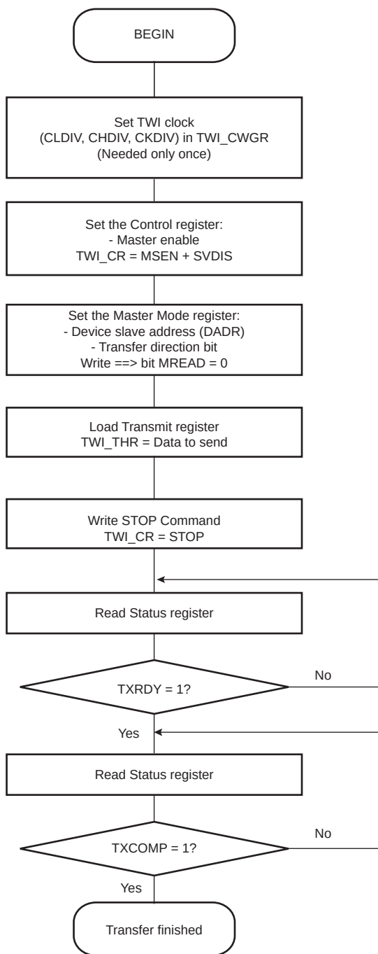
Figure 36-16. TWI Write Operation with Single Data Byte without Internal Addressf
