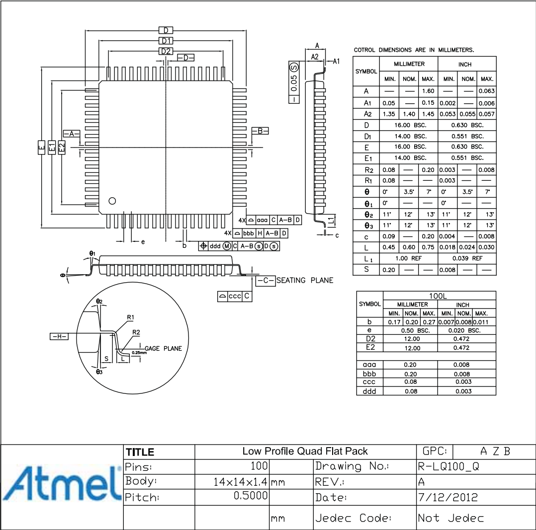
Figure 48-3. 100-lead LQFP Package Drawing
