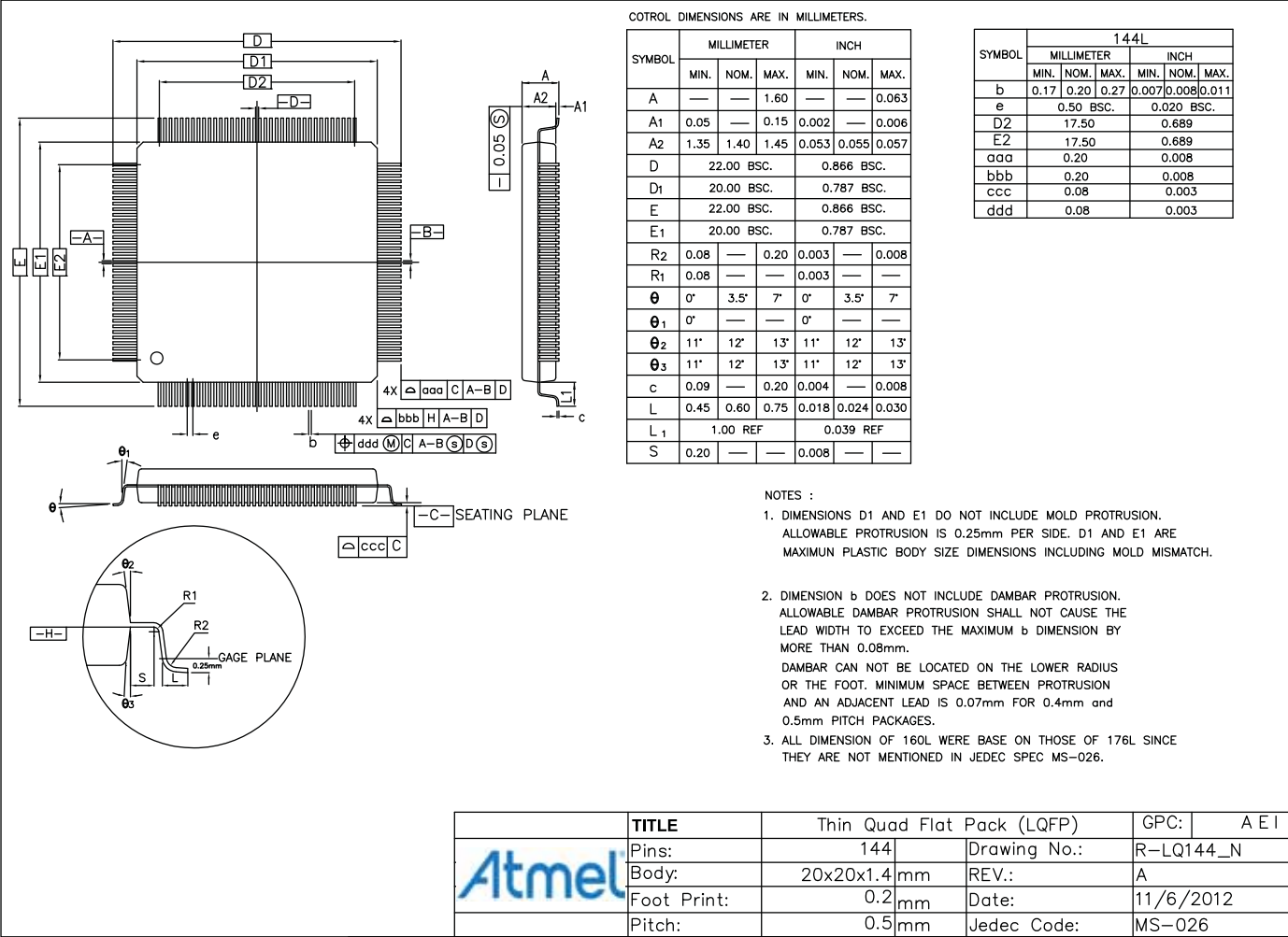
Figure 48-4. 144-lead LQFP Package Drawing
