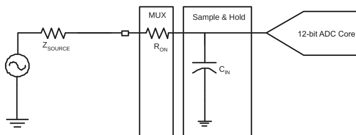
Figure 47-18. Simplified Acquisition Path
