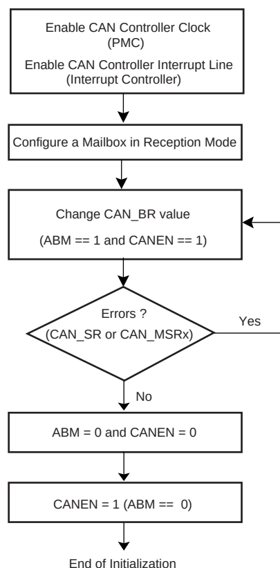
Figure 33-10. Possible Initialization Procedure
