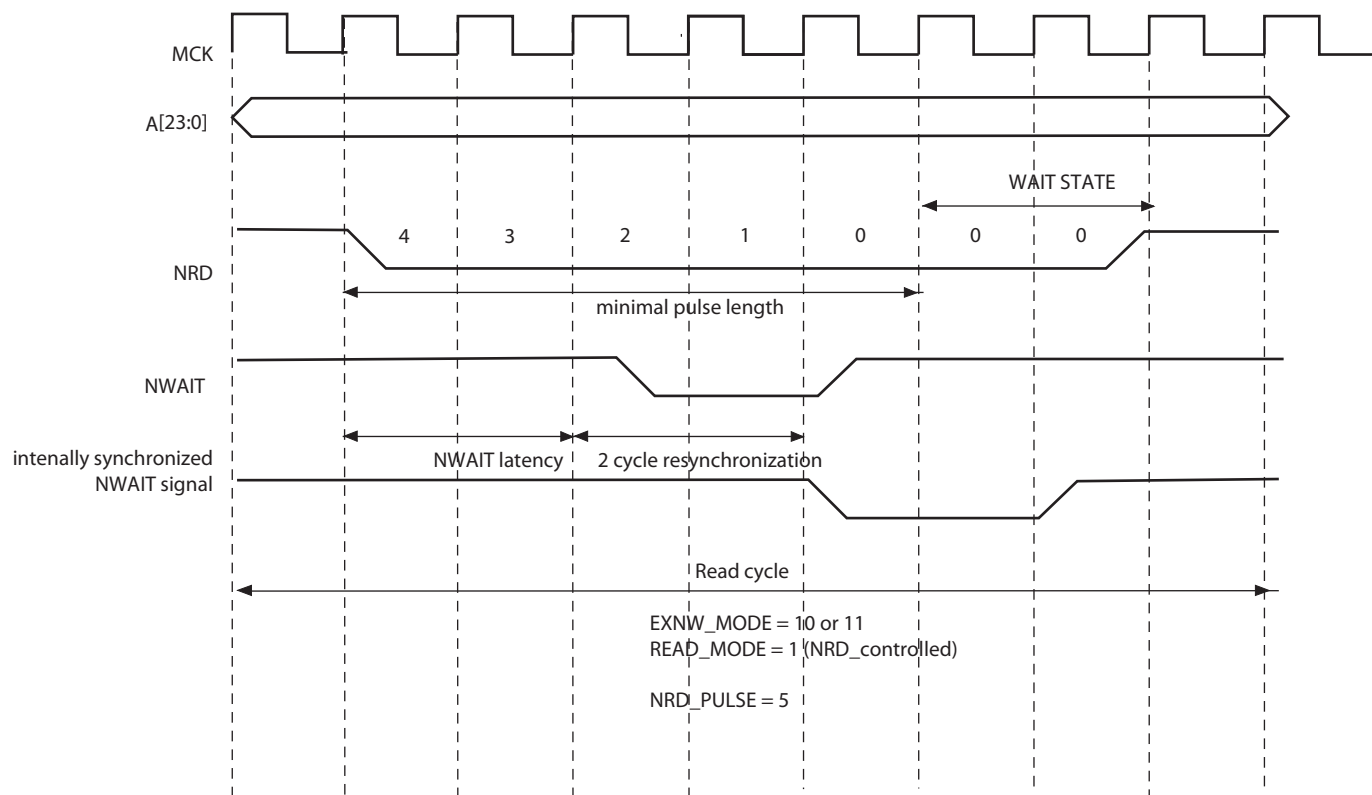
Figure 28-27. NWAIT Latency
