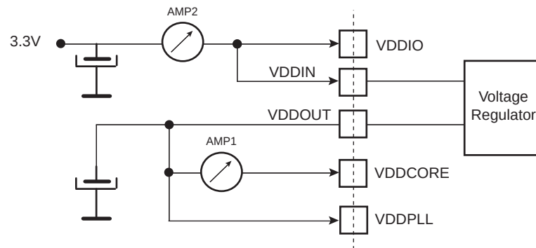
Figure 47-8. Active Mode Measurement Setup
