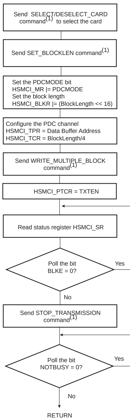
Figure 41-10. Multiple Write Functional Flow Diagram
