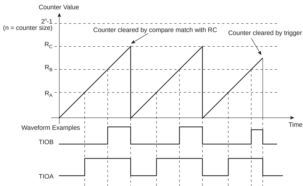
Figure 39-11. WAVSEL = 10 with Trigger
