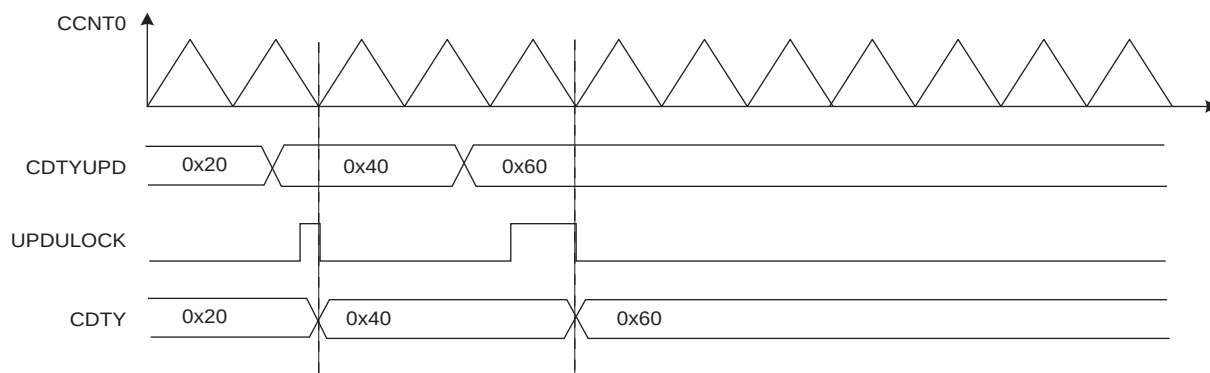
Figure 40-12. Method 1 (UPDM = 0)
