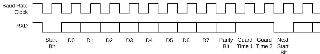
Figure 38-31. T = 0 Protocol without Parity Error
