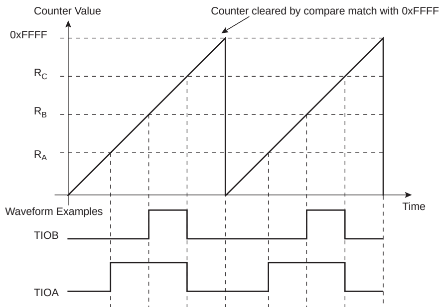
Figure 39-8. WAVSEL = 00 without trigger
