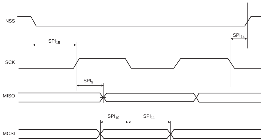
Figure 47-27. USART SPI Slave Mode (Mode 0 or 3)
