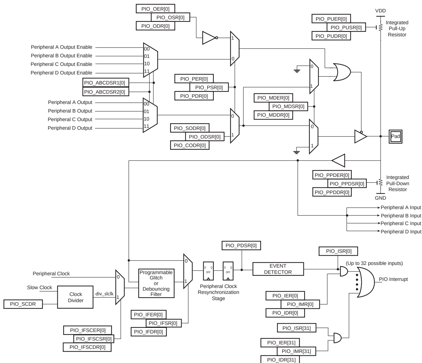
Figure 34-3. I/O Line Control Logic
