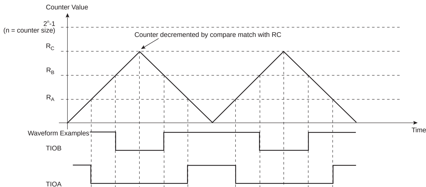
Figure 39-14. WAVSEL = 11 without Trigger
