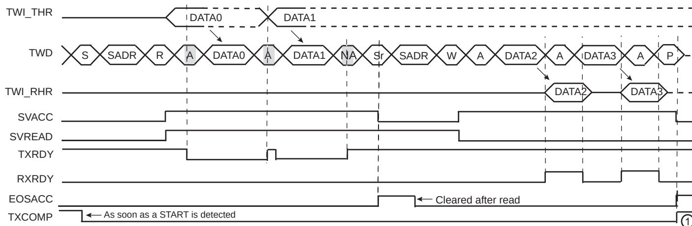
Figure 36-31. Repeated Start + Reversal from Read to Write Mode
