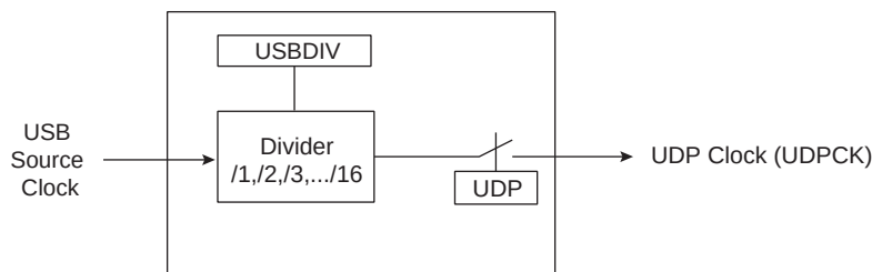
Figure 30-3. USB Clock Controller
