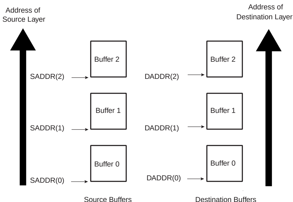
Figure 26-5. Multi-buffer with Linked List Address for Source and Destination
