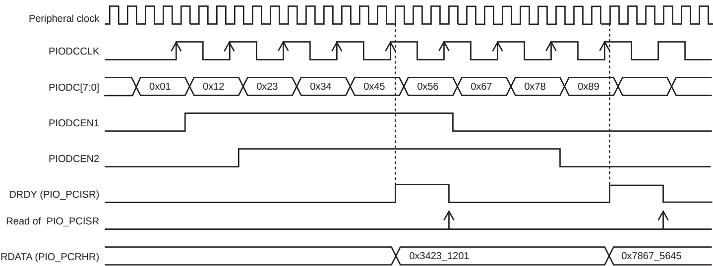
Figure 34-12. Parallel Capture Mode Waveforms (DSIZE = 2, ALWAYS = 1, HALFS = 0)
