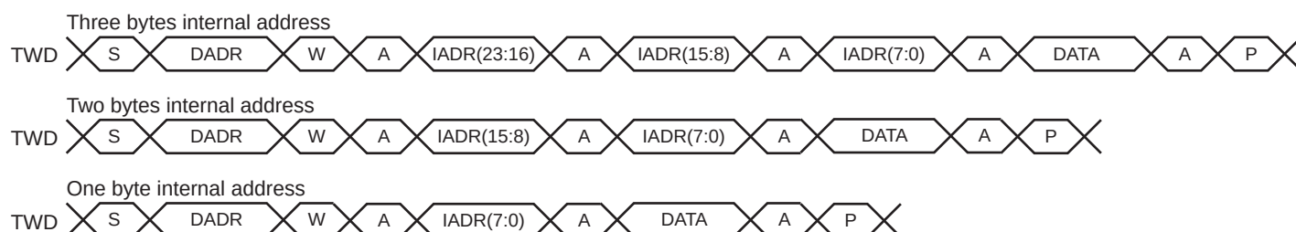
Figure 36-12. Master Write with One, Two or Three Bytes Internal Address and One Data Byte
