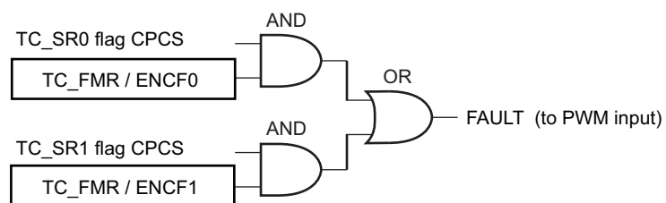
Figure 39-24. Fault Output Generation
