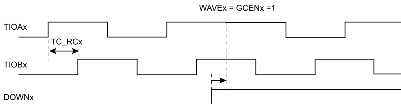
Figure 39-23. 2-bit Gray Up/Down Counter
