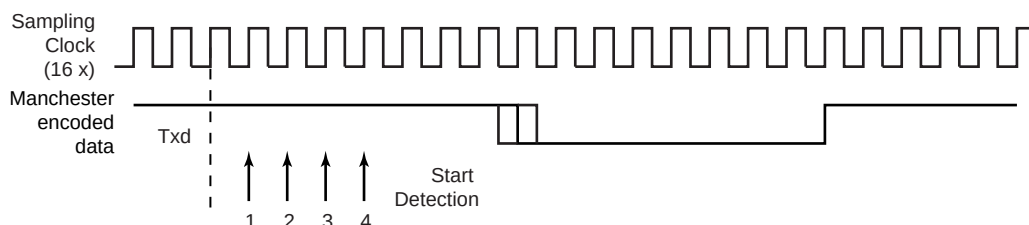
Figure 38-14. Asynchronous Start Bit Detection
