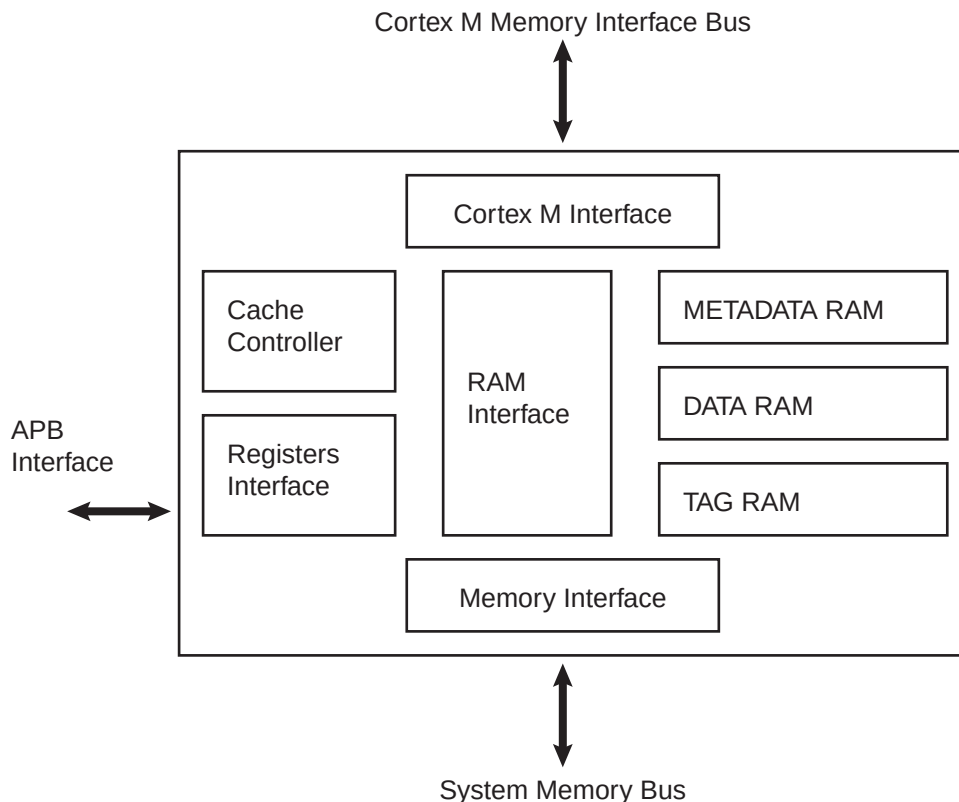
Figure 23-1. Block Diagram
