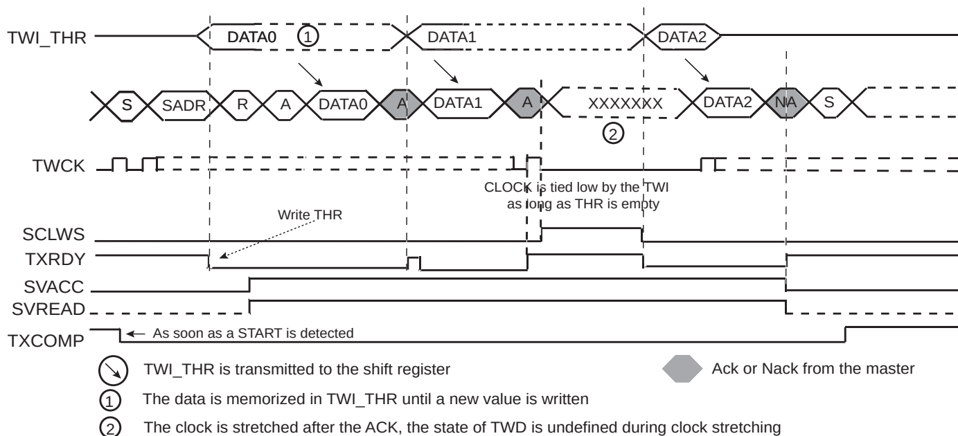
Figure 36-29. Clock Synchronization in Read Mode
