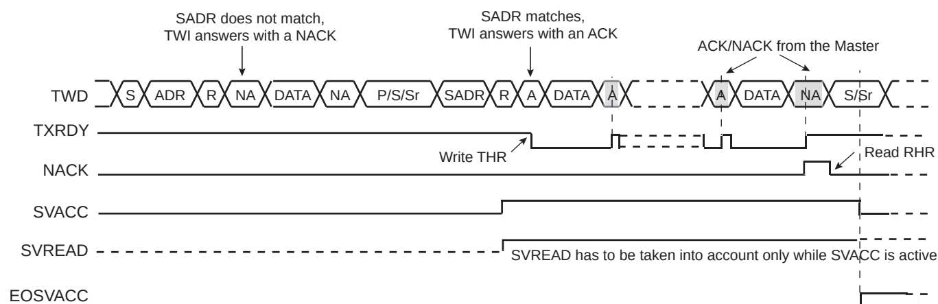
Figure 36-26. Read Access Ordered by a MASTER
