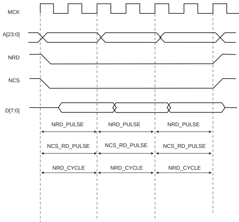
Figure 28-6. No Setup, No Hold on NRD and NCS Read Signals
