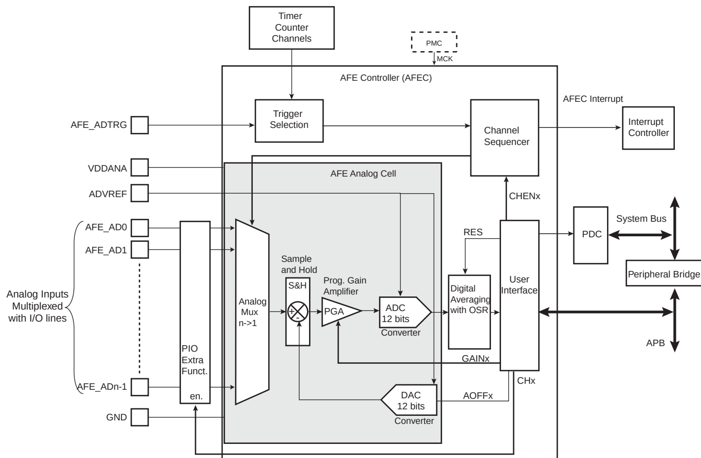
Figure 45-1. Analog-Front-End Converter Block Diagram
