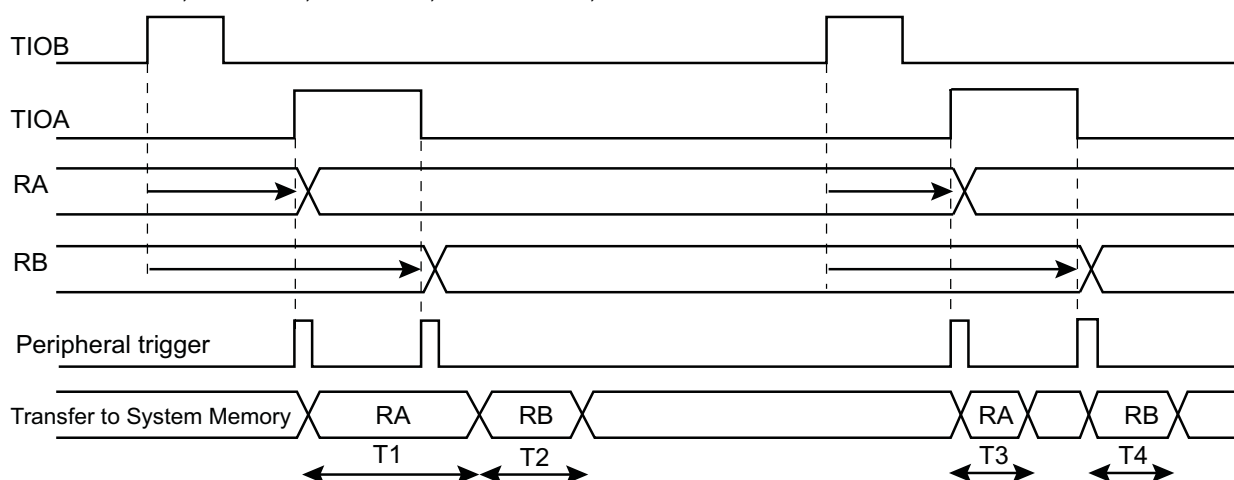
Figure 39-5. Example of Transfer with PDC
