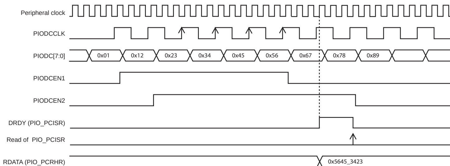
Figure 34-11. Parallel Capture Mode Waveforms (DSIZE = 2, ALWYS = 0, HALFS = 0)
