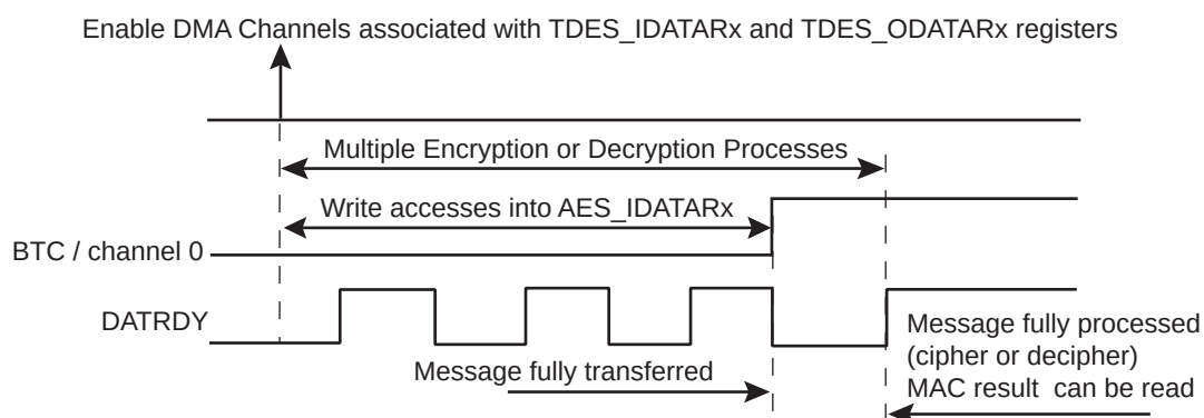
Figure 31-4. DMA transfer with LOD = 1
