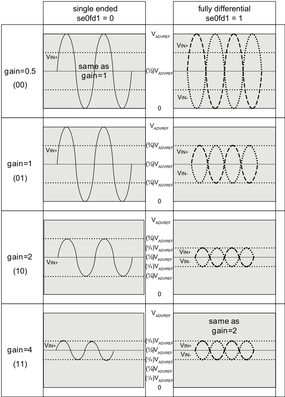
Figure 45-7. Analog Full Scale Ranges in Single Ended/Differential Applications Versus Gain
