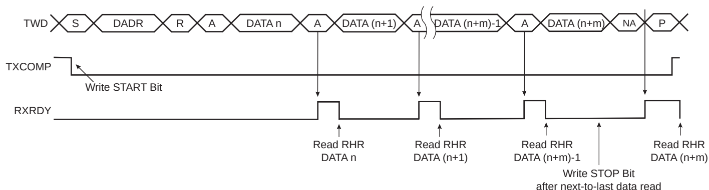
Figure 36-10. Master Read with Multiple Data Bytes
