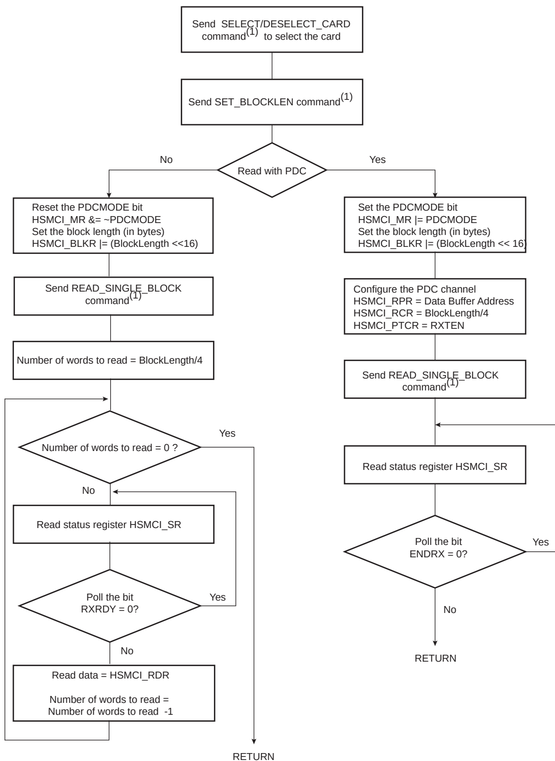
Figure 41-8. Read Functional Flow Diagram
