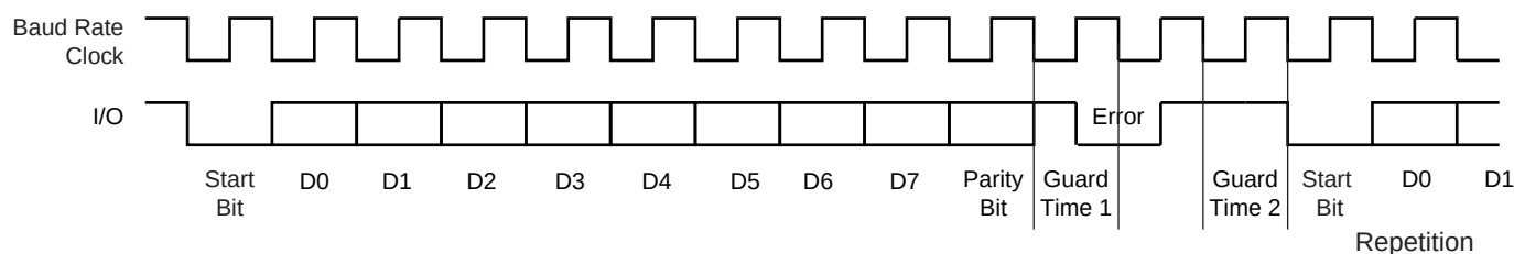
Figure 38-32. T = 0 Protocol with Parity Error
