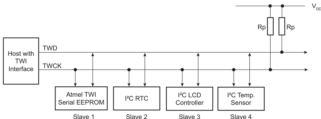
Figure 36-5. Master Mode Typical Application Block Diagram
