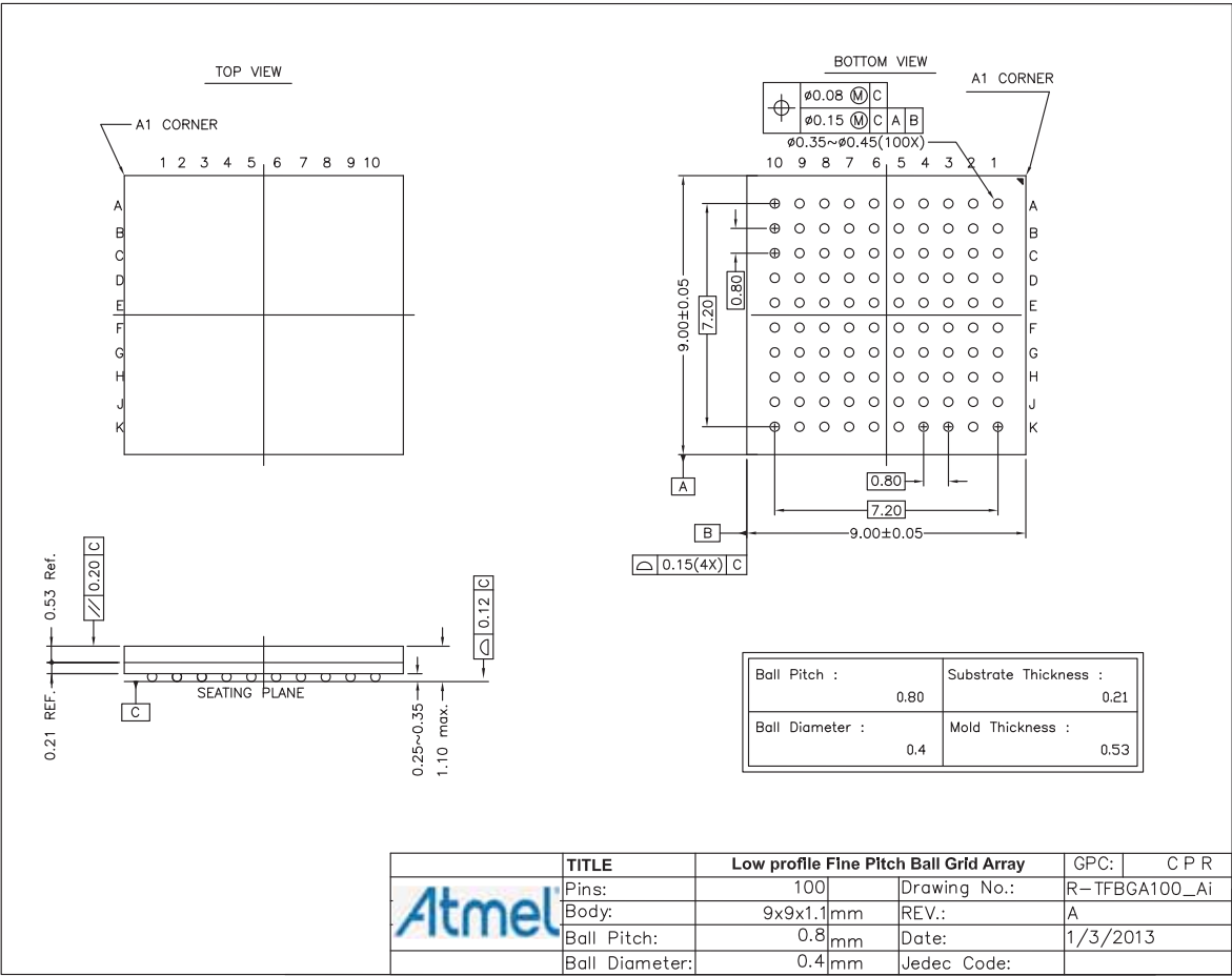
Figure 48-1. 100-ball TFBGA Package Drawing
