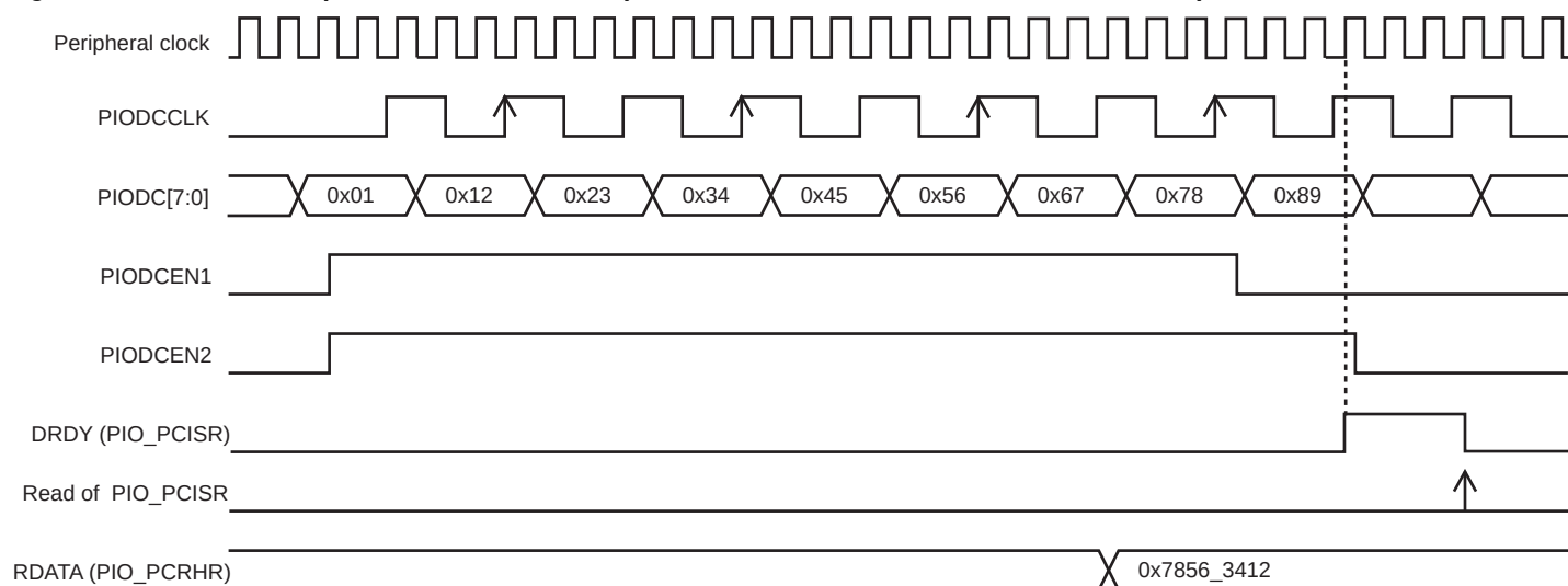
Figure 34-14. Parallel Capture Mode Waveforms (DSIZE = 2, ALWAYS = 0, HALFS = 1, FRSTS = 1)
