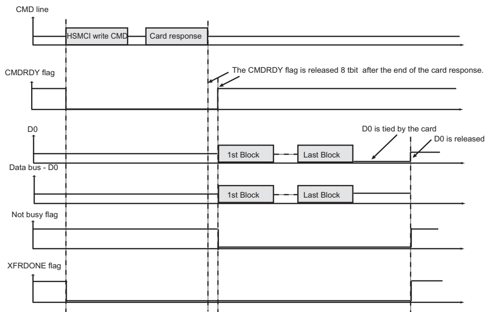
Figure 41-12. XFRDONE During a Write Access
