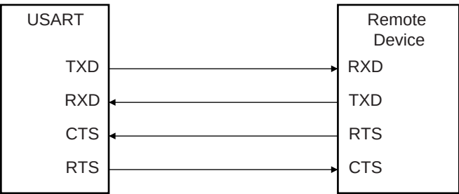
Figure 38-27. Connection with a Remote Device for Hardware Handshaking
