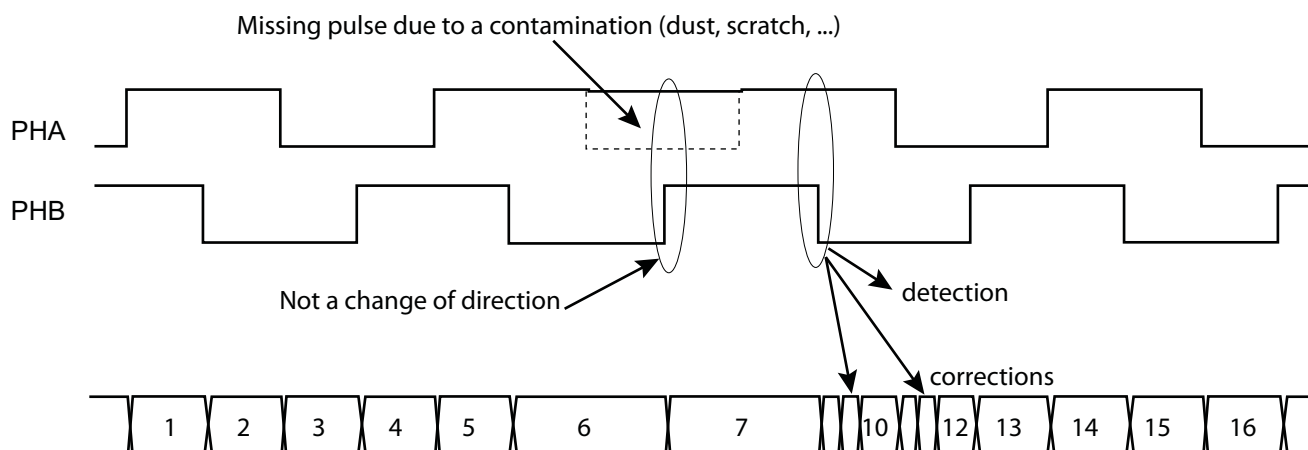
Figure 39-22. Detection and Auto-correction of Missing Pulses
