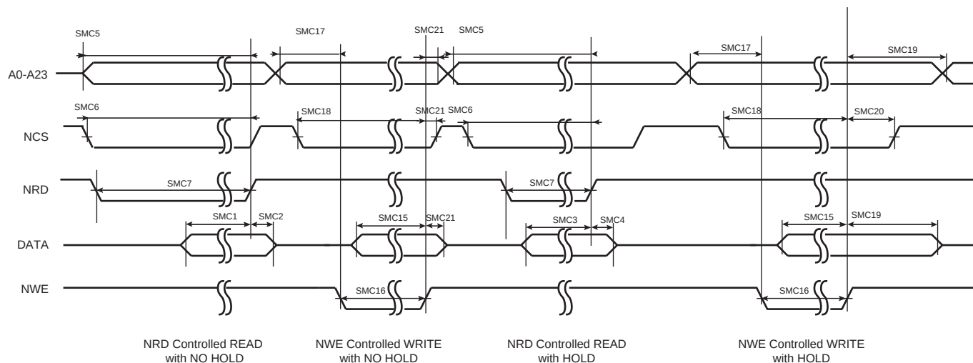
Figure 47-24. SMC Timings - NRD Controlled Read and NWE Controlled Write
