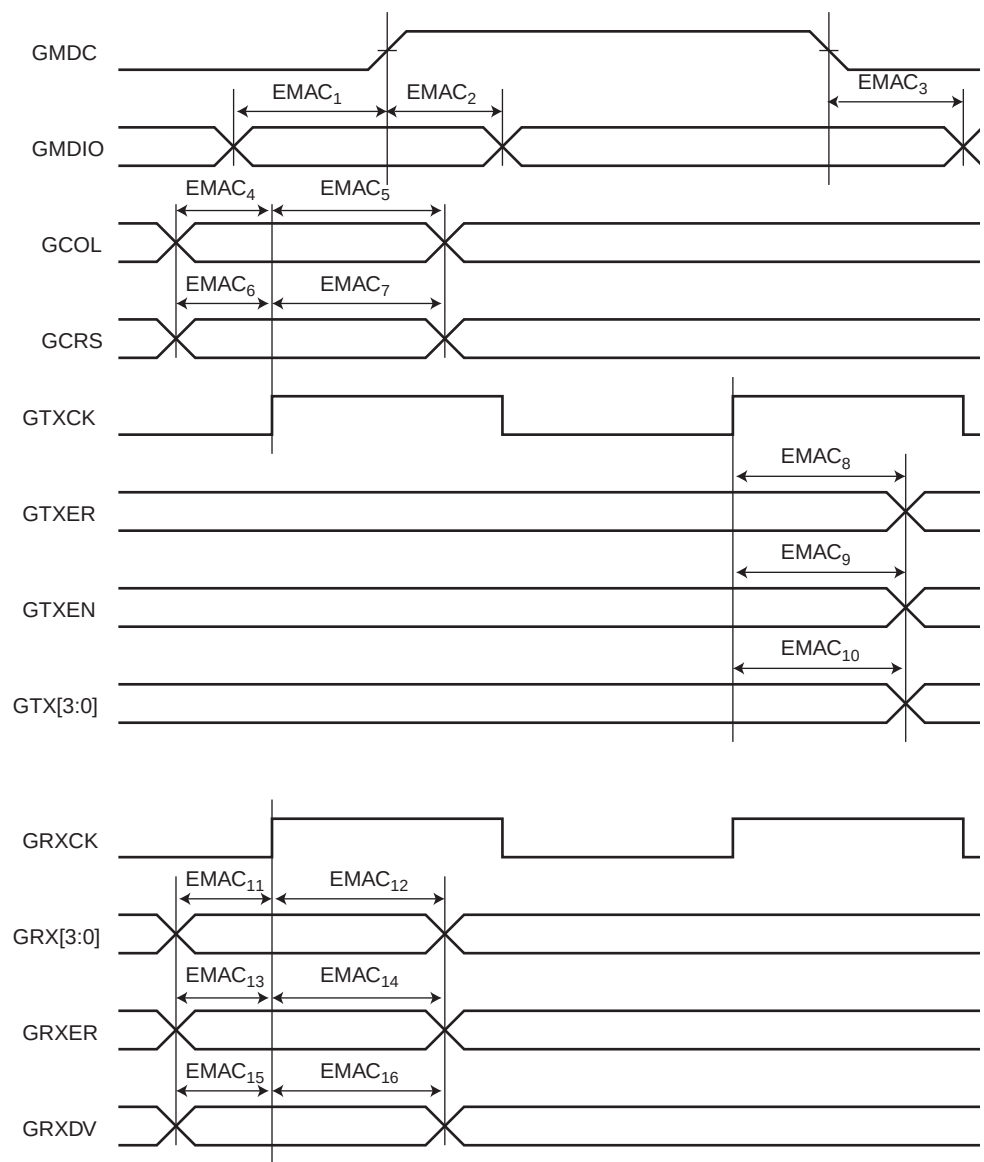
Figure 47-30. EMAC MII Mode Signals
