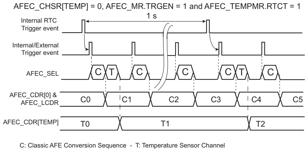
Figure 45-9. Optimized Temperature Conversion combined with classical conversions
