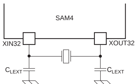
Figure 47-11. 32.768 kHz Crystal Oscillator Schematics
