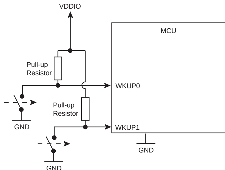
Figure 19-7. Using WKUP Pins Without RTCOUTx Pins
