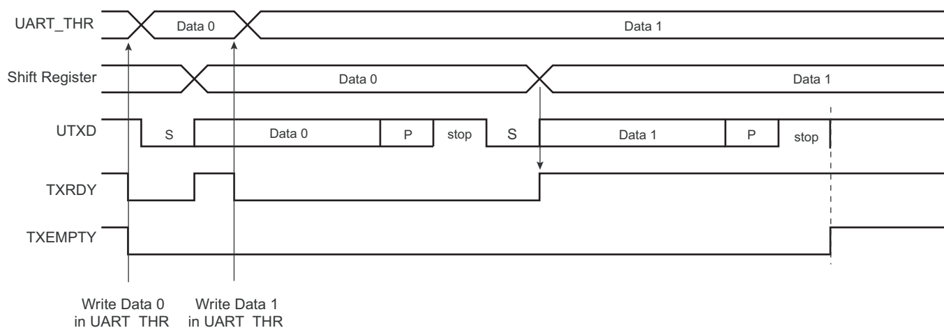
Figure 37-10. Transmitter Control
