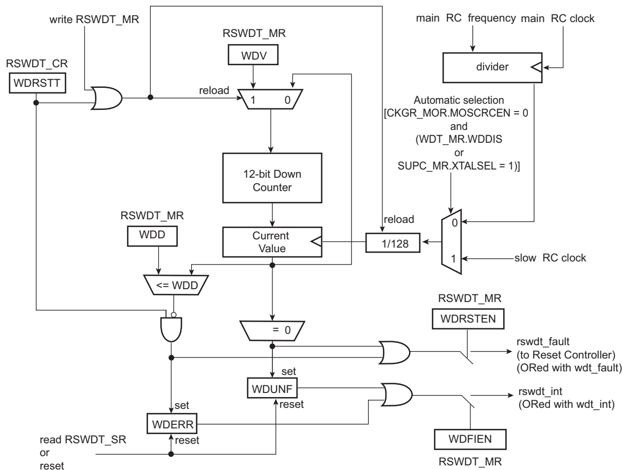
Figure 18-1. Reinforced Safety Watchdog Timer Block Diagram
