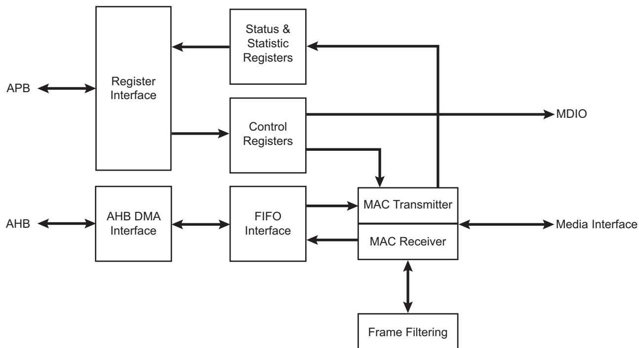
Figure 43-1. Block Diagram
