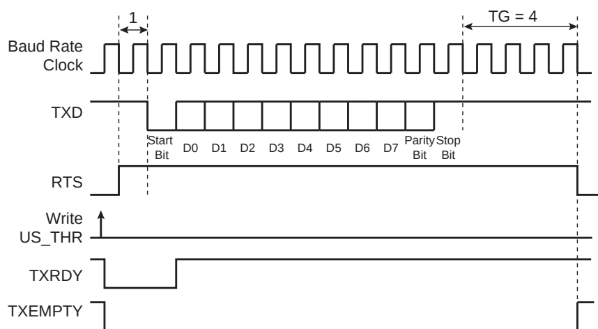
Figure 38-37. Example of RTS Drive with Timeguard
