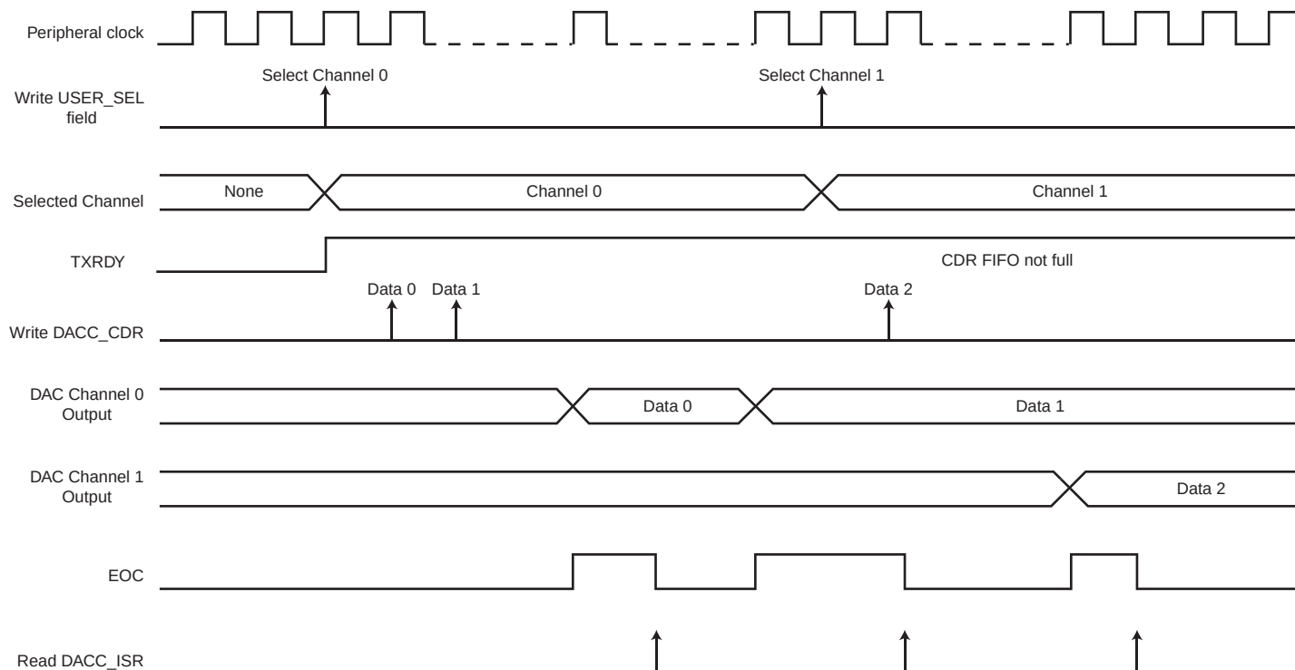
Figure 46-2. Conversion Sequence
