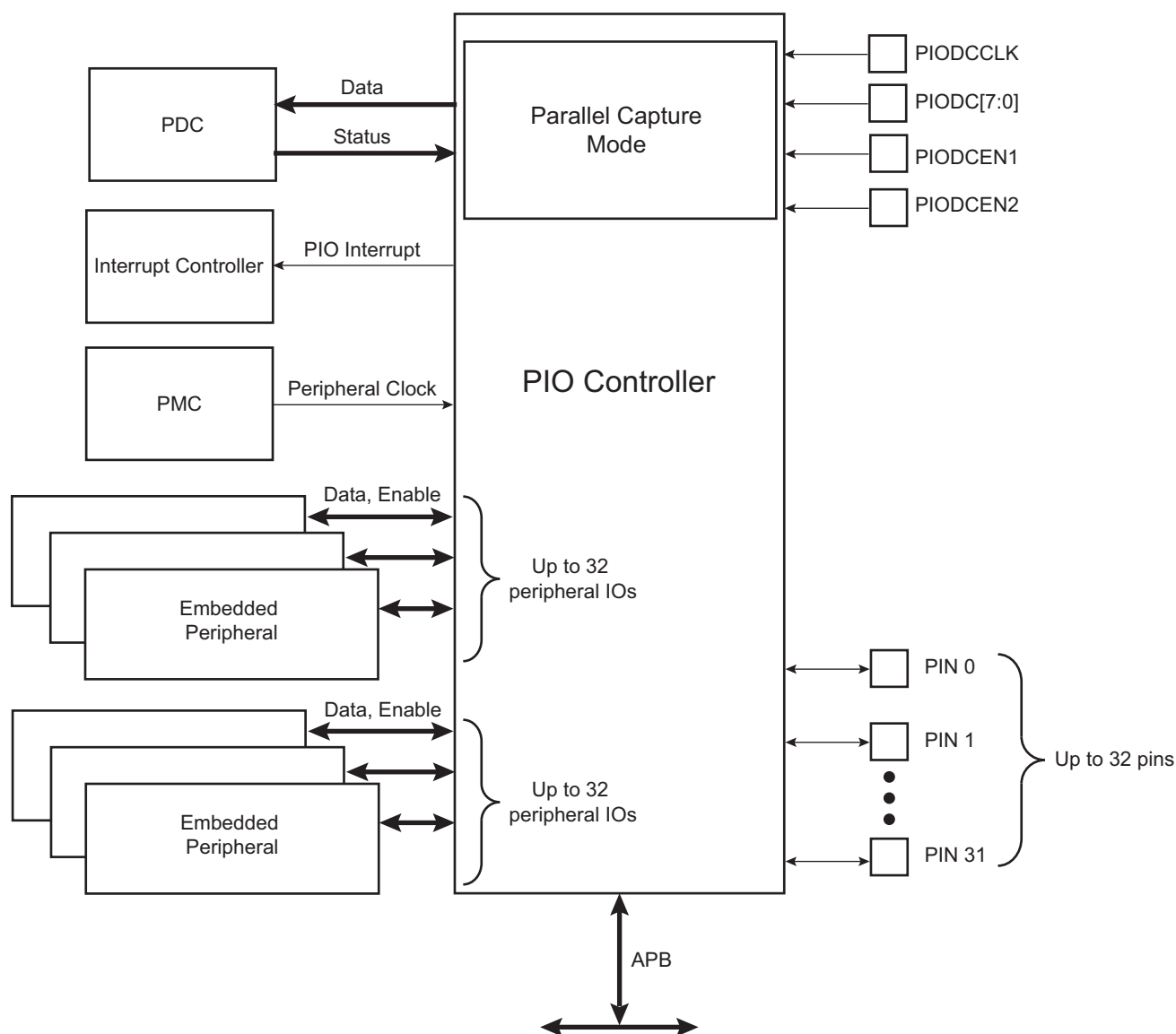
Figure 34-1. Block Diagram
