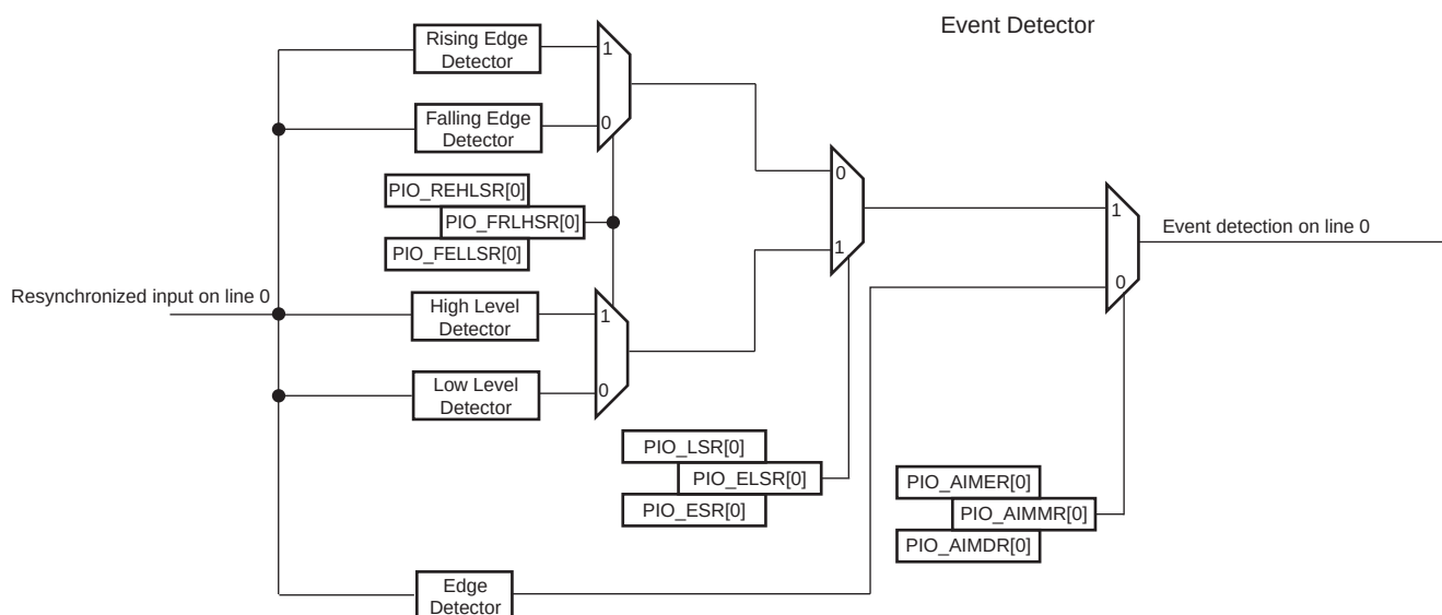
Figure 34-7. Event Detector on Input Lines (Figure Represents Line 0)
