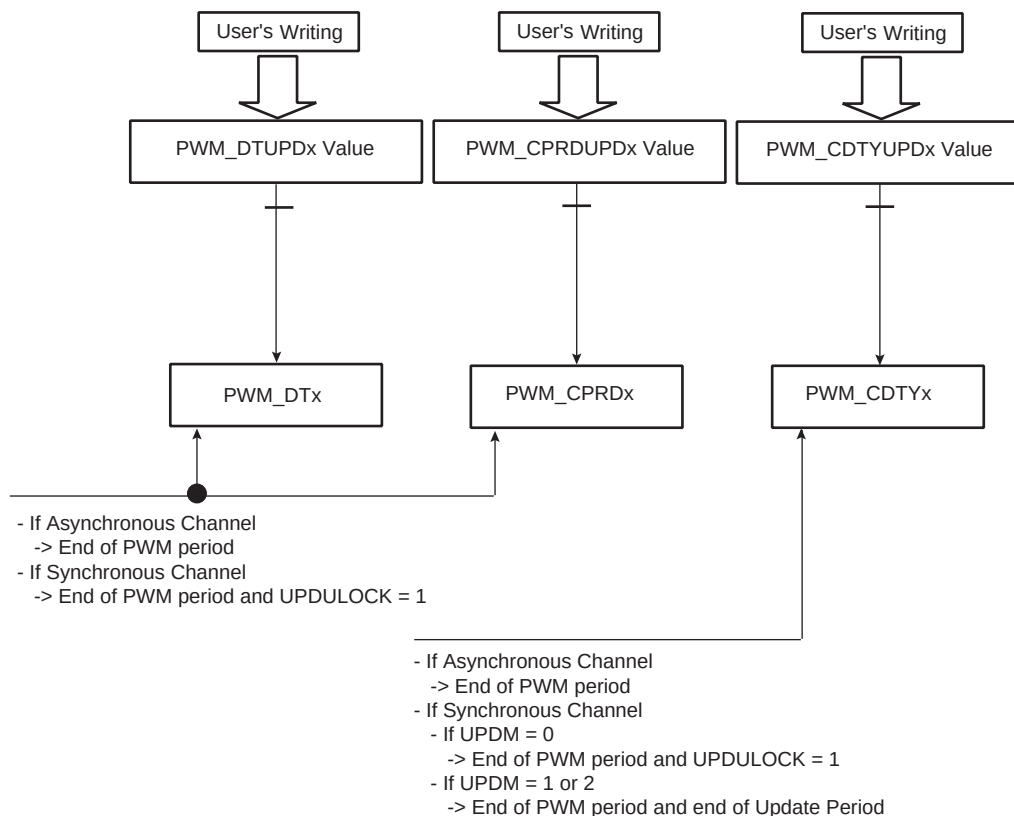
Figure 40-19. Synchronized Period, Duty-Cycle and Dead-Time Update
