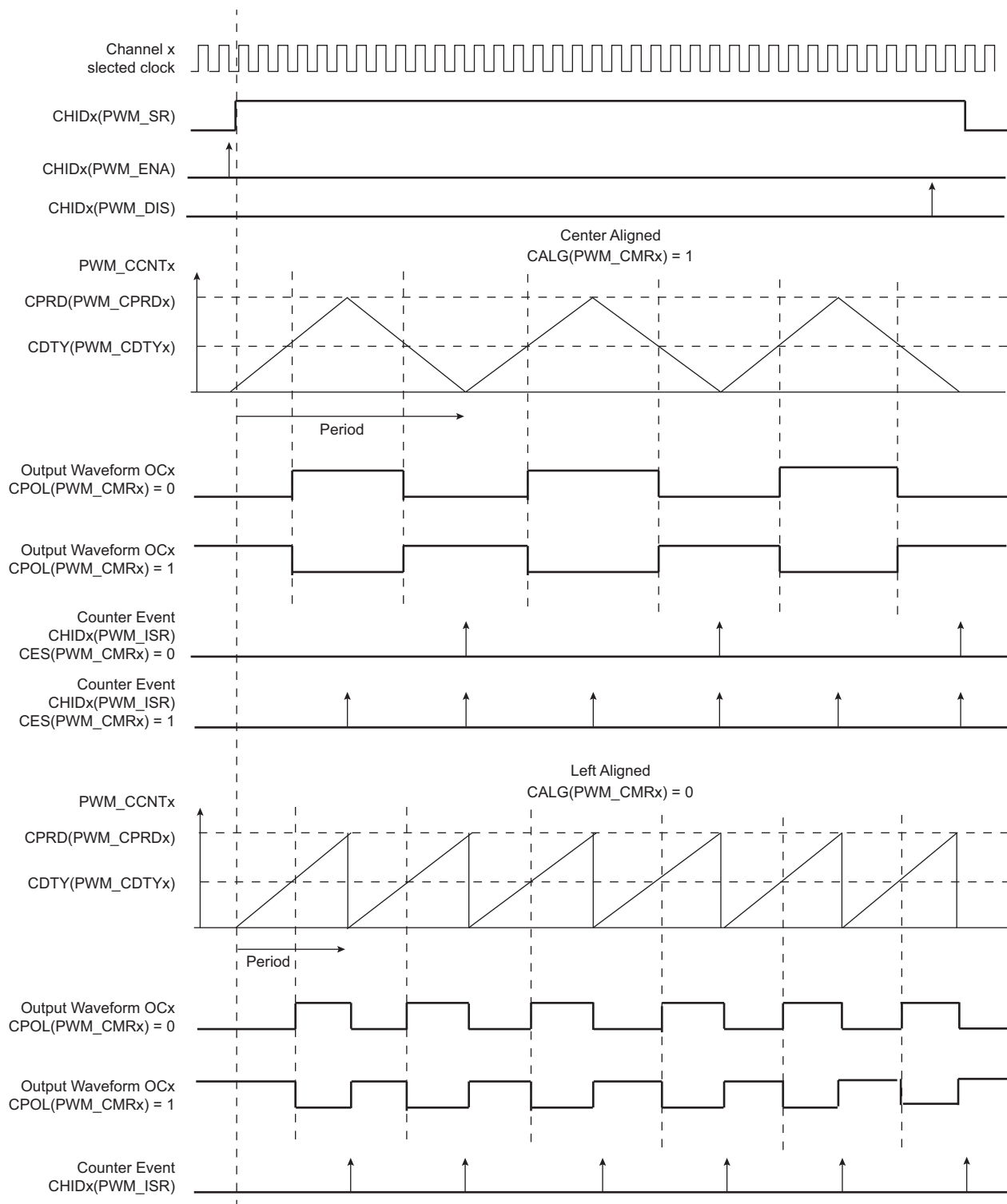
Figure 40-5. Waveform Properties
