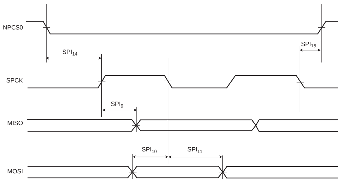
Figure 47-22. SPI Slave Mode with (CPOL = NCPHA = 0) or (CPOL= NCPHA= 1)
