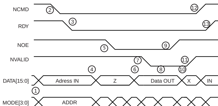
Figure 22-5. Parallel Programming Timing, Read Sequence
