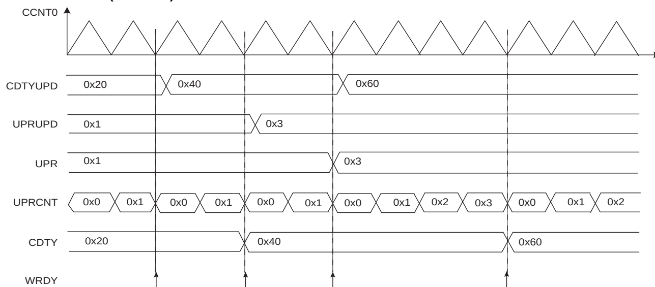
Figure 40-13. Method 2 (UPDM = 1)
