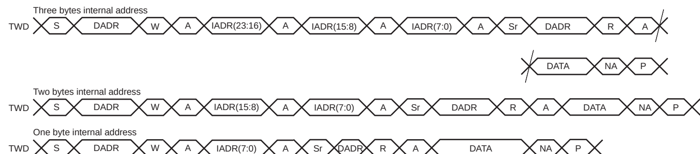
Figure 36-13. Master Read with One, Two or Three Bytes Internal Address and One Data Byte
