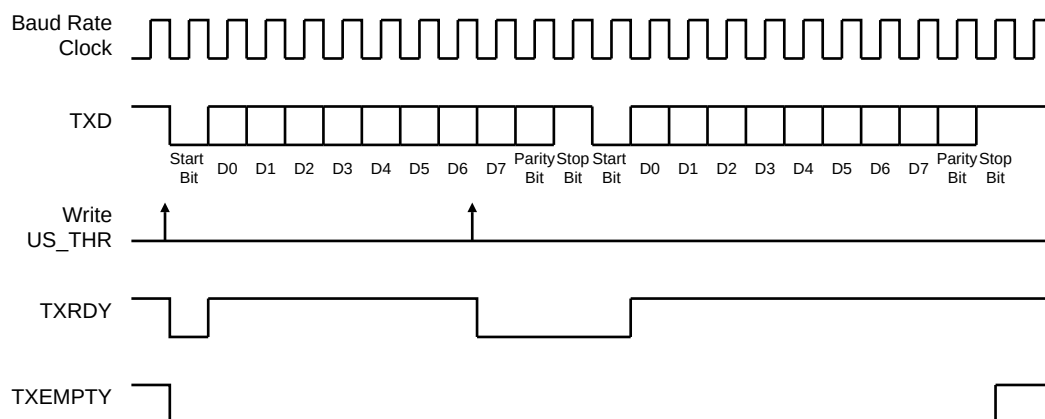
Figure 38-7. Transmitter Status
