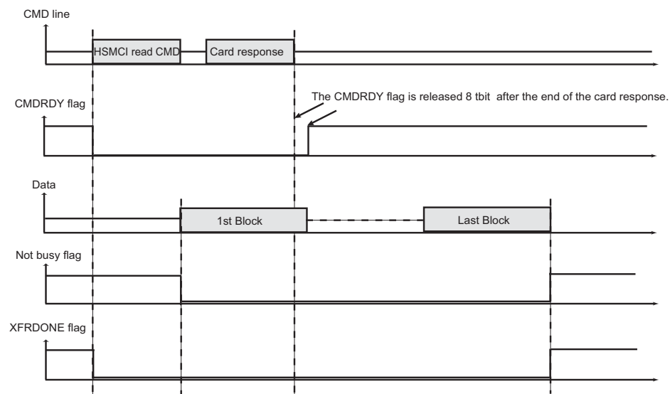
Figure 41-11. XFRDONE During a Read Access
