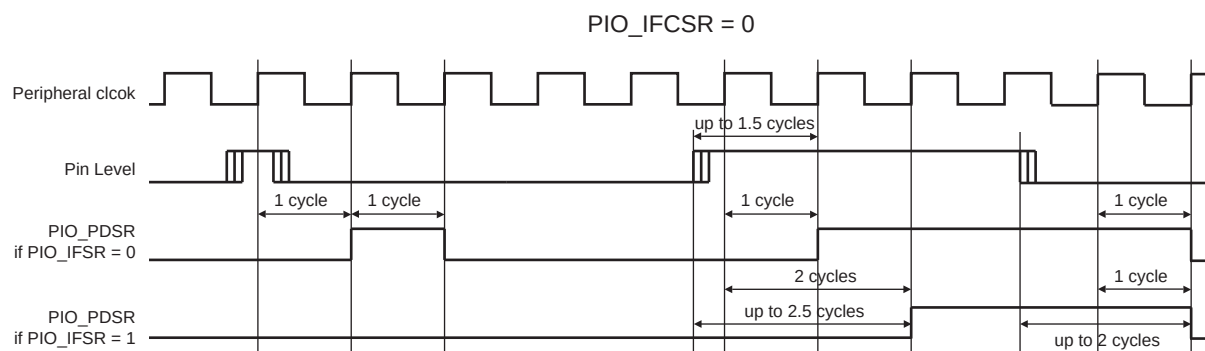
Figure 34-5. Input Glitch Filter Timing
