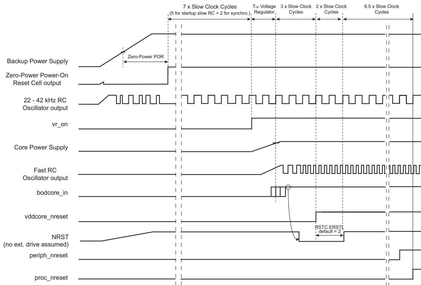
Figure 19-3. Raising the VDDIO Power Supply
