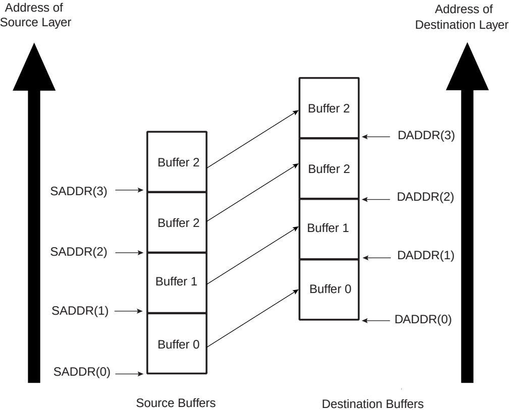
Figure 26-6. Multi-buffer with Linked Address for Source and Destination Buffers are Contiguous
