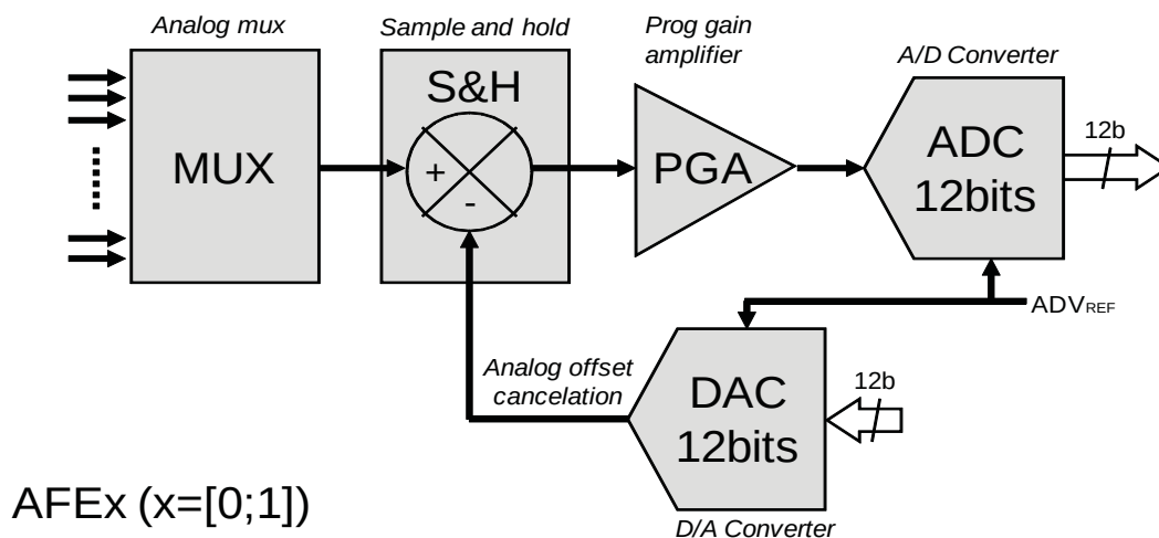
Figure 47-14. 12-bit AFE (Analog Front End) Diagram
