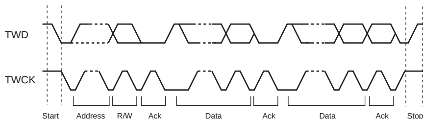
Figure 36-4. Transfer Format
