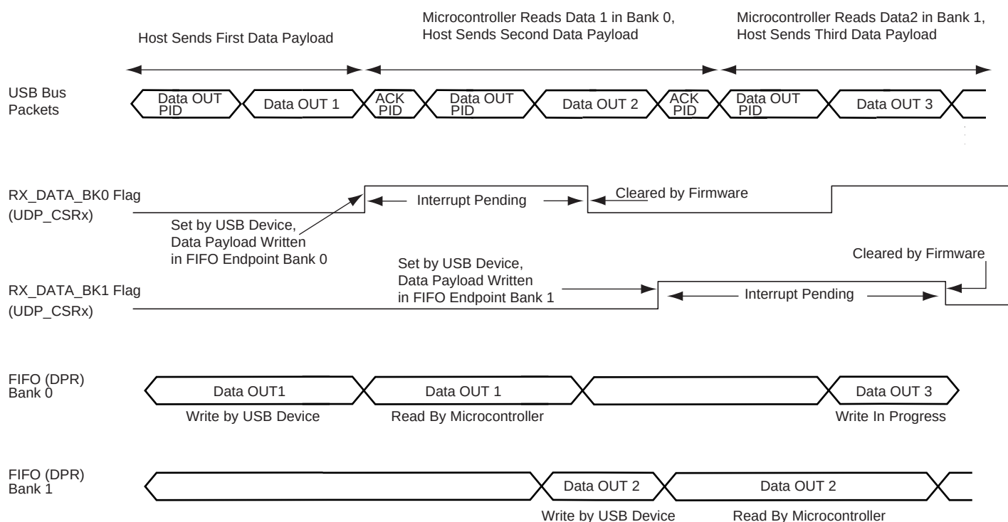
Figure 42-11. Data OUT Transfer for Ping-pong Endpoint
