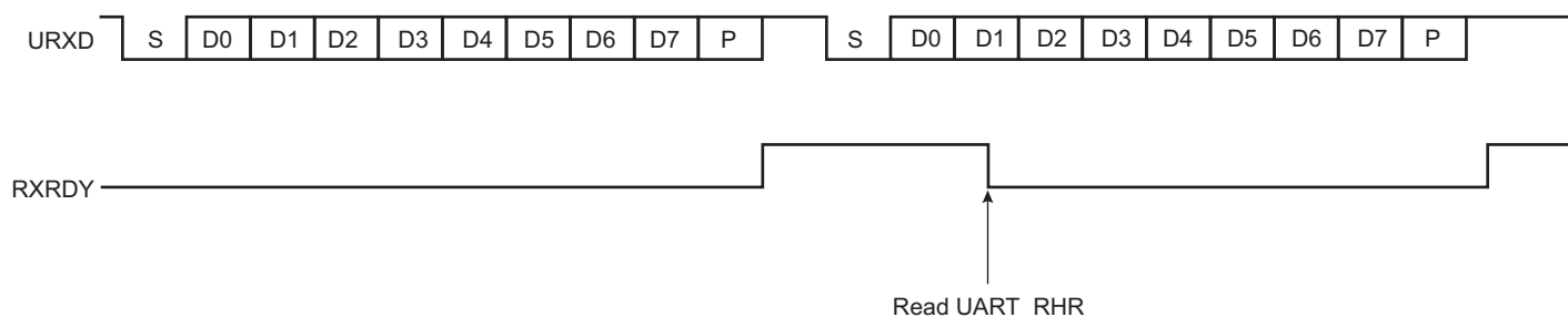
Figure 37-5. Receiver Ready
