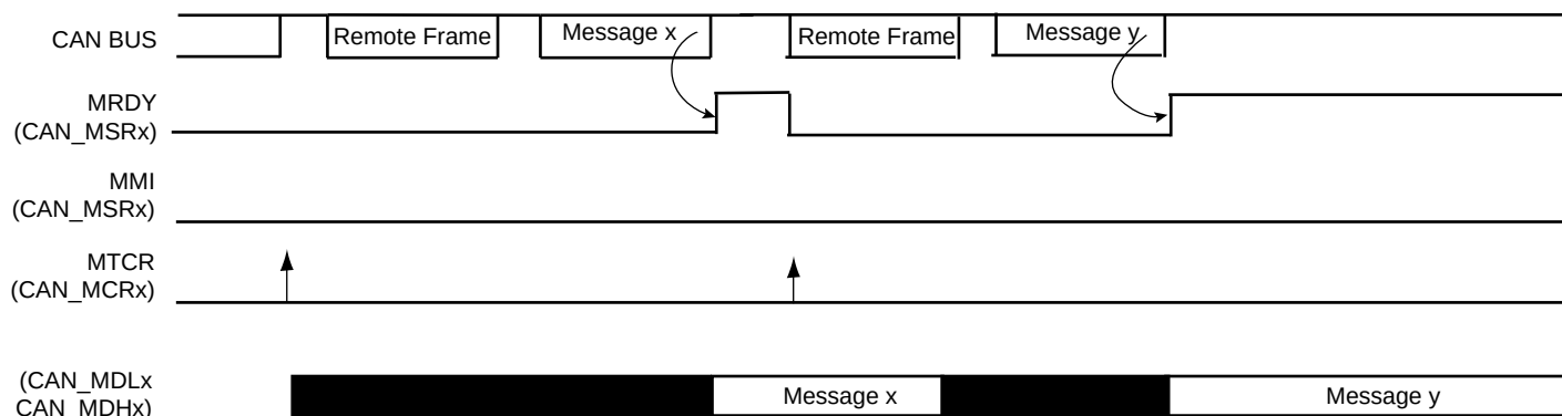
Figure 33-18. Consumer Handling
