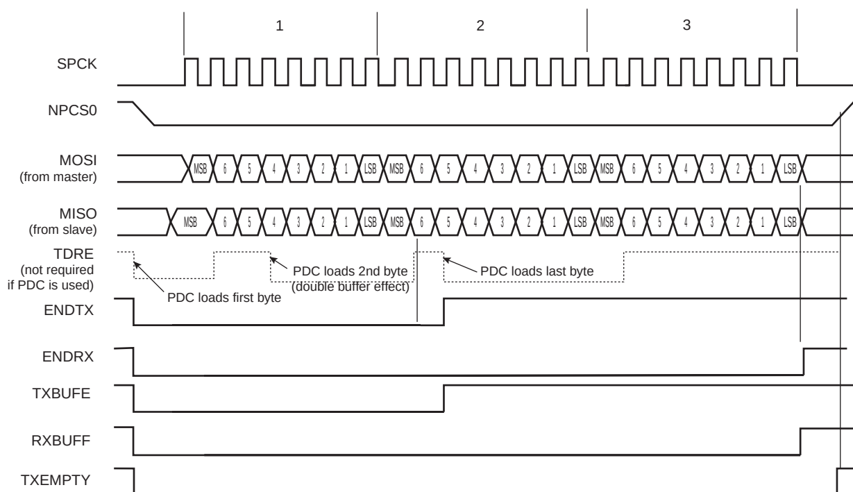
Figure 35-8. PDC Status Register Flags Behavior
