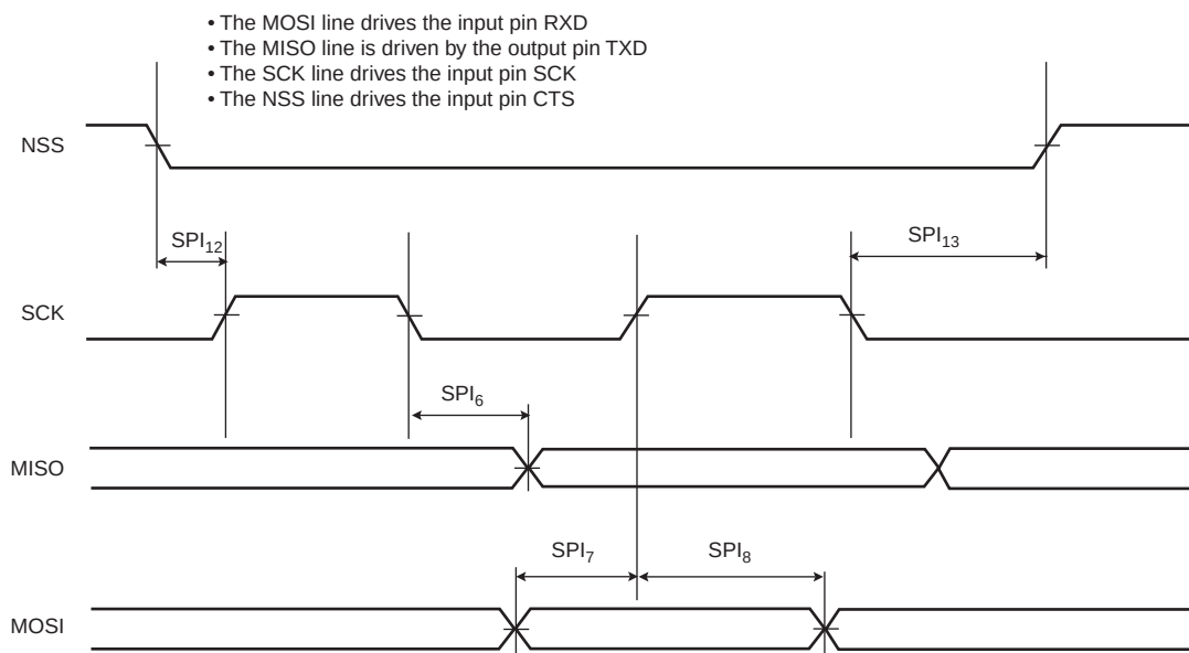
Figure 47-26. USART SPI Slave Mode (Mode 1 or 2)
