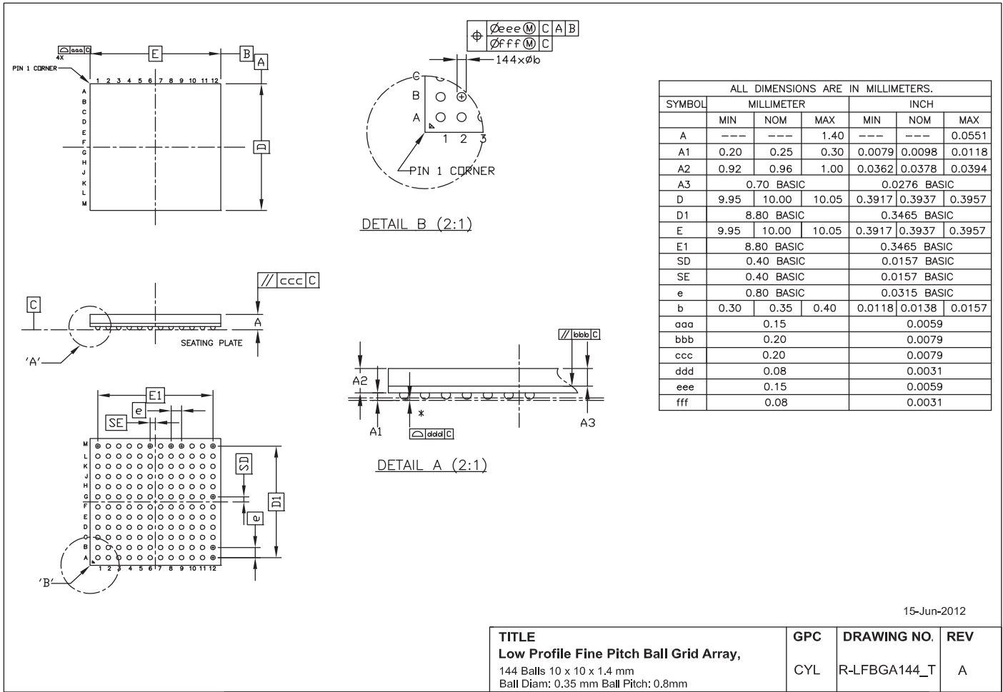
Figure 48-2. 144-ball LFBGA Package Drawing
