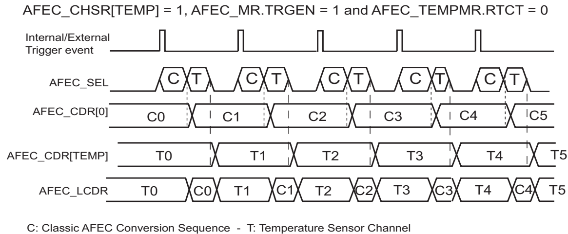
Figure 45-8. Non-Optimized Temperature Conversion
