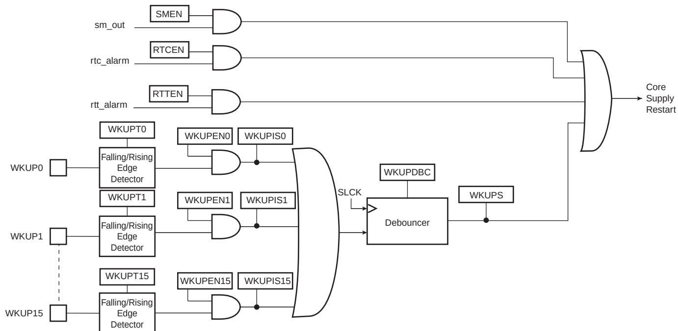
Figure 5-3. Wake-up Source
