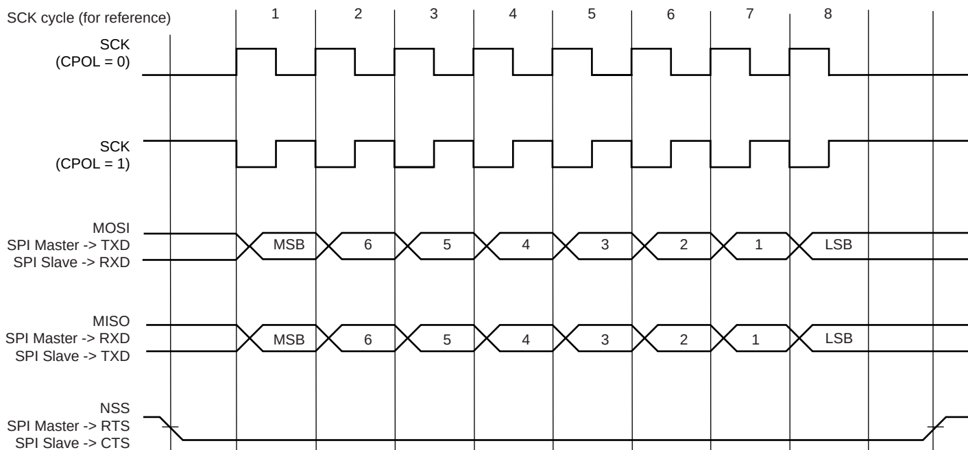
Figure 38-39. SPI Transfer Format (CPHA = 0, 8 bits per transfer)
