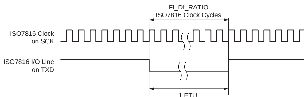
Figure 38-5. Elementary Time Unit (ETU)
