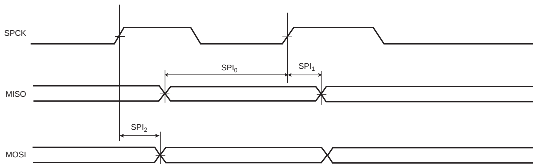
Figure 47-19. SPI Master Mode with (CPOL= NCPHA = 0) or (CPOL= NCPHA= 1)
