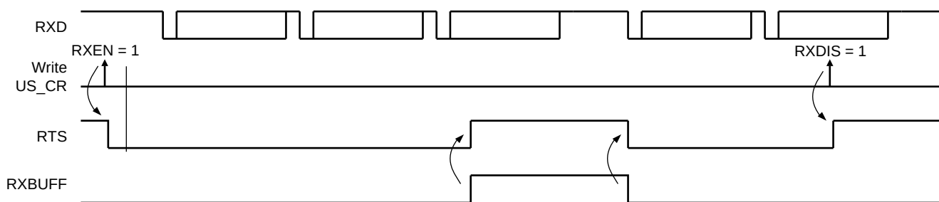
Figure 38-28. Receiver Behavior when Operating with Hardware Handshaking
