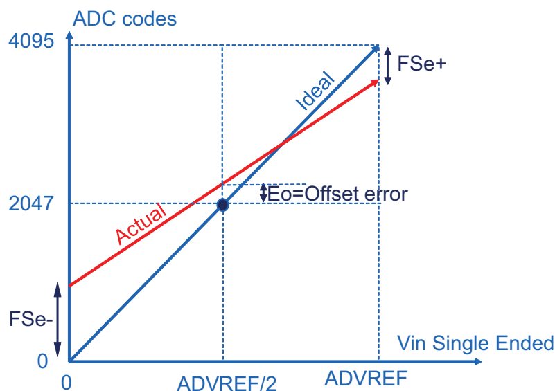
Figure 47-16. Gain and Offset Errors in Single-ended Mode
