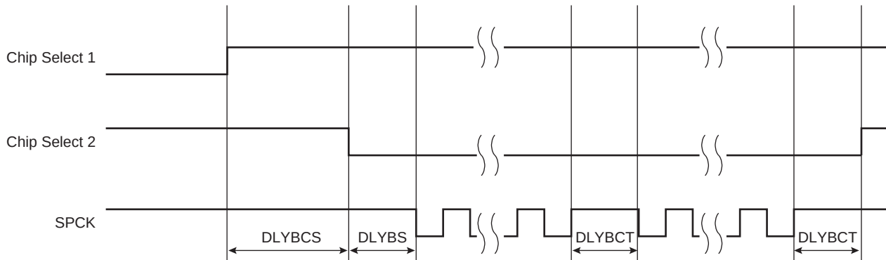
Figure 35-9. Programmable Delays
