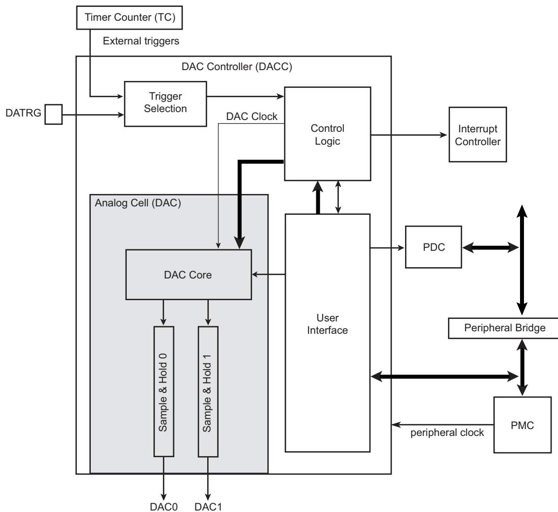
Figure 46-1. DACC Block Diagram
