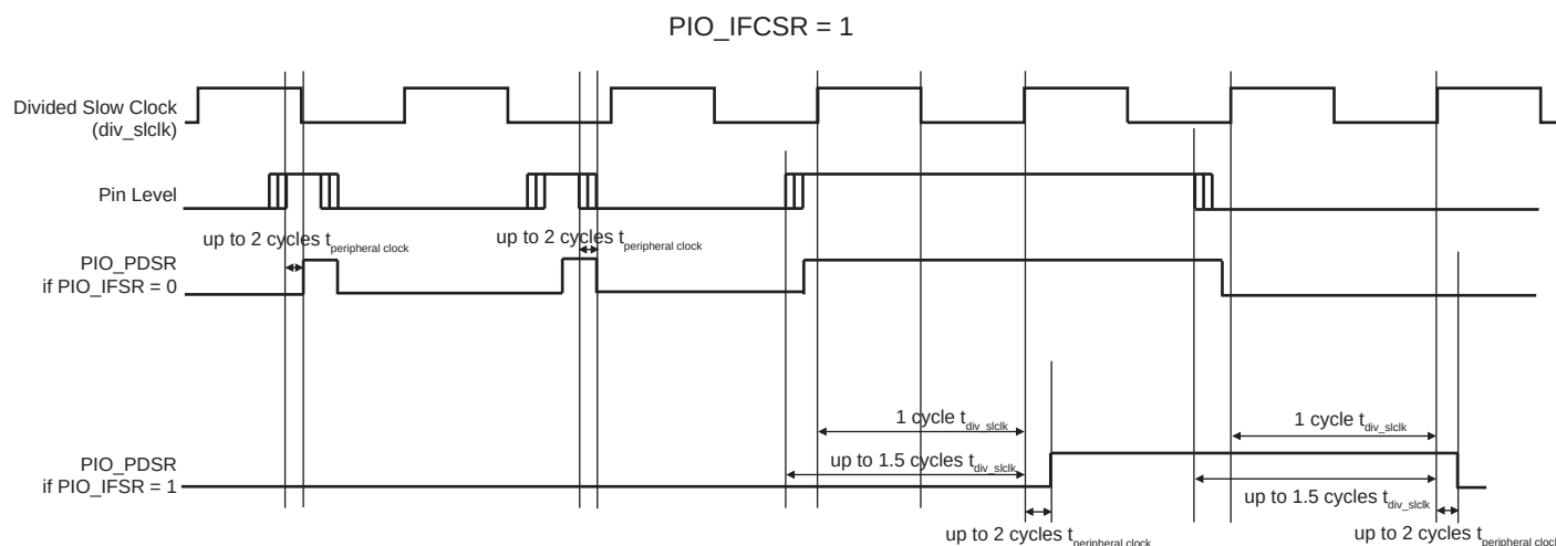
Figure 34-6. Input Debouncing Filter Timing
