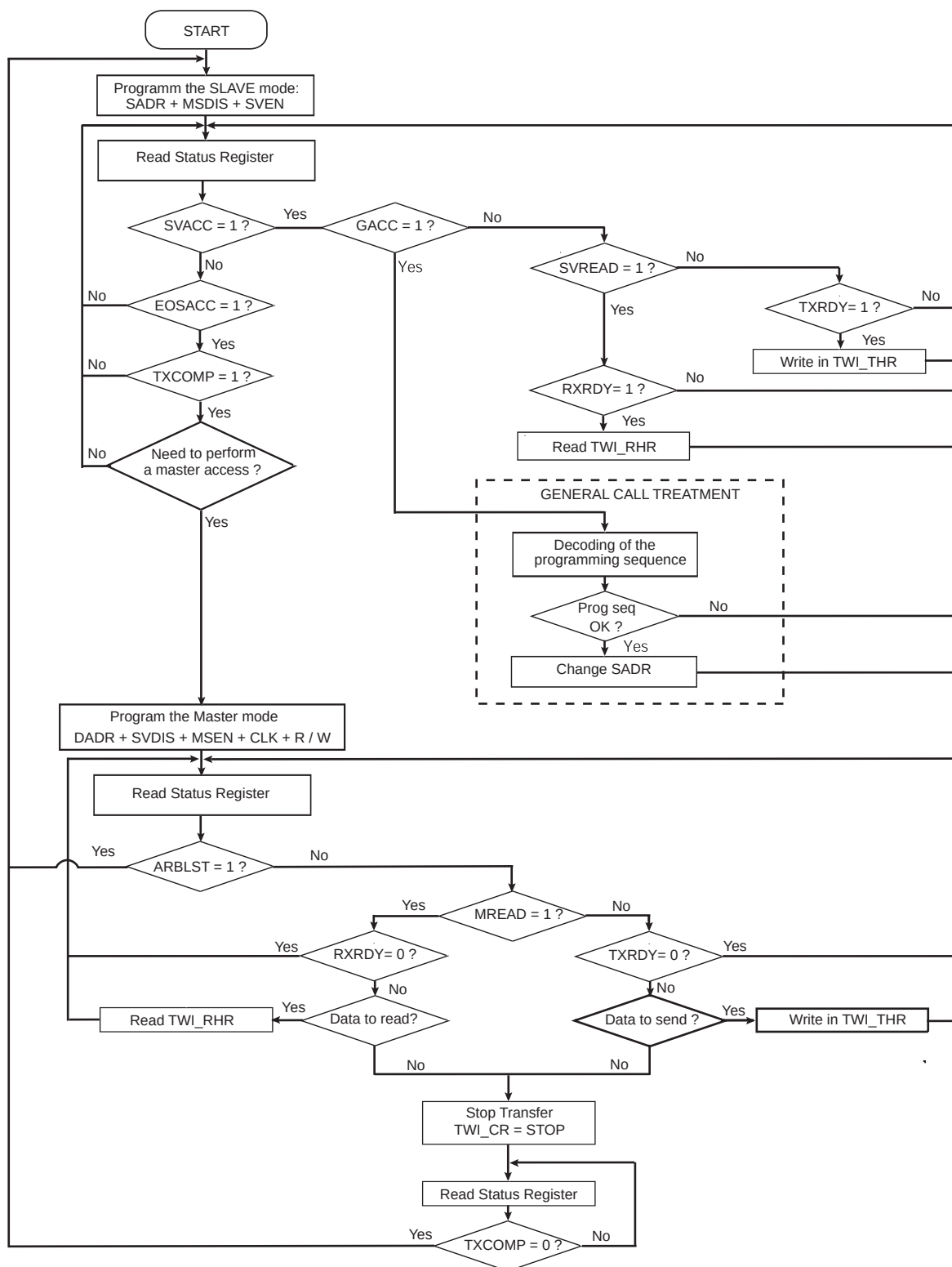
Figure 36-24. Multi-master Flowchart
