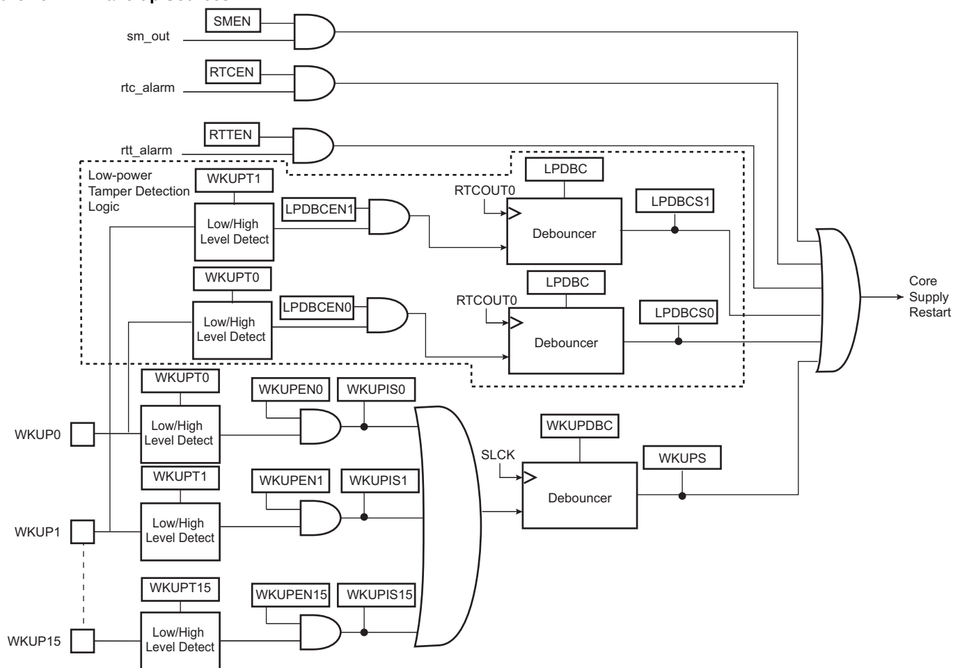
Figure 19-4. Wake-up Sources
