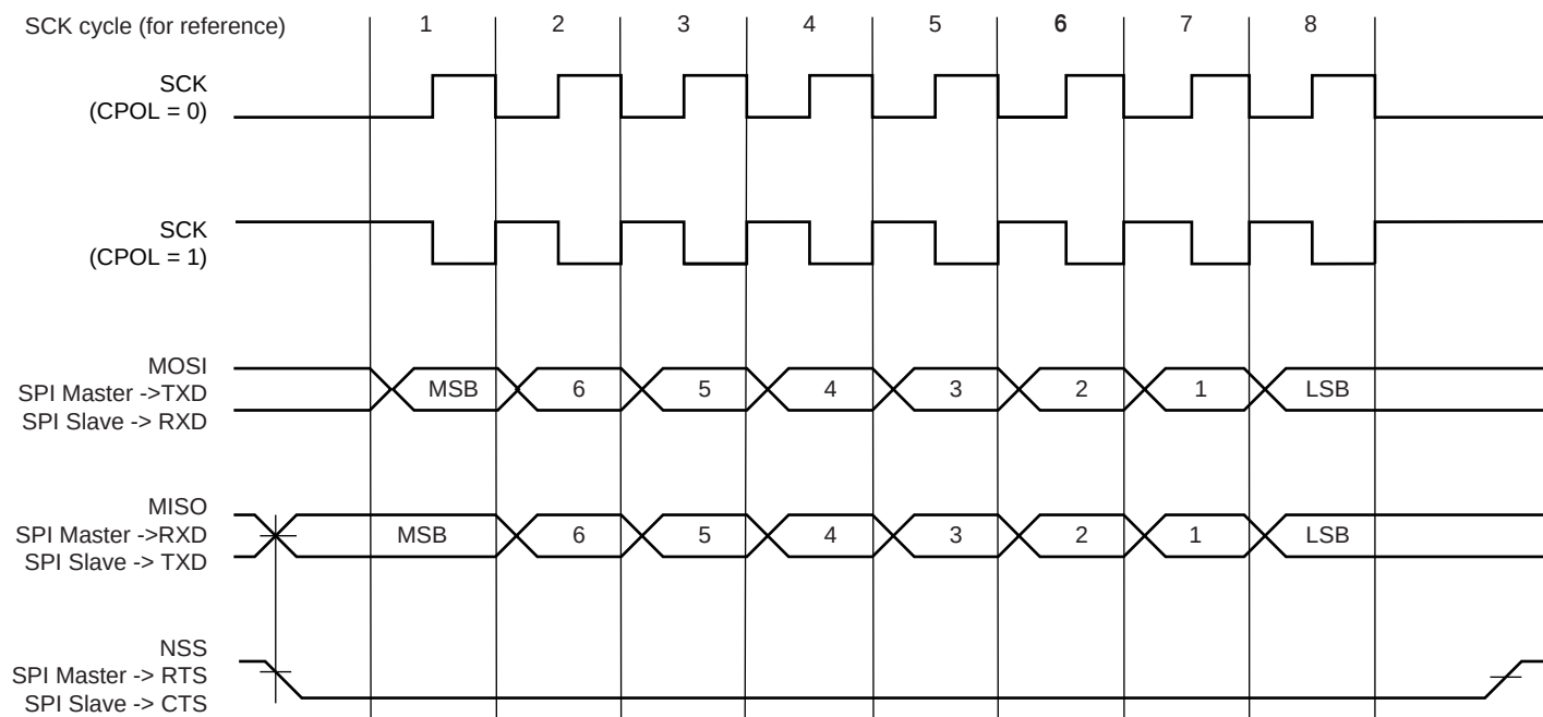
Figure 38-38. SPI Transfer Format (CPHA = 1, 8 bits per transfer)
