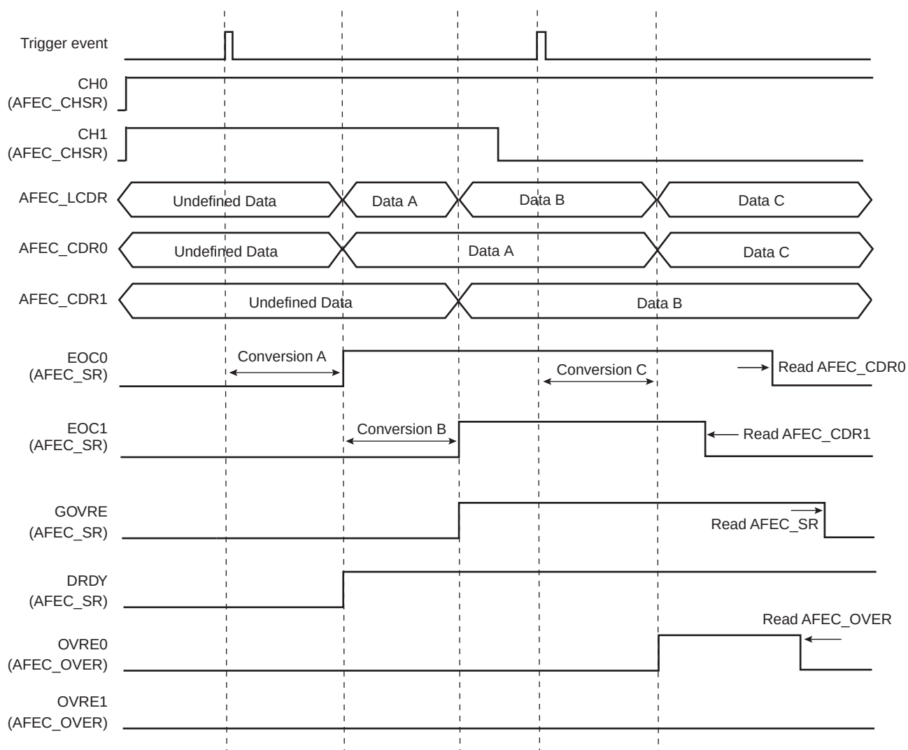
Figure 45-5. GOVRE and OVREx Flag Behavior
