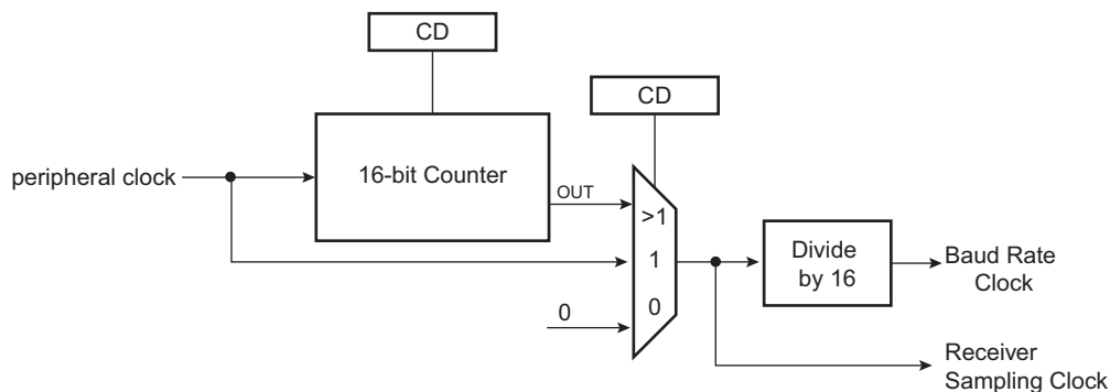
Figure 37-2. Baud Rate Generator
