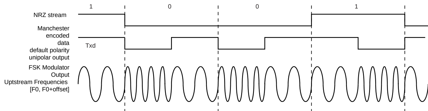
Figure 38-19. FSK Modulator Output
