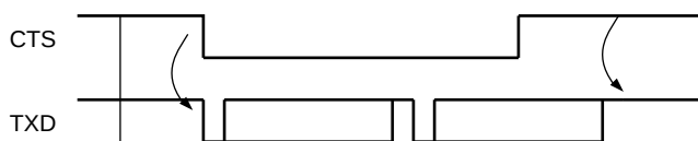
Figure 38-29. Transmitter Behavior when Operating with Hardware Handshaking
