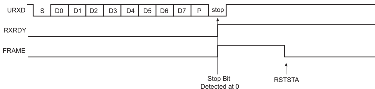
Figure 37-8. Receiver Framing Error
