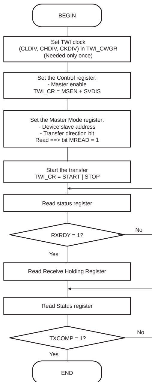
Figure 36-19. TWI Read Operation with Single Data Byte without Internal Address
