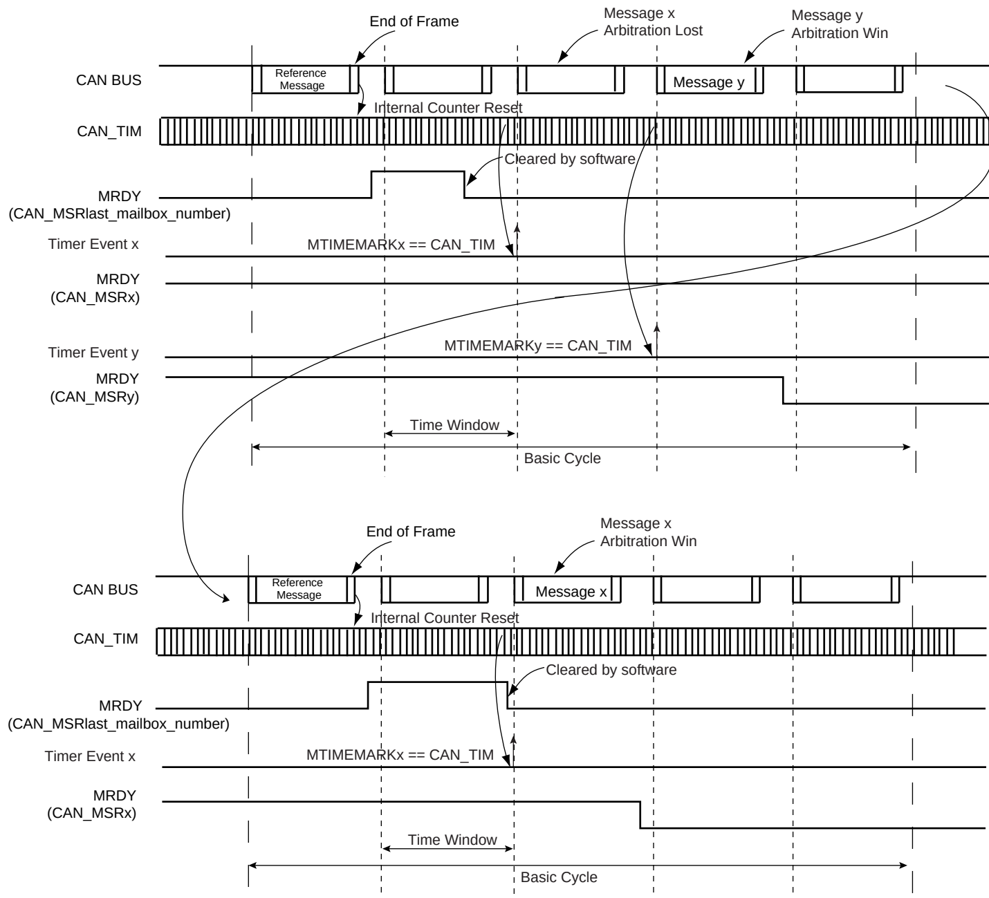
Figure 33-21. Time Triggered Operations
