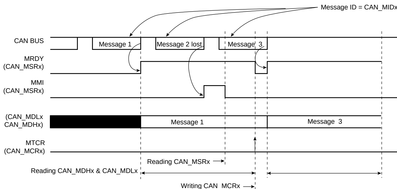
Figure 33-11. Receive Mailbox
