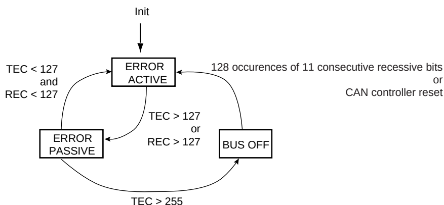
Figure 33-7. Line Error Mode
