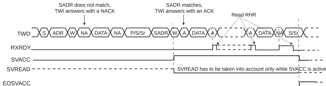
Figure 36-27. Write Access Ordered by a Master
