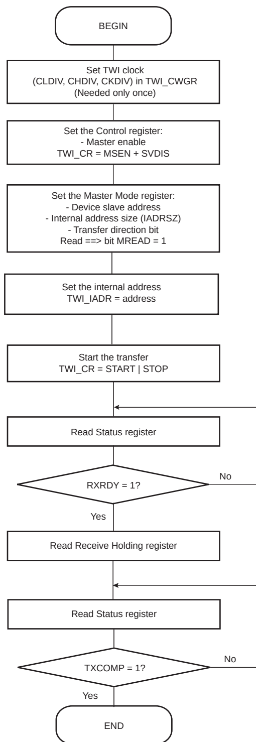
Figure 36-20. TWI Read Operation with Single Data Byte and Internal Address
