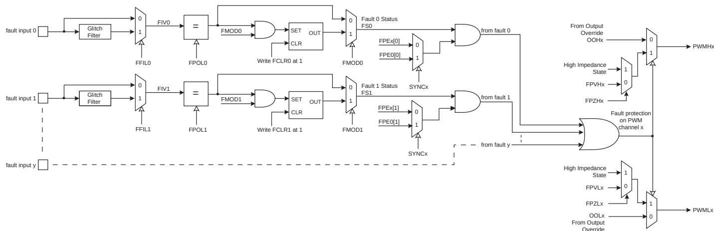
Figure 40-9. Fault Protection
