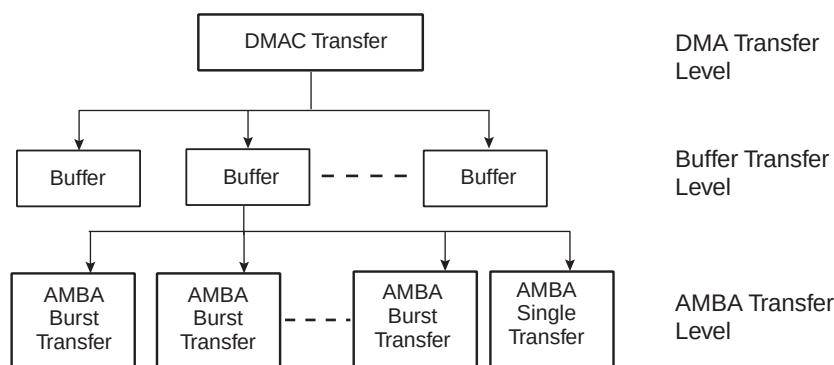
Figure 26-3. DMAC Transfer Hierarchy for Memory
