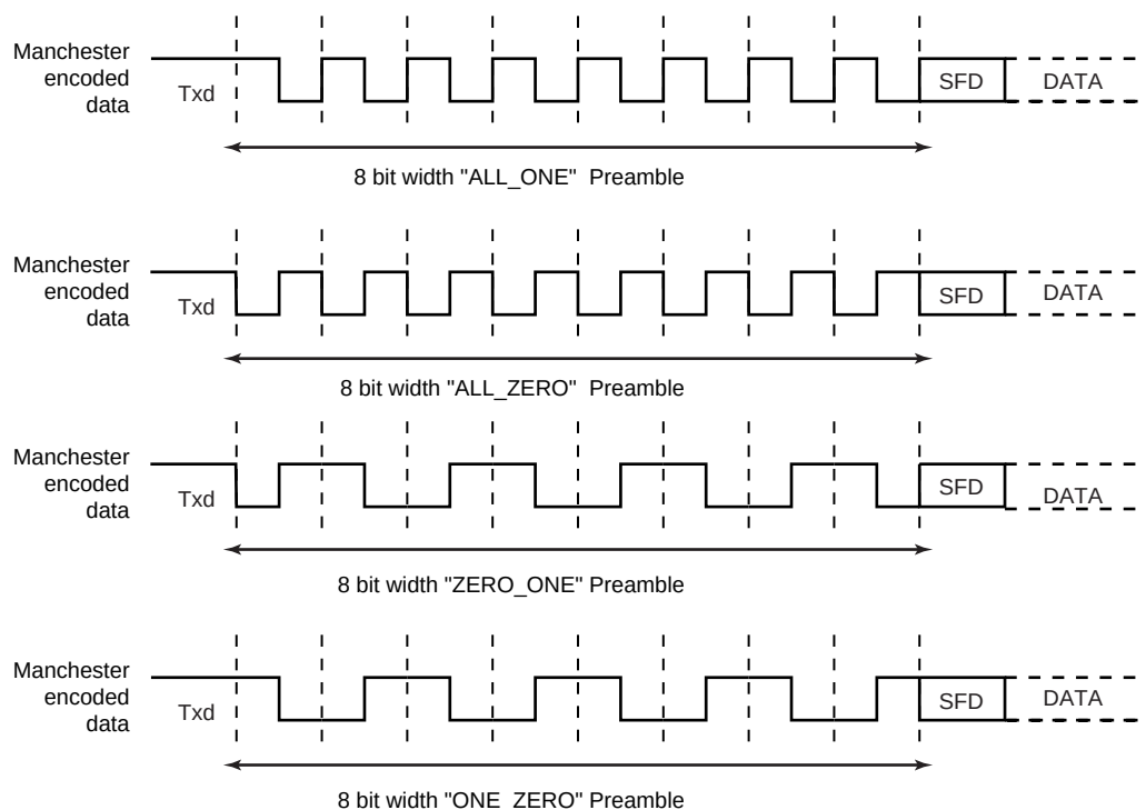
Figure 38-9. Preamble Patterns, Default Polarity Assumed
