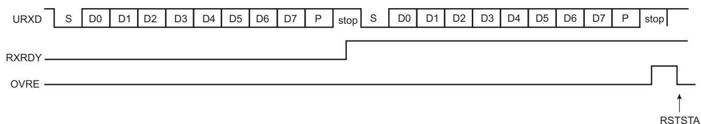
Figure 37-6. Receiver Overrun
