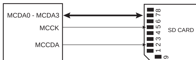
Figure 41-6. SD Card Bus Connections with One Slot
