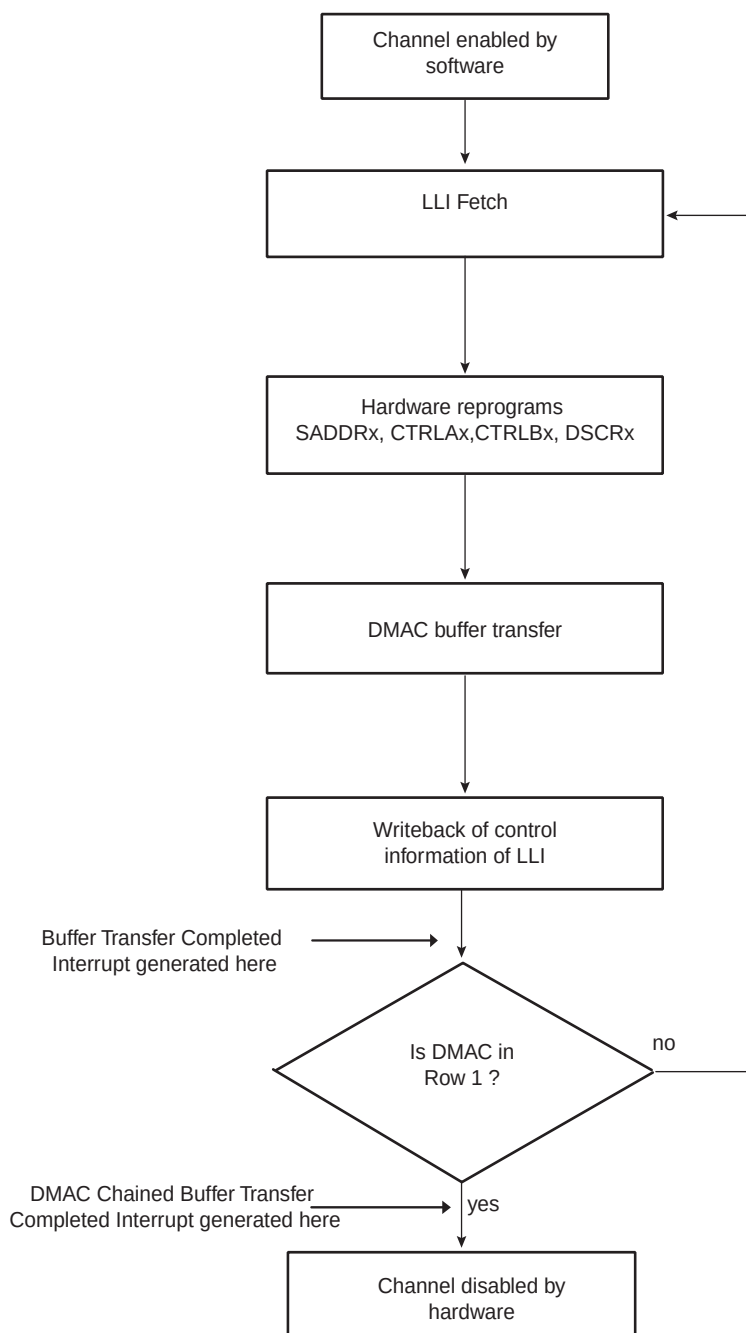
Figure 26-9. DMAC Transfer Flow for Linked List Source Address and Contiguous Destination Address
