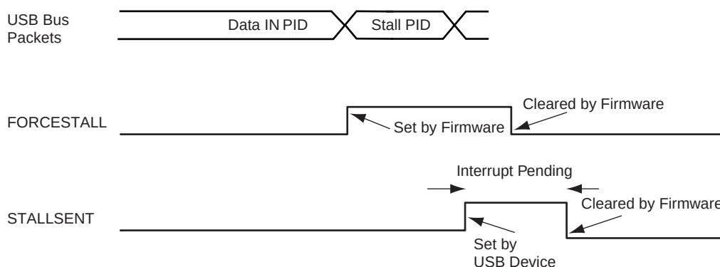
Figure 42-12. Stall Handshake (Data IN Transfer)
