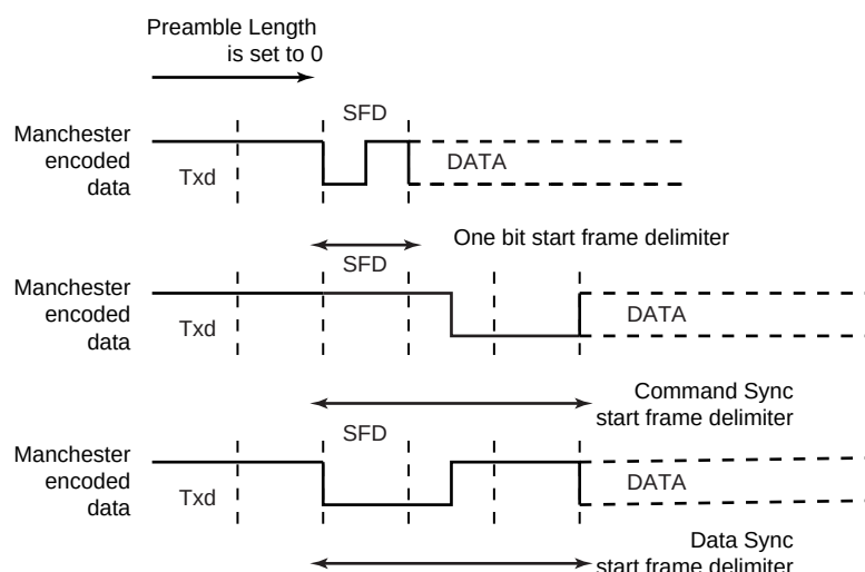
Figure 38-10. Start Frame Delimiter
