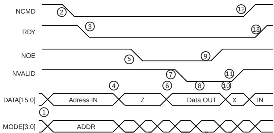
Figure 22-4. Parallel Programming Timing, Read Sequence
