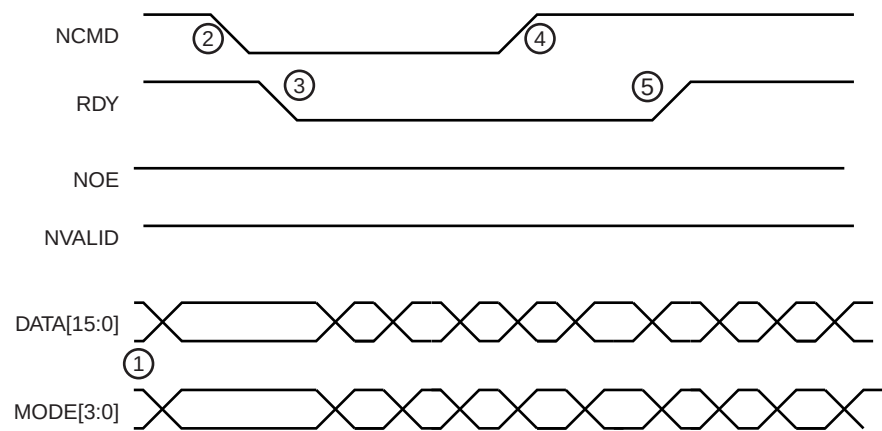
Figure 22-3. Parallel Programming Timing, Write Sequence
