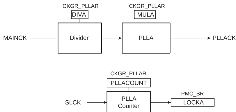
Figure 29-4. Divider and PLL Block Diagram
