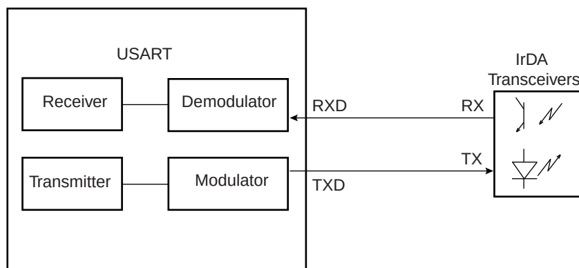
Figure 38-33. Connection to IrDA Transceivers
