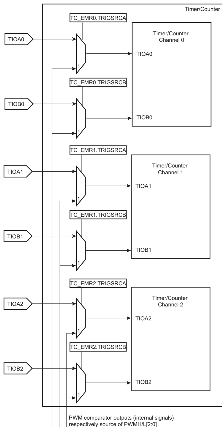
Figure 39-16. Synchronization with PWM
