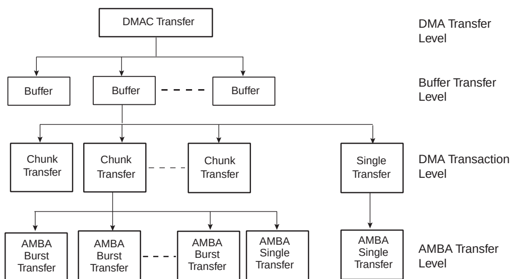
Figure 26-2. DMAC Transfer Hierarchy for Non-Memory Peripheral
