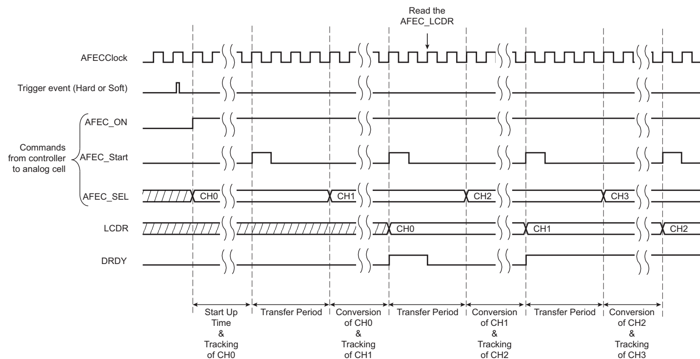
Figure 45-3. Sequence of AFEC conversions when Tracking time < Conversion time
