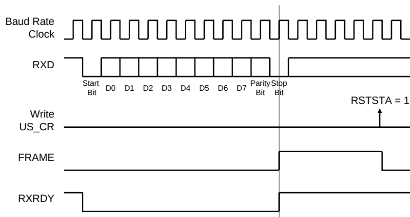
Figure 38-25. Framing Error Status
