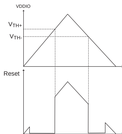
Figure 47-3. Zero-Power-On Reset Characteristics
