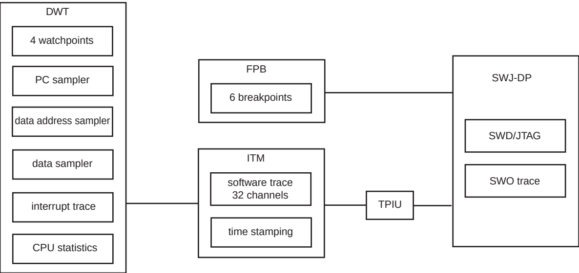
Figure 13-4. Debug Architecture
