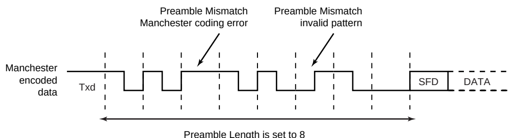
Figure 38-15. Preamble Pattern Mismatch
