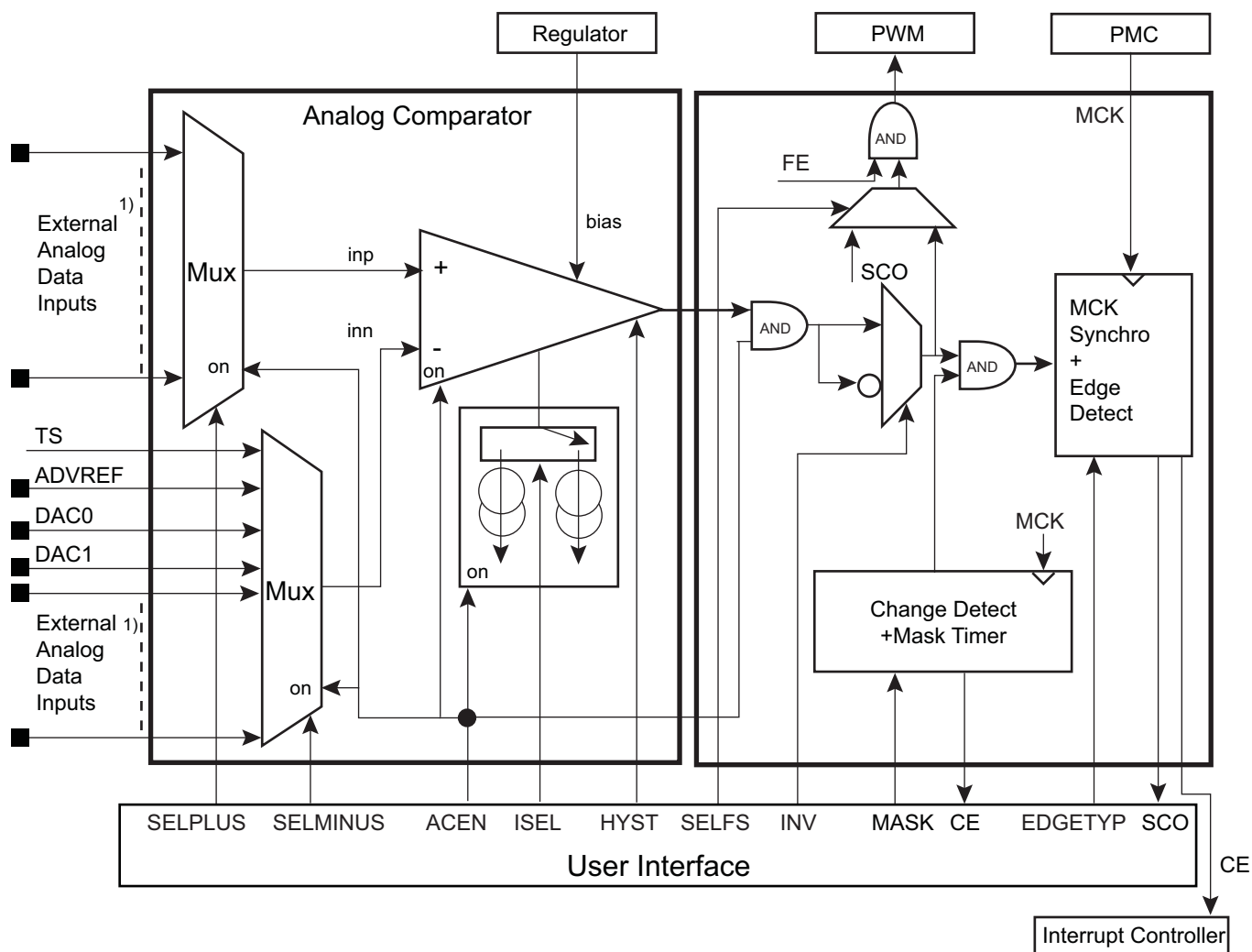
Figure 44-1. Analog Comparator Controller Block Diagram
