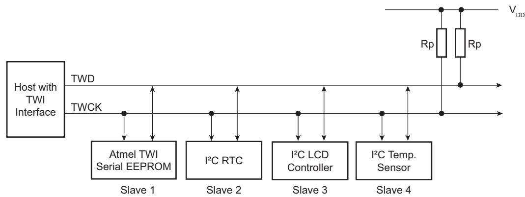
Figure 36-2. Application Block Diagram
