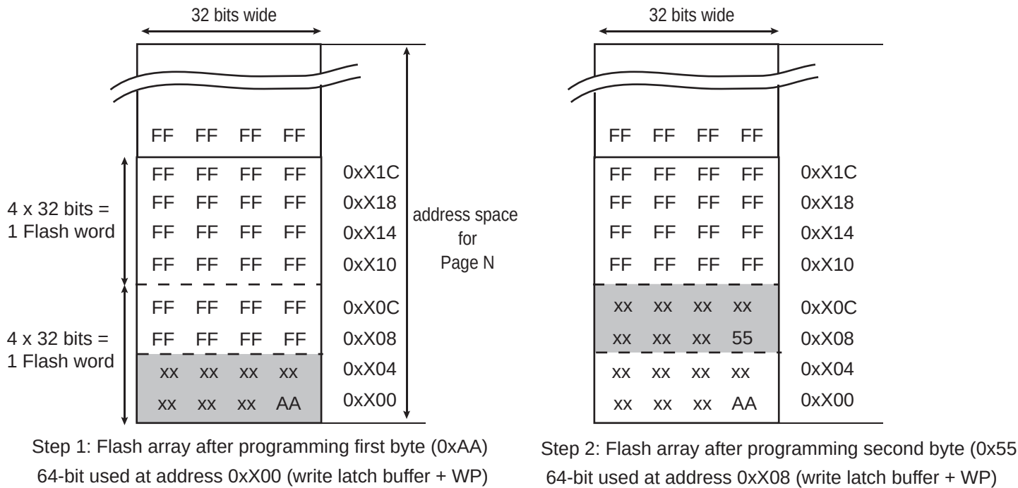
Figure 21-9. Programming Bytes in the Flash
