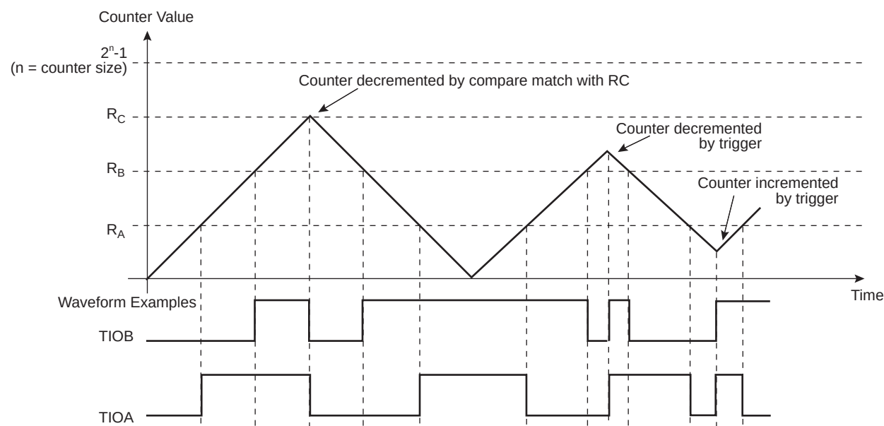
Figure 39-15. WAVSEL = 11 with Trigger
