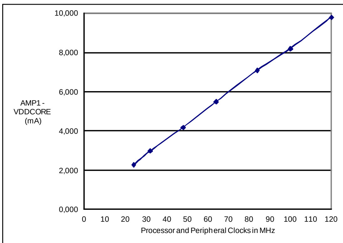
Figure 47-6. Current Consumption in Sleep Mode (AMP1) versus Master Clock Ranges (Condition from Table 47-10)
