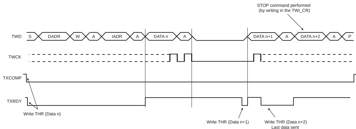
Figure 36-8. Master Write with One Byte Internal Address and Multiple Data Bytes
