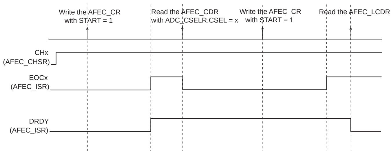
Figure 45-4. EOCx and DRDY Flag Behavior
