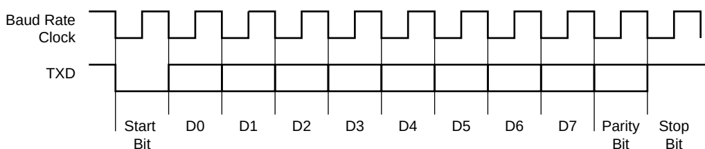
Figure 38-6. Character Transmit
