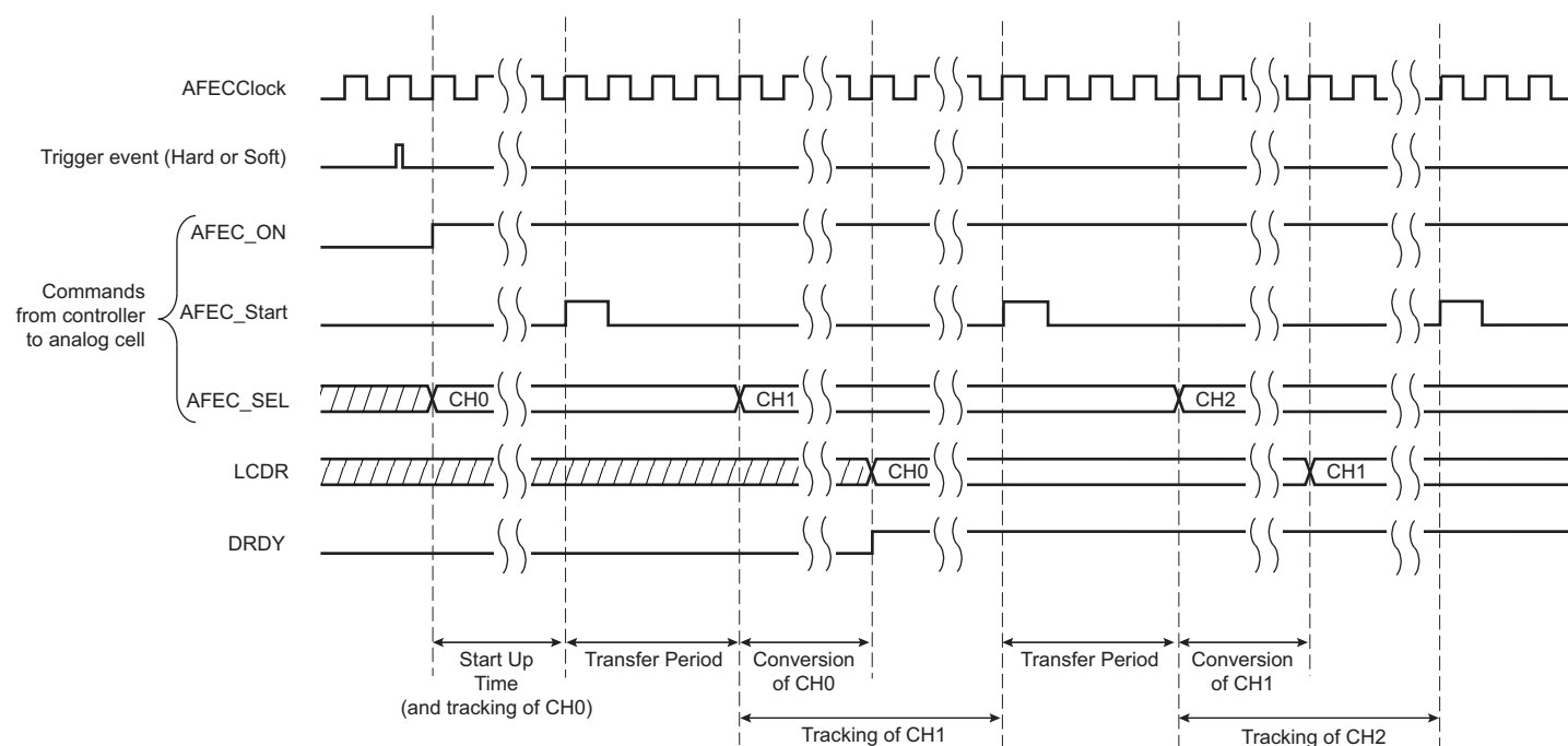
Figure 45-2. Sequence of AFEC conversions when Tracking time > Conversion time
