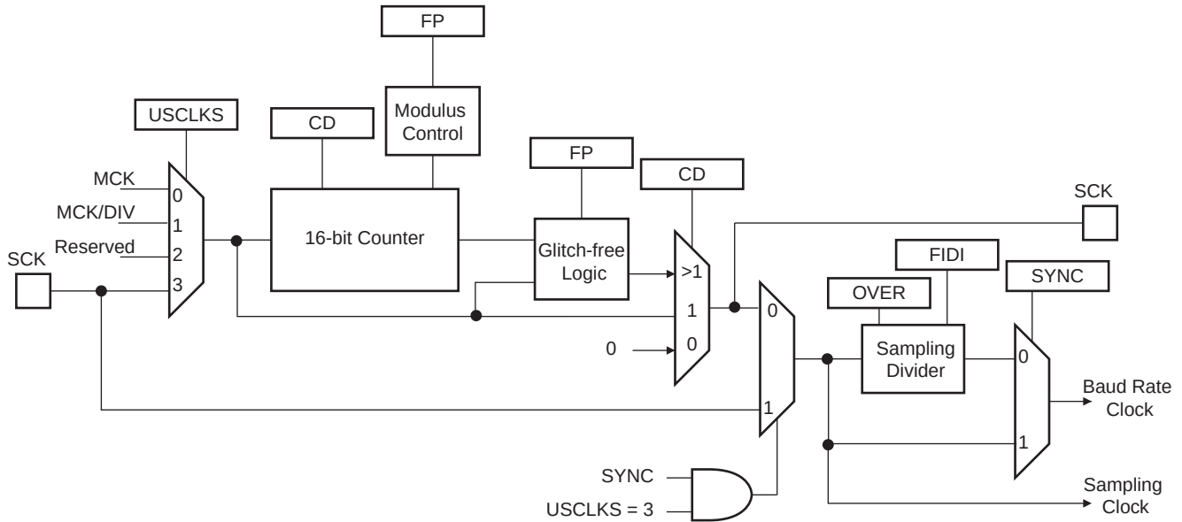
Figure 38-4. Fractional Baud Rate Generator
