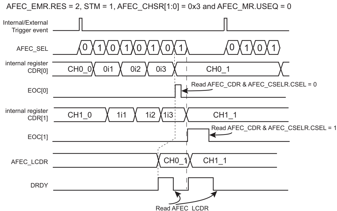
Figure 45-12. Digital Averaging Function Waveforms on a single trigger event
