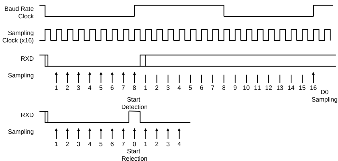
Figure 38-12. Asynchronous Start Detection
