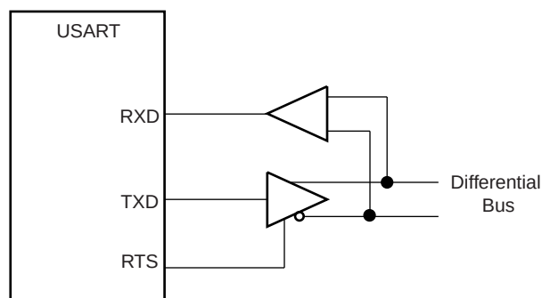
Figure 38-36. Typical Connection to a RS485 Bus
