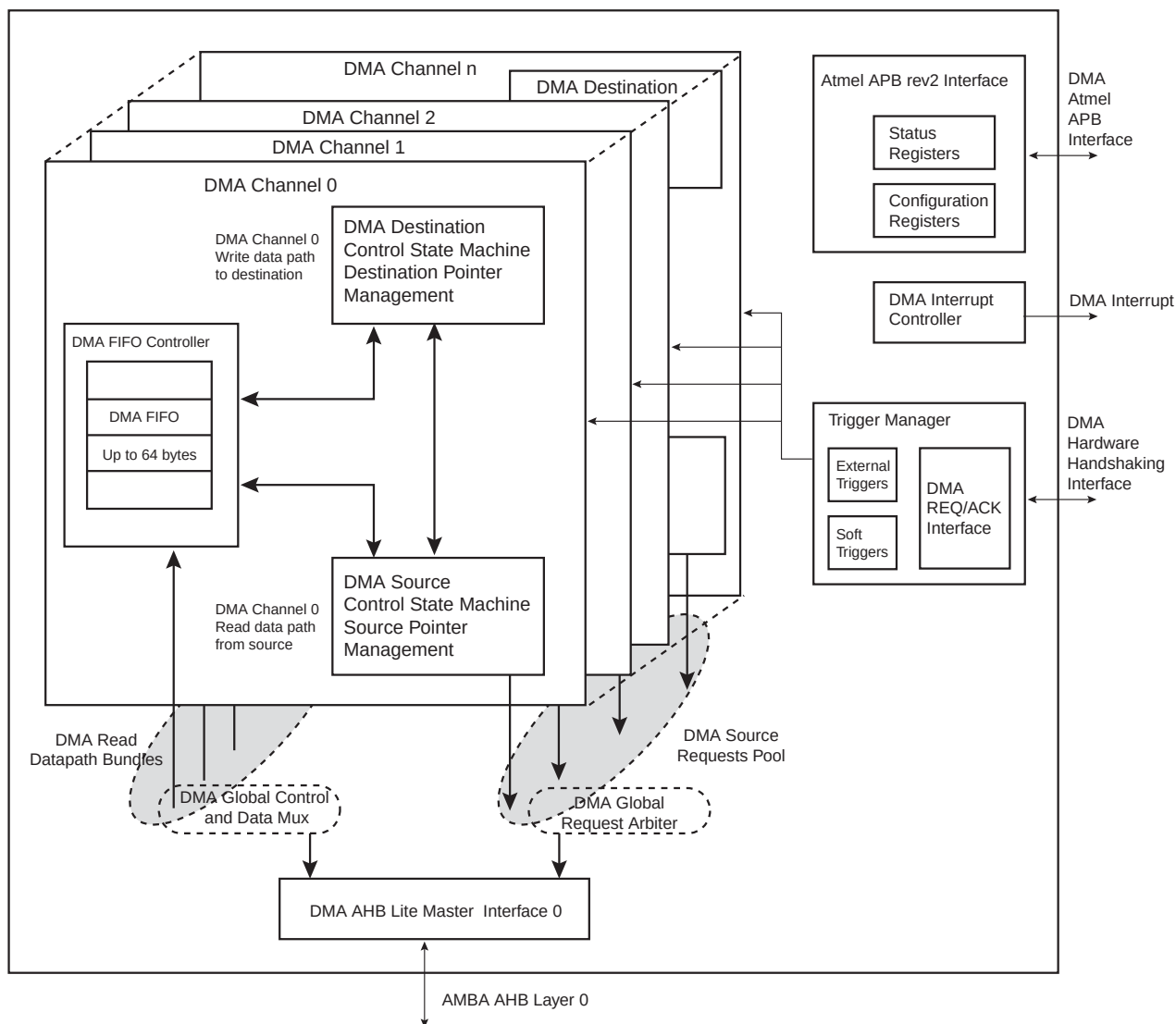
Figure 26-1. DMA Controller (DMAC) Block Diagram
