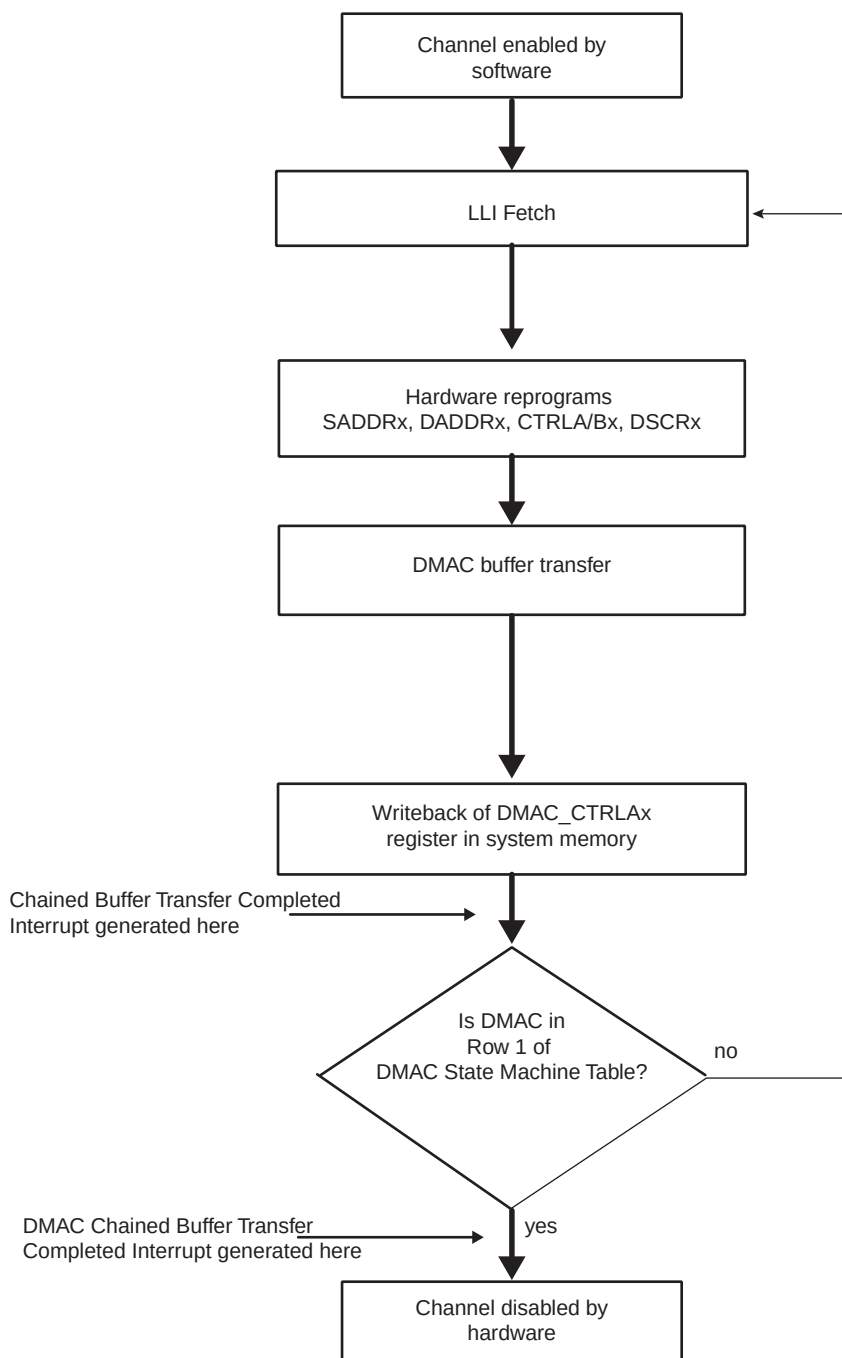
Figure 26-7. DMAC Transfer Flow for Source and Destination Linked List Address
