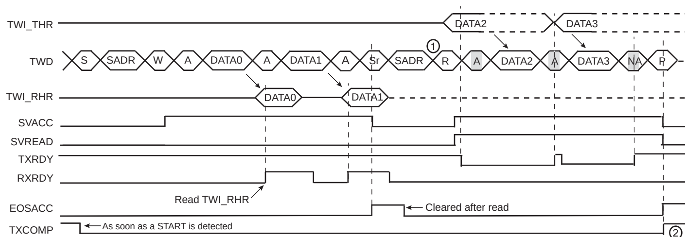
Figure 36-32. Repeated Start + Reversal from Write to Read Mode
