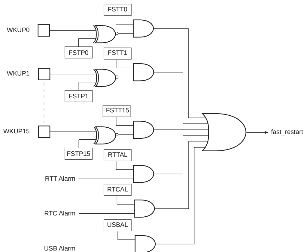
Figure 30-4. Fast Startup Circuitry
