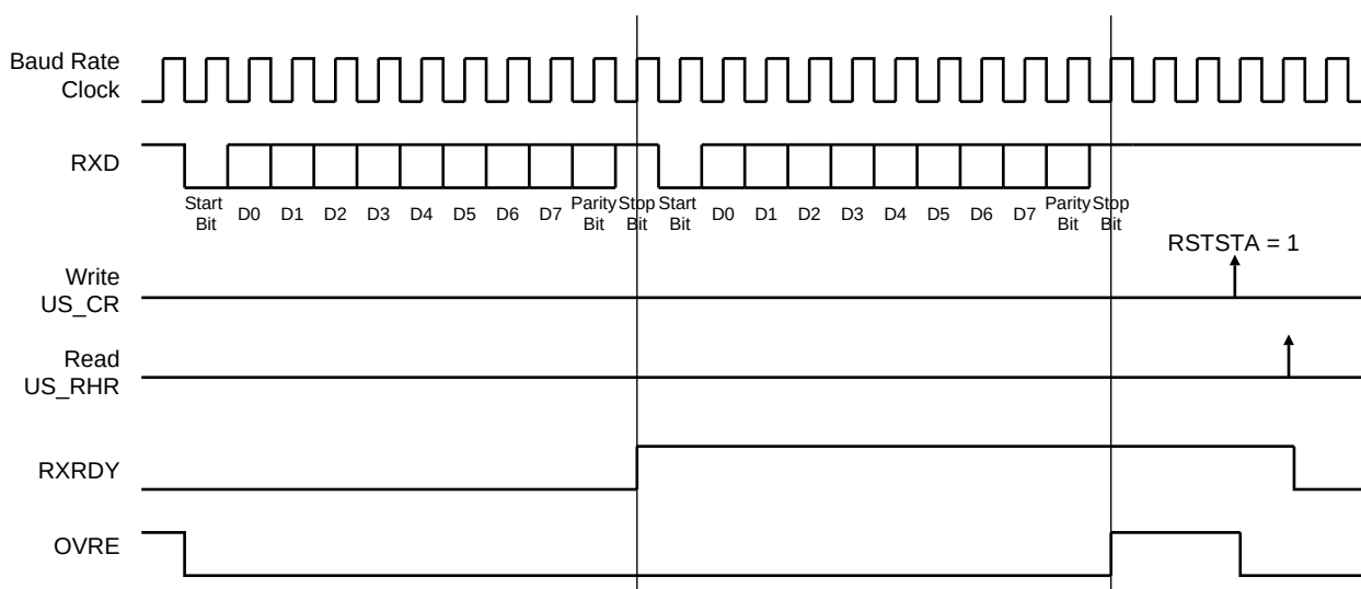
Figure 38-21. Receiver Status
