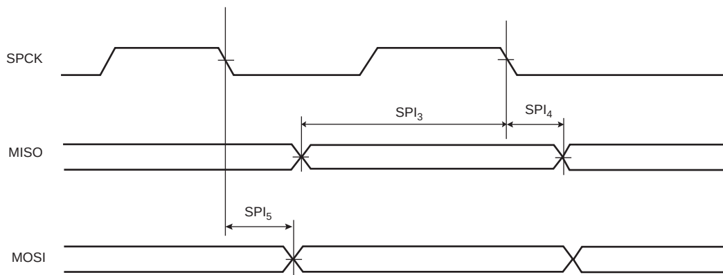
Figure 47-20. SPI Master Mode with (CPOL = 0 and NCPHA=1) or (CPOL=1 and NCPHA= 0)
