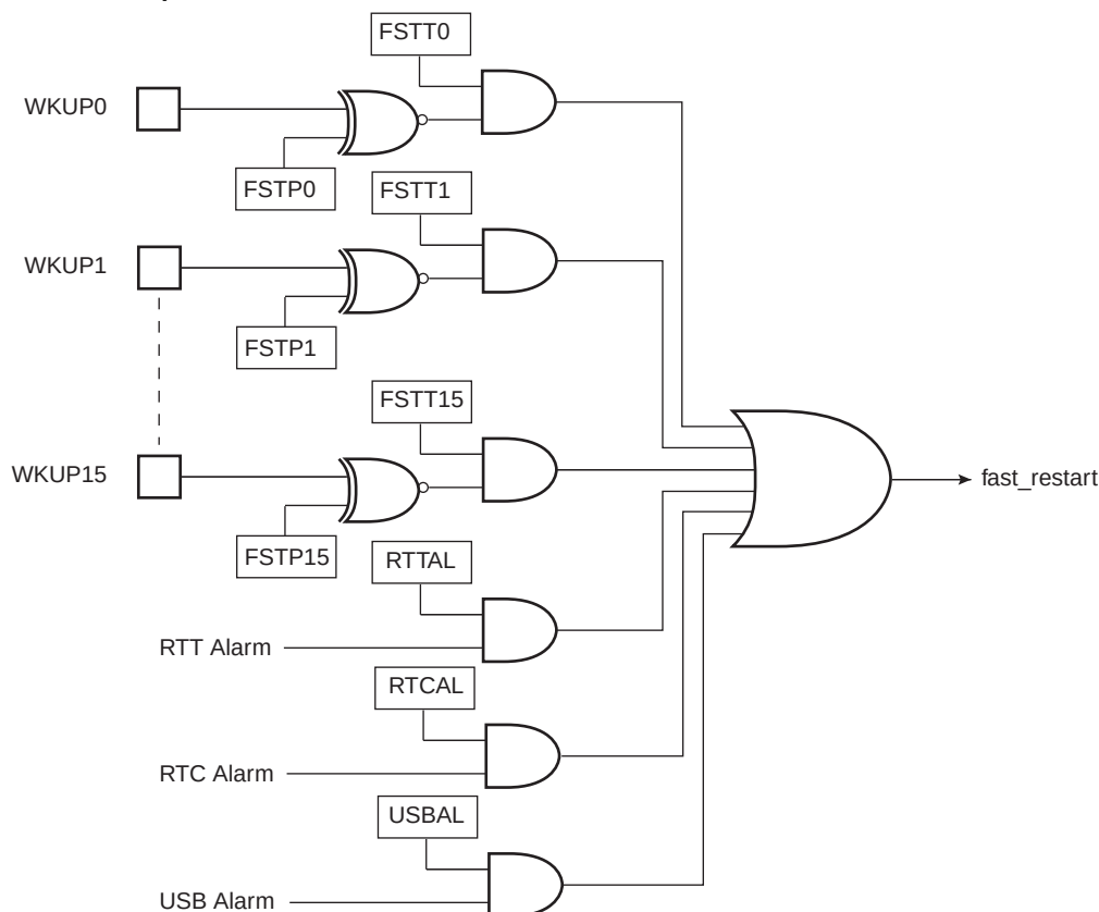
Figure 5-4. Fast Start-up Sources
