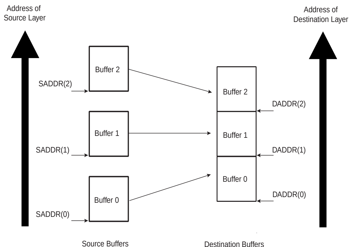
Figure 26-8. DMAC Transfer with Linked List Source Address and Contiguous Destination Address
