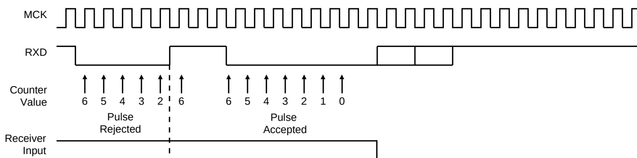
Figure 38-35. IrDA Demodulator Operations
