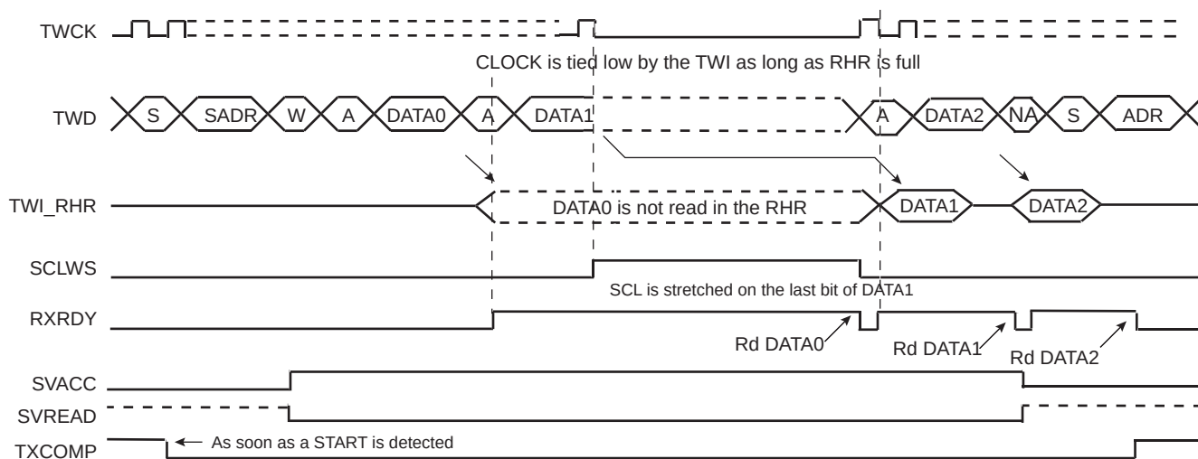
Figure 36-30. Clock Synchronization in Write Mode
