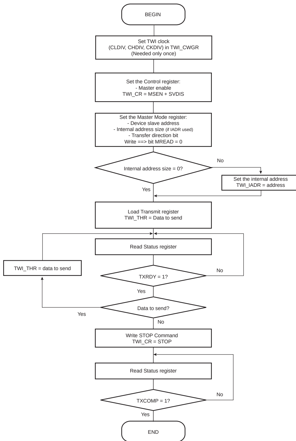
Figure 36-18. TWI Write Operation with Multiple Data Bytes with or without Internal Address
