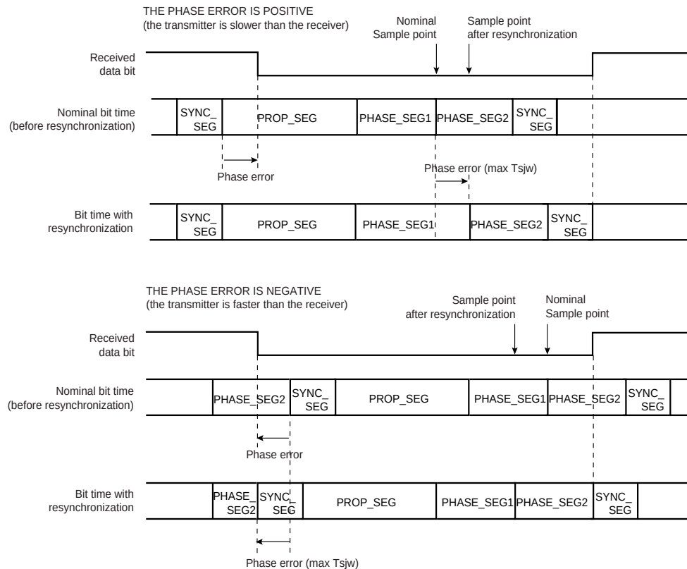
Figure 33-6. CAN Resynchronization
