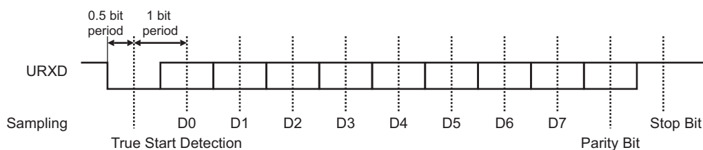
Figure 37-4. Character Reception
