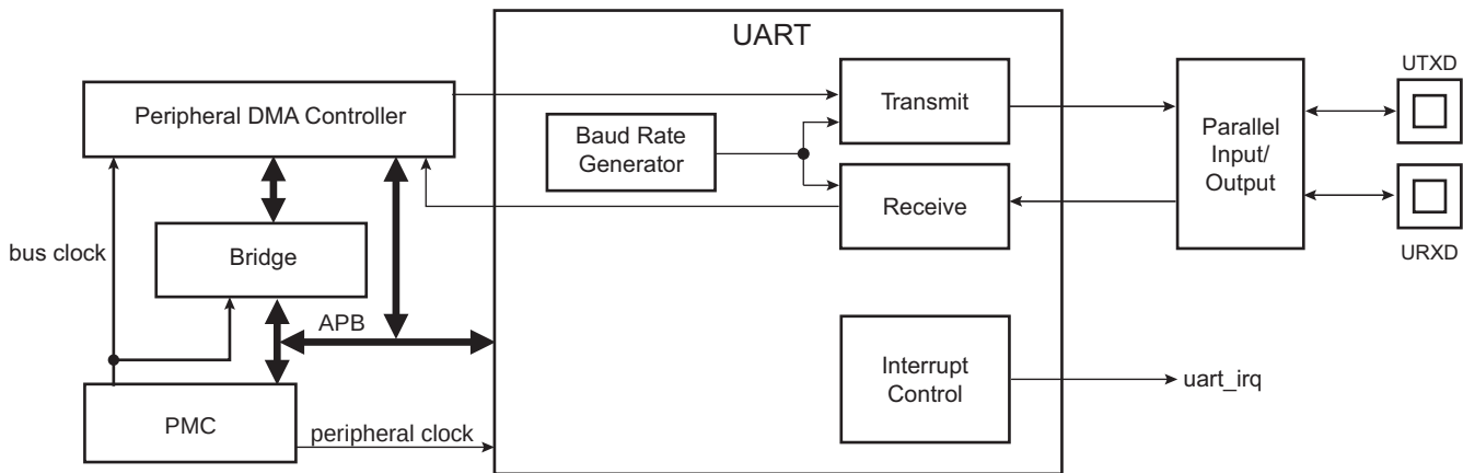
Figure 37-1. UART Functional Block Diagram
