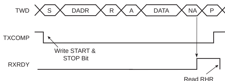
Figure 36-9. Master Read with One Data Byte
