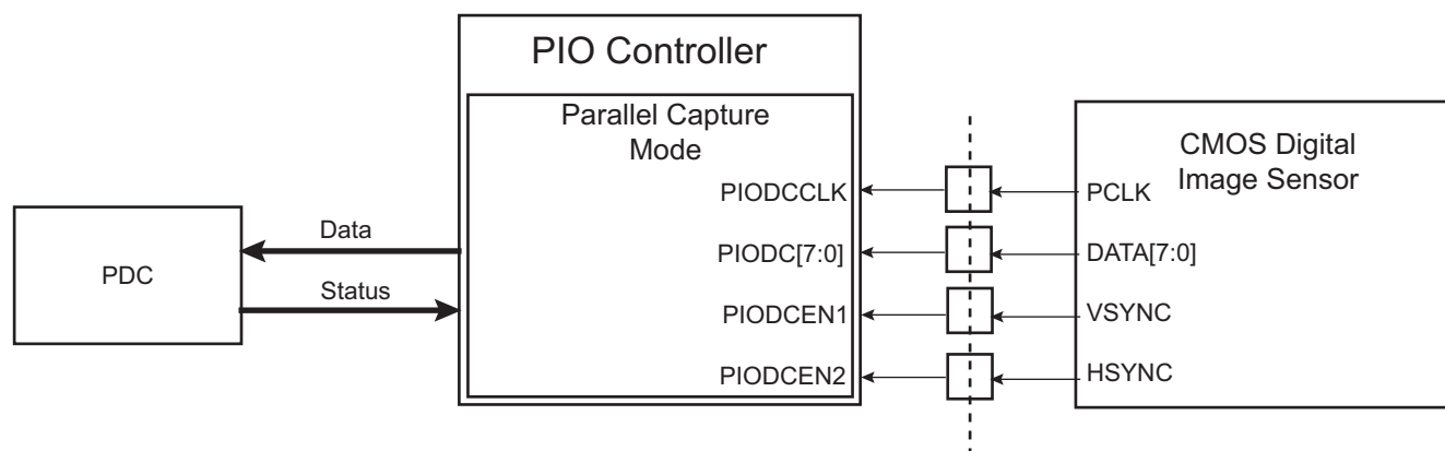
Figure 34-10. PIO Controller Connection with CMOS Digital Image Sensor
