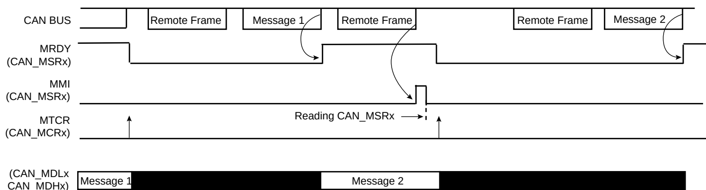
Figure 33-17. Producer Handling
