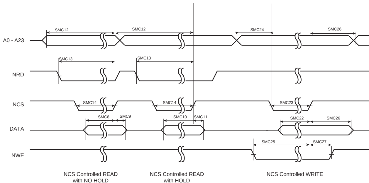
Figure 47-23. SMC Timings - NCS Controlled Read and Write
