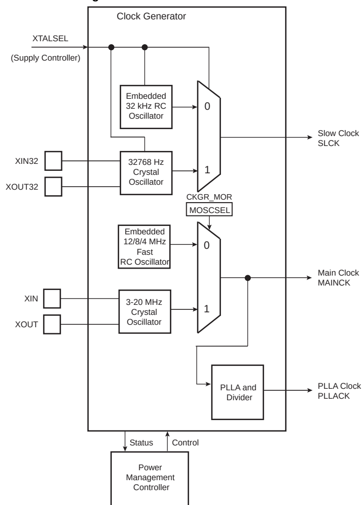
Figure 29-1. Clock Generator Block Diagram
