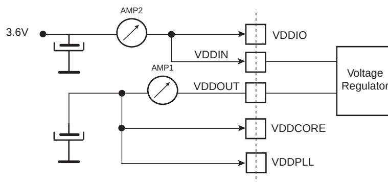
Figure 47-7. Measurement Setup for Wait Mode
