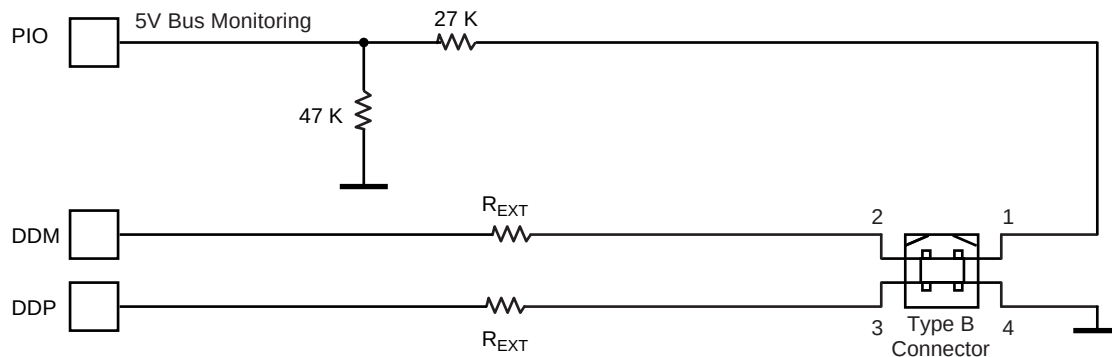
Figure 42-2. Board Schematic to Interface Device Peripheral
