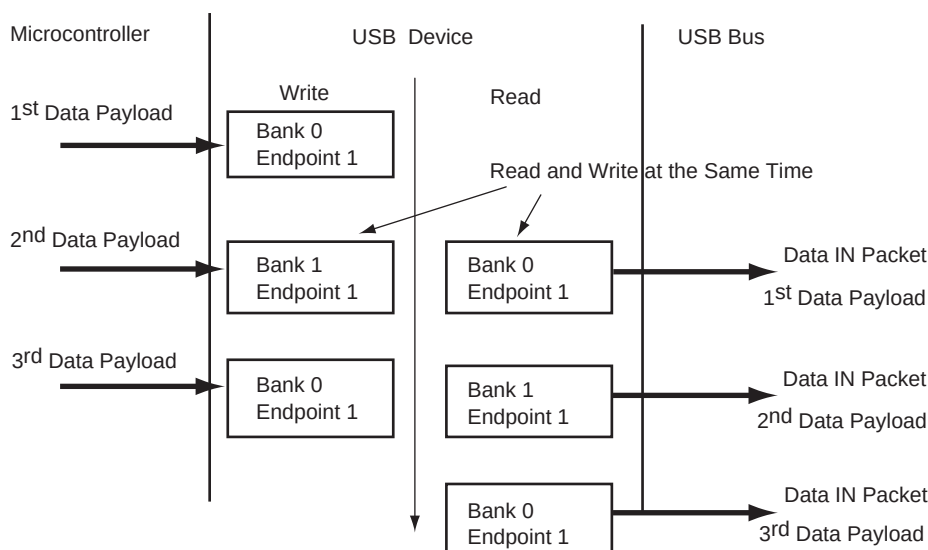
Figure 42-7. Bank Swapping Data IN Transfer for Ping-pong Endpoints
