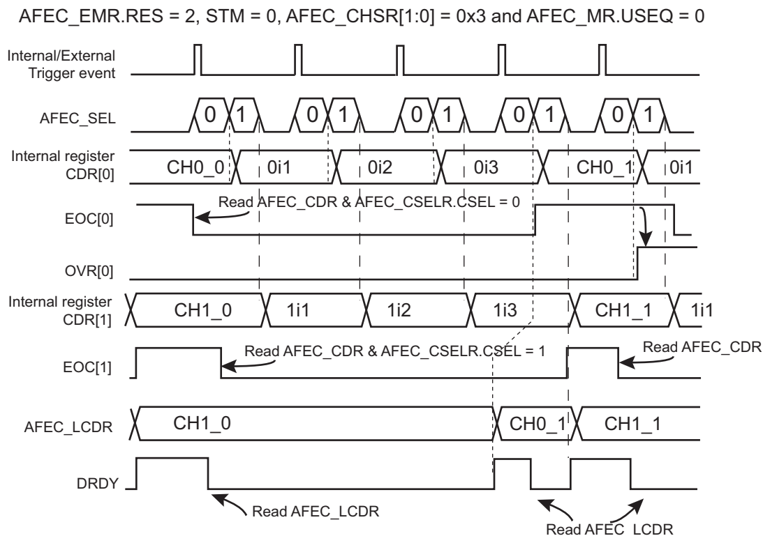
Figure 45-11. Digital Averaging Function Waveforms over multiple trigger events
