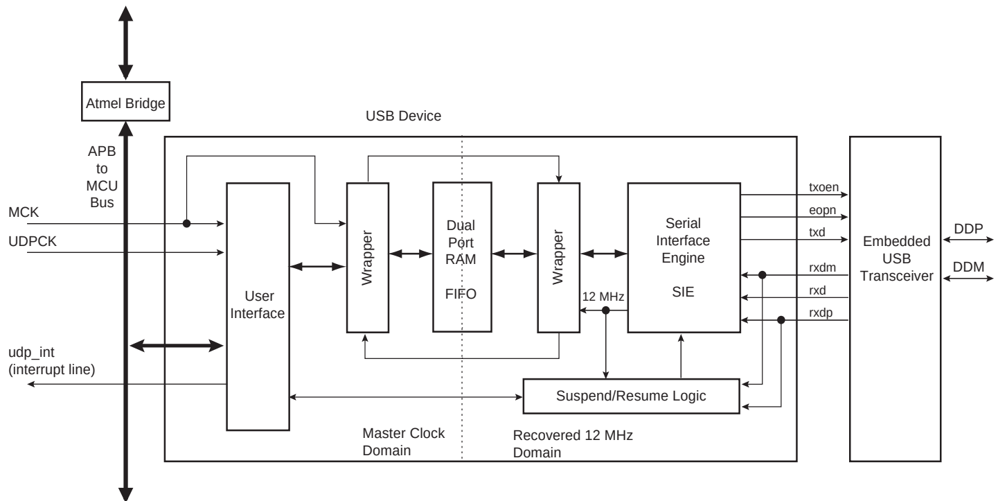
Figure 42-1. Block Diagram
