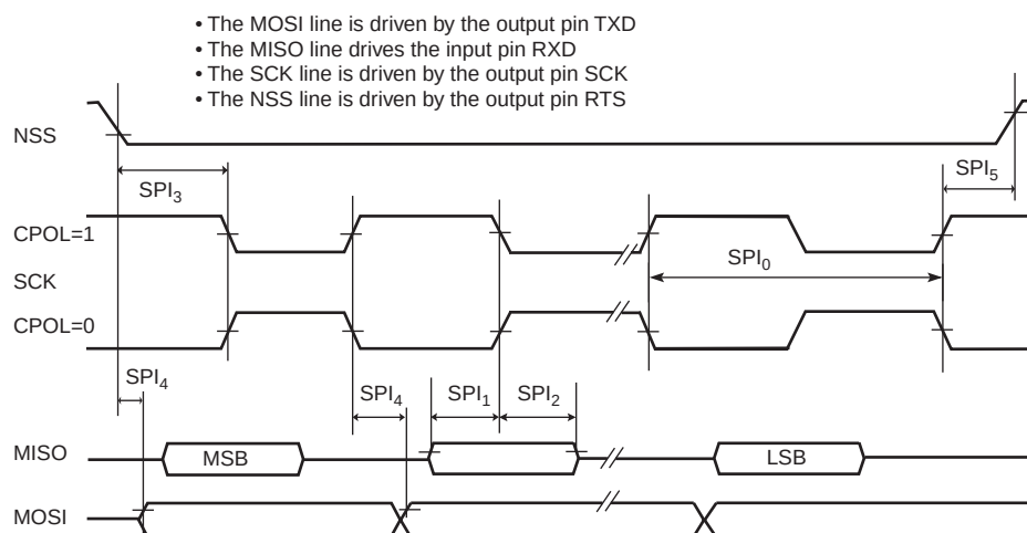
Figure 47-25. USART SPI Master Mode
