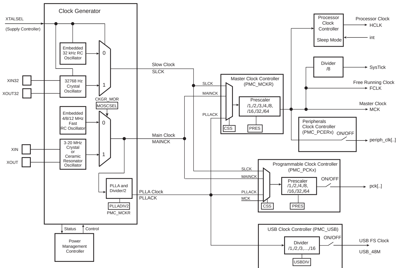
Figure 30-1. General Clock Block Diagram
