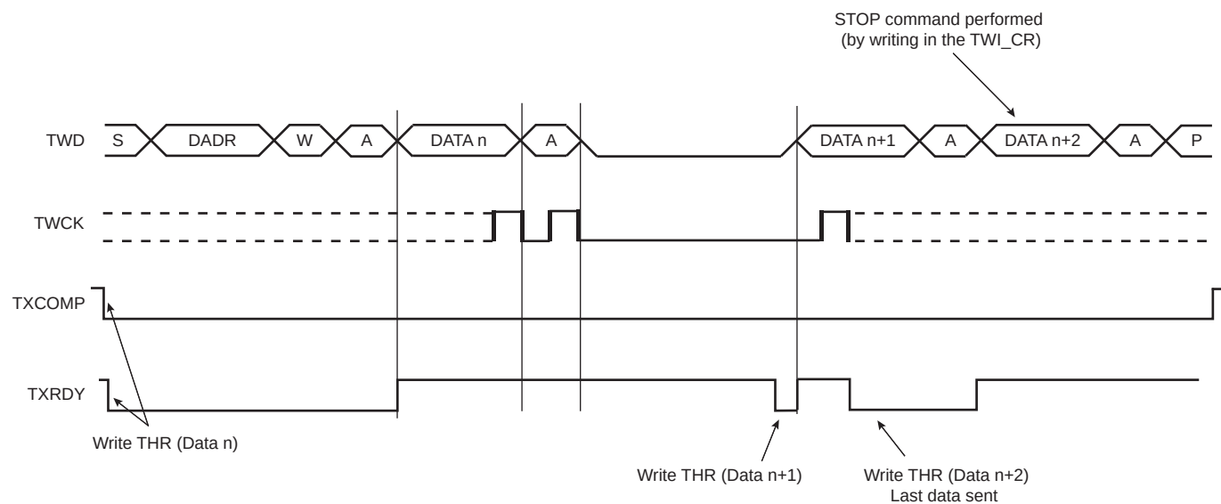
Figure 36-7. Master Write with Multiple Data Bytes
