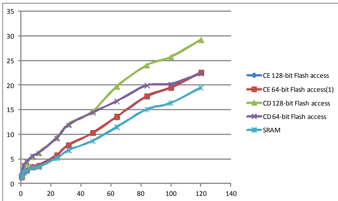
Figure 47-10. Active Total Power Consumption with VDDCORE @ 1.2V
