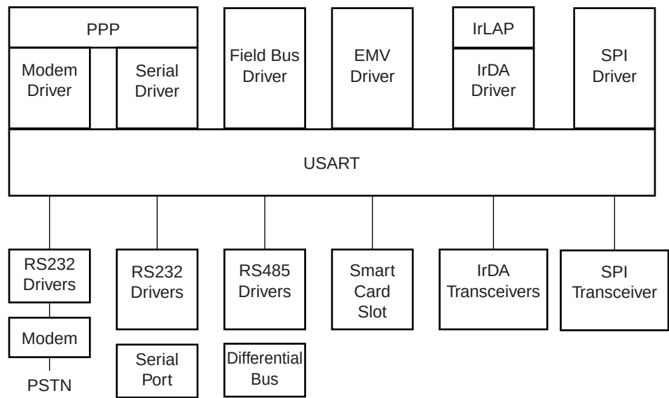
Figure 38-2. Application Block Diagram
