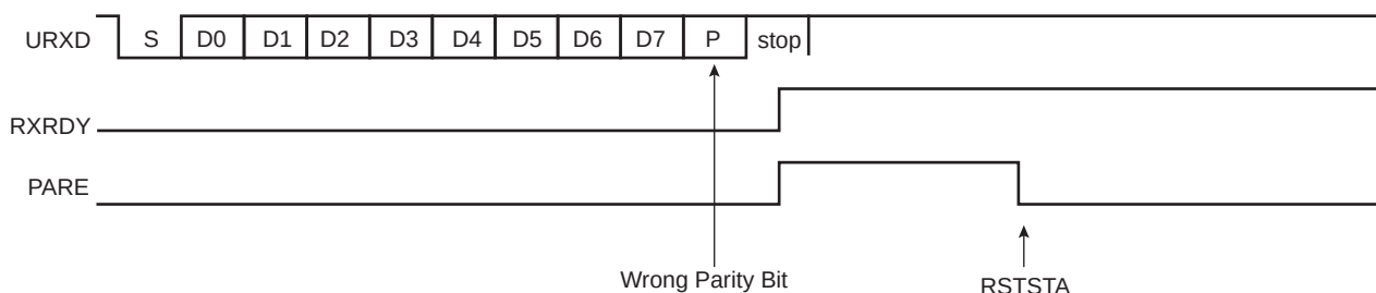
Figure 37-7. Parity Error
