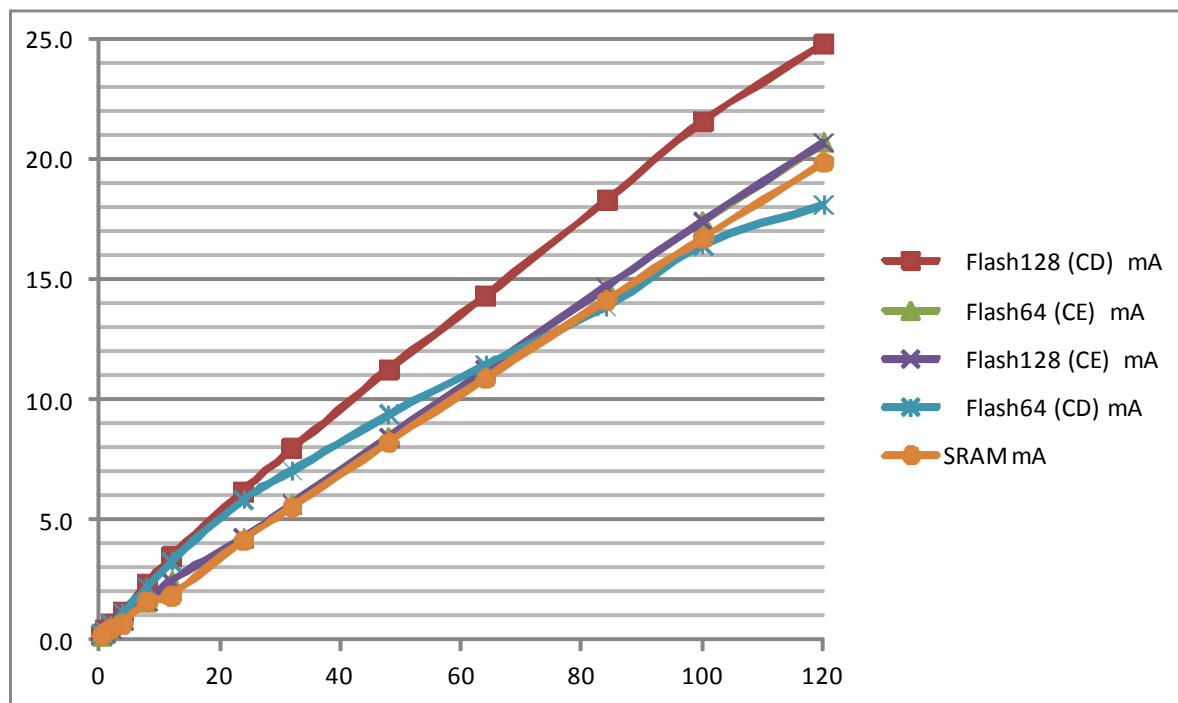
Figure 47-9. Active Power Consumption with VDDCORE @ 1.2V
