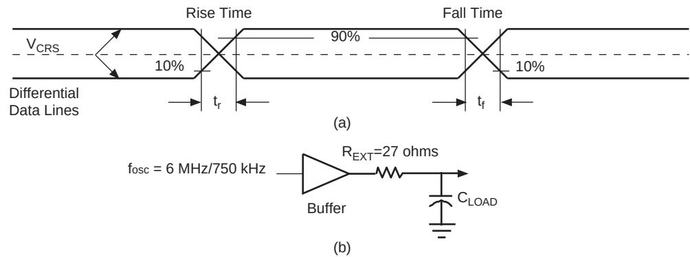
Figure 47-13. USB Data Signal Rise and Fall Times
