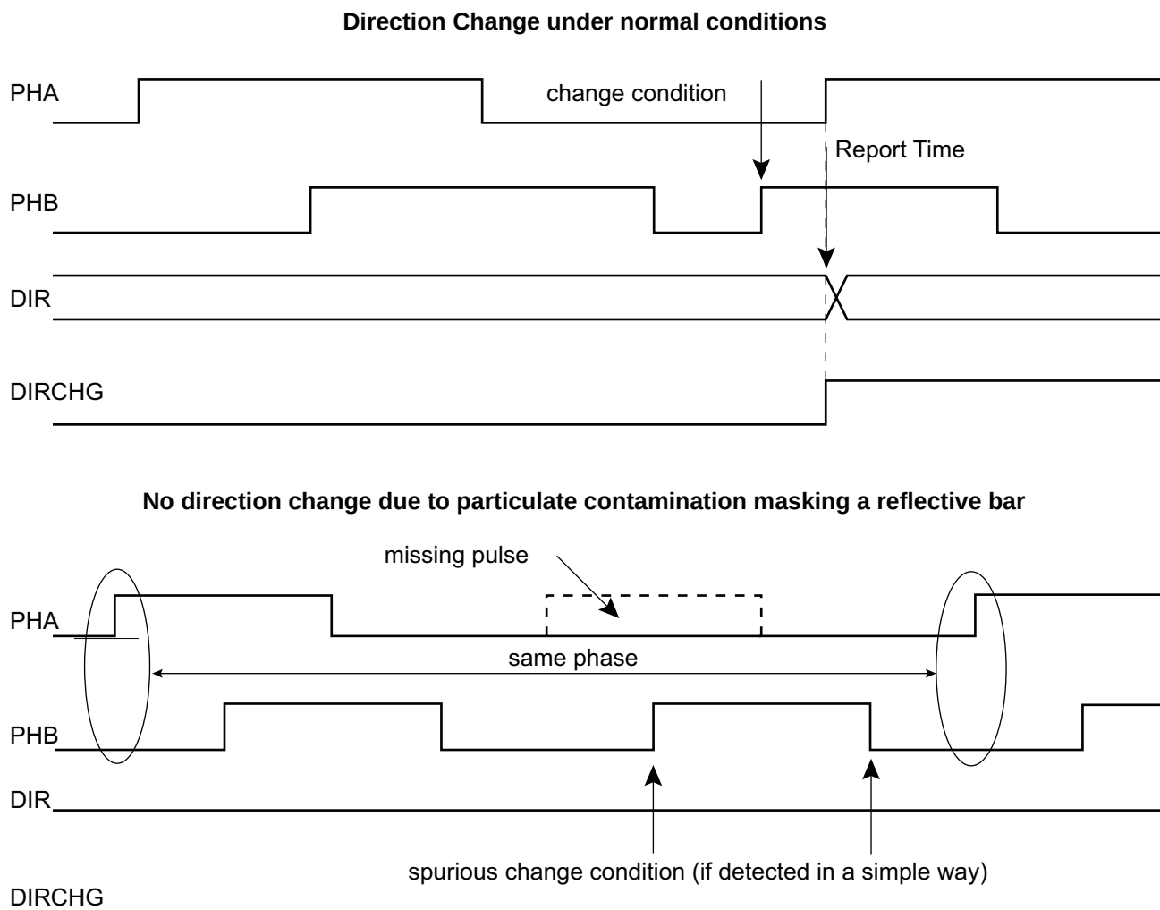
Figure 39-20. Rotation Change Detection
