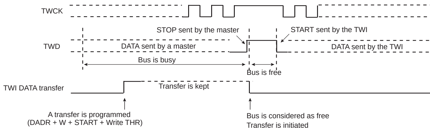
Figure 36-22. Programmer Sends Data While the Bus is Busy
