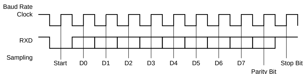
Figure 38-20. Synchronous Mode Character Reception
