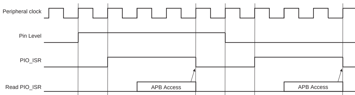
Figure 34-8. Input Change Interrupt Timings When No Additional Interrupt Modes
