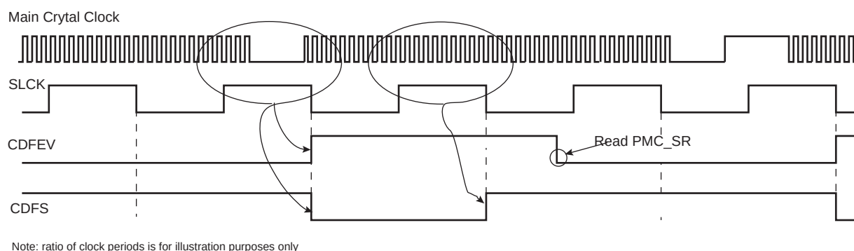
Figure 30-5. Clock Failure Detection (Example)
