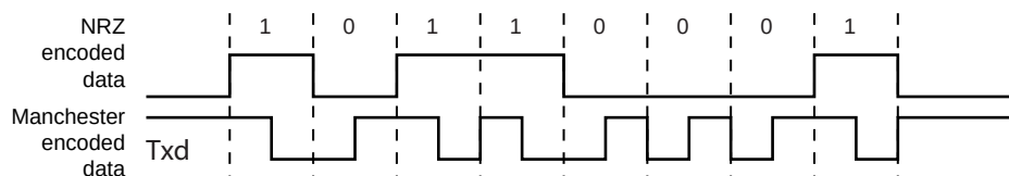
Figure 38-8. NRZ to Manchester Encoding
