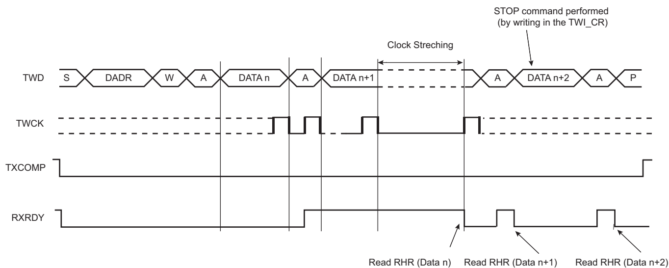
Figure 36-11. Master Read Clock Stretching with Multiple Data Bytes
