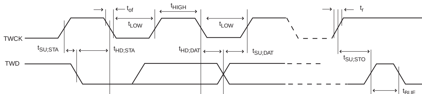
Figure 47-28. Two-wire Serial Bus Timing
