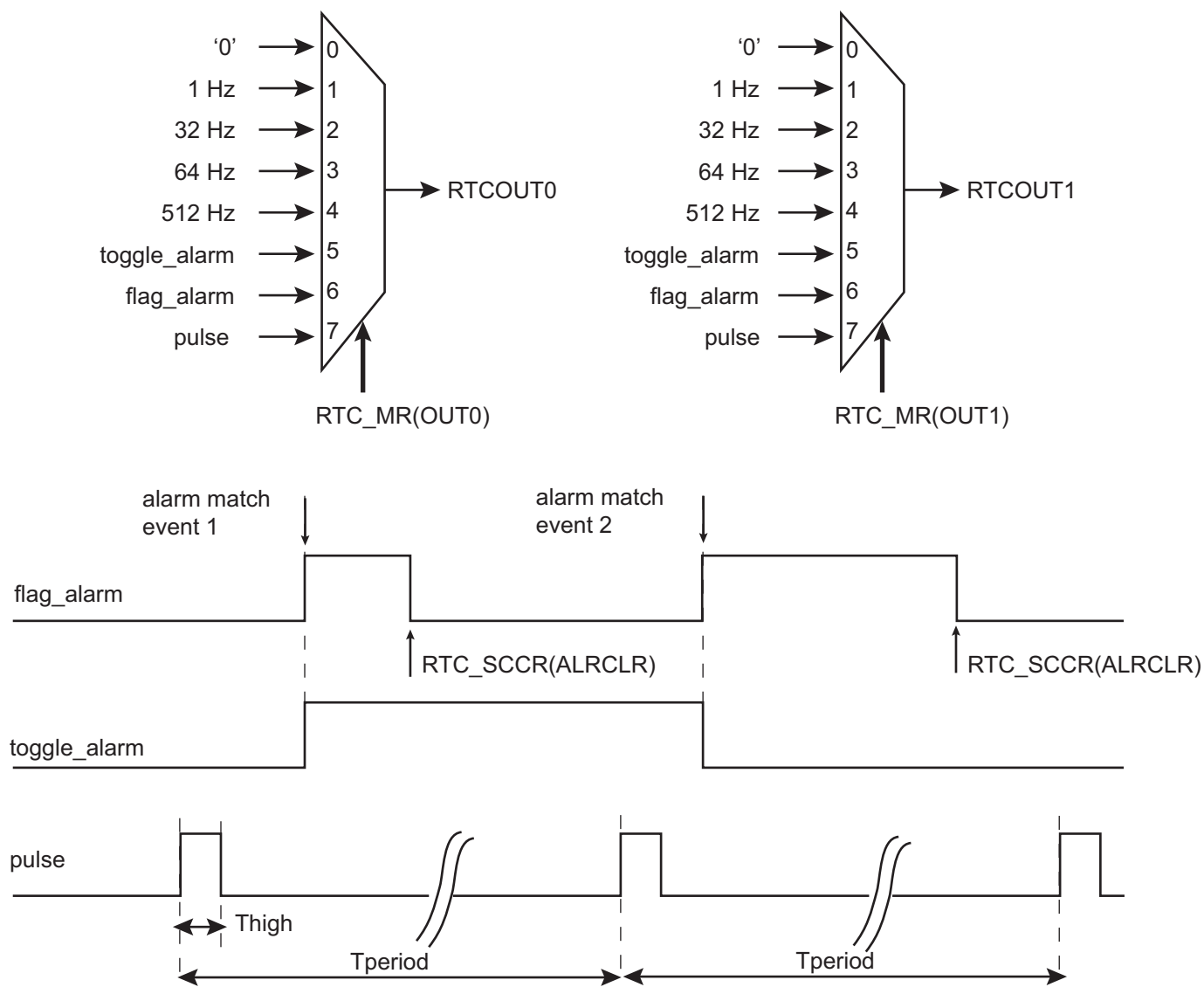
Figure 15-6. Waveform Generation
