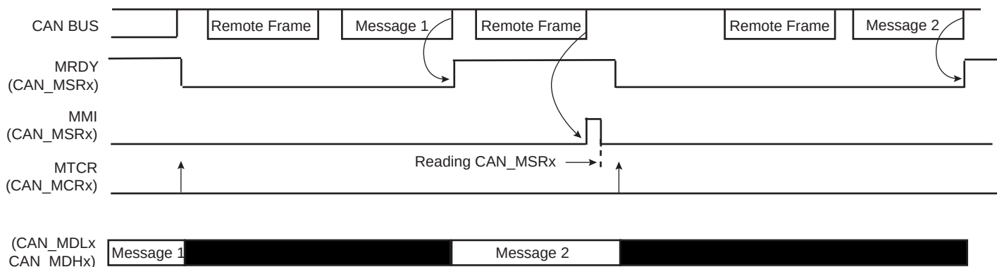
Figure 31-17. Producer Handling
