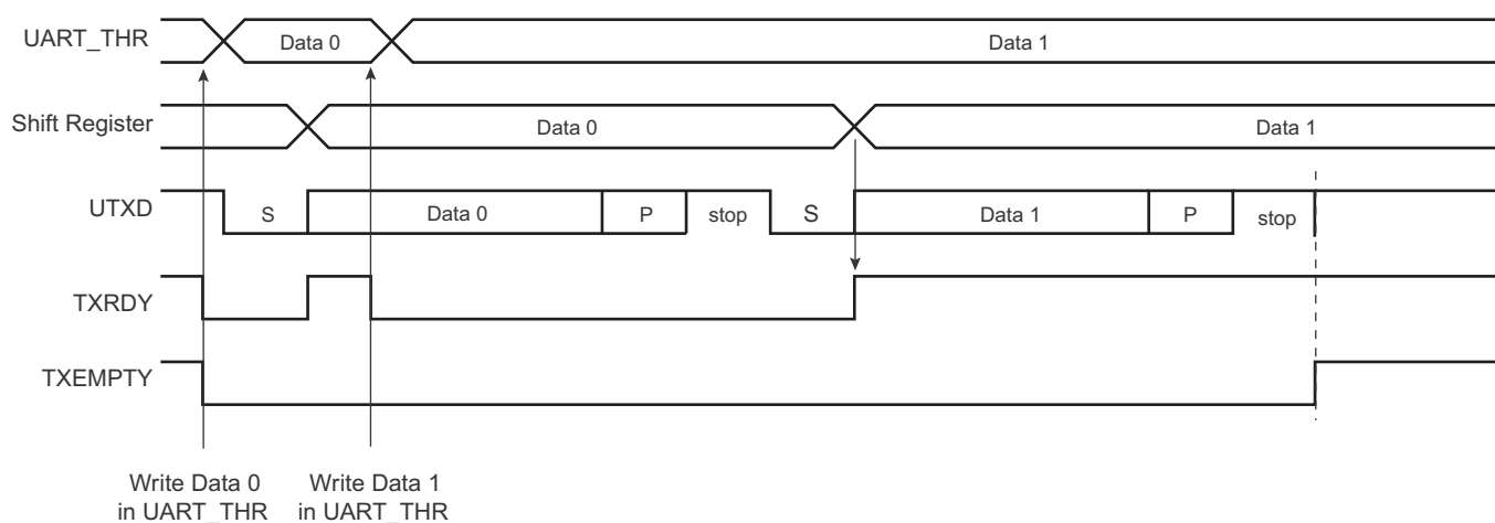
Figure 36-10. Transmitter Control
