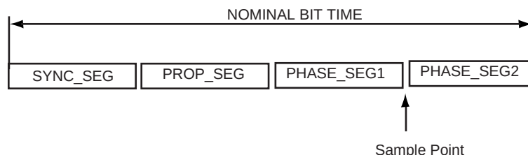
Figure 31-4. Partition of the CAN Bit Time
