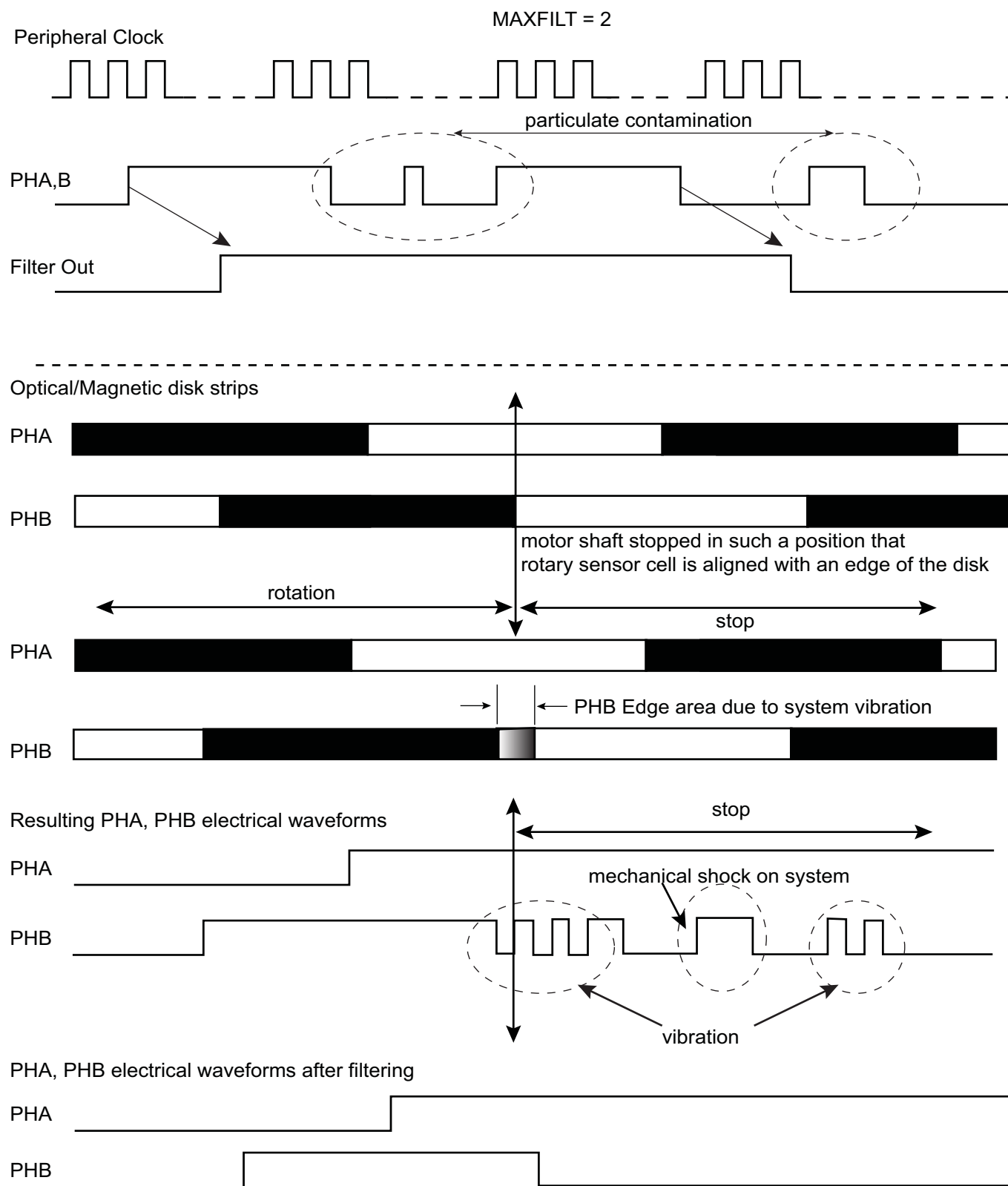
Figure 38-19. Filtering Examples
