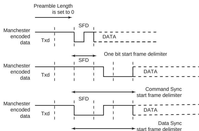
Figure 37-9. Start Frame Delimiter
