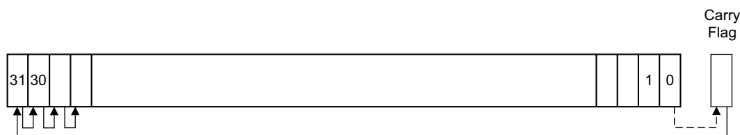
Figure 11-12. RRX
