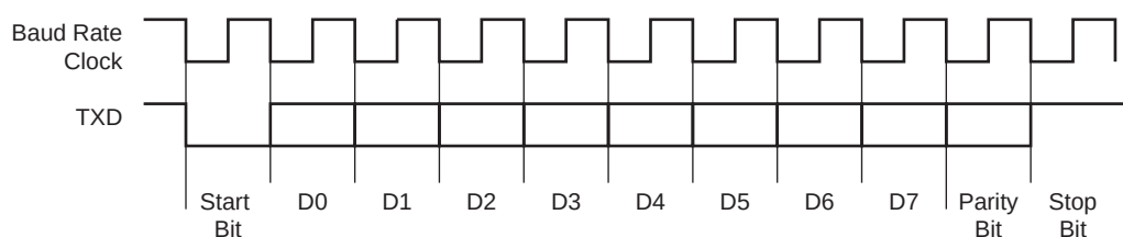
Figure 37-5. Character Transmit
