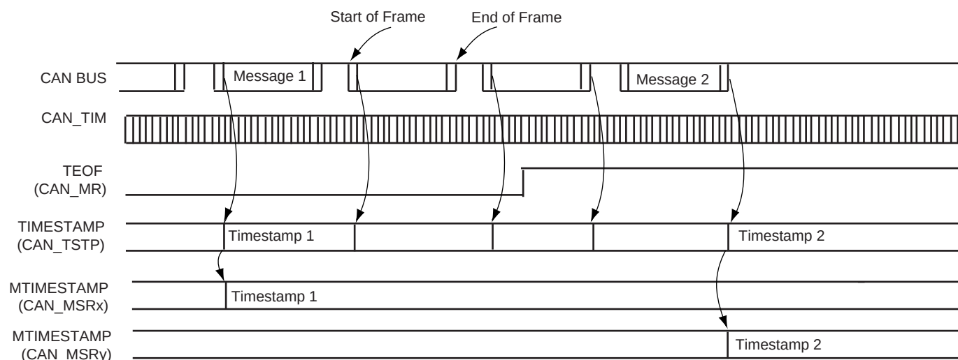
Figure 31-19. Mailbox Timestamp
