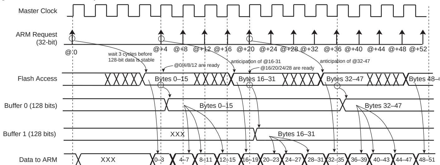
Figure 20-4. Code Read Optimization for FWS = 3
