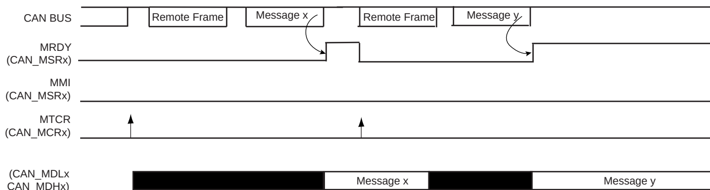
Figure 31-18. Consumer Handling
