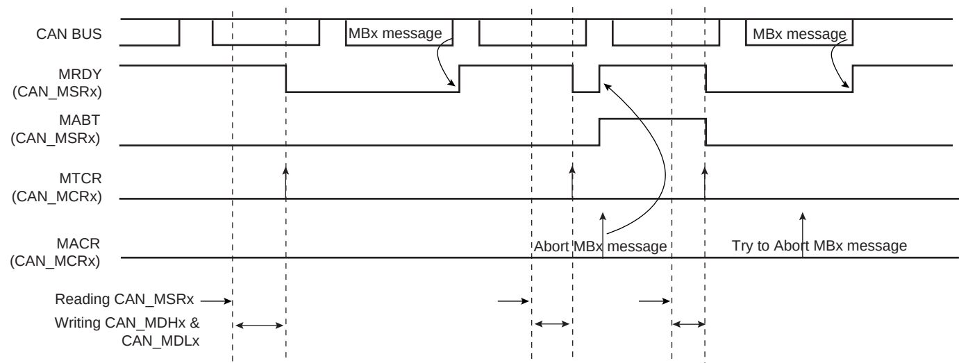
Figure 31-15. Transmitting Messages
