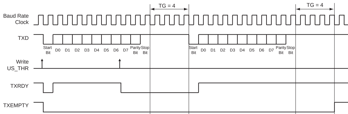
Figure 37-22. Timeguard Operations
