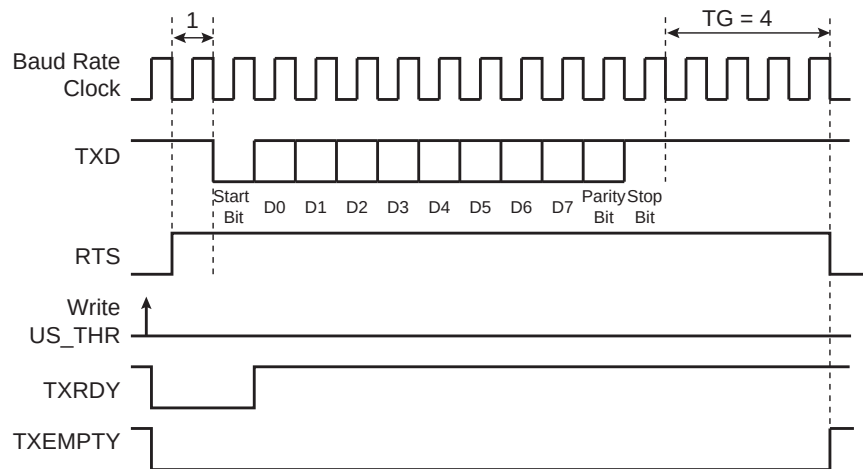
Figure 37-36. Example of RTS Drive with Timeguard
