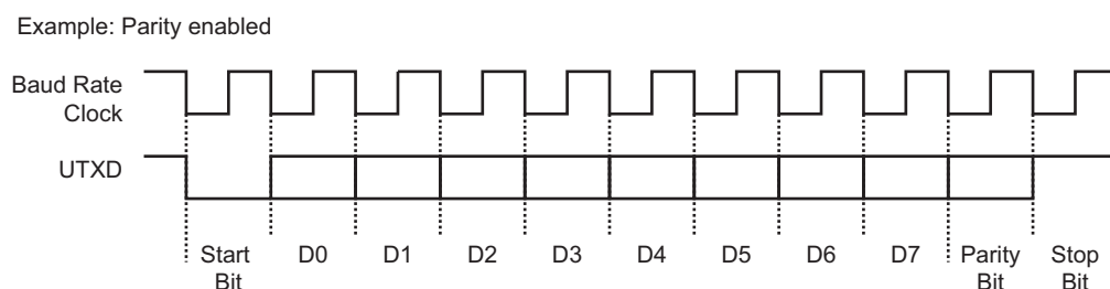
Figure 36-9. Character Transmission
