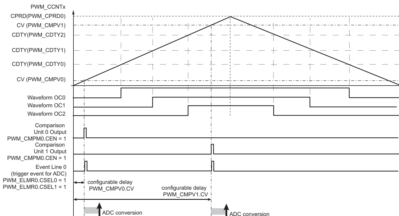
Figure 39-20. Event Line Generation Waveform (Example)
