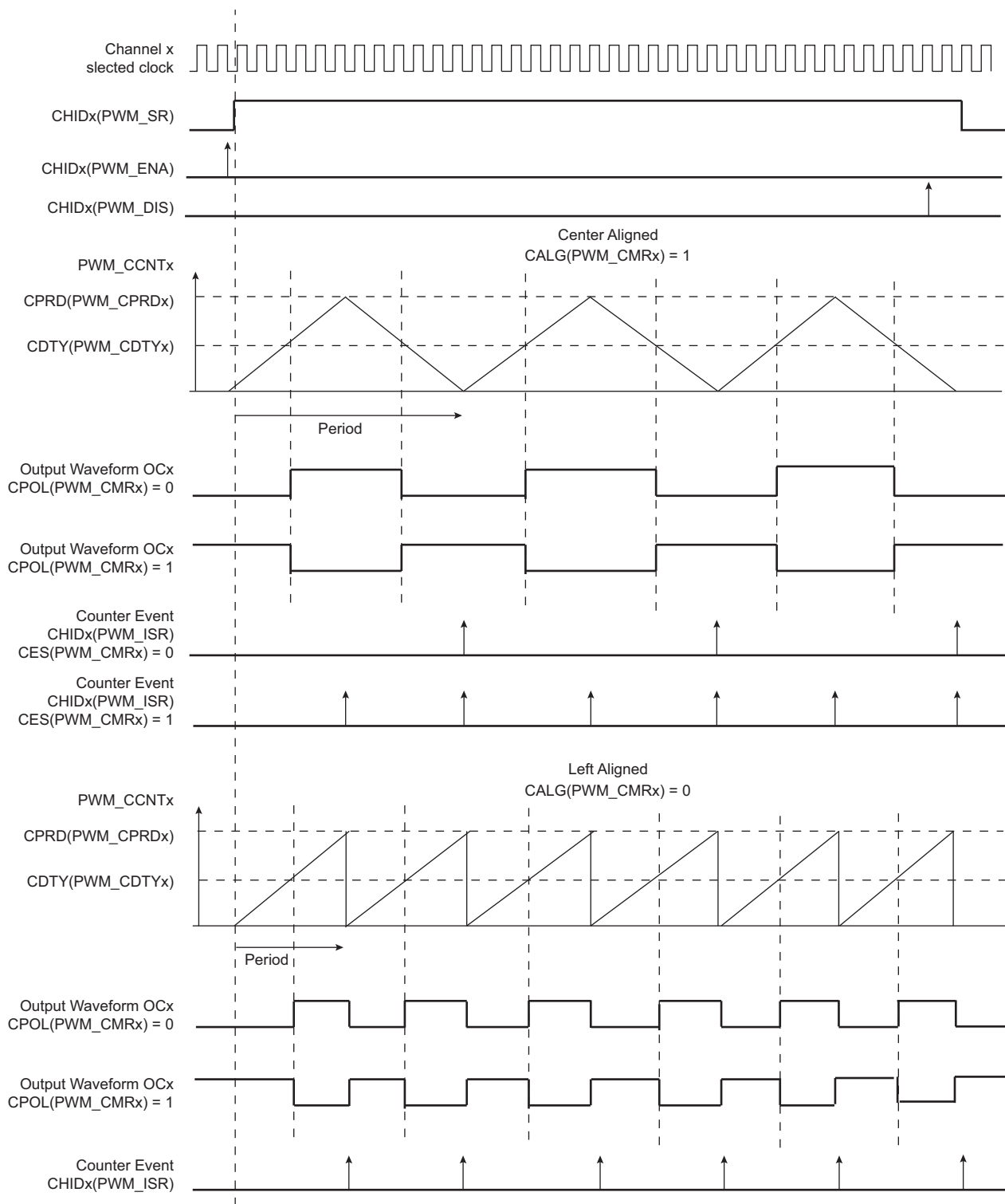
Figure 39-5. Waveform Properties
