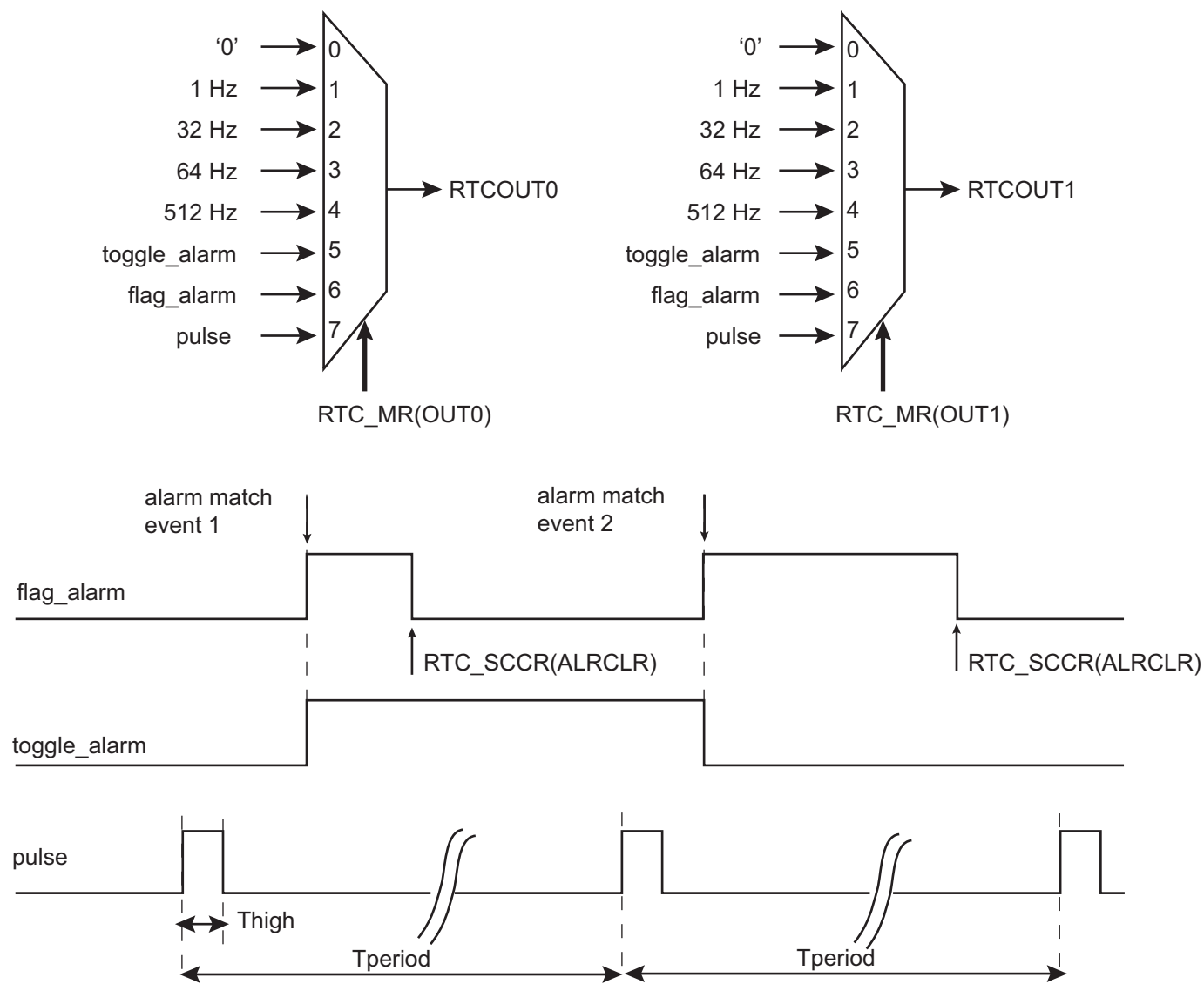
Figure 16-5. Waveform Generation
