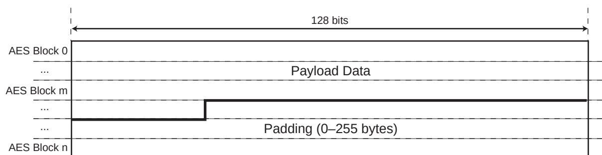
Figure 57-10. SSL Padding
