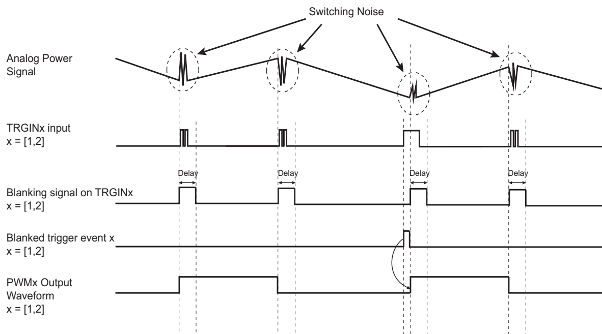
Figure 53-33. Leading-Edge Blanking
