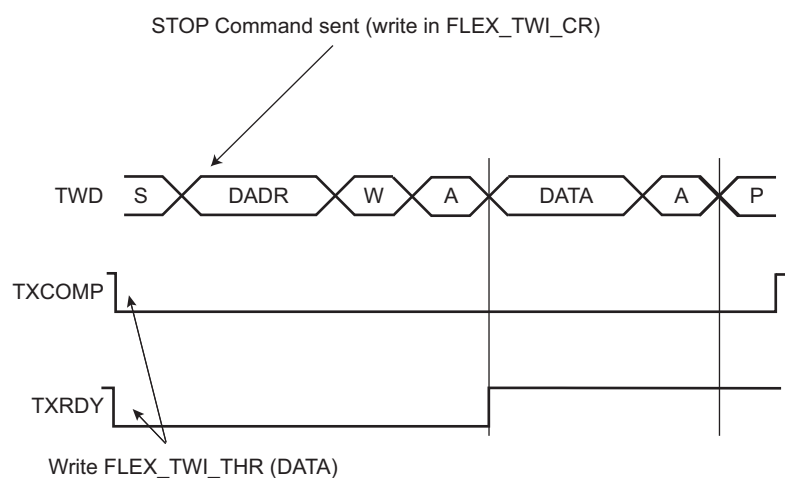
Figure 44-85. Master Write with One Data Byte
