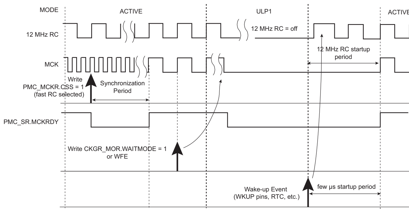
Figure 30-7. Fast Startup from ULP Mode 1
