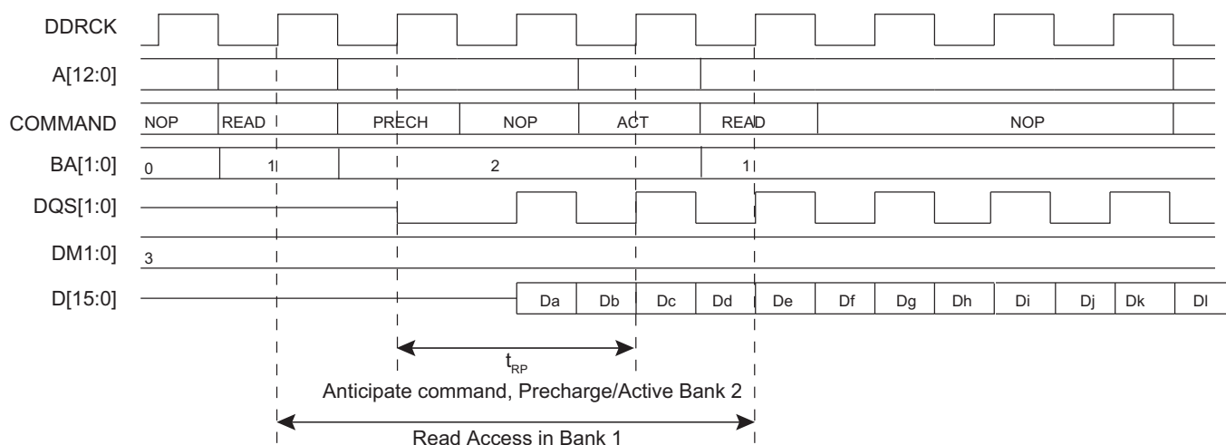
Figure 33-19. Anticipate Precharge/Activate Command in Bank 2 during Read Access in Bank 1
