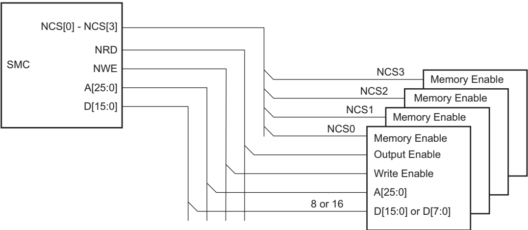
Figure 34-3. Memory Connections for External Devices
