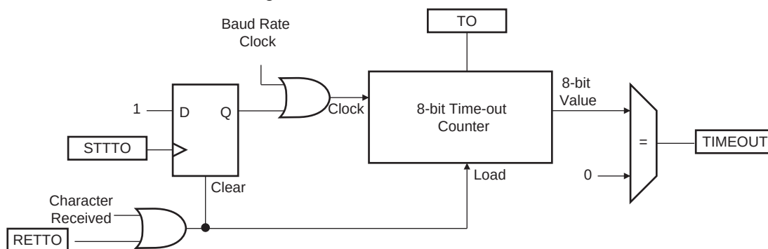
Figure 45-9. Receiver Time-out Block Diagram
