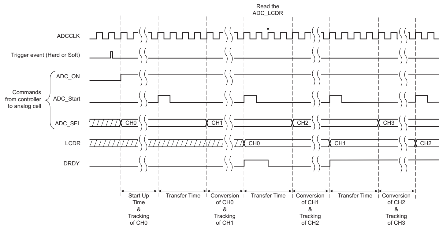
Figure 62-3. Sequence of ADC Conversions When Tracking Time < Conversion Time
