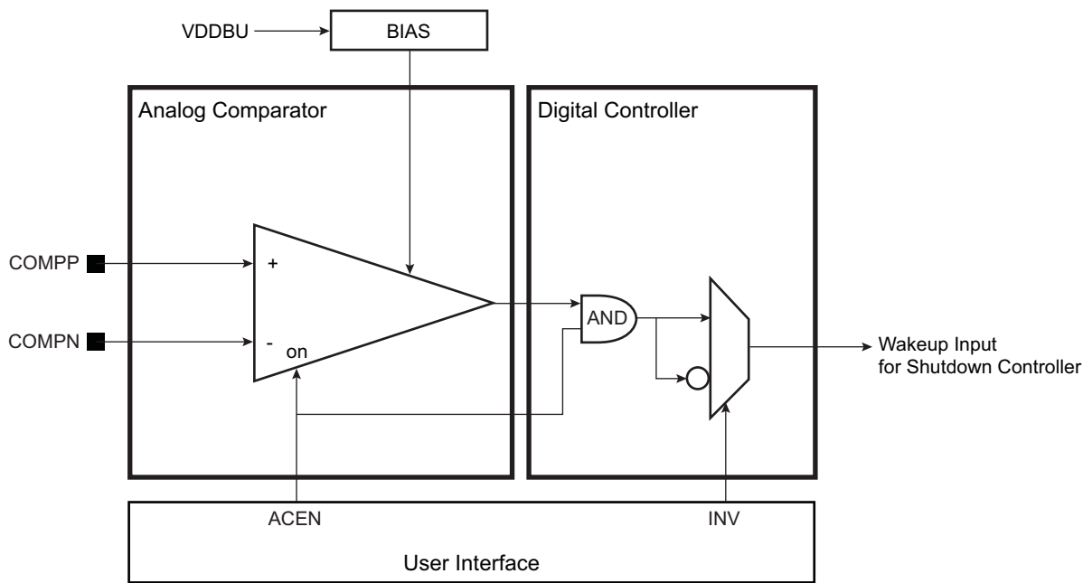
Figure 28-1. Analog Comparator Controller Block Diagram
