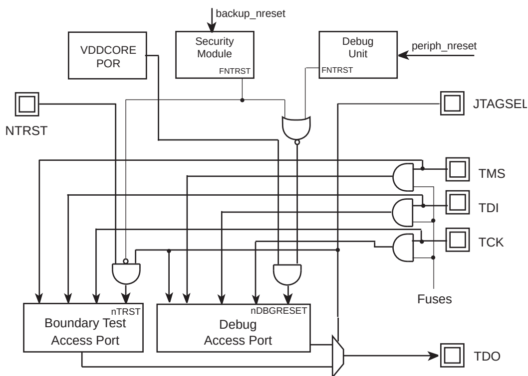
Figure 61-11. JTAG Protection Principle
