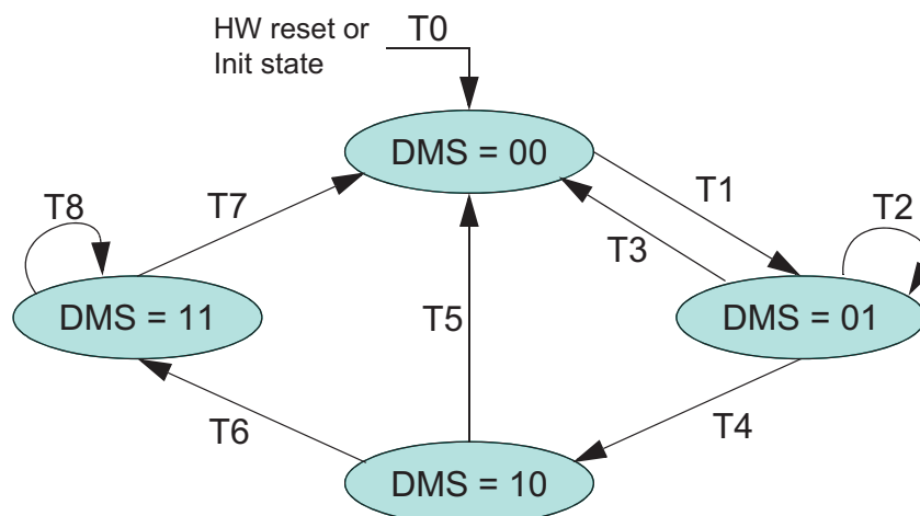
Figure 50-9. Debug Message Handling State Machine
