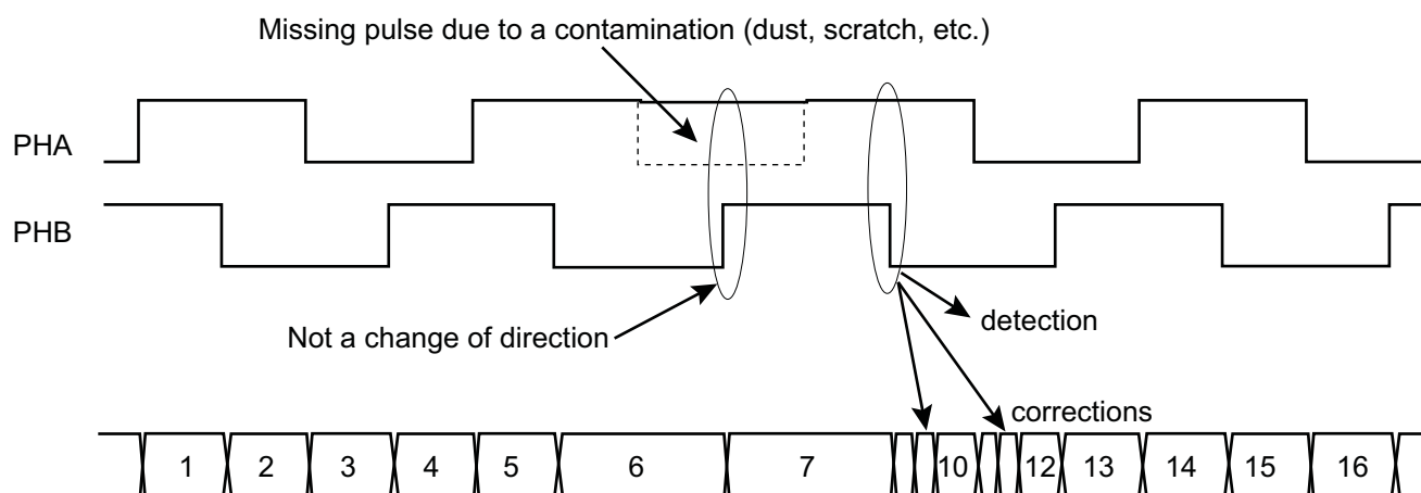
Figure 51-22. Detection and Auto-correction of Missing Pulses
