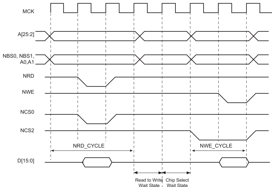
Figure 34-13. Chip Select Wait State between a Read Access on NCS0 and a Write Access on NCS2
