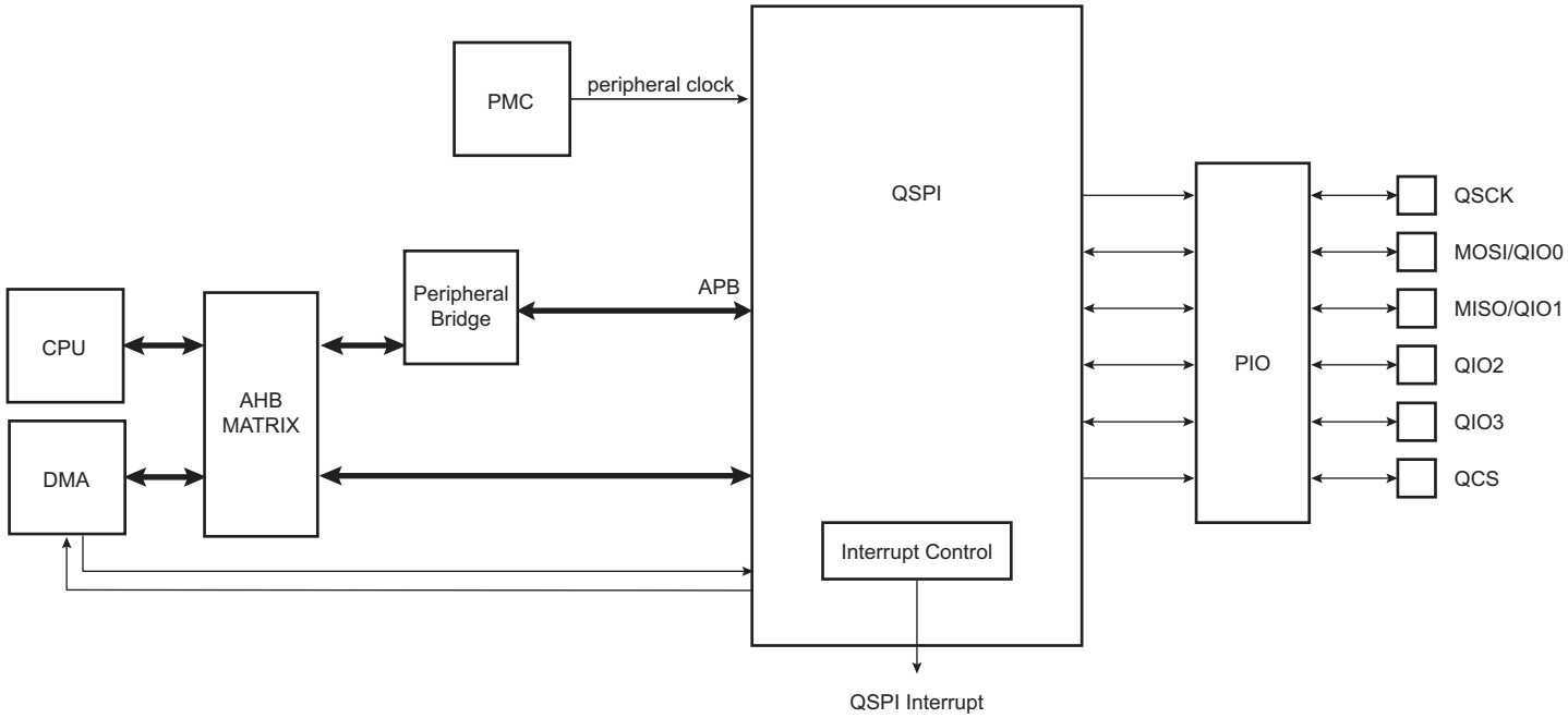
Figure 47-1. Block Diagram
