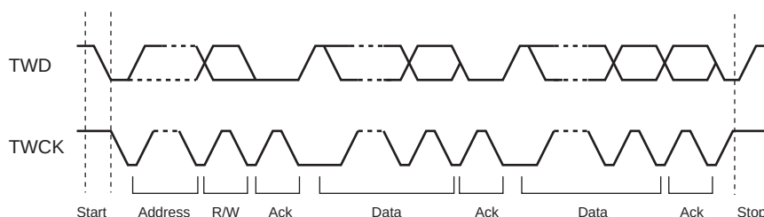
Figure 43-3. Transfer Format
