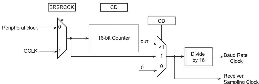
Figure 45-2. Baud Rate Generator
