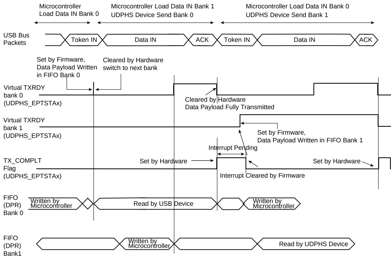
Figure 38-10. Data IN Transfer for Endpoint with Two Banks
