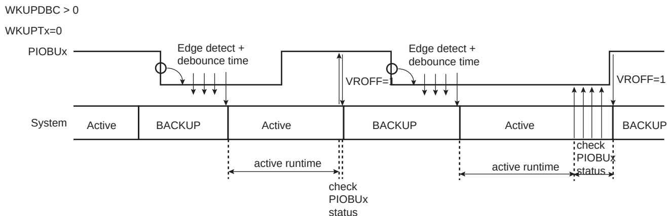
Figure 23-2. Entering and Exiting Backup Mode with a PIOBUX, WKUP Pin
