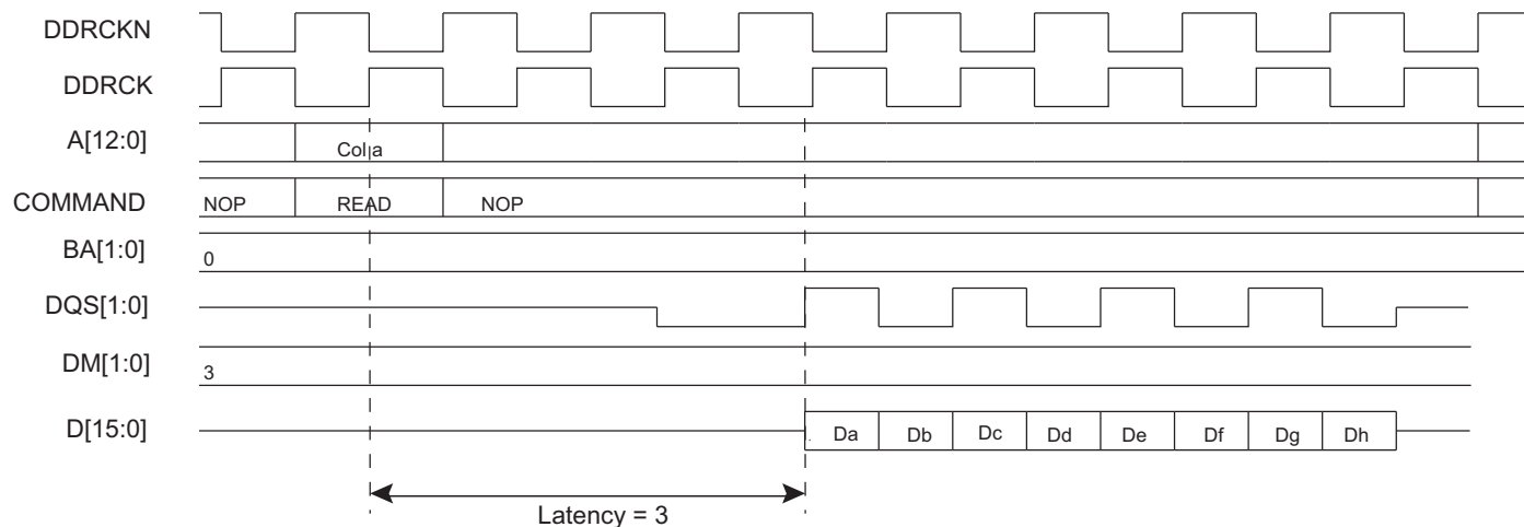
Figure 33-12. Burst Read Access, Latency = 3, DDR2-SDRAM Devices
