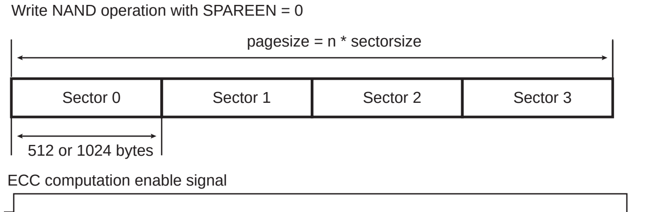
Figure 34-41. NAND Write Operation
