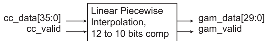
Figure 49-23. GAM Block Diagram
