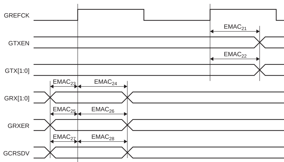
Figure 63-43. Ethernet MAC RMII Timings
