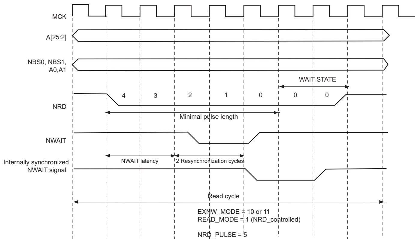
Figure 34-27. NWAIT Latency
