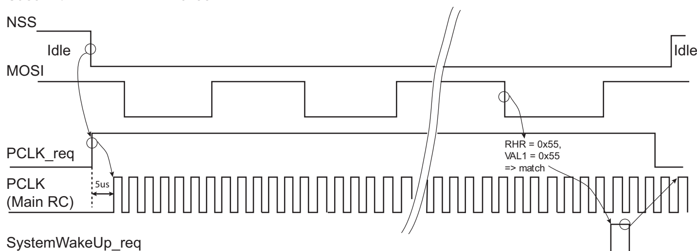
Figure 44-76. Asynchronous Wake-up Use Case Example
