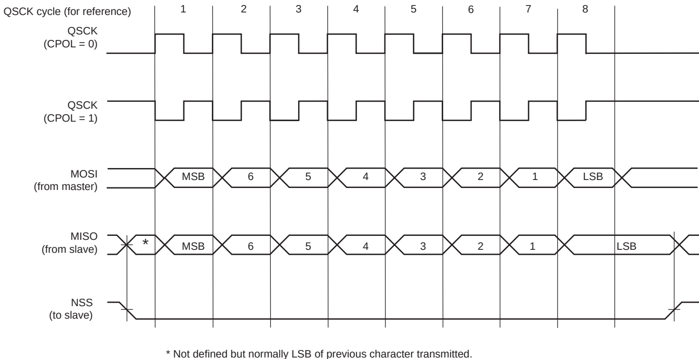
Figure 47-3. QSPI Transfer Format (QSPI_SCR.CPHA = 1, 8 bits per transfer)
