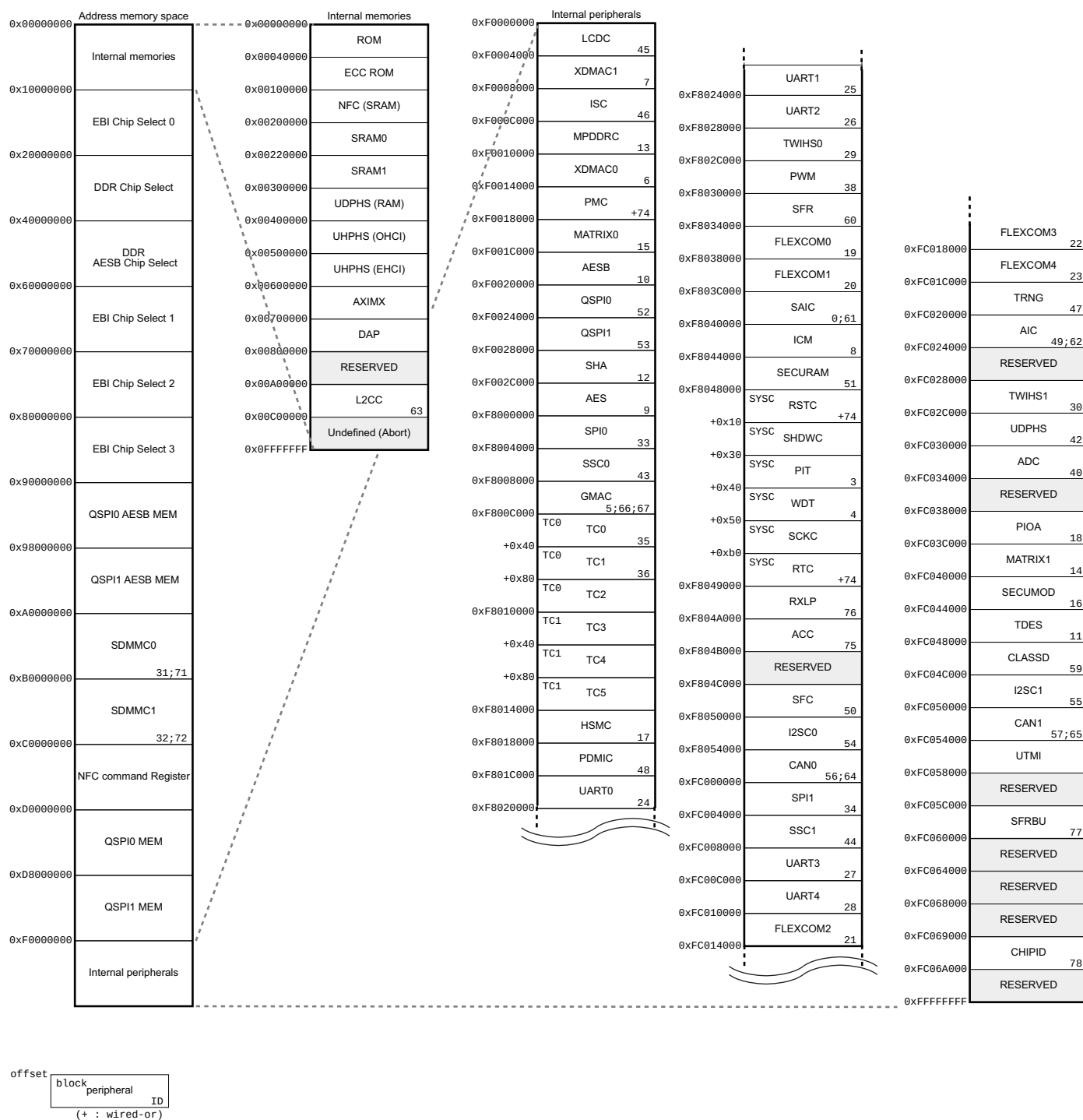
Figure 7-1. Memory Mapping
