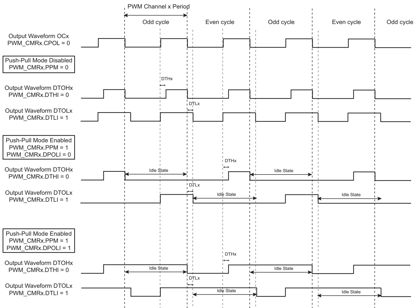
Figure 53-10. PWM Push-Pull Mode
