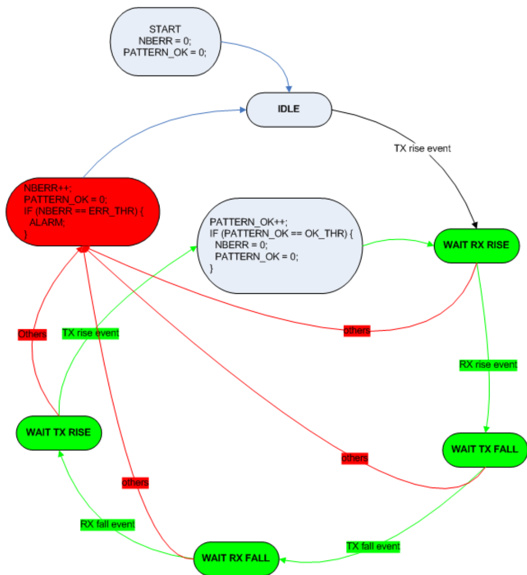
Figure 61-6. Dynamic Detection Mechanism State Machine
