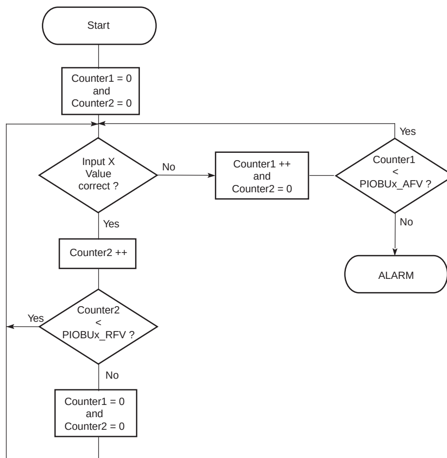
Figure 61-4. PIOBUx Alarm Filtering Principle
