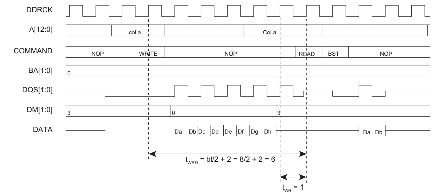
Figure 33-6. Write Command Followed by a Read Command without Burst Write Interrupt, DDR-SDRAM Devices
