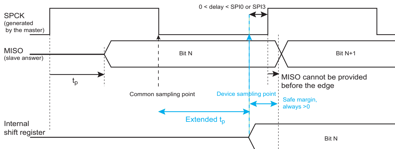
Figure 63-11. MISO Capture in Master Mode
