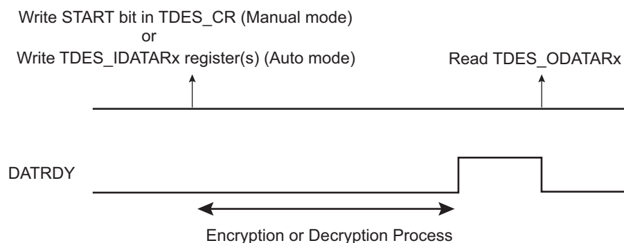
Figure 59-1. Manual and Auto Modes with LOD = 0
