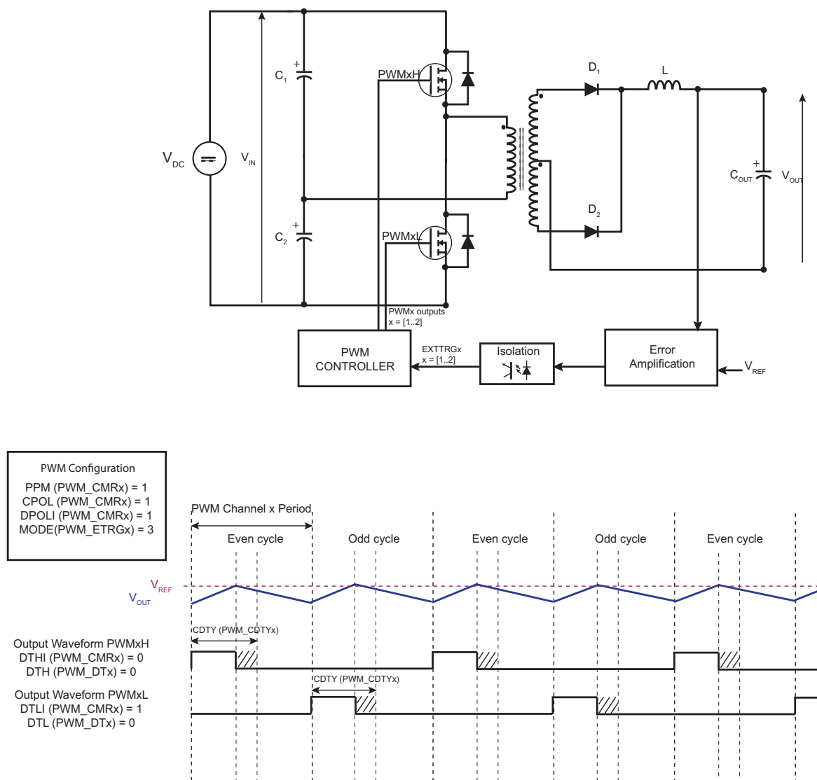
Figure 53-14. Half-Bridge Converter Application: Feedback Regulation
