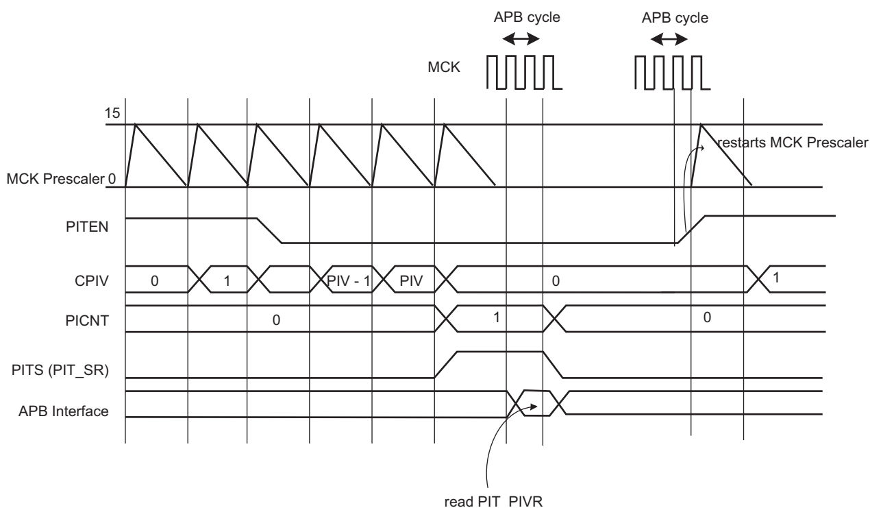
Figure 24-2. Enabling/Disabling PIT with PITEN
