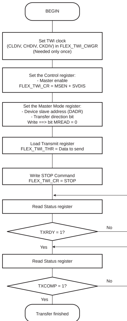
Figure 44-95. TWI Write Operation with Single Data Byte without Internal Address
