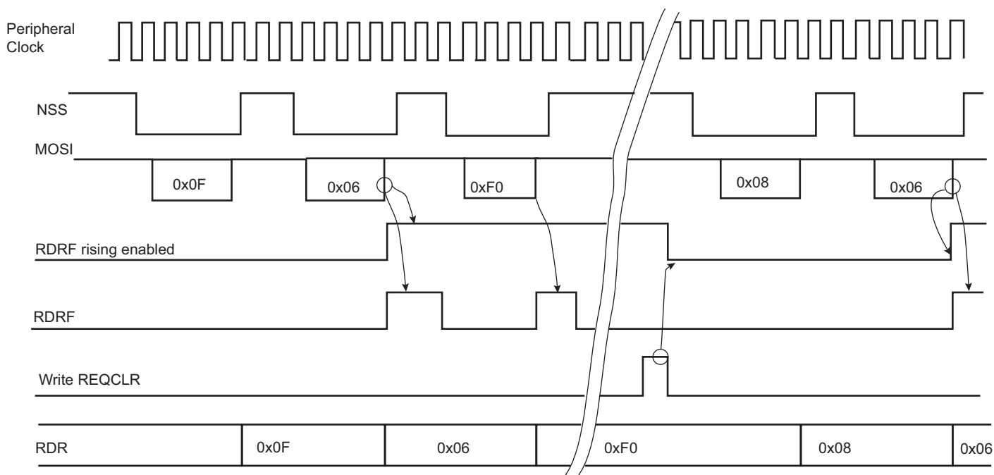
Figure 46-13. Receive Data Register Management
