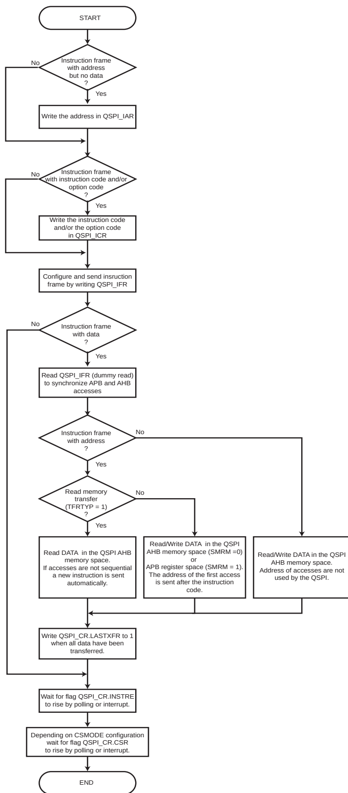
Figure 47-9. Instruction Transmission Flow Diagram
