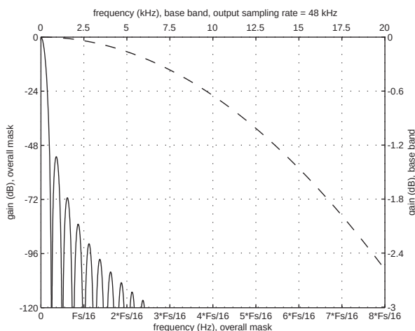
Figure 52-4. Spectral Mask of an OSR = 64 , F_s = 3.072 MHz, Fourth-order Sinc Filter: Overall Response (continuous line) and 0 to 20 kHz Bandwidth Response (dashed line)
