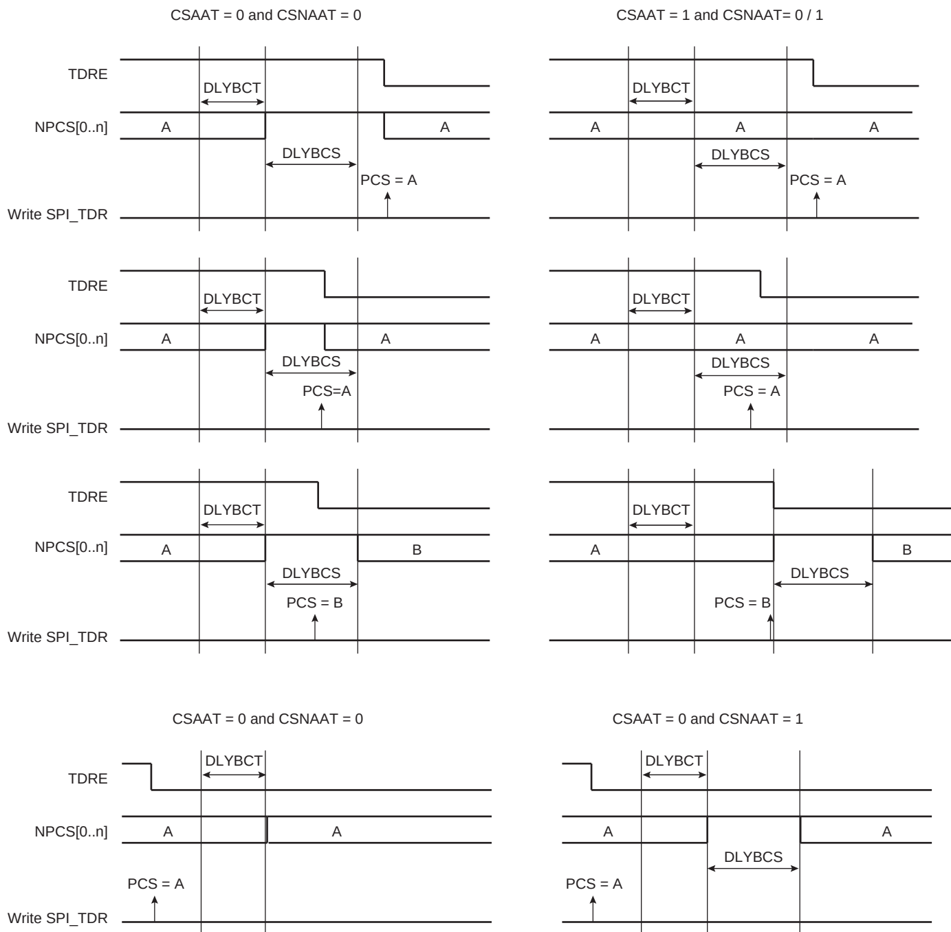
Figure 46-11. Peripheral Deselection
