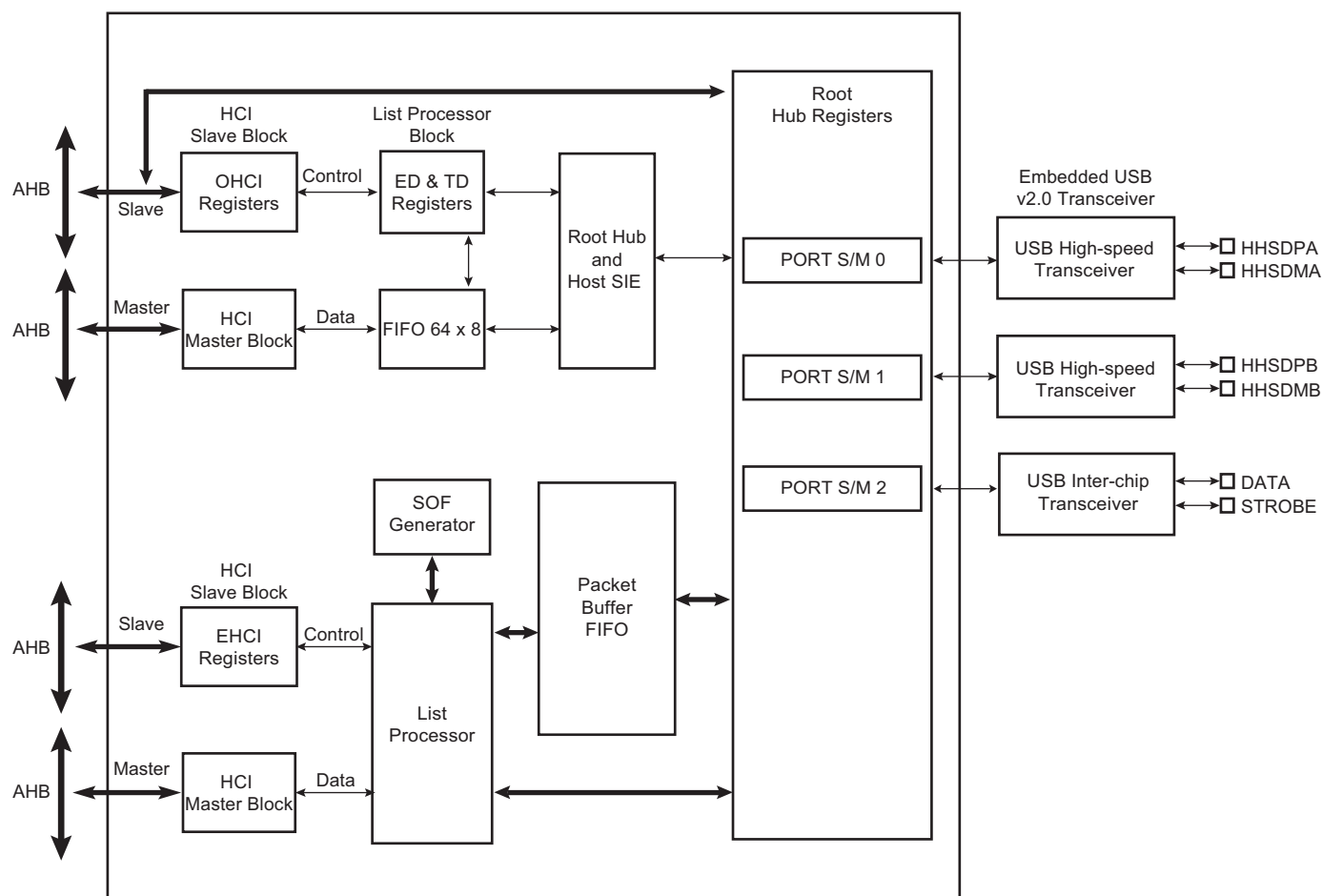
Figure 39-1. Block Diagram
