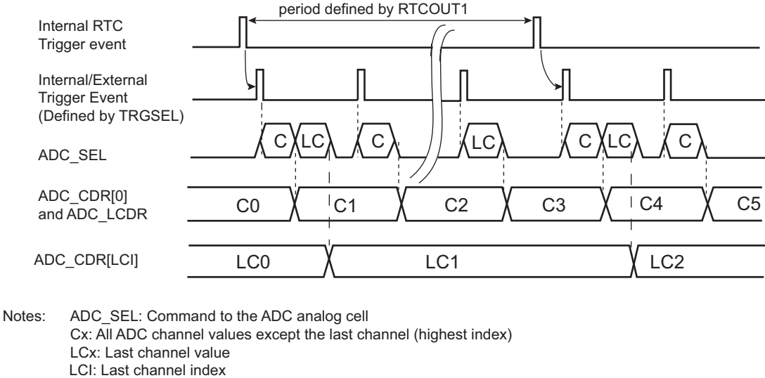
Figure 62-9. Independent Trigger Measurement for Last Channel (ADC_CHSR[LCI] = 0 and ADC_TRGR.TRGMOD = 1, 2, 3, 5) ADC_LCTMR.DUALTRIG = 1
