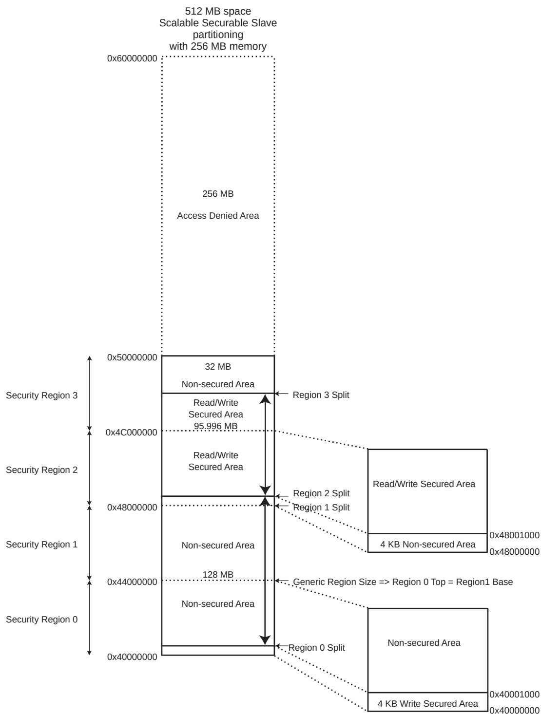
Figure 17-4. Partitioning Example of a Scalable Securable Slave Featuring 4 Equally-sized Security Regions of 1 MB to 128 MB each and up to 8 Security Areas of 4 KB to 128 MB
