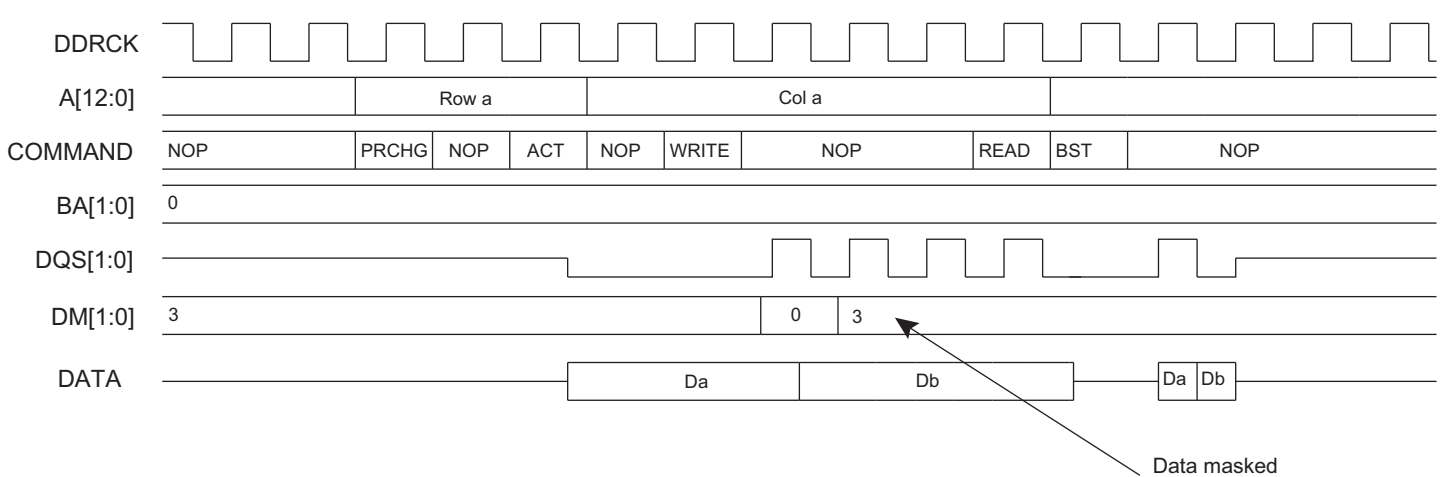
Figure 33-7. SINGLE Write Access Followed by a Read Access, DDR-SDRAM Devices
