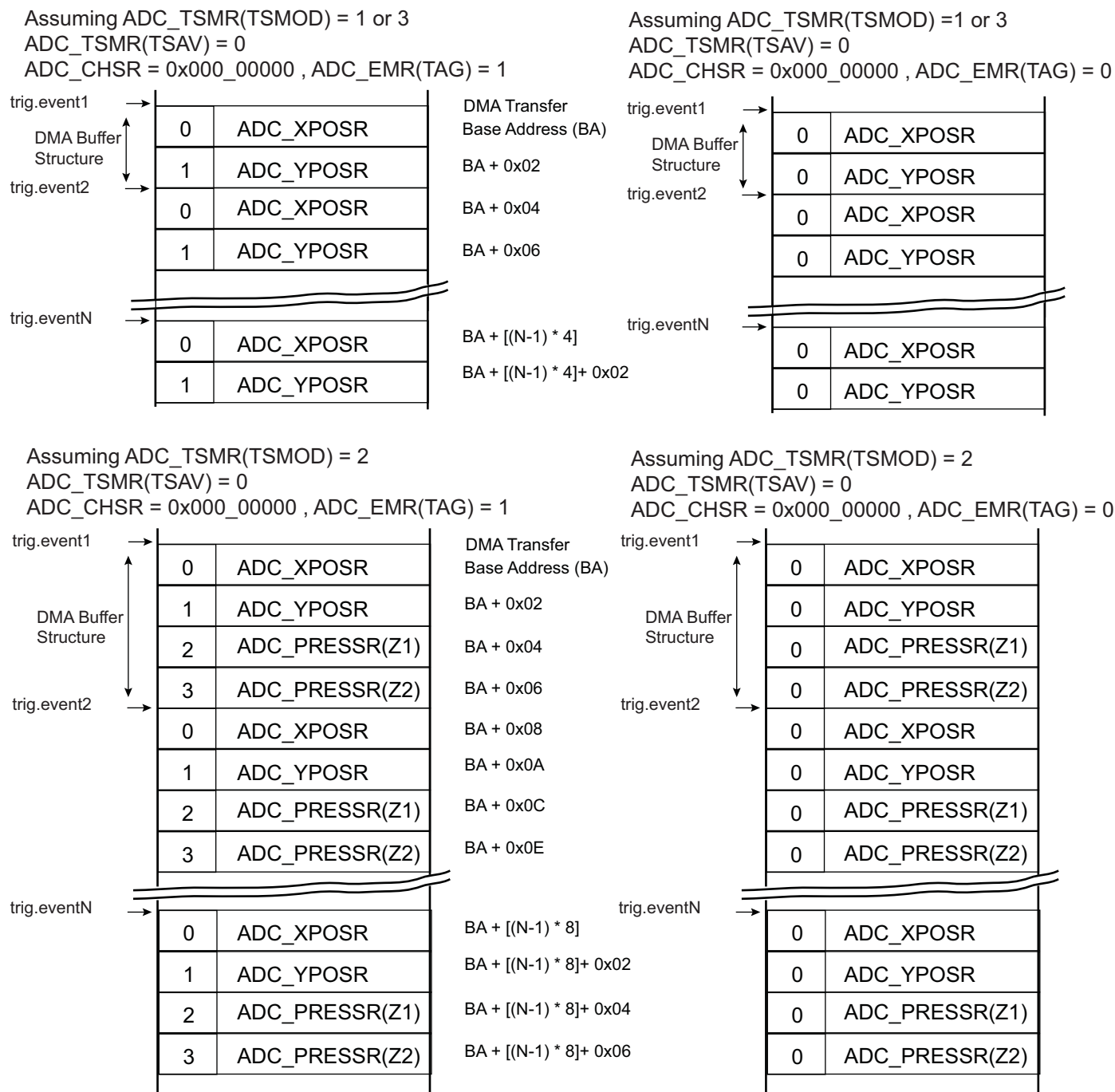
Figure 62-22. Buffer Structure When Only Touchscreen Channels are Enabled
