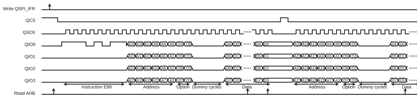
Figure 47-17. Instruction Transmission Waveform 7
