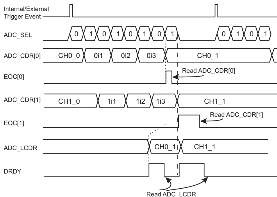
Figure 62-12. Digital Averaging Function Waveforms on a Single Trigger Event
