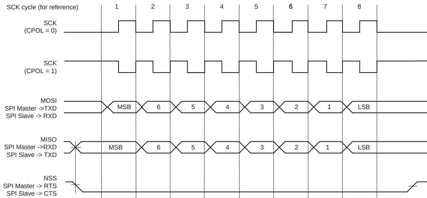
Figure 44-39. SPI Transfer Format (CPHA = 1, 8 bits per transfer)
