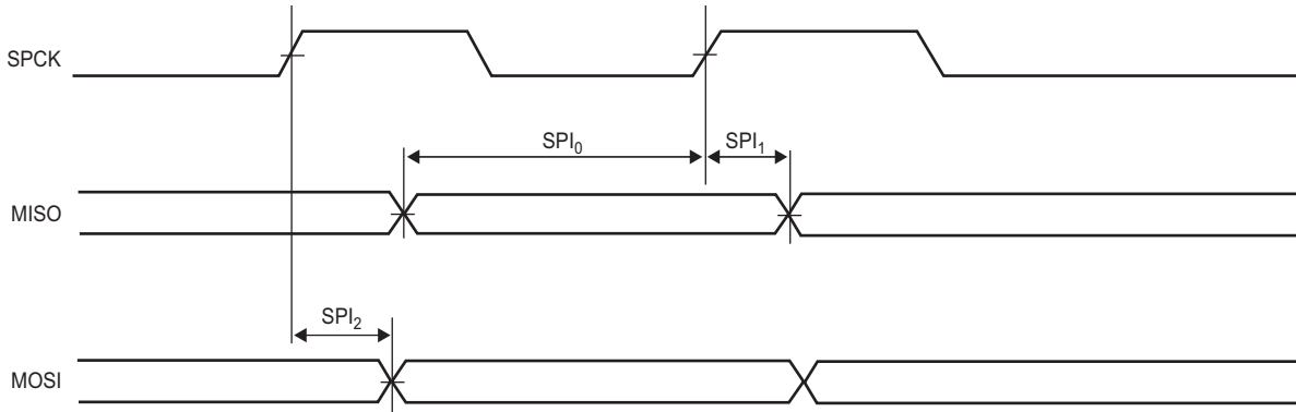
Figure 63-18. FLEXCOM in SPI Master Modes 1 and 2
