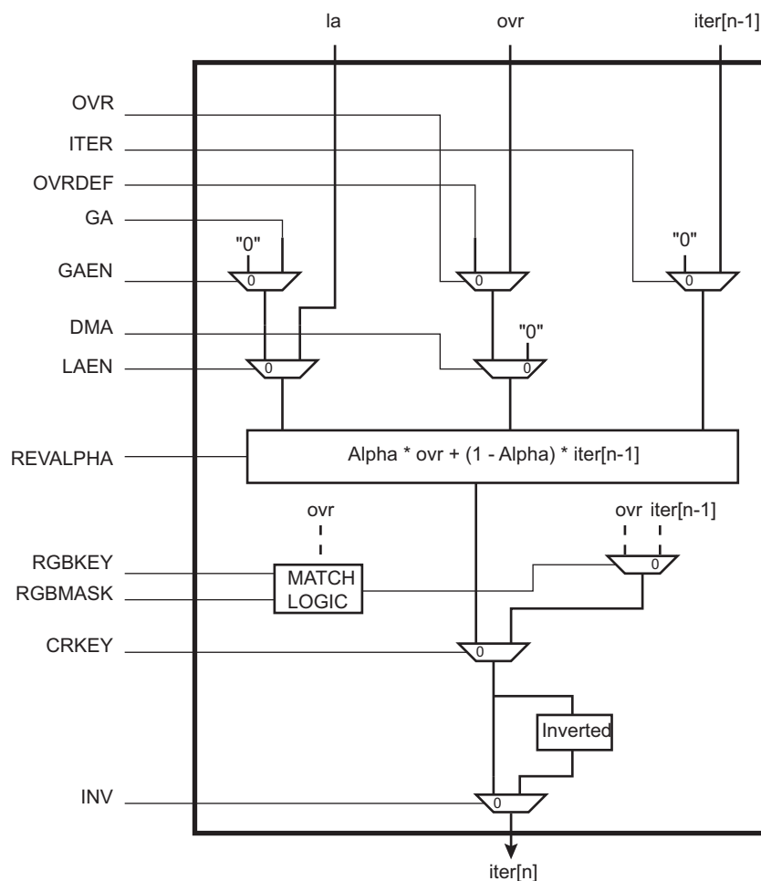
Figure 36-12. Alpha Blender Database
