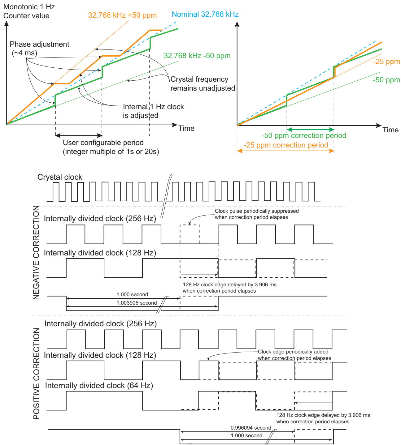
Figure 25-5. Calibration Circuitry Waveforms
