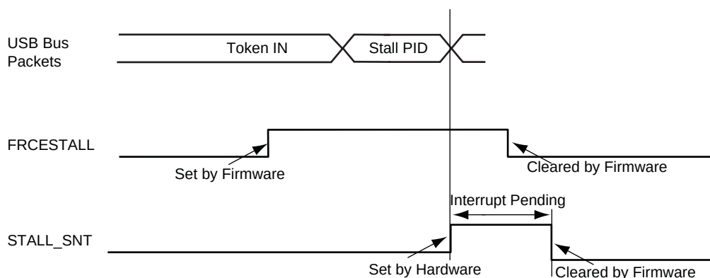
Figure 38-18. Stall Handshake Data IN Transfer
