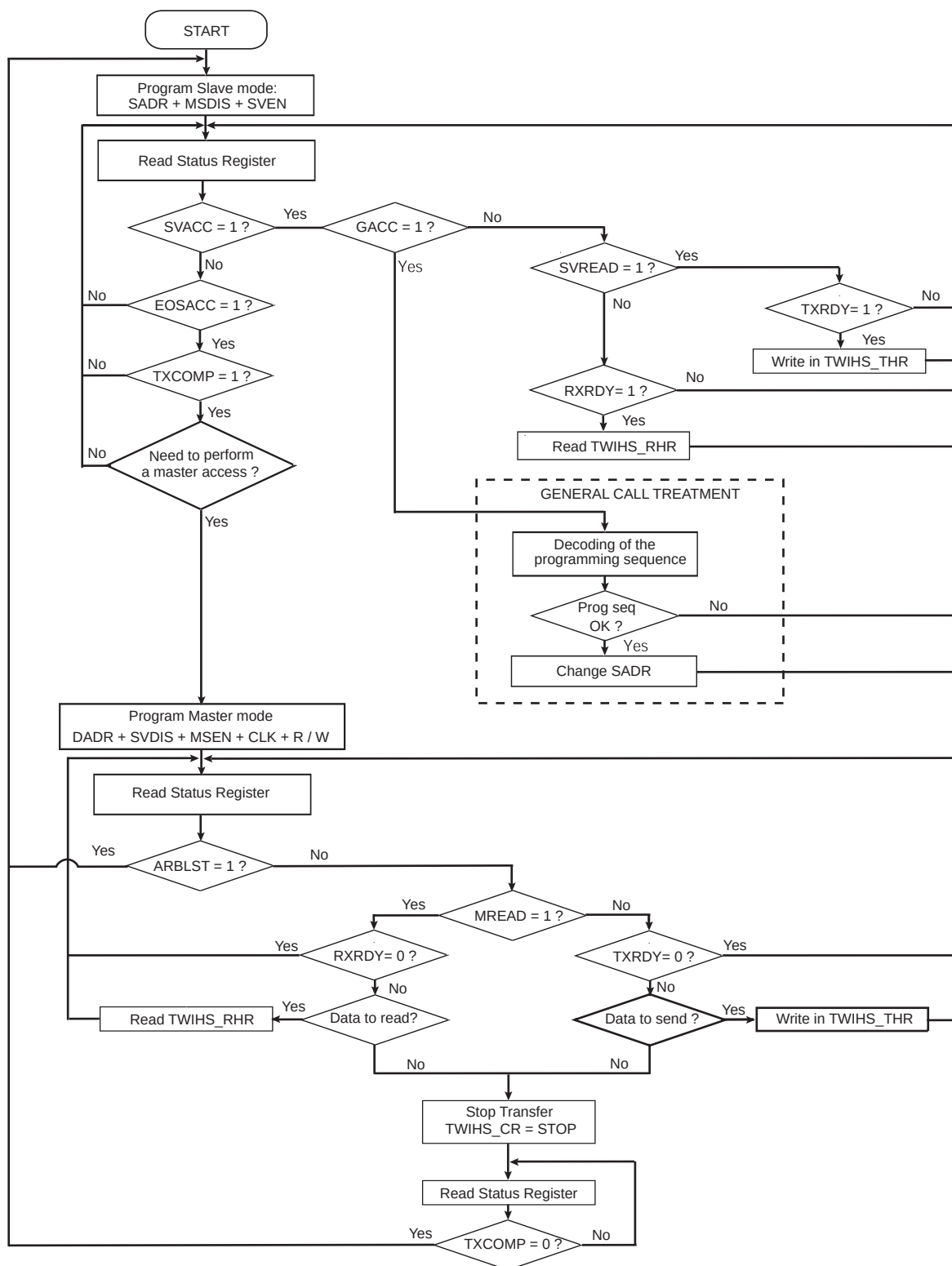
Figure 43-35. Multi-master Flowchart
