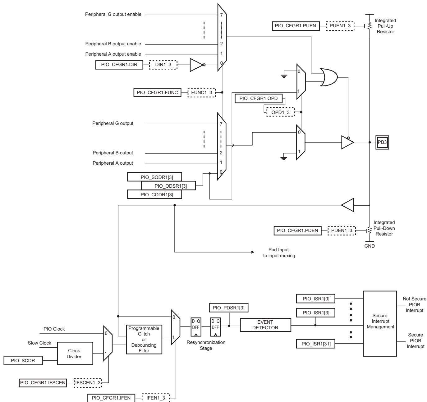
Figure 31-2. I/O Line Control Logic
