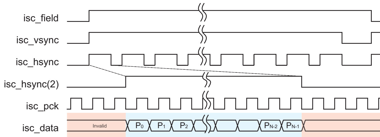
Figure 49-10. Free-Running Pixel Clock
