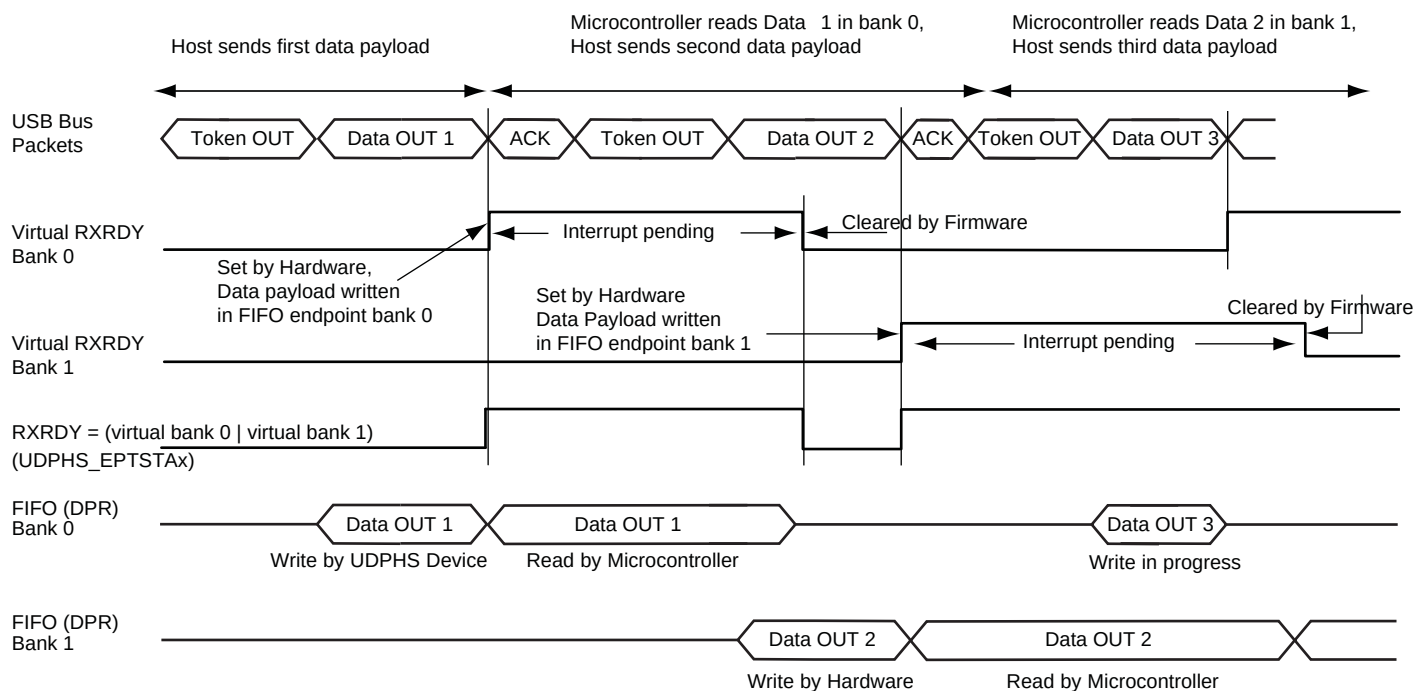
Figure 38-15. Data OUT Transfer for an Endpoint with Two Banks
