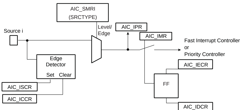
Figure 20-4. Internal Interrupt Source Input Stage
