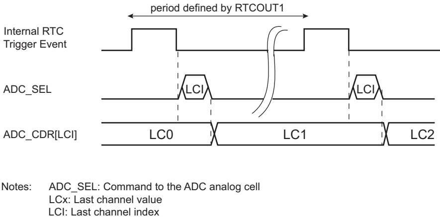
Figure 62-10. Only Last Channel Measurement Triggered at Low Speed (ADC_CHSR[LCI] = 0 and ADC_TRGR.TRGMOD = 0) ADC_LCTMR.DUALTRIG = 1
