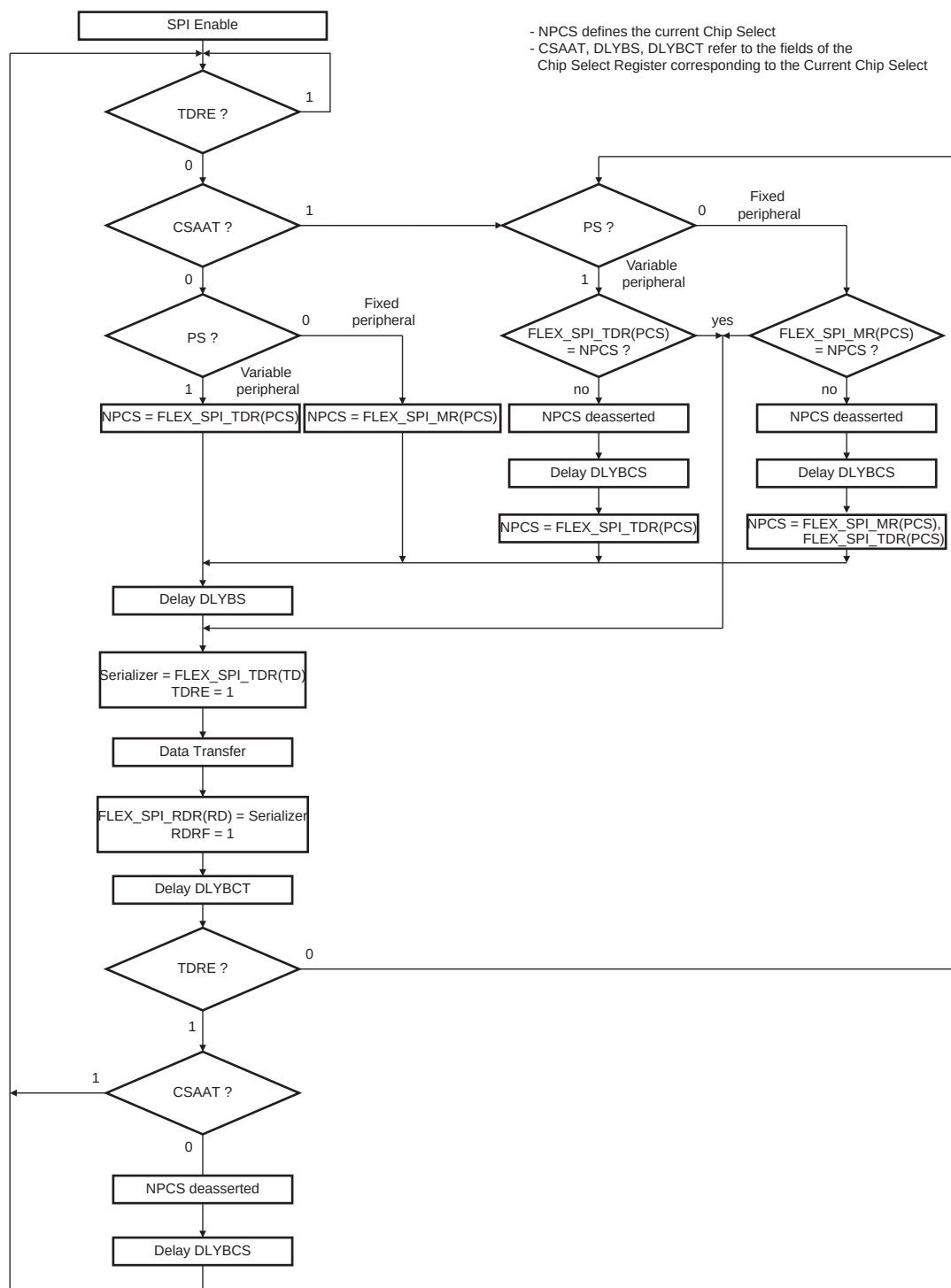
Figure 44-69. Master Mode Flow Diagram
