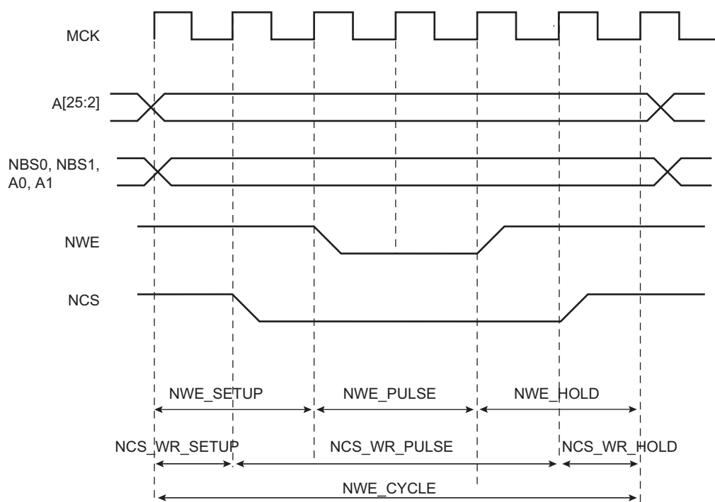
Figure 34-10. Write Cycle
