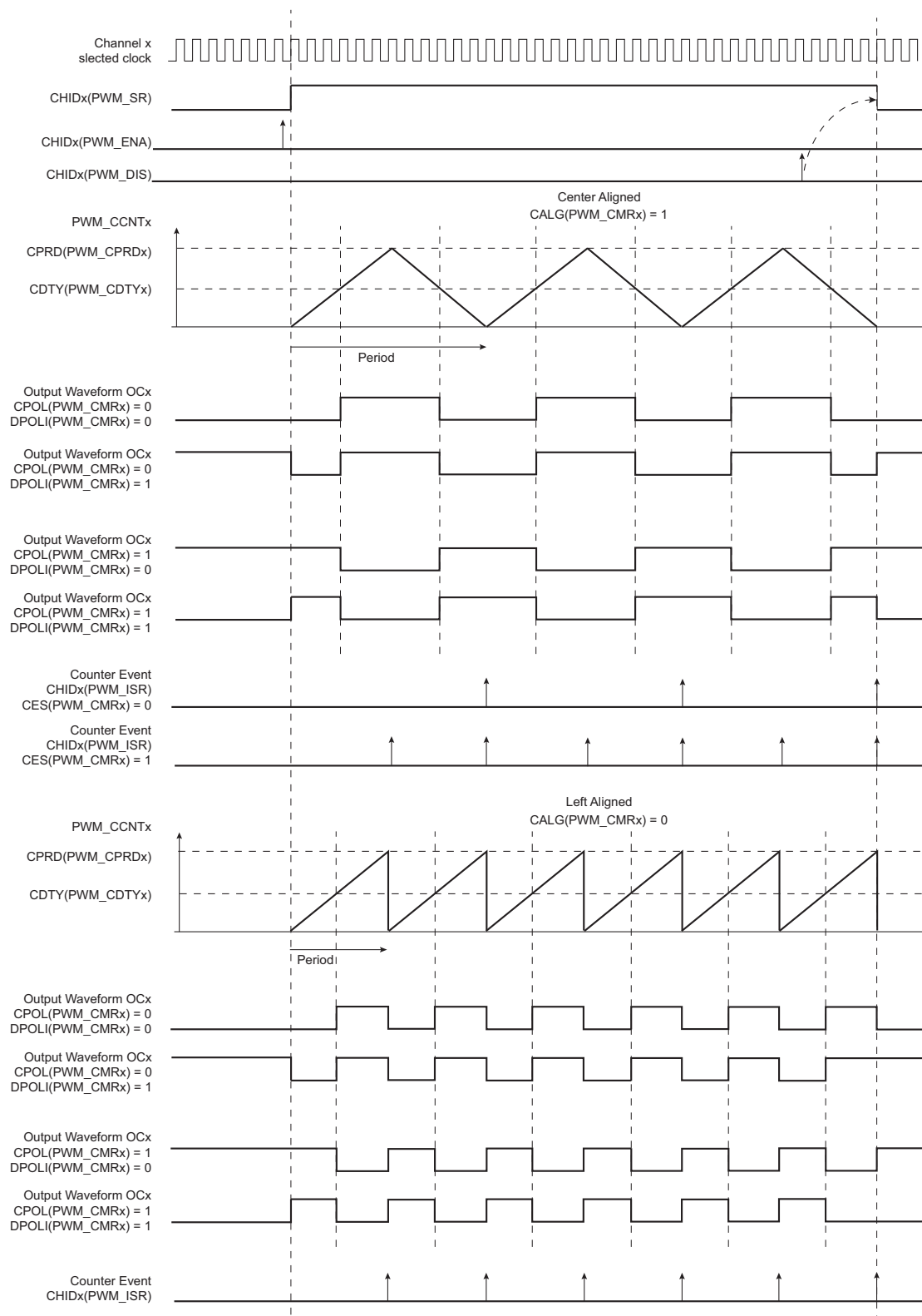
Figure 53-5. Waveform Properties
