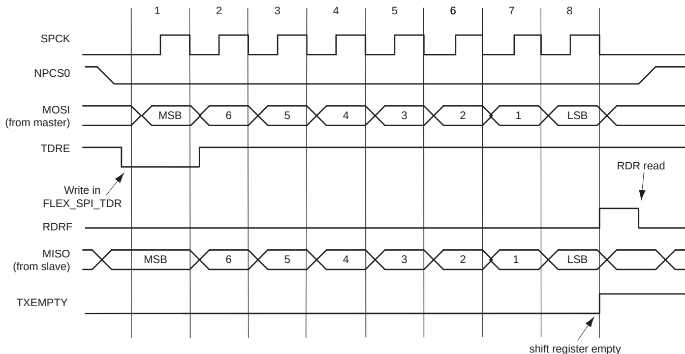
Figure 44-70. Status Register Flags Behavior
