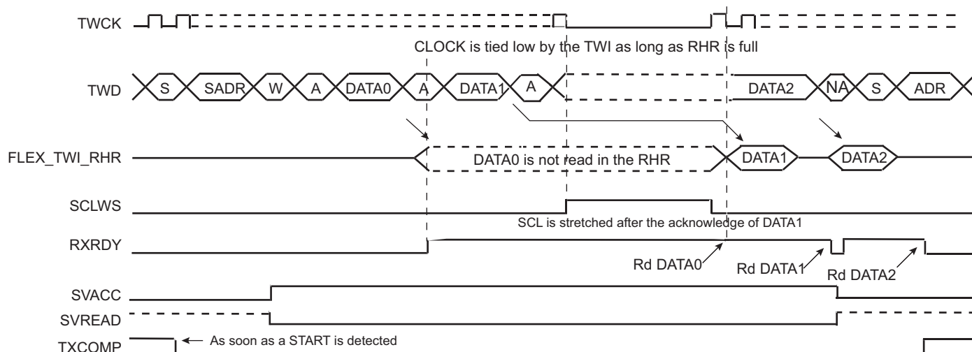
Figure 44-122. Clock Stretching in Write Mode
