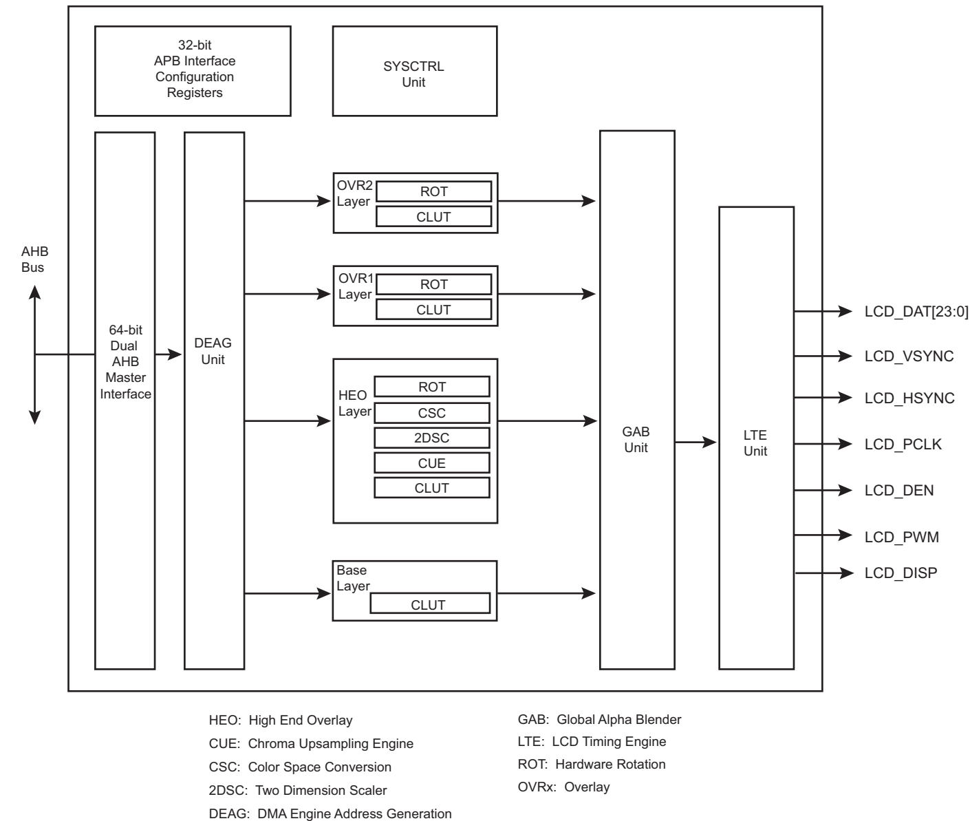
Figure 36-1. Block Diagram
