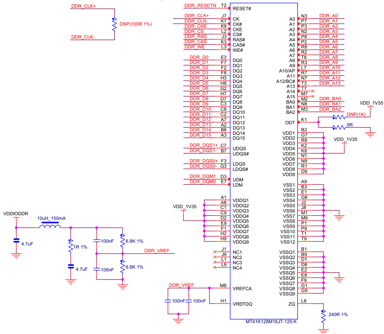
Figure 32-5. 16-bit DDR3/DDR3L Hardware Configuration
