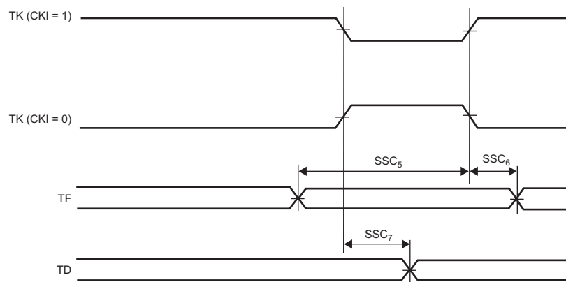
Figure 63-33. SSC Transmitter, TK and TF in Input
