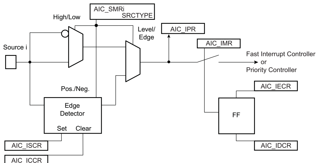
Figure 20-5. External Interrupt Source Input Stage
