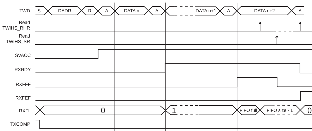
Figure 43-54. RXRDY in Single Data Mode and RXRDYM = 0x0
