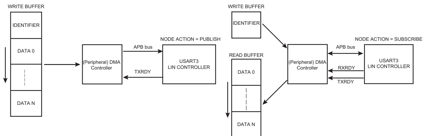
Figure 44-54. Master Node with DMAC (PDCM = 0)
