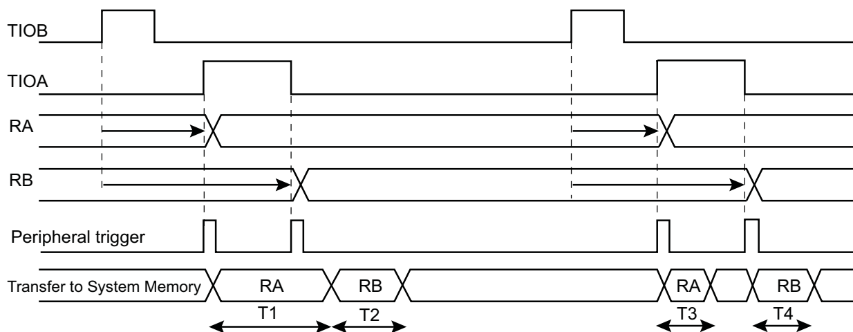
Figure 51-5. Example of Transfer with DMAC
