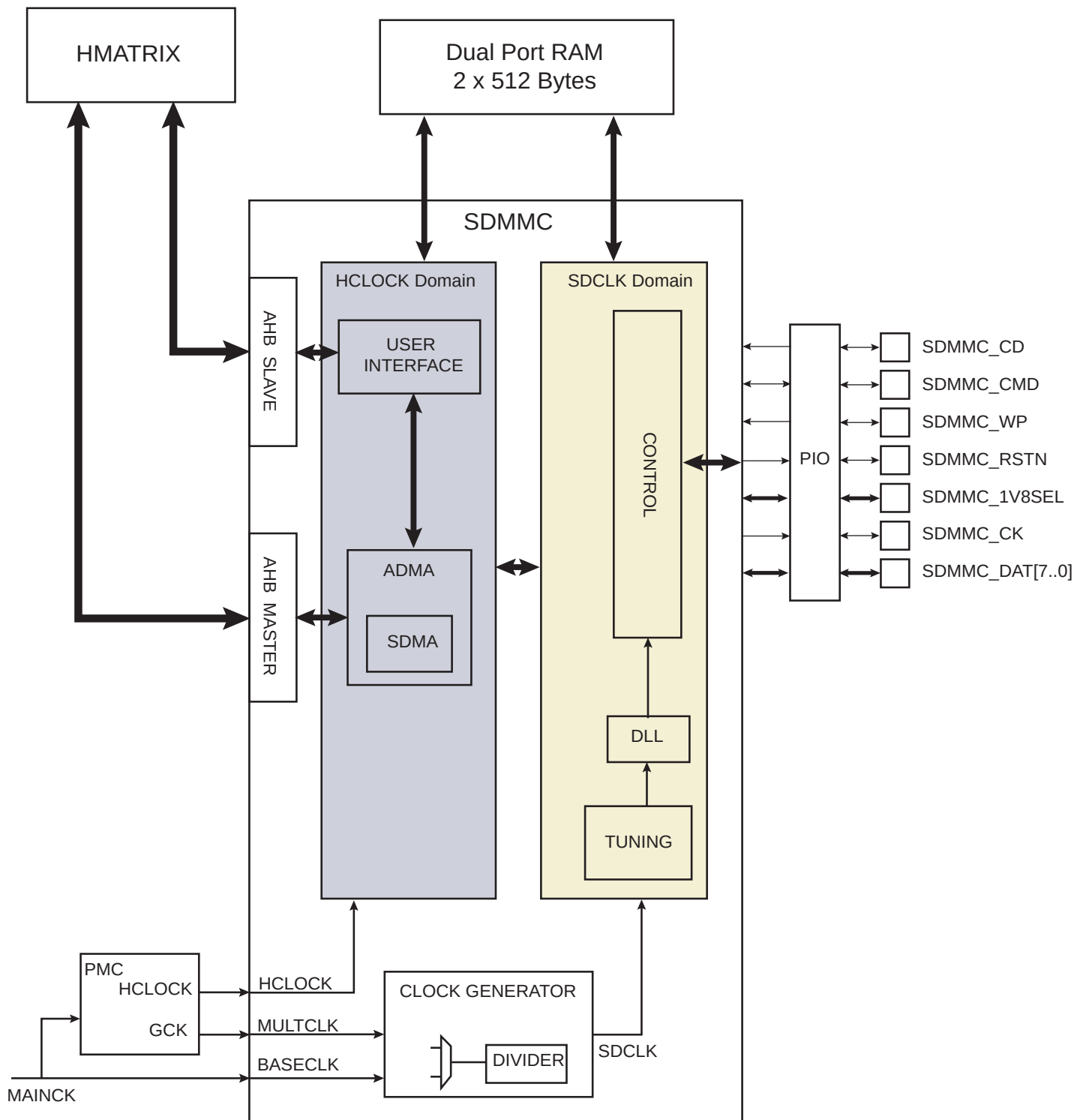
Figure 48-1. Block Diagram
