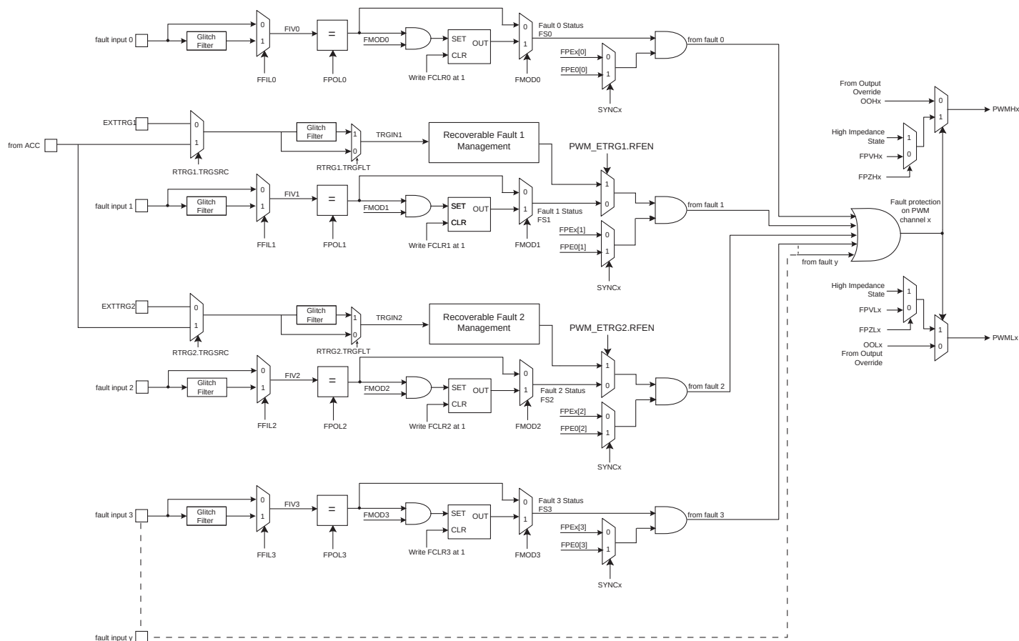
Figure 53-16. Fault Protection
