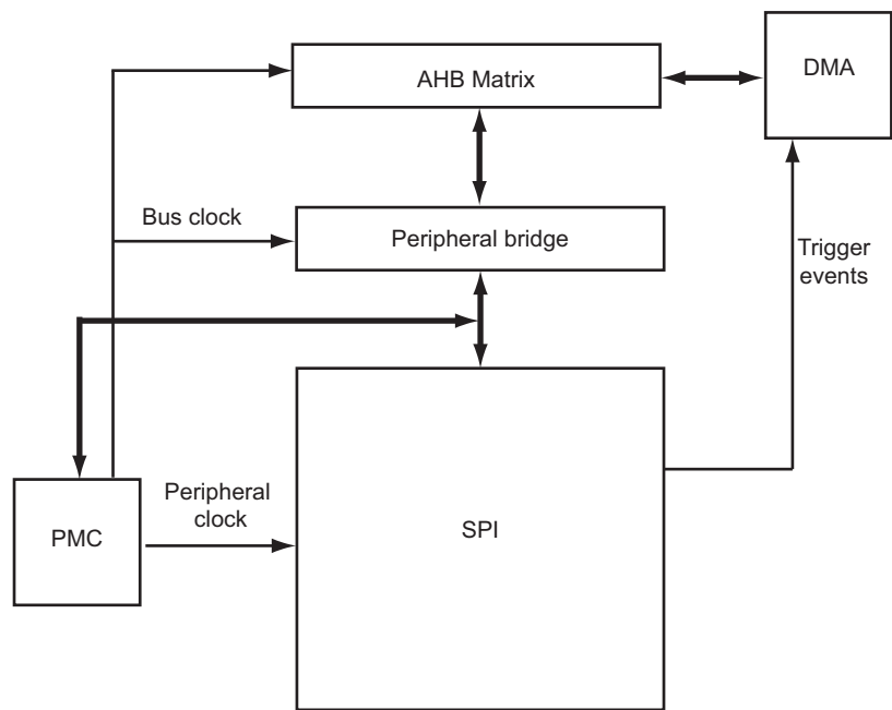
Figure 46-1. Block Diagram
