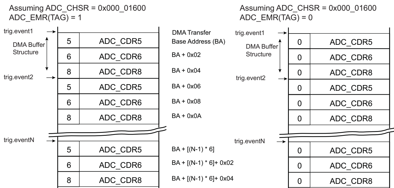
Figure 62-21. Buffer Structure
