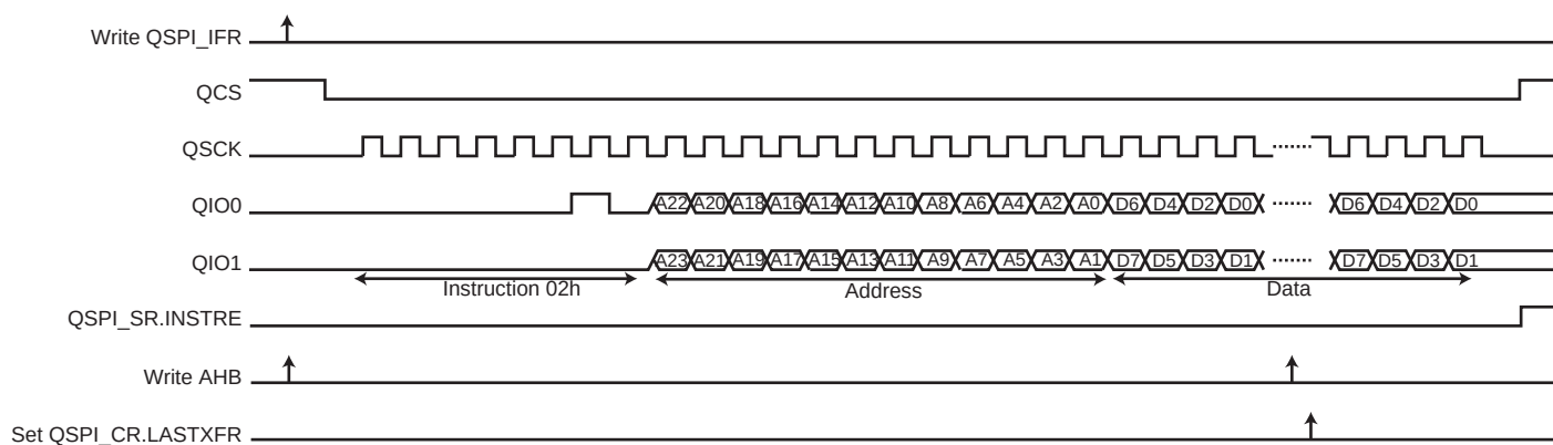
Figure 47-15. Instruction Transmission Waveform 5
