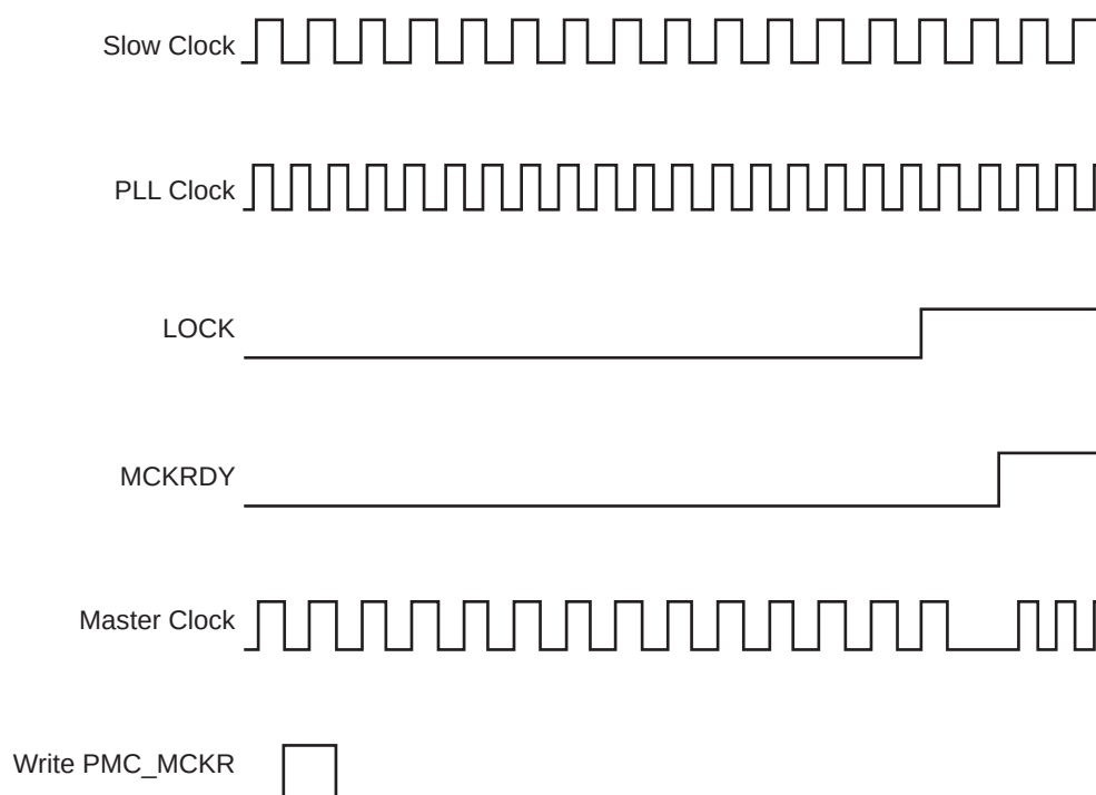
Figure 30-12. Switch Master Clock from Slow Clock to PLL Clock
