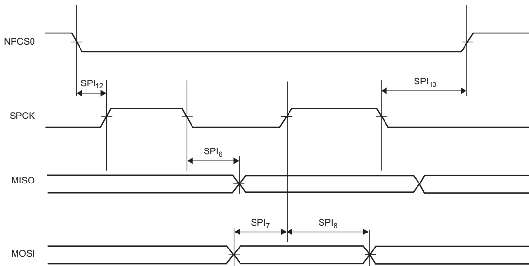
Figure 63-20. FLEXCOM in SPI Slave Modes 0 and 3
