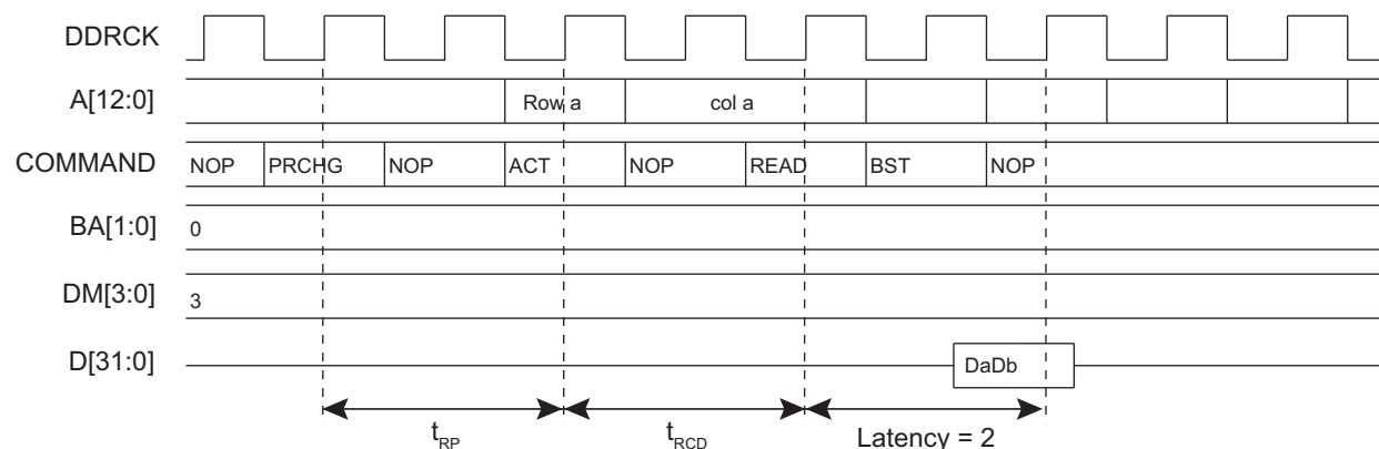
Figure 33-9. Single Read Access, Row Closed, Latency = 2, DDR-SDRAM Devices
