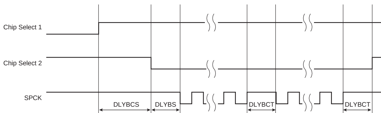
Figure 46-9. Programmable Delays
