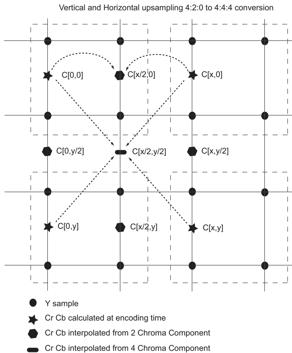
Figure 36-5. 4:2:0 Upsampling Algorithm
