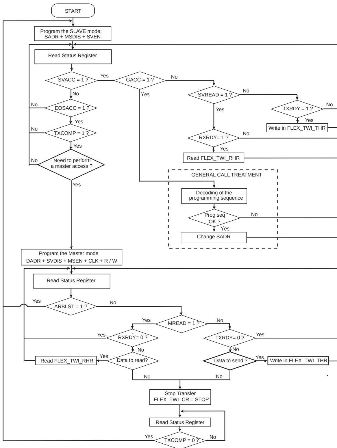
Figure 44-117. Multi-Master Flowchart
