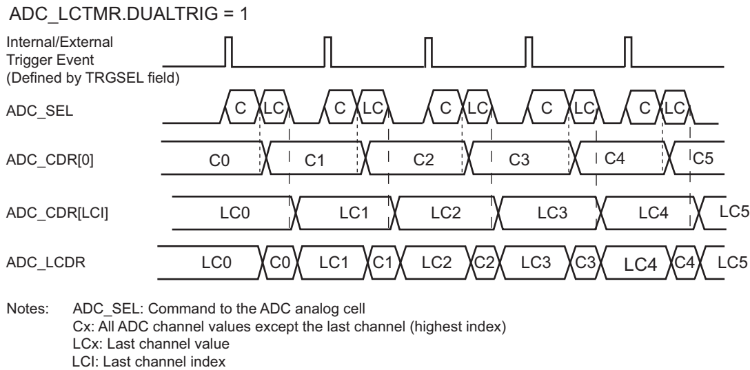
Figure 62-8. Same Trigger for All Channels (ADC_CHSR[LCI] = 1 and ADC_TRGR.TRGMOD = 1, 2, 3, 5)
