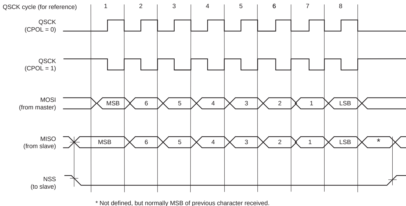
Figure 47-2. QSPI Transfer Format (QSPI_SCR.CPHA = 0, 8 bits per transfer)
