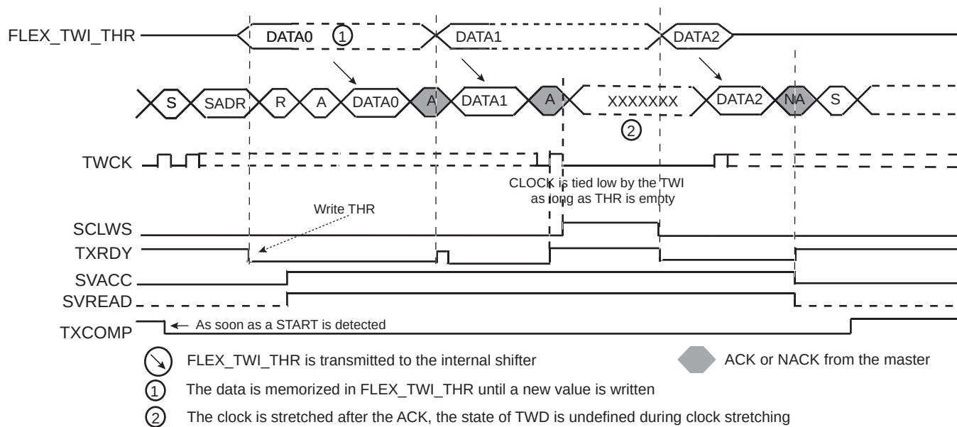
Figure 44-121. Clock Stretching in Read Mode
