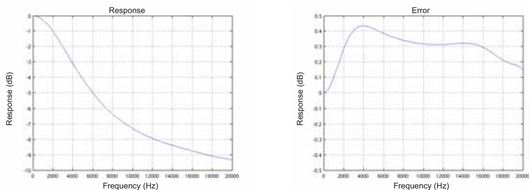
Figure 40-10. De-emphasis Filter: Frequency Response & Error ( f_s = 48 kHz)
