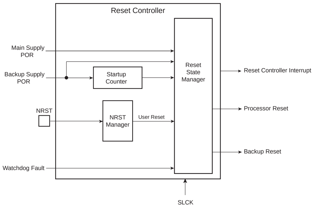
Figure 22-1. Reset Controller Block Diagram
