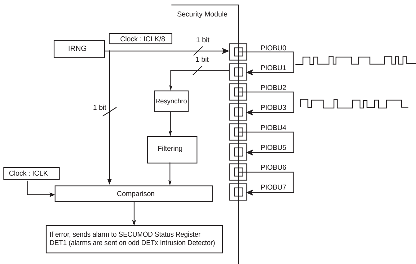
Figure 61-5. Dynamic Detection System
