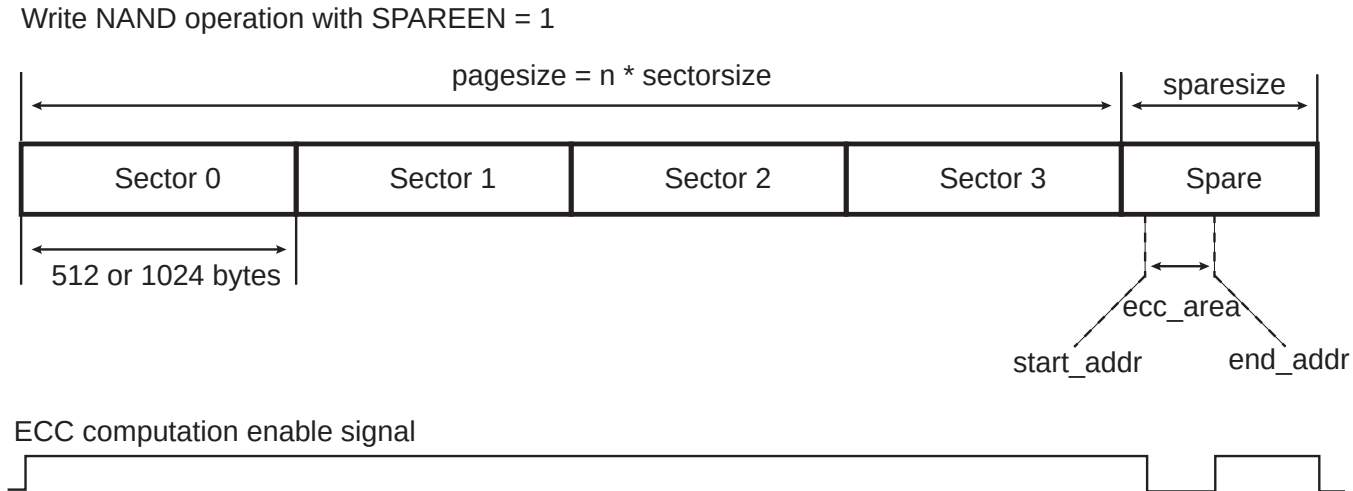
Figure 34-40. NAND Write Operation with Spare Encoding
