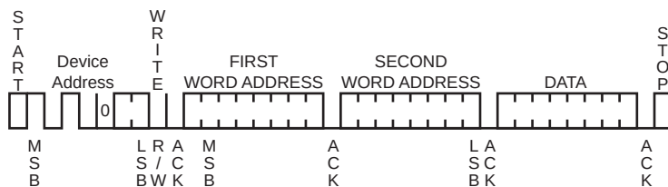
Figure 44-93. Internal Address Usage
