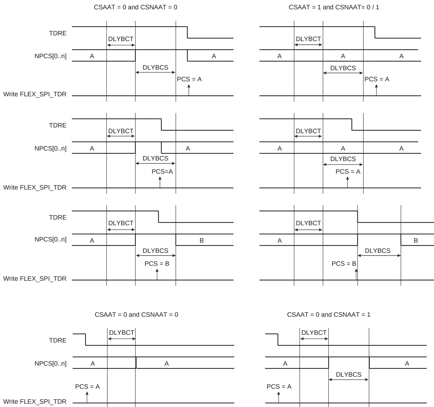
Figure 44-73. Peripheral Deselection
