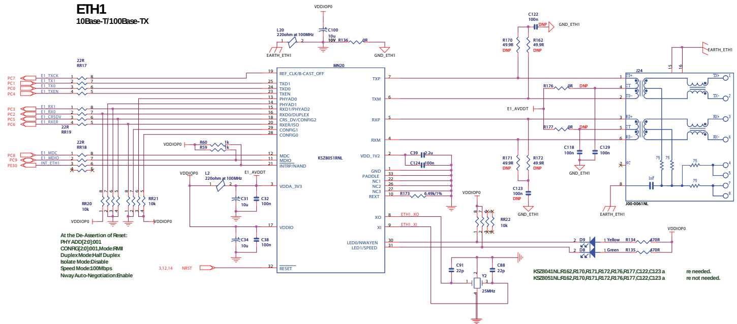
Figure 5-11. ETH1 Port
