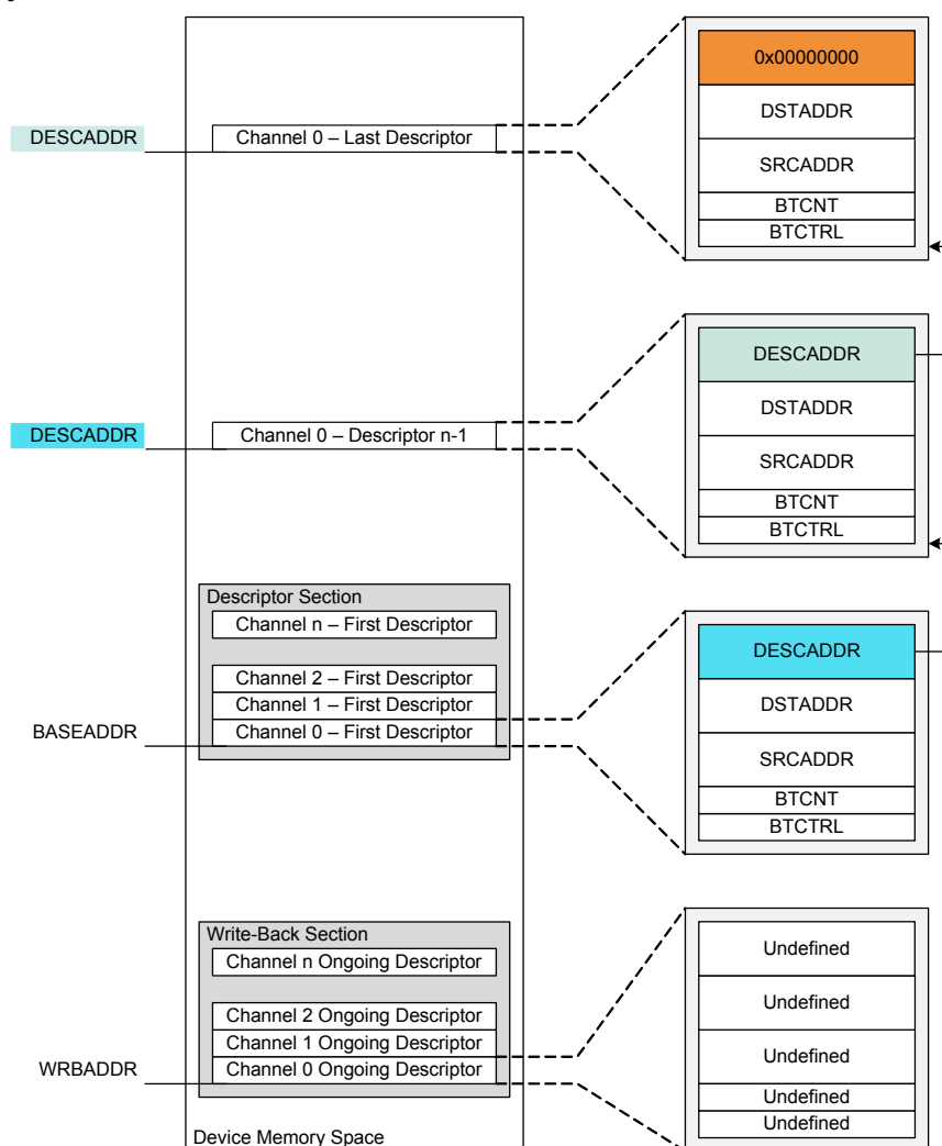
Figure 19-3. Memory Sections
