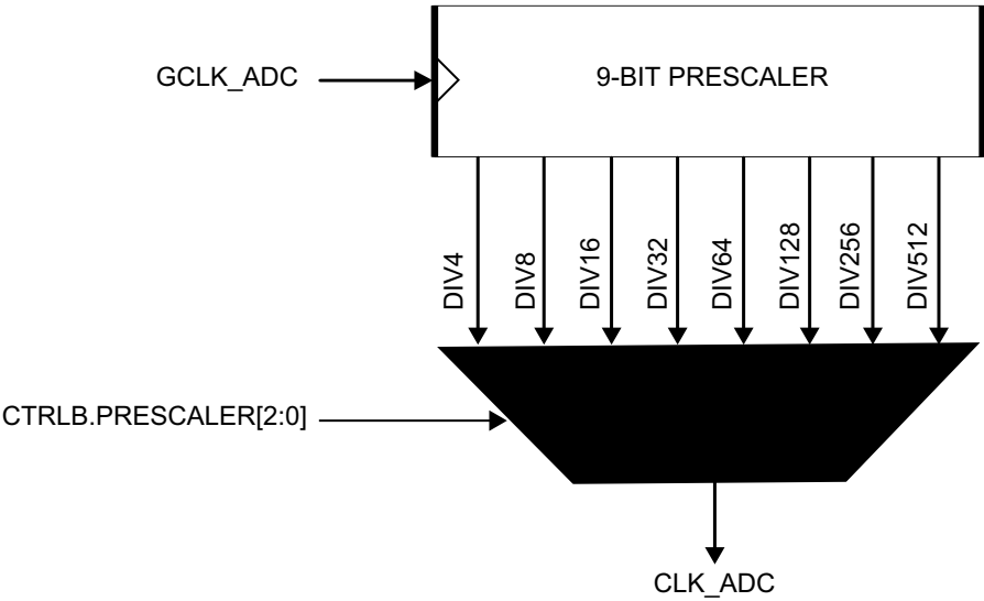
Figure 29-2. ADC Prescaler
