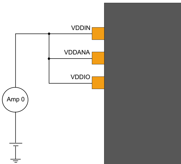
Figure 39-1. Measurement Schematic
