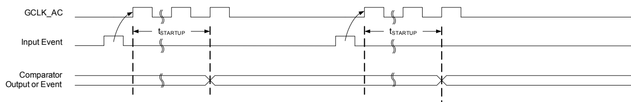
Figure 31-10. Single-Shot SleepWalking
