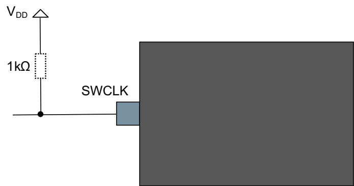
Figure 37-10.SWCLK Circuit Connections
