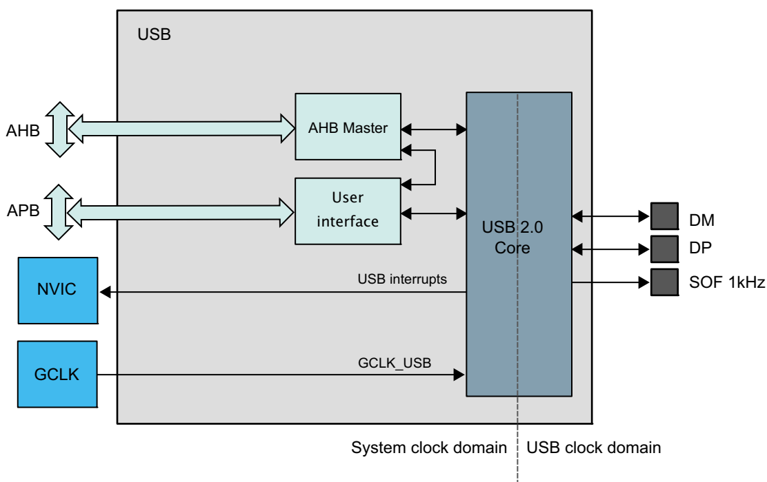
Figure 31-2. LS/FS Implementation: USB Block Diagram
