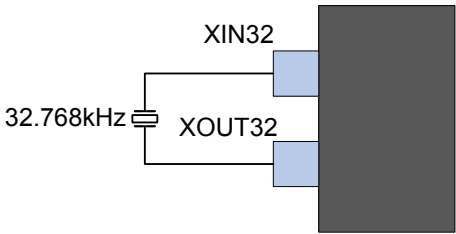
Figure 38-7. External Real Time Oscillator without Load Capacitor
