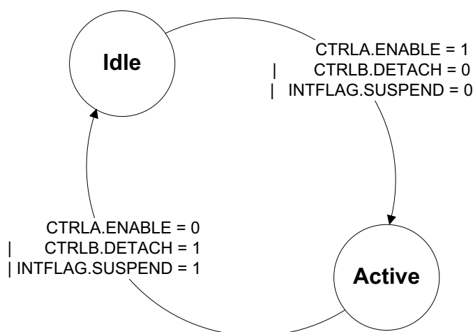
Figure 31-9. Pad Behavior
