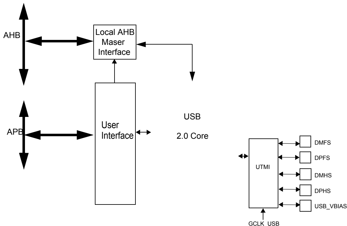
Figure 31-1. High-speed Implementation: USB Block Diagram
