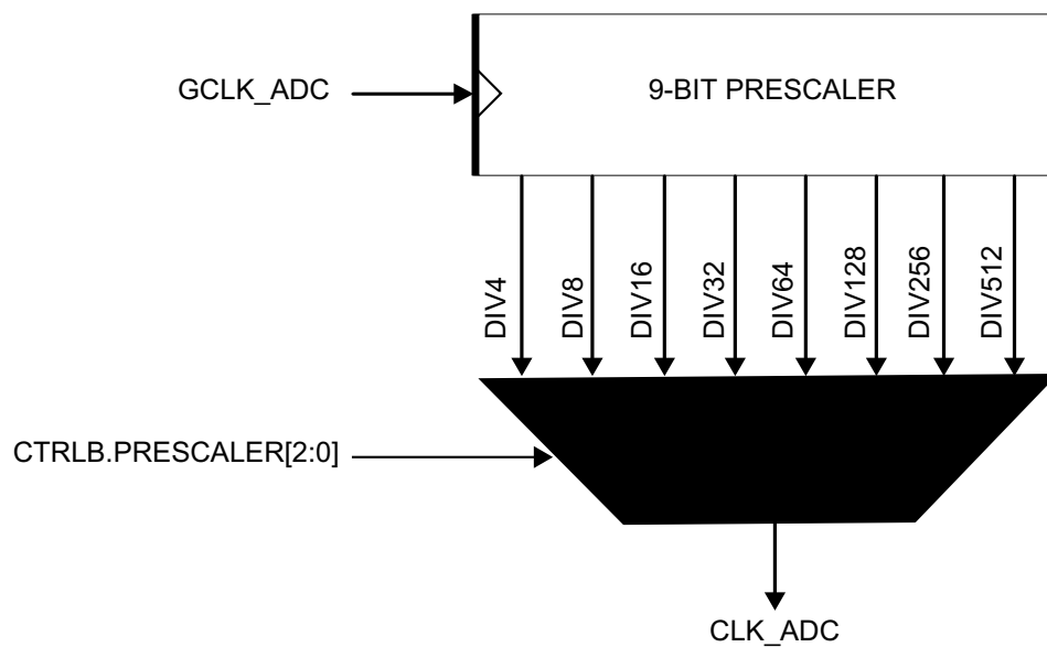
Figure 32-2. ADC Prescaler
