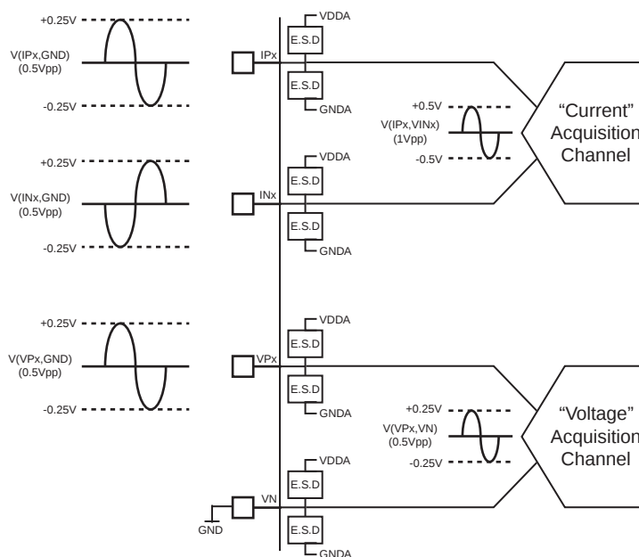
Figure 4-1. Analog Inputs: Recommended Input Range
