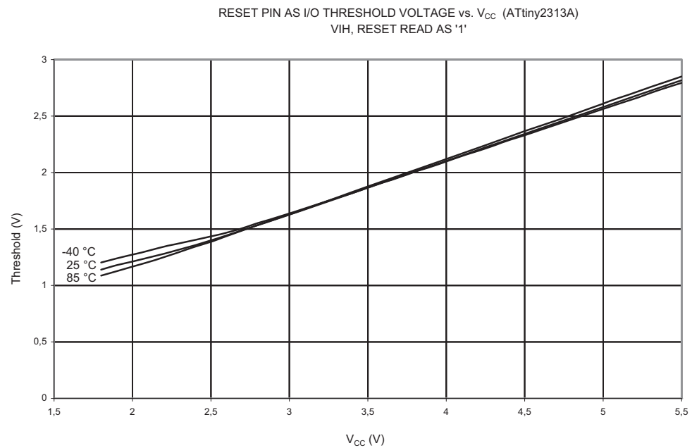
Figure 23-34. V_{IH} : Input Threshold Voltage vs. V_{CC} (Reset Pin as I/O, Read as '1')
