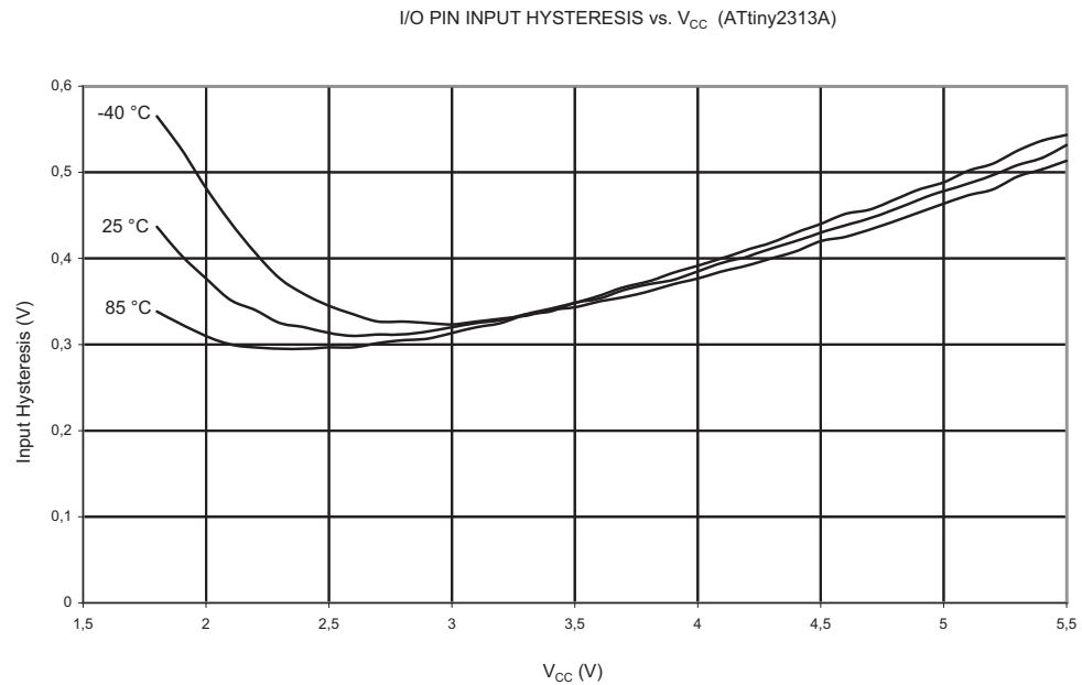
Figure 23-33. V_{IH}-V_{IL} : Input Hysteresis vs. V_{CC} (I/O Pin)
