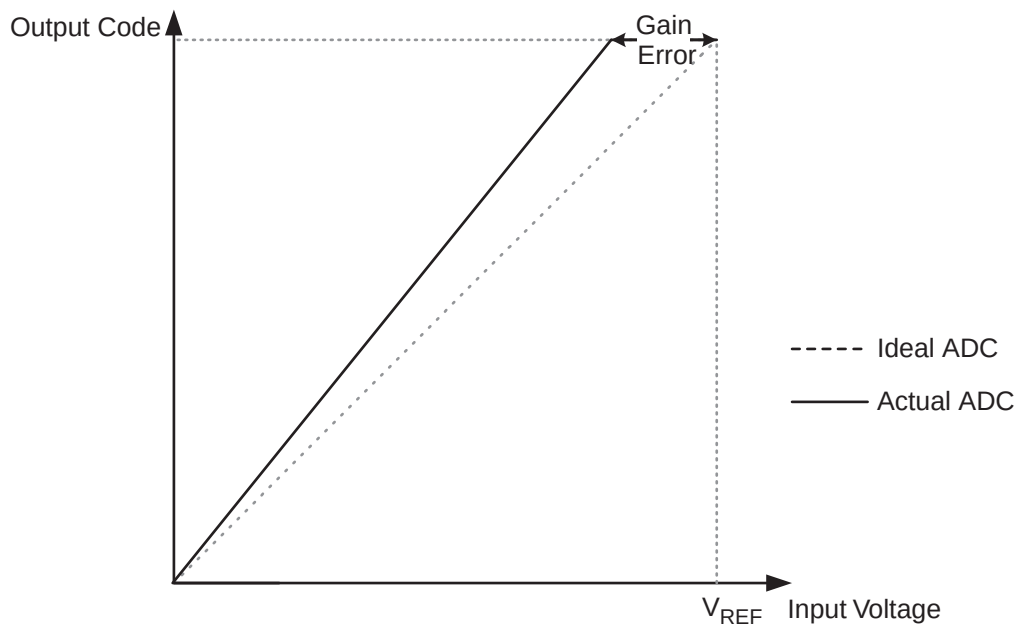
Figure 15-10. Gain Error
