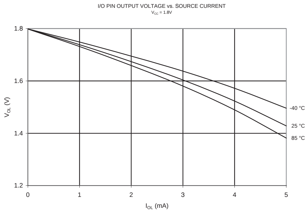
Figure 20-80. V_{OH} : Output Voltage vs. Source Current (I/O Pin, V_{CC} = 1.8V )
