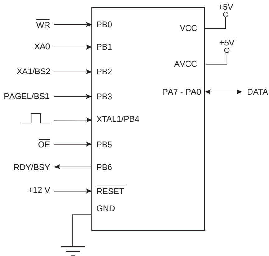
Figure 18-3. Parallel Programming.
