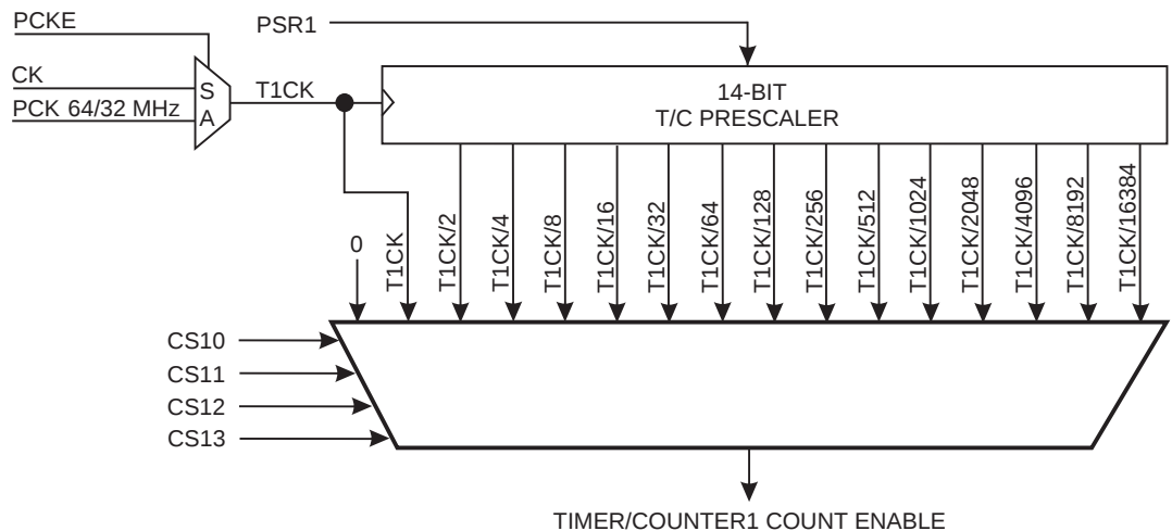
Figure 12-3. Timer/Counter1 Prescaler
