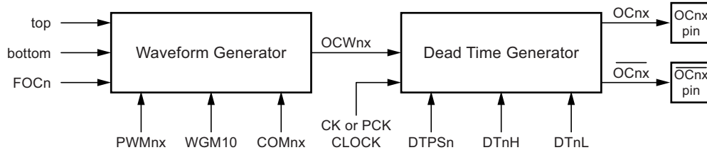
Figure 16-6. Output Compare Unit, Block Diagram
