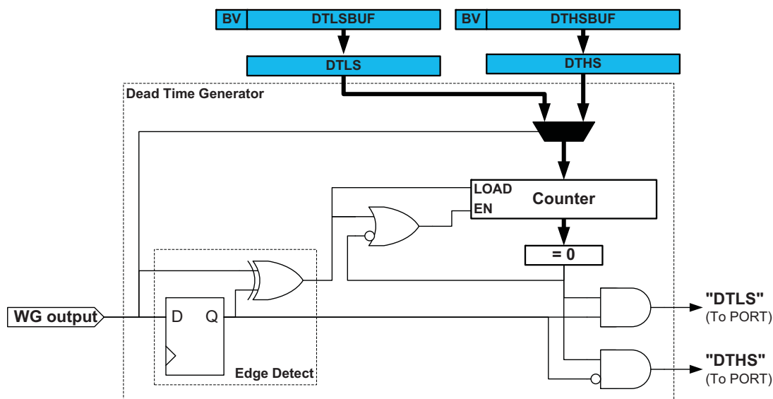
dead time. The high side and low side have independent dead-time setting, and the dead-time registers are double buffered.
