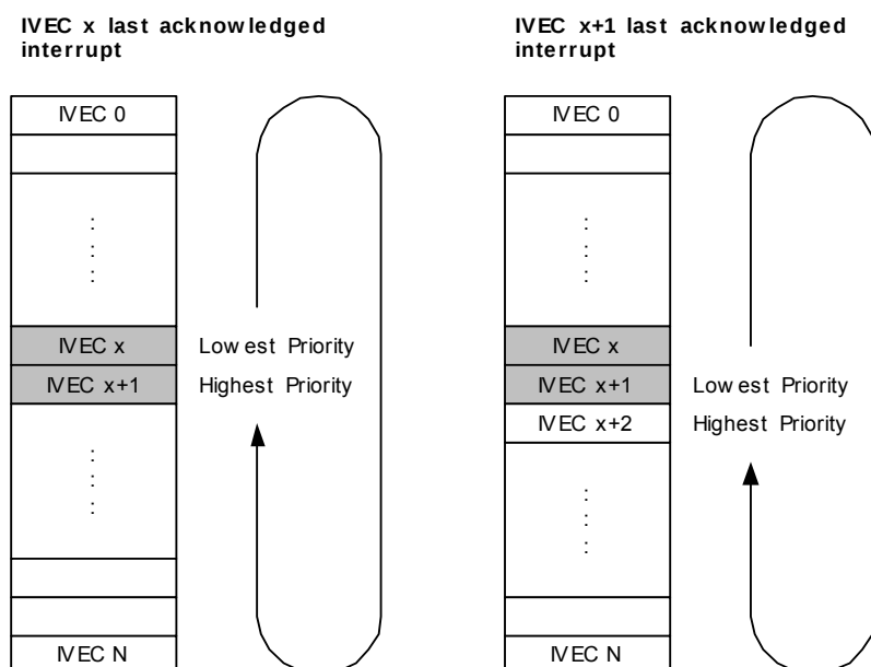
Figure 12-4. Round-robin scheduling.
