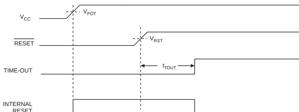
Figure 9-3. MCU startup, RESET extended externally,
