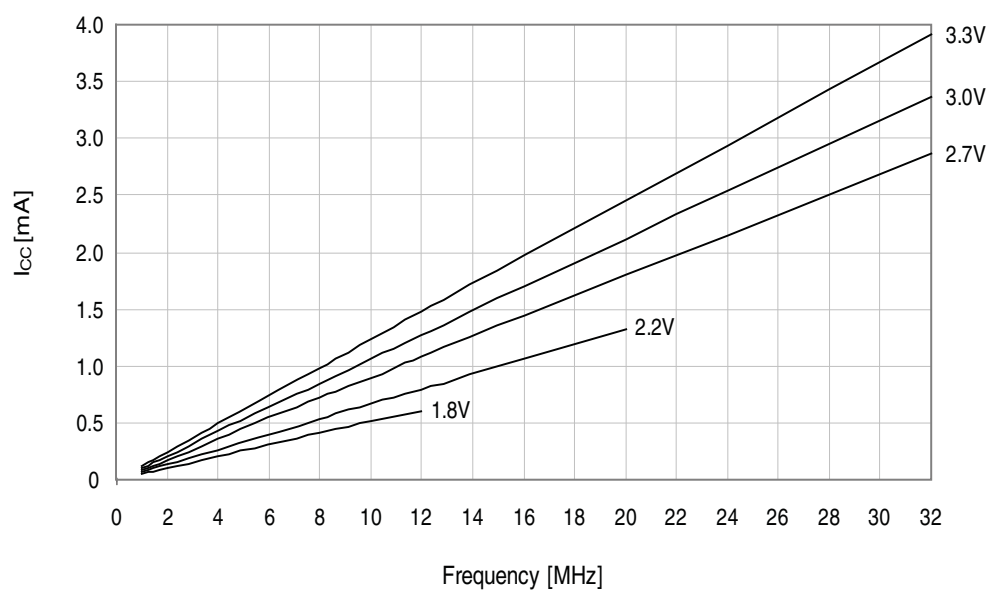
Figure 33-292. Idle Mode Supply Current vs. V_{CC}
