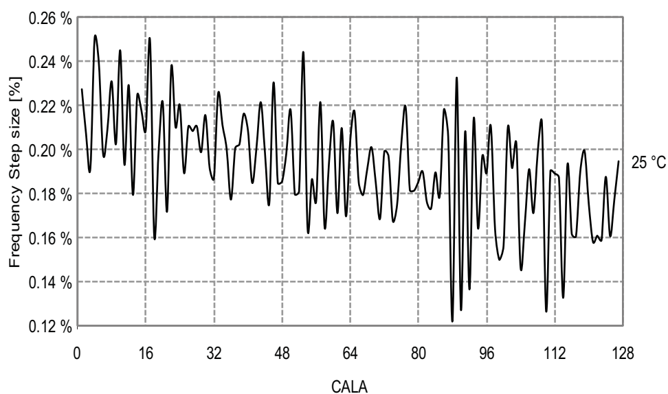
Figure 33-135. 32MHz Internal Oscillator CALA Calibration Step Size
