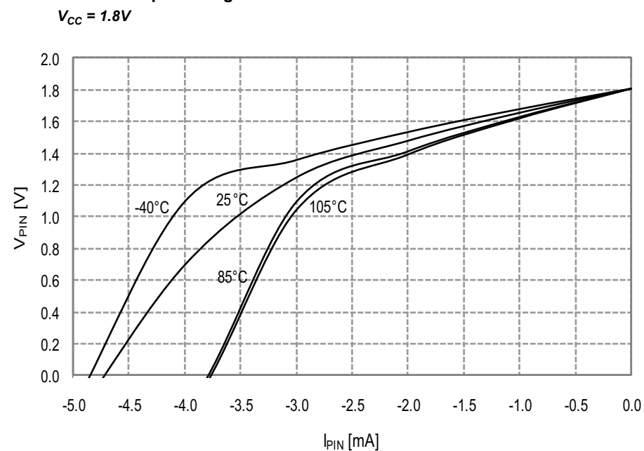
Figure 33-93. I/O Pin Output Voltage vs. Source Current
