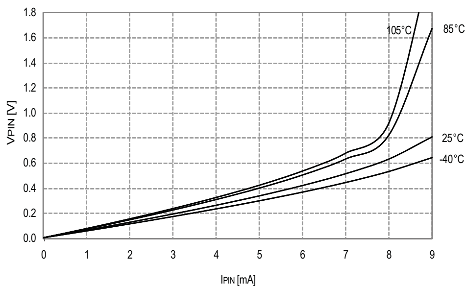
Figure 33-97. I/O Pin Output Voltage vs. Sink Current
