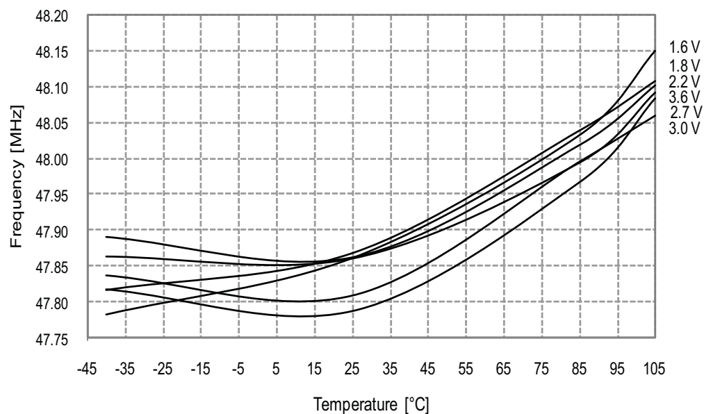
Figure 33-279. 48MHz Internal Oscillator Frequency vs. Temperature DPLL enabled, from the 32.768kHz internal oscillator
