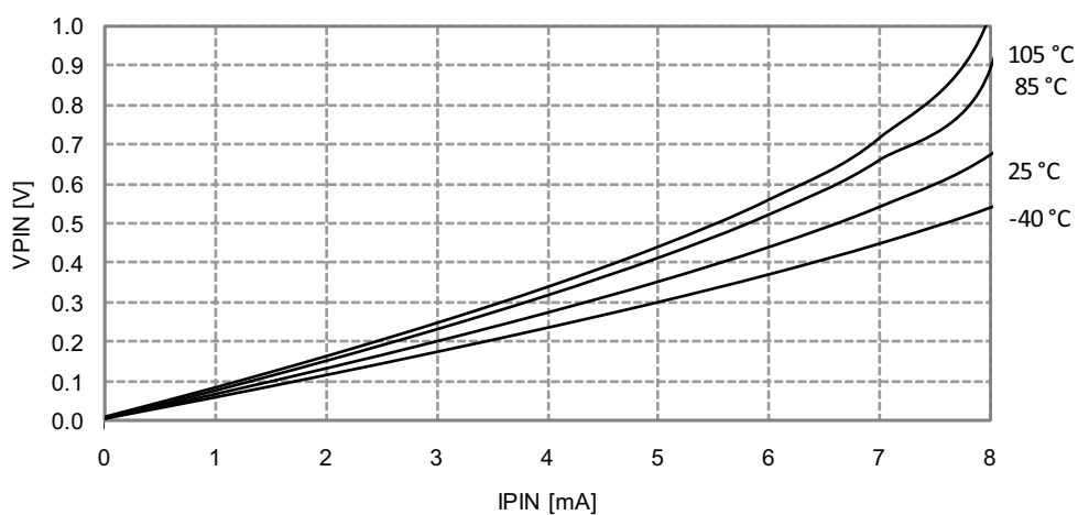
Figure 33-306. I/O Pin Output Voltage vs. Sink Current
