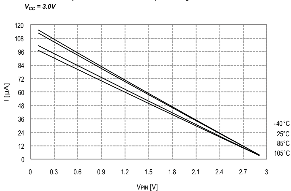
Figure 33-20. I/O Pin Pull-up Resistor Current vs. Input Voltage
