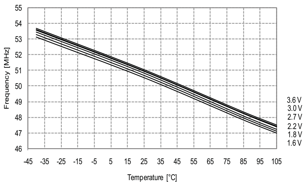
Figure 33-278. 48MHz Internal Oscillator Frequency vs. Temperature
