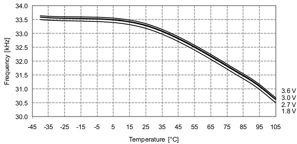
Figure 33-335. Ultra Low-Power Internal Oscillator Frequency vs. Temperature
