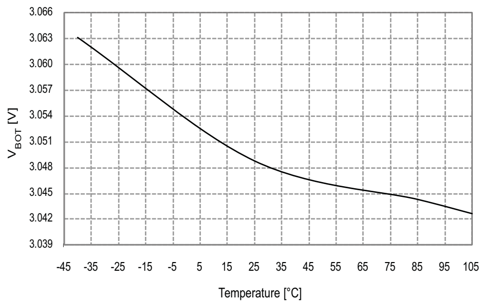
Figure 33-48. BOD Thresholds vs. Temperature
