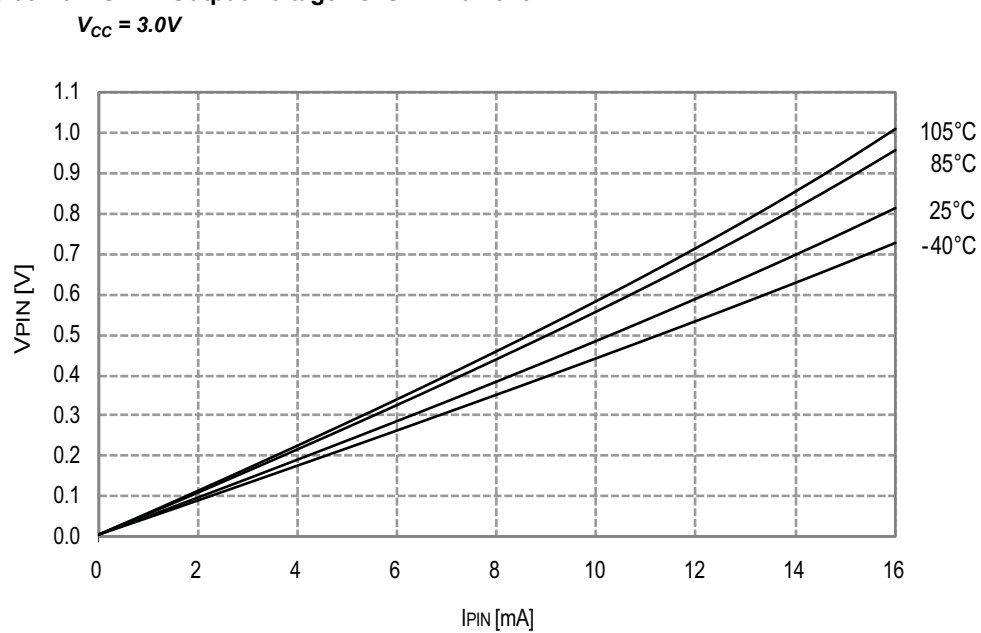
Figure 33-26. I/O Pin Output Voltage vs. Sink Current
