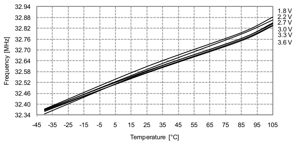
Figure 33-336. 32.768kHz Internal Oscillator Frequency vs. Temperature
