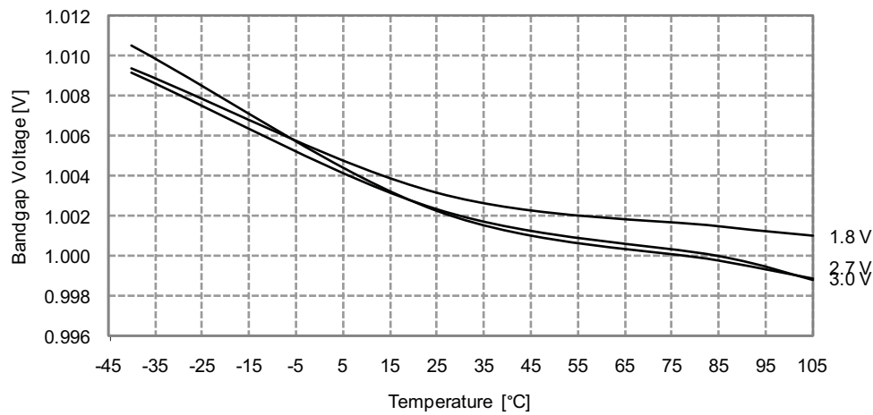
Figure 33-257.ADC Internal 1.0V Reference vs. Temperature
