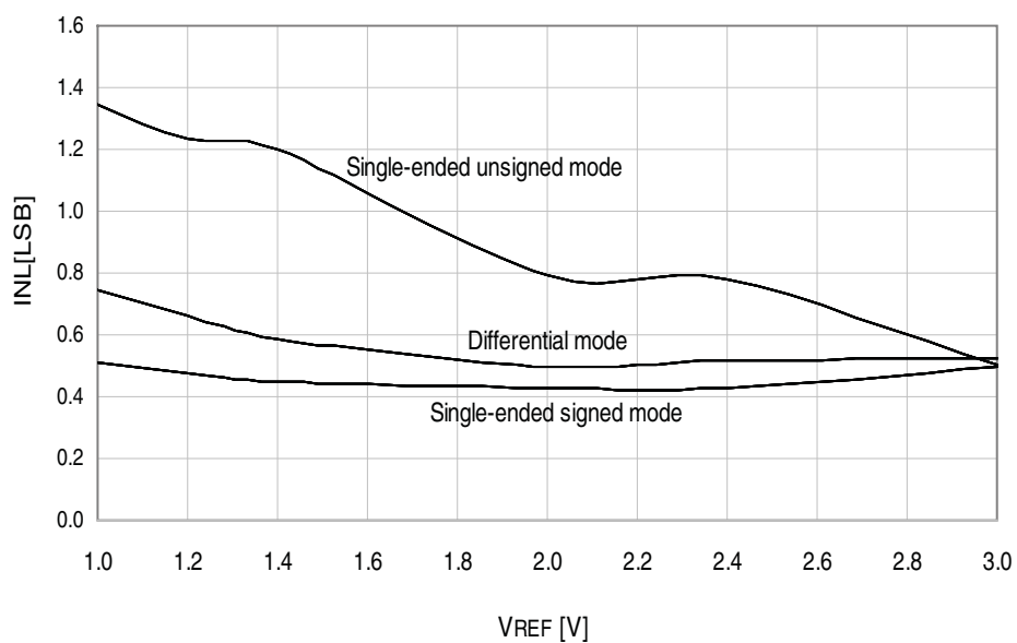
Figure 33-382. INL Error vs. External V_{REF} T = 25\text{ °C} , V_{CC} = 3.6\text{V} , external reference
