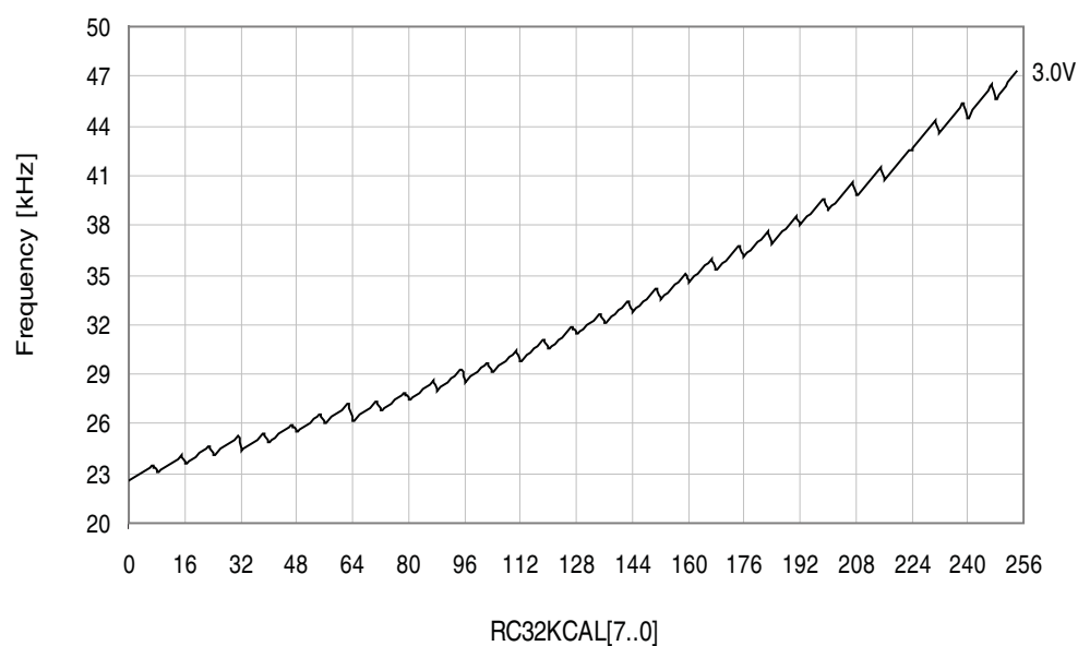
Figure 33-337. 32.768kHz Internal Oscillator Frequency vs. Calibration Value
