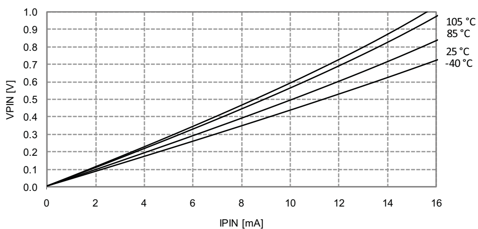
Figure 33-308. I/O Pin Output Voltage vs. Sink Current
