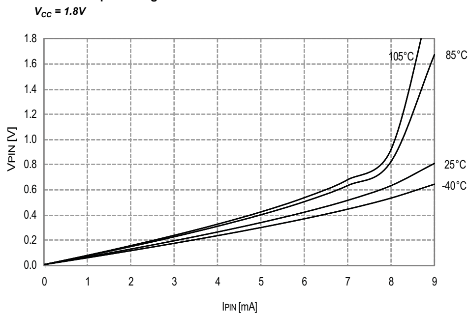
Figure 33-25. I/O Pin Output Voltage vs. Sink Current
