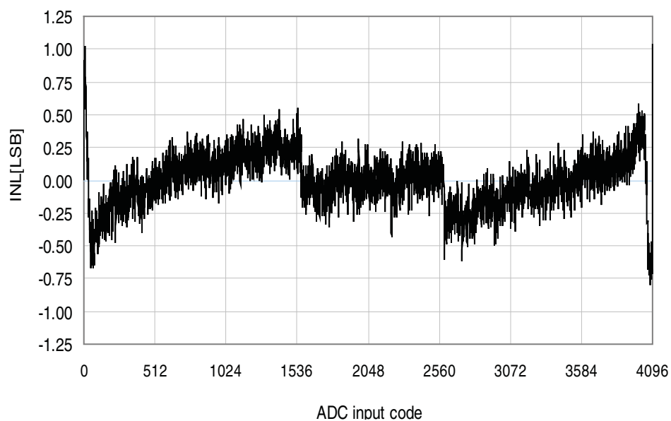
Figure 33-244. INL Error vs. Input Code
