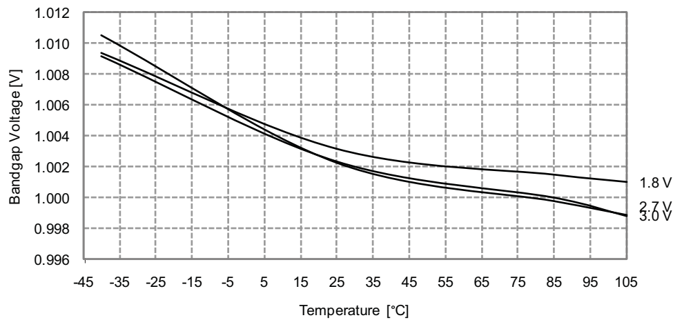
Figure 33-327. ADC Internal 1.0V Reference vs. Temperature
