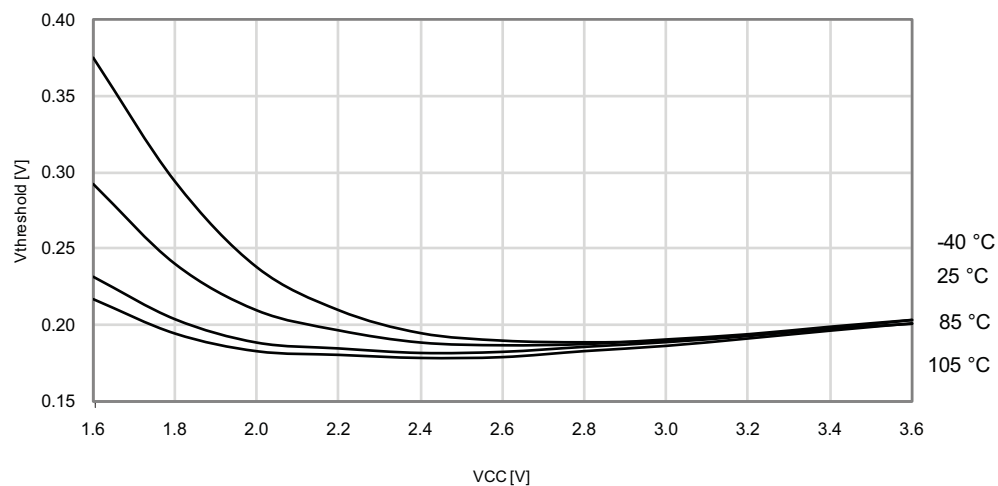
Figure 33-241. I/O Pin Input Hysteresis vs. V_{CC}
