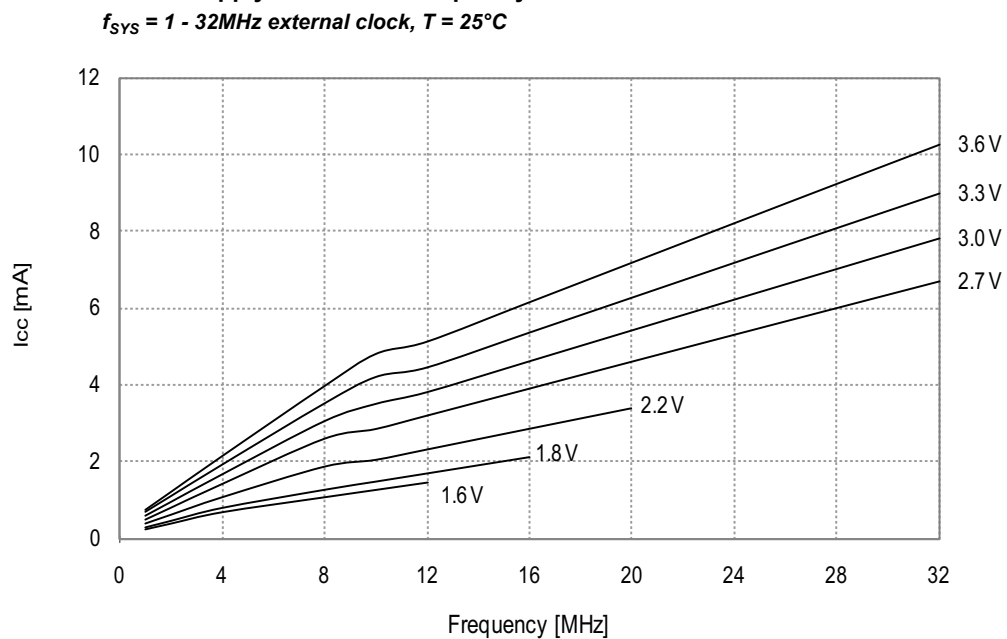
Figure 33-2. Active Supply Current vs. Frequency
