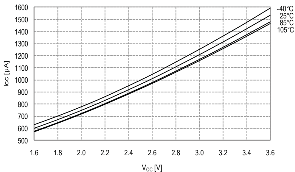
Figure 33-84. Idle Mode Supply Current vs. V_{CC} f_{SYS} = 32\text{MHz} internal oscillator prescaled to 8MHz
