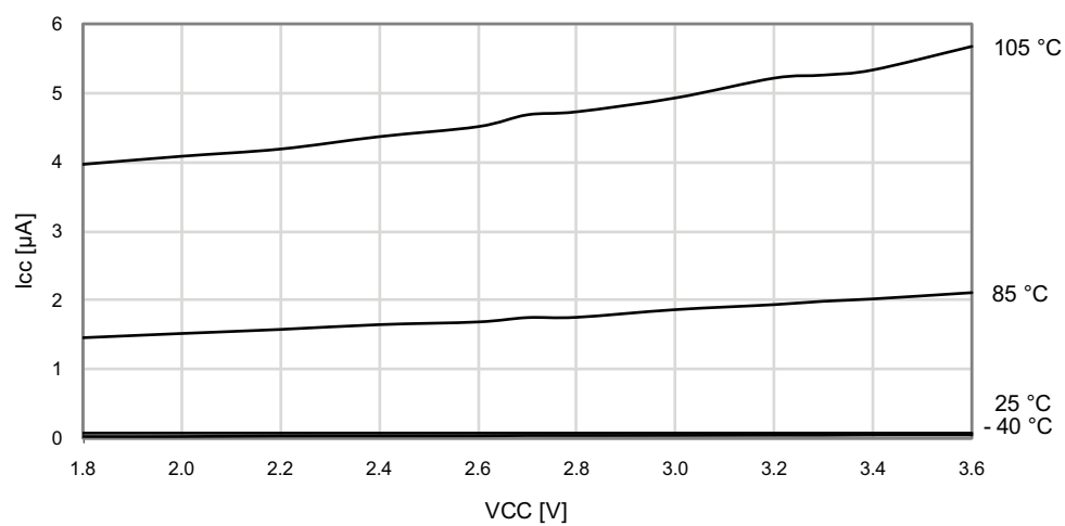
Figure 33-158. Power-down Mode Supply Current vs. V_{CC} Watchdog and sampled BOD enabled
