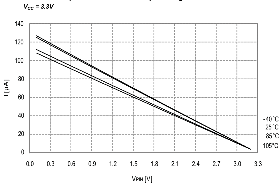
Figure 33-92. I/O Pin Pull-up Resistor Current vs. Input Voltage
