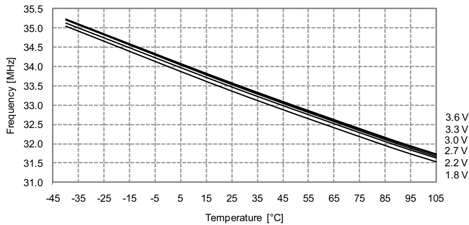
Figure 33-341. 32MHz Internal Oscillator Frequency vs. Temperature DFLL disabled
