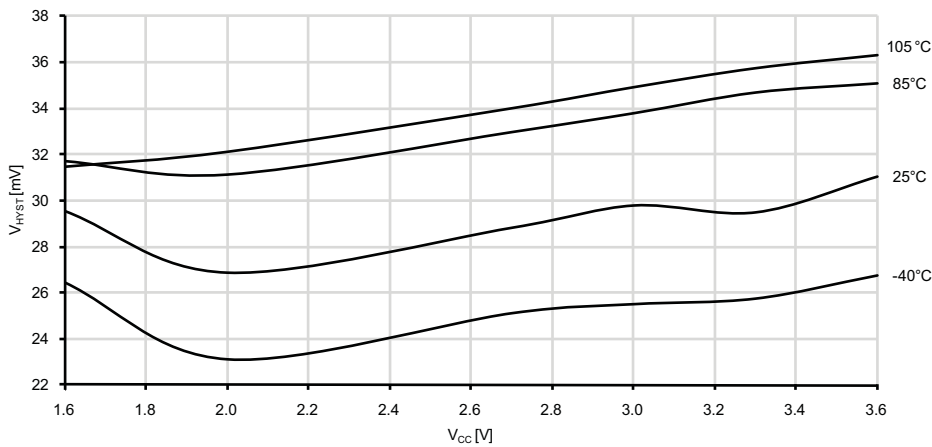
Figure 33-324. Analog Comparator Hysteresis vs. V_{CC} Large hysteresis
