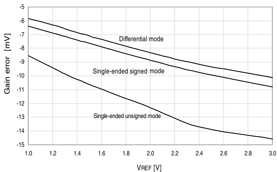
Figure 33-178. Gain Error vs. V_{REF} T = 25^{\circ}\text{C} , V_{CC} = 3.6\text{V} , ADC sample rate = 300ksps
