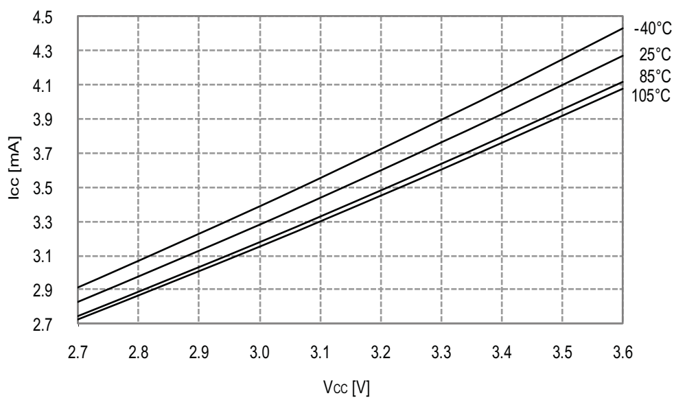
Figure 33-85. Idle Mode Current vs. V_{CC} f_{SYS} = 32\text{MHz} internal oscillator
