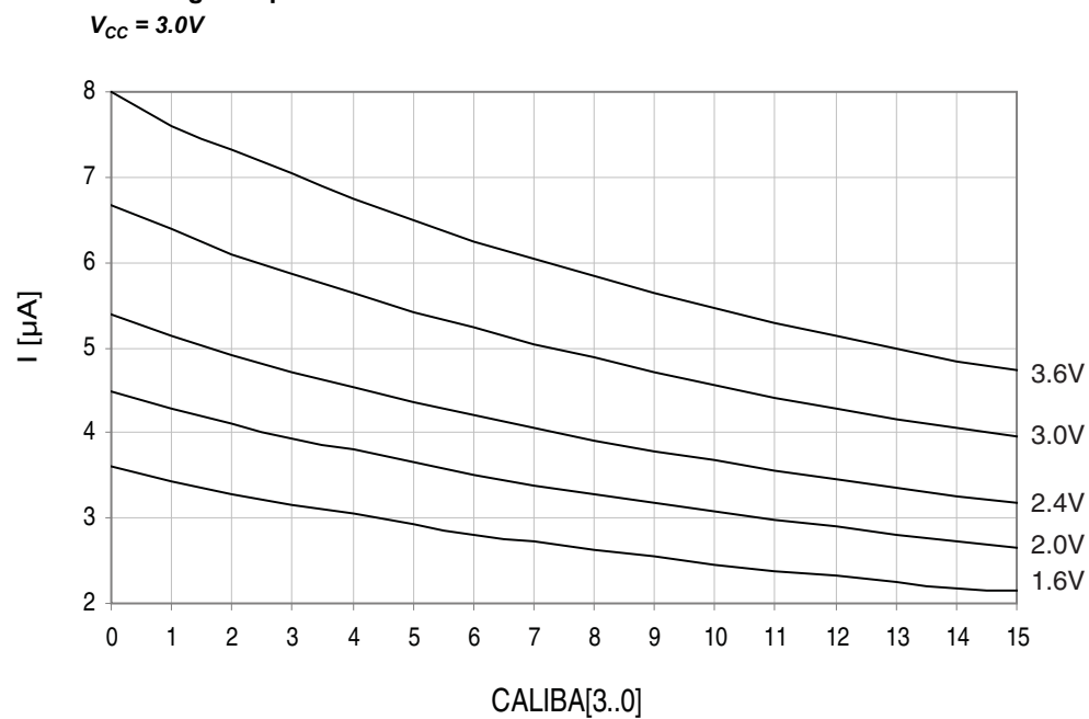
Figure 33-395. Analog Comparator Current Source vs. Calibration Value
