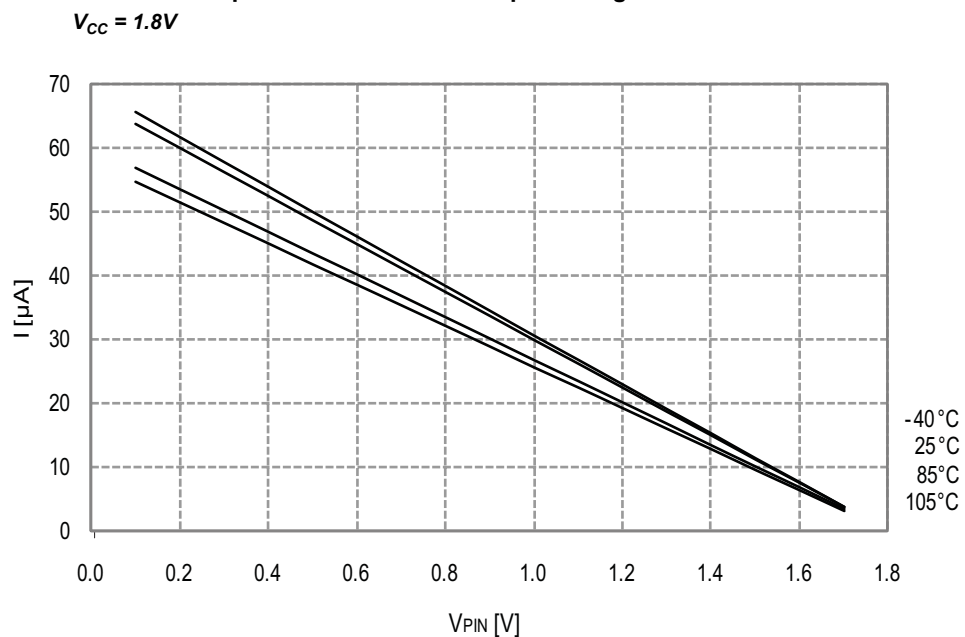
Figure 33-19. I/O Pin Pull-up Resistor Current vs. Input Voltage
