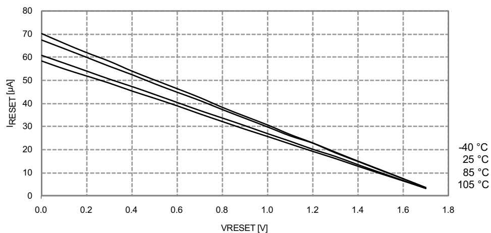
Figure 33-331. Reset Pin Pull-up Resistor Current vs. Reset Pin Voltage
