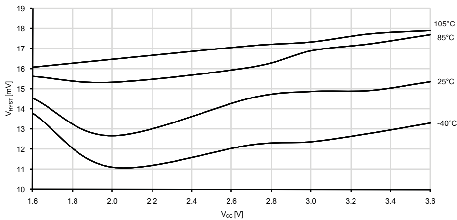
Figure 33-323. Analog Comparator Hysteresis vs. V_{CC} Small hysteresis
