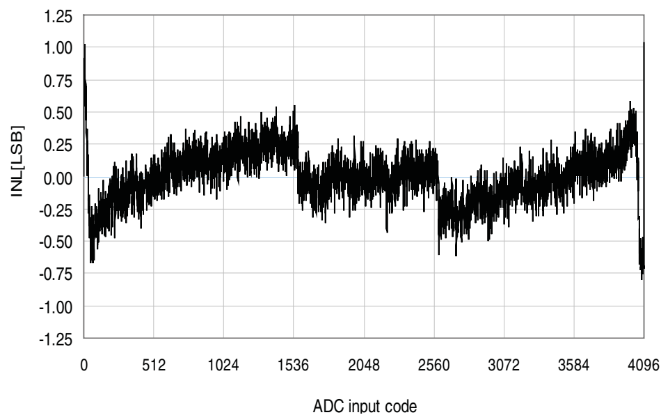
Figure 33-384. INL Error vs. Input Code
