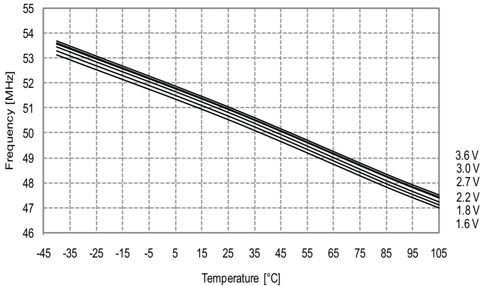
Figure 33-139. 48MHz Internal Oscillator Frequency vs. Temperature DPLL enabled, from the 32.768kHz internal oscillator
