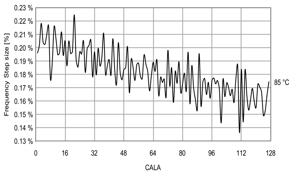
Figure 33-206. 32MHz Internal Oscillator CALA Calibration Step Size
