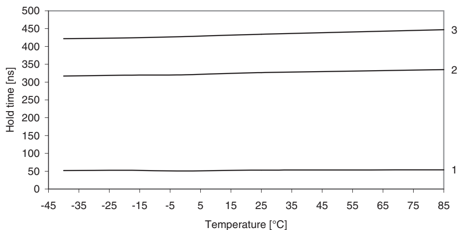
Figure 33-350. SDA Hold Time vs. Temperature
