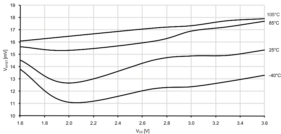
Figure 33-253. Analog Comparator Hysteresis vs. V_{CC} Small hysteresis
