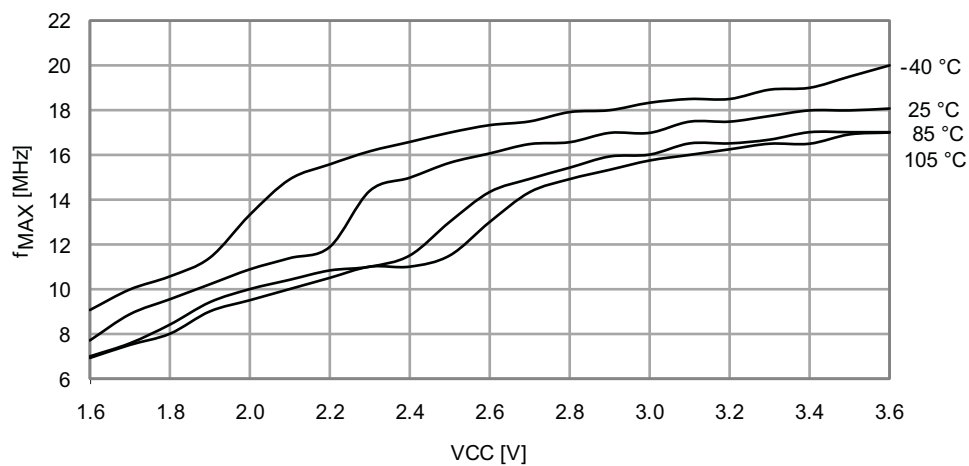
Figure 33-282.Maximum PDI Frequency vs. V_{CC}
