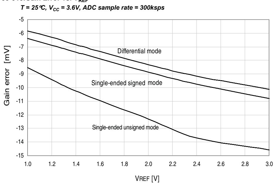
Figure 33-318.Gain Error vs. V_{REF}
