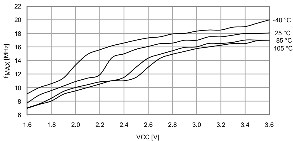
Figure 33-352. Maximum PDI Frequency vs. V_{CC}
