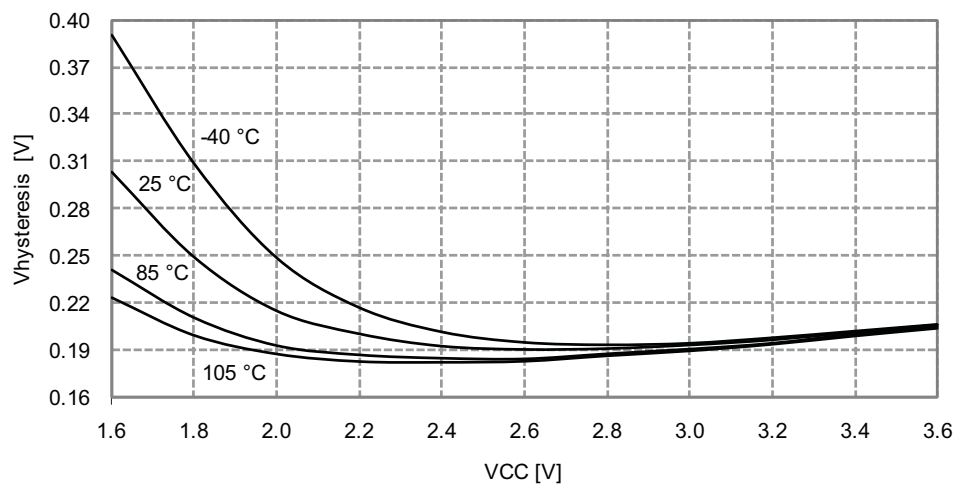
Figure 33-311. I/O Pin Input Hysteresis vs. V_{CC}
