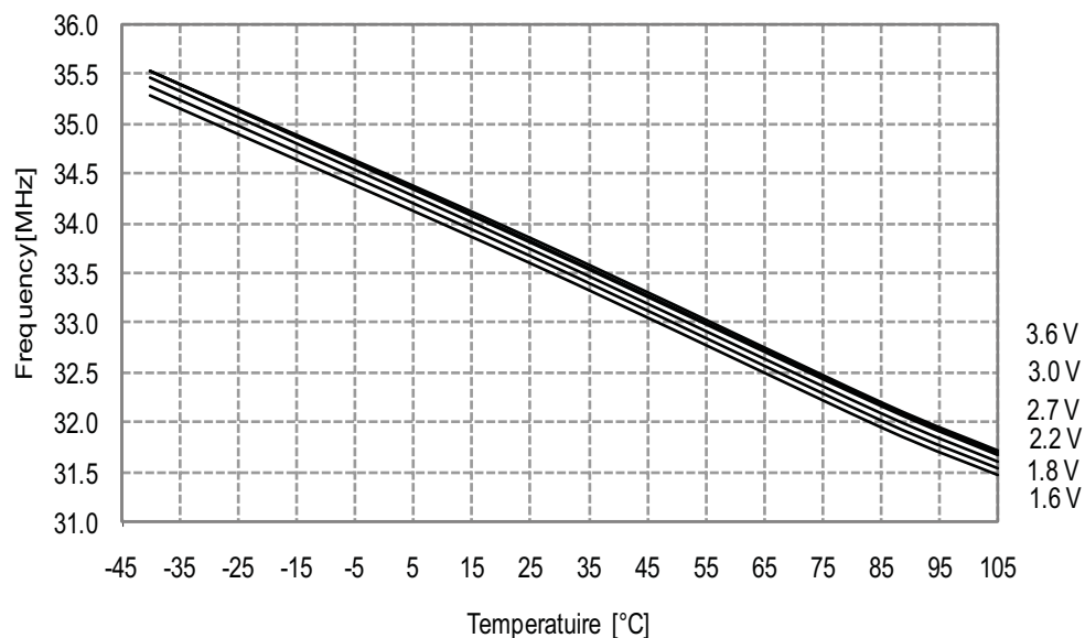
Figure 33-271. 32MHz Internal Oscillator Frequency vs. Temperature
