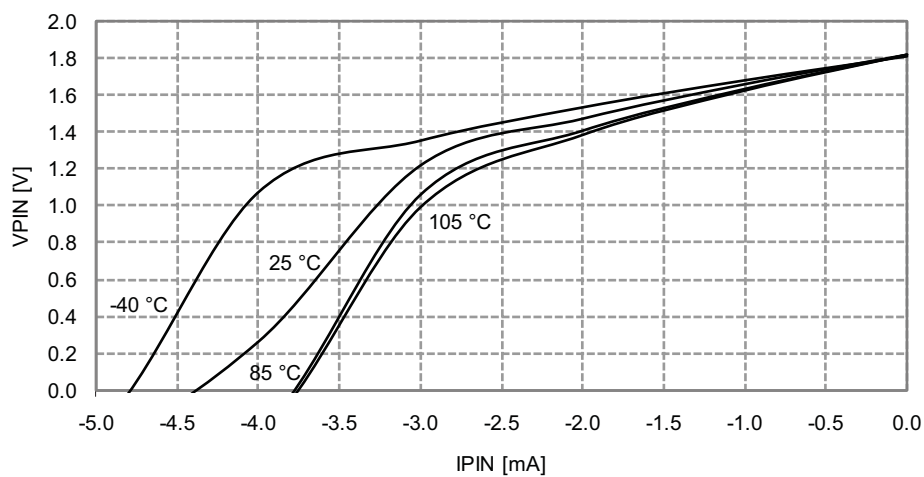
Figure 33-304. I/O Pin Output Voltage vs. Source Current
