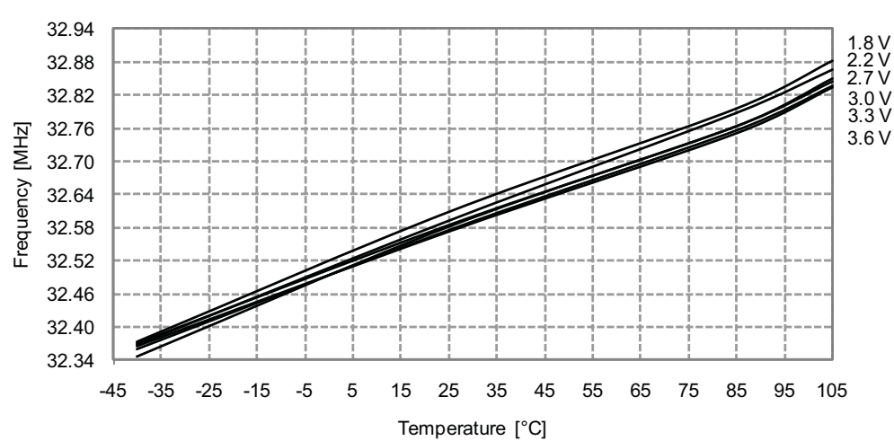
Figure 33-266.32.768kHz Internal Oscillator Frequency vs. Temperature
