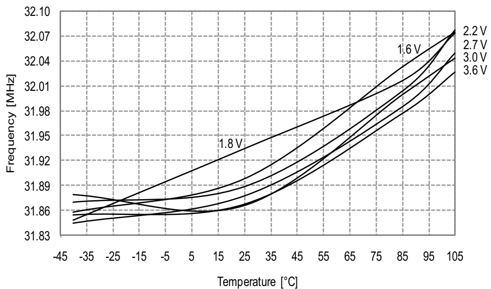
Figure 33-272. 32MHz Internal Oscillator Frequency vs. Temperature
