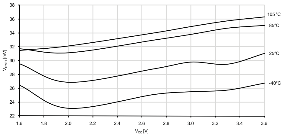
Figure 33-254. Analog Comparator Hysteresis vs. V_{CC} Large hysteresis
