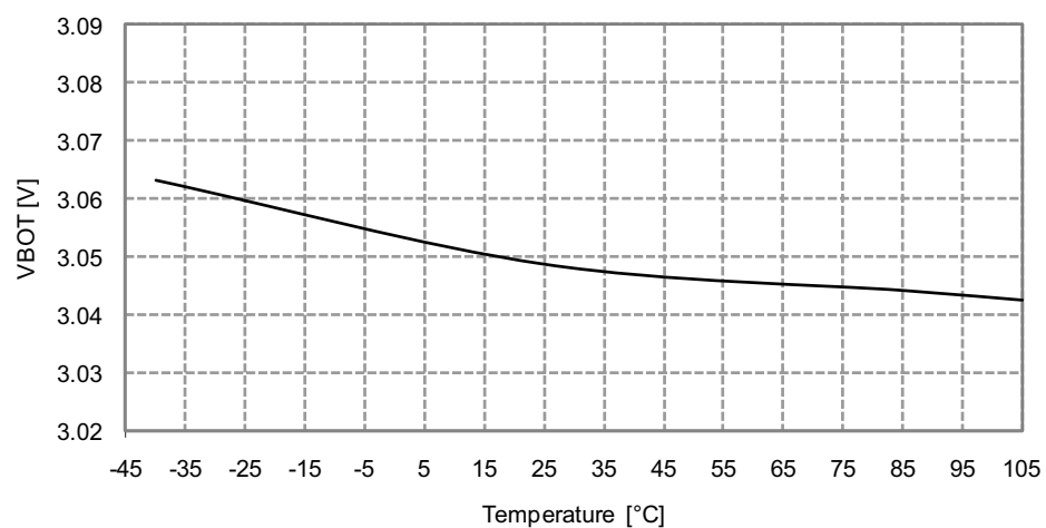
Figure 33-329. BOD Thresholds vs. Temperature
