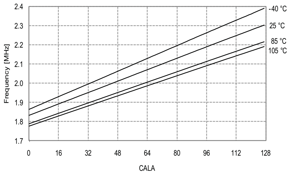
Figure 33-270. 2MHz Internal Oscillator Frequency vs. CALA Calibration Value V_{CC} = 3V
