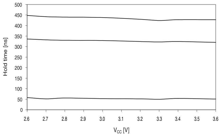
Figure 33-281.SDA Hold Time vs. Supply Voltage
