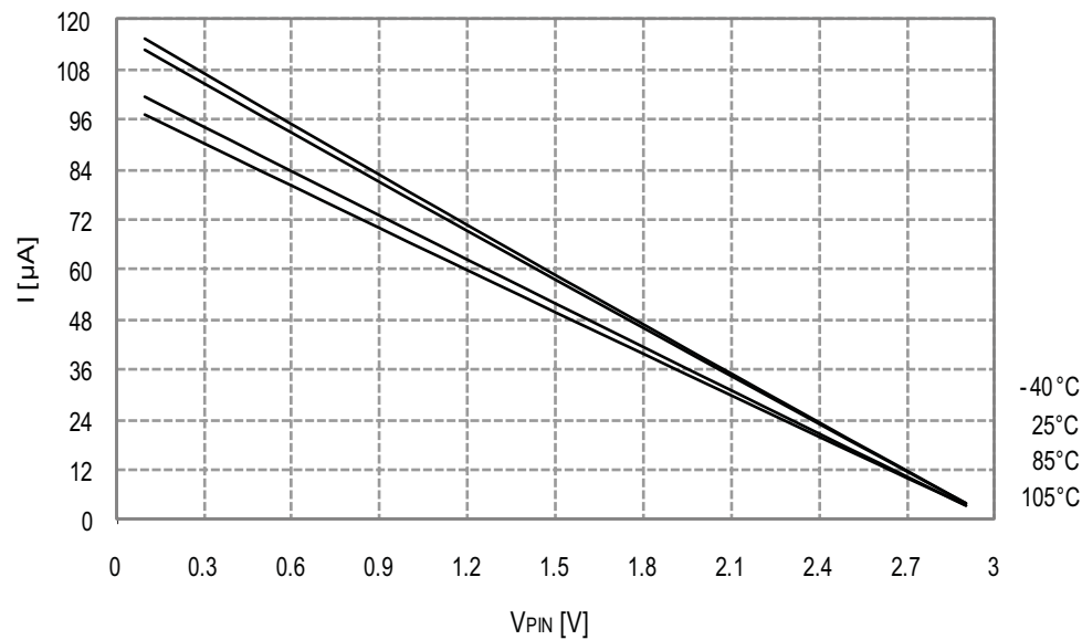
Figure 33-91. I/O Pin Pull-up Resistor Current vs. Input Voltage V_{CC} = 3.0V
