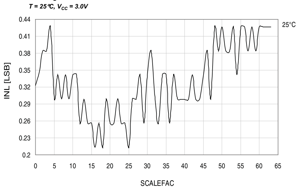
Figure 33-396. Voltage Scaler INL vs. SCALEFAC
