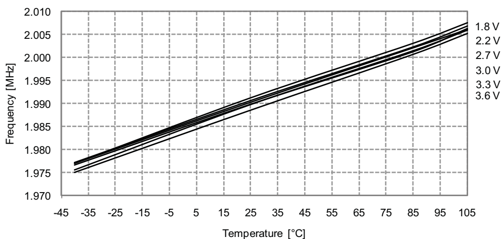
Figure 33-269. 2MHz Internal Oscillator Frequency vs. Temperature DFLL enabled, from the 32.768kHz internal oscillator
