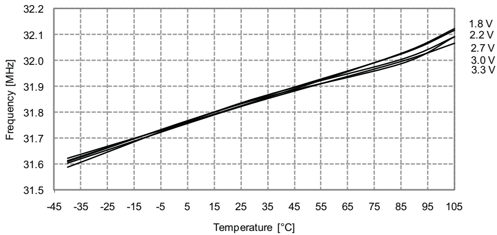
Figure 33-342. 32MHz Internal Oscillator Frequency vs. Temperature DFLL enabled, from the 32.768kHz internal oscillator
