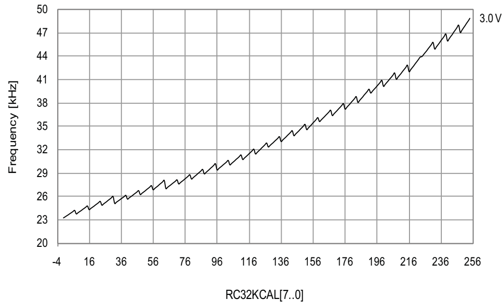
Figure 33-127. 32.768kHz Internal Oscillator Frequency vs. Calibration Value V_{CC} = 3.0V, T = 25^{\circ}C
