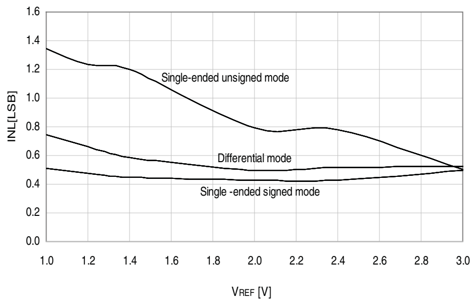
Figure 33-172. INL Error vs. External V_{REF} T = 25^{\circ}\text{C} , V_{CC} = 3.6\text{V} , external reference
