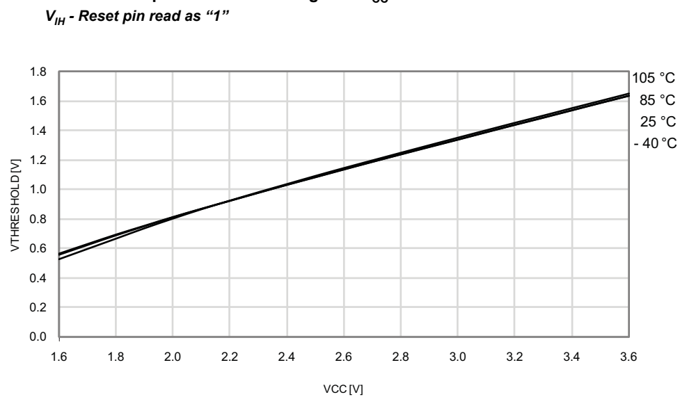
Figure 33-264. Reset Pin Input Threshold Voltage vs. V_{CC}
