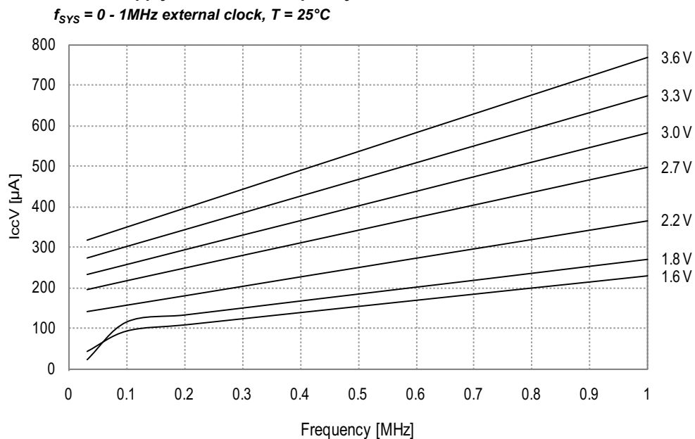
Figure 33-1. Active Supply Current vs. Frequency
