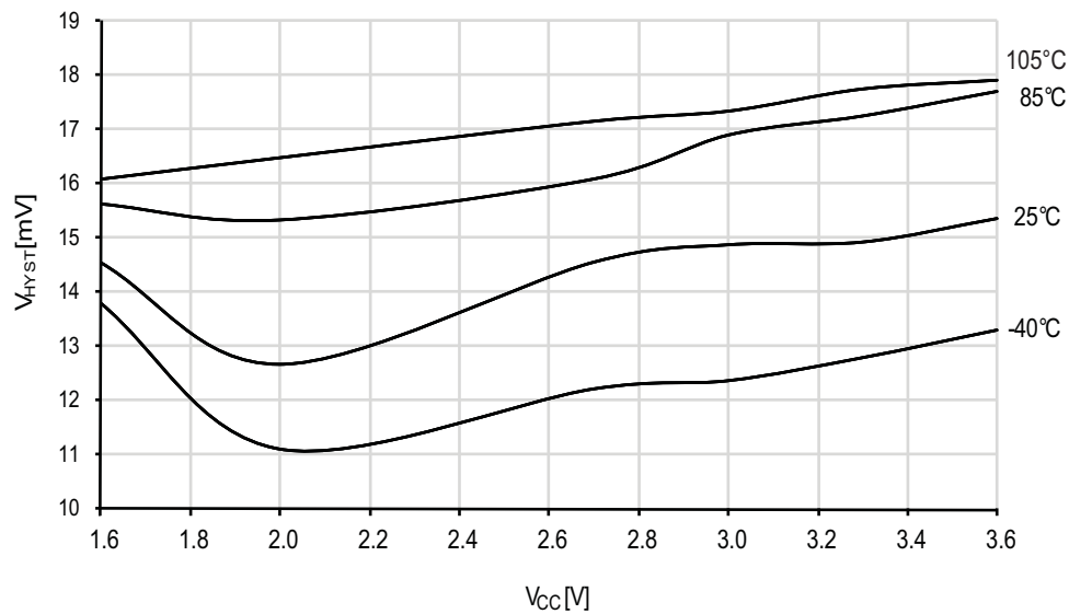
Figure 33-184. Analog Comparator Hysteresis vs. V_{CC} Large hysteresis
