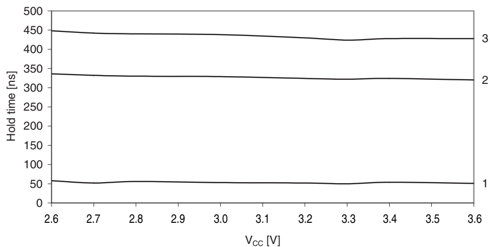
Figure 33-351. SDA Hold Time vs. Supply Voltage
