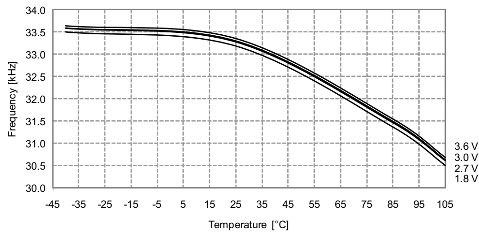
Figure 33-265.Ultra Low-Power Internal Oscillator Frequency vs. Temperature
