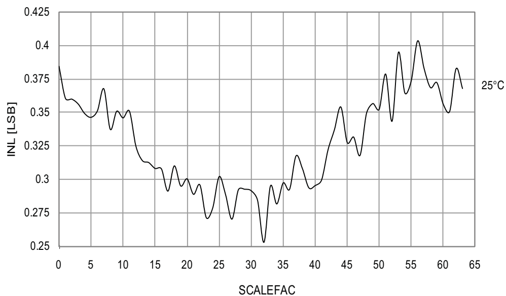
Figure 33-186. Voltage Scaler INL vs. SCALEFAC
