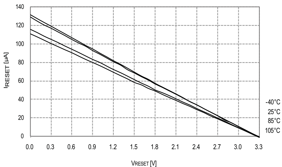
Figure 33-123. Reset Pin Pull-up Resistor Current vs. Reset Pin Voltage
