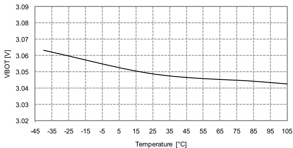
Figure 33-259. BOD Thresholds vs. Temperature
