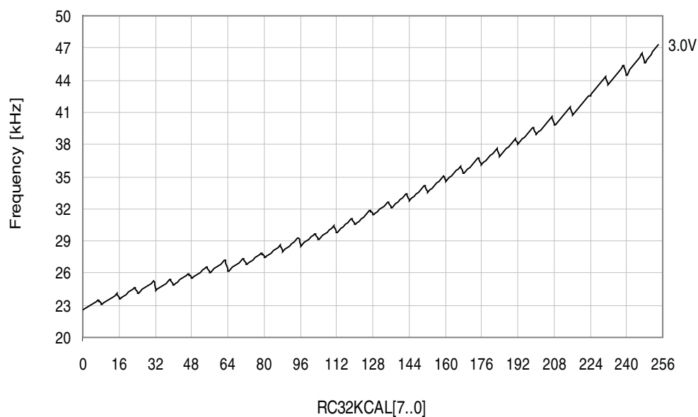
Figure 33-267. 32.768kHz Internal Oscillator Frequency vs. Calibration Value
