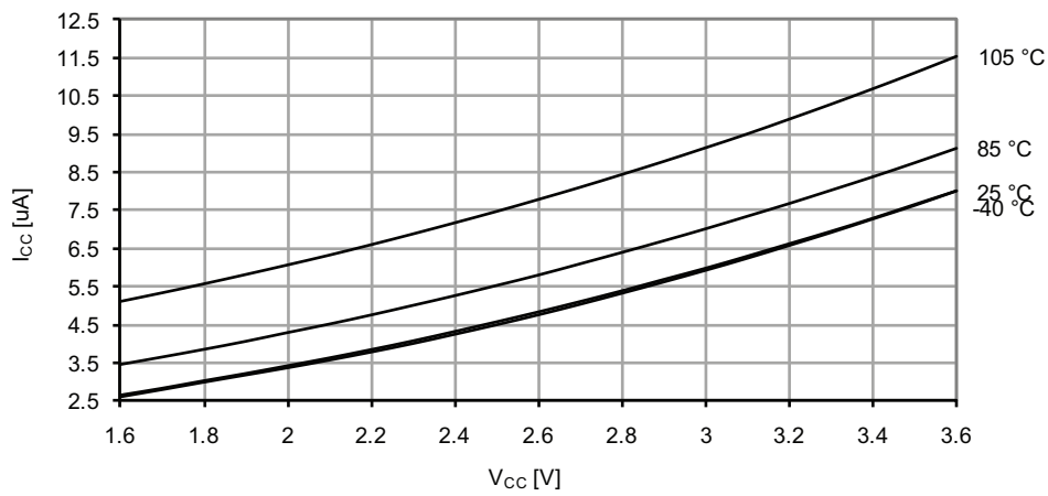
Figure 33-261. Standby Supply Current vs. V_{CC}
