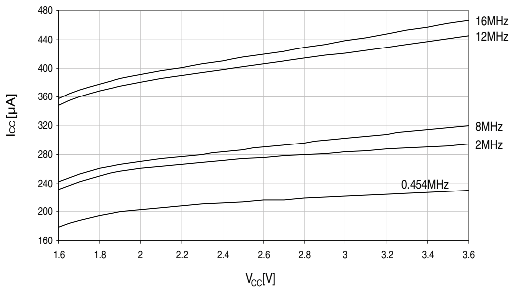
Figure 33-262. Standby Supply Current vs. V_{CC}
