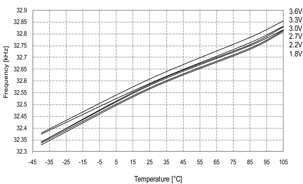
Figure 33-145. 32.768kHz Internal Oscillator Frequency vs. Temperature
