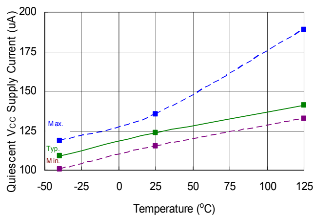
Figure 16. V_{CC} Supply Current vs. Temperature
