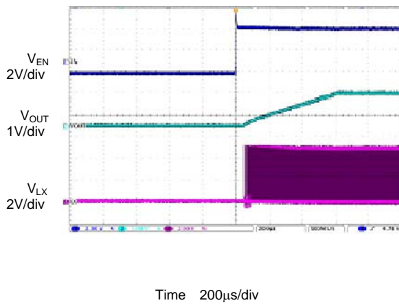
Figure 16. Soft Start
