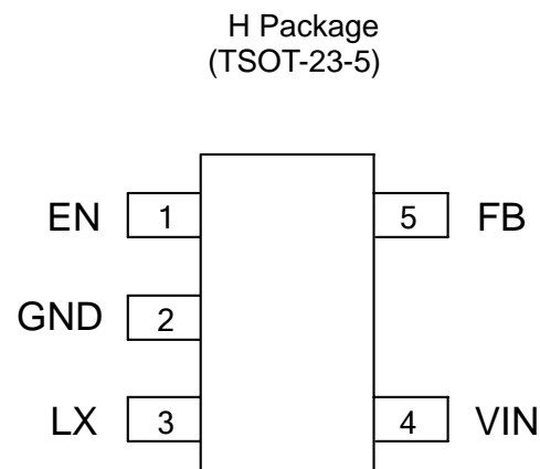
Figure 2. Pin Configuration of AUR9713 (Top View)
