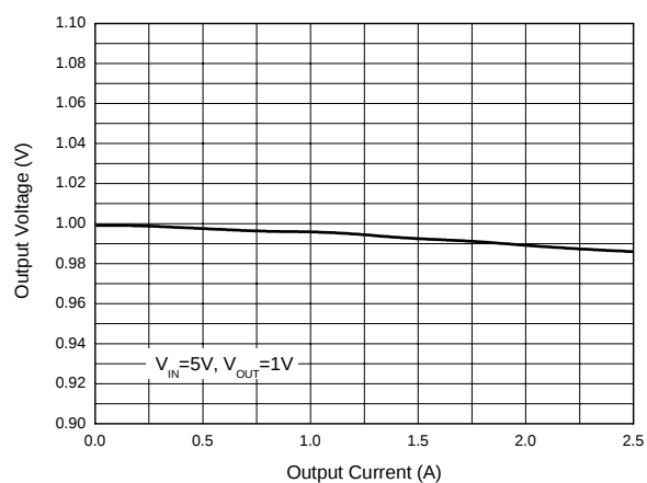
Figure 9. 1.0V Load Regulation
