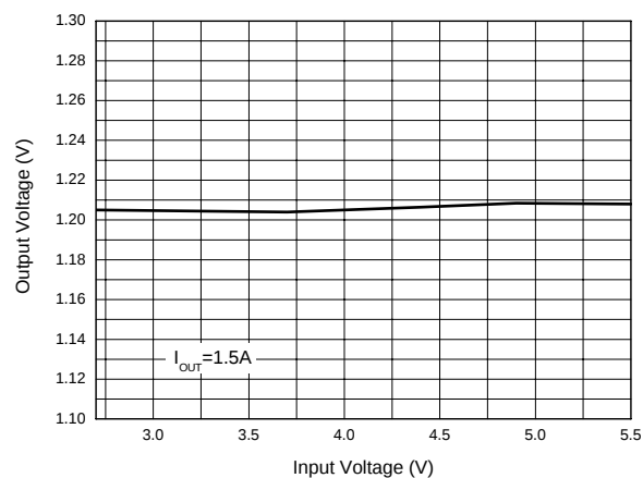
Figure 11. 1.2V Line Regulation
