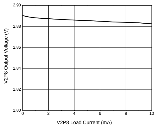
V2P8 Output Voltage vs. V2P8 Load Current
