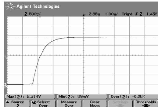
Fig.6 Typical start-up from CNT on
