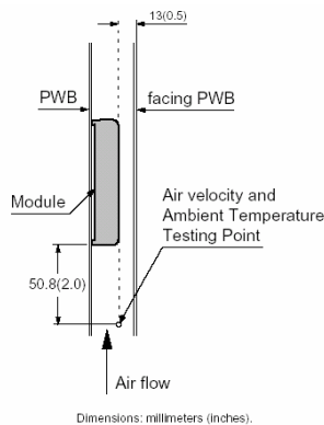
Figure 20 Experiment setup
