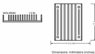
Figure 24 Longitudinal fins heatsink
