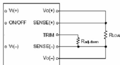
Figure 10 Trim down circuit
