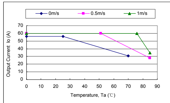
Figure 22 Forced convection power derating with baseplate
