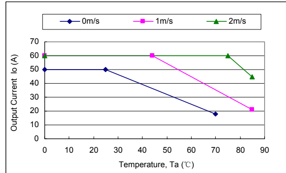
Figure 21 Forced convection power derating without baseplate
