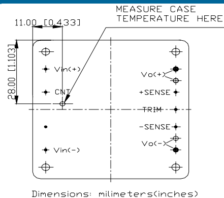
Figure 19 Temperature measurement location (without baseplate)
