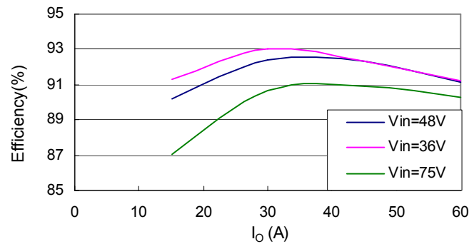
Fig.1 AVE300-48S2V5-4 Typical Efficiency
