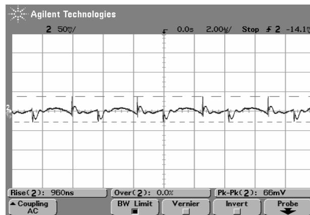
Fig.2 AVE300-48S2V5-4 Typical Output Ripple Voltage
