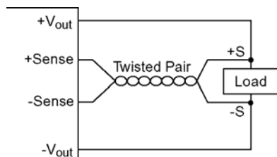
Figure 8 Sense connection
