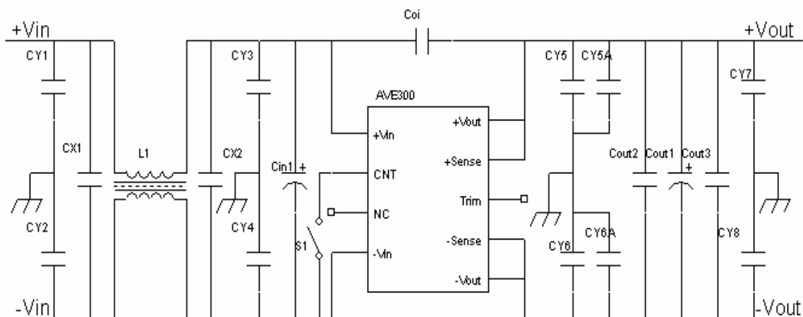
Figure 17 EMI reduction filter
