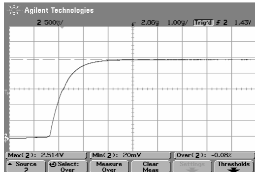
Fig.5 Typical start-up from power on
