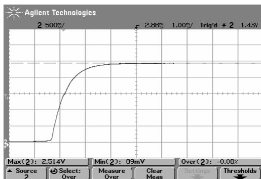
Fig3 AVE300-48S2V5-4 Typical Transient Response to Ta:25°C, Air velocity: 300LFM, forced air direction: from Vin+ to Vin-. Vin: 48V, Vonom, 25% Ionom step from 50% Ionom, 0.1A/ \mu s”, the external capacitor should be “10 \mu tantalum(ESR \leq 100 m \Omega ) // 1 \mu ceramic capacitor.
