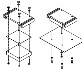
Figure 26 Heatsink mounting
