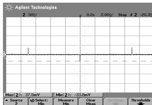
Fig4 AVE300-48S2V5-4. Typical Transient Response to Ta:25°C, Air velocity: 300LFM, forced air direction: from Vin+ to Vin-. Vin: 48V, Vonom, 50% Ionom from 75% Ionom, 0.1A/ \mu s”, the external capacitor should be “10 \mu tantalum(ESR \leq 100 m \Omega ) // 1 \mu ceramic capacitor.
