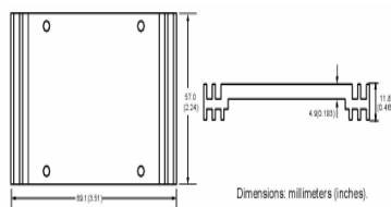
Figure 23 Non-standard heatsink
