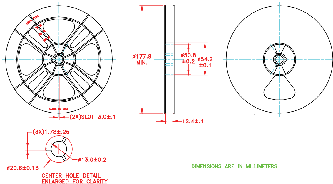
Figure 8: Carrier Tape
