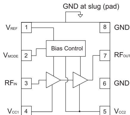
Figure 1: Block Diagram
