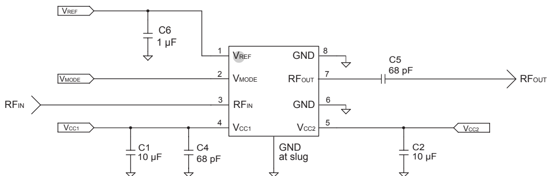
Figure 3: Application Circuit
