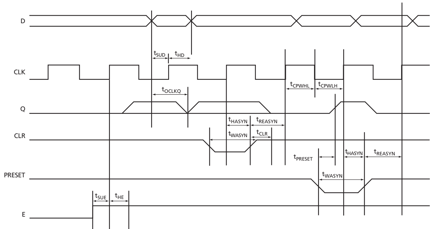
Figure 2-13 • Output Register Timing Characteristics
