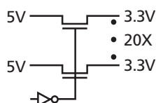
Figure 2-4 • Bus Switch IDTQS32X2384
