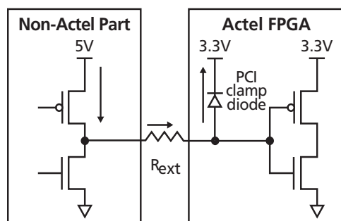
Figure 2-3 • Use of an External Resistor for 5V Tolerance
