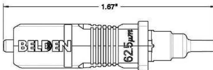
900 \mu\text{m} VERSION (OM1 SHOWN)
