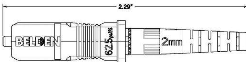
JACKETED VERSION (OM1 SHOWN)
