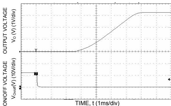
Figure 15. Typical Start-Up Using Remote On/Off with Low-ESR external capacitors (7x150uF Polymer) ( V_{IN} = 12.0\text{Vdc} , V_o = 3.3\text{Vdc} , I_o = 3\text{A} , C_o = 1050\text{ }\mu\text{F} ).
