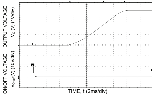
Figure 15. Typical Start-Up Using Remote On/Off with Low-ESR external capacitors (7x150µF Polymer) ( V_{IN} = 12.0\text{Vdc} , V_o = 3.3\text{Vdc} , I_o = 3\text{A} , C_o = 1050\mu\text{F} ).
