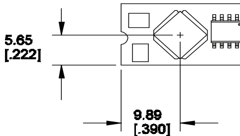
Figure 33. Pick and Place Location.
