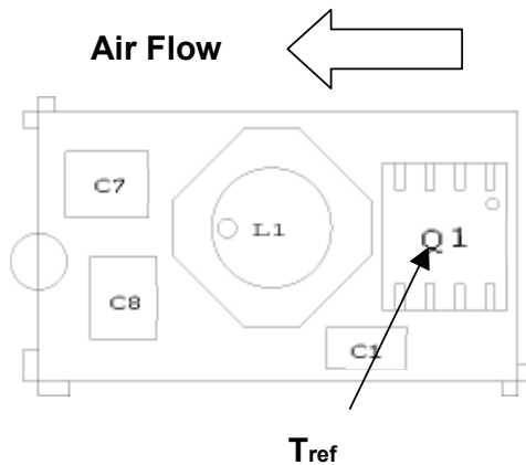
Figure 31. T_{ref} Temperature measurement location.
