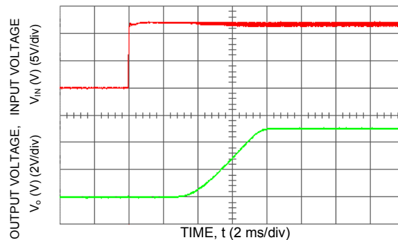
Figure 16. Typical Start-Up with application of V_{in} with low-ESR polymer capacitors at the output (7x150 μF) ( V_{in} = 12 Vdc, V_o = 5.0 Vdc, I_o = 16 A, C_o = 1050 μF).
