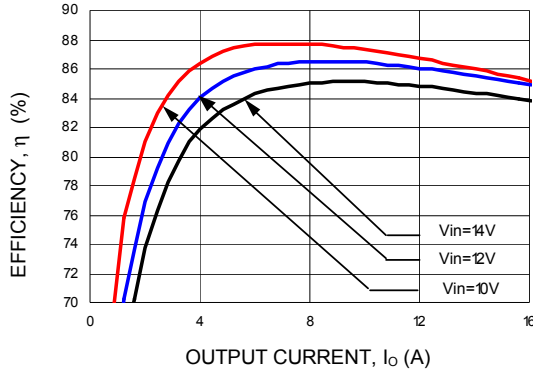
Figure 1. Converter Efficiency versus Output Current ( V_{out} = 0.75Vdc ).
