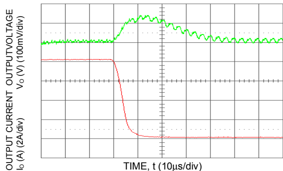
Figure 13. Transient Response to Dynamic Load Change from 100% of 50% full load ( V_o = 5.0 Vdc, C_{ext} = 2 \times 150 μF Polymer Capacitors).
