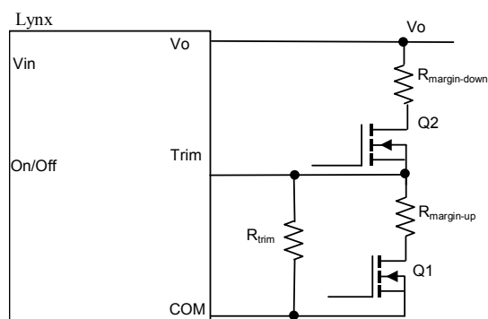
Figure 30. Circuit Configuration for margining Output voltage.
