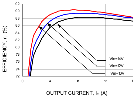
Figure 3. Converter Efficiency versus Output Current ( V_{out} = 1.5Vdc ).
