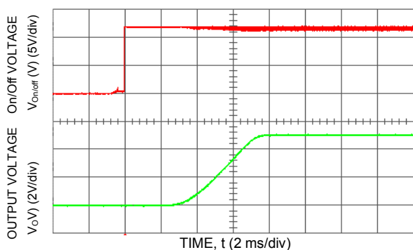
Figure 15. Typical Start-Up Using Remote On/Off with Low-ESR external capacitors (7x150μF Polymer) ( V_{in} = 12 Vdc, V_o = 5.0 Vdc, I_o = 16 A, C_o = 1050 μF).
