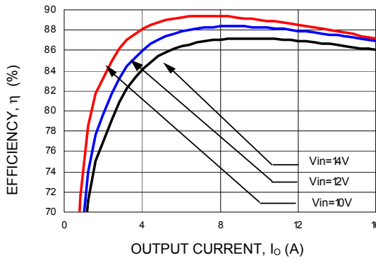
Figure 2. Converter Efficiency versus Output Current ( V_{out} = 1.2Vdc ).
