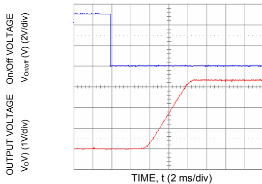
Figure 16. Typical Start-Up Using Remote On/Off with Low-ESR external capacitors (7x150µF Polymer) ( V_{in} = 5.0 Vdc, V_o = 3.3 Vdc, I_o = 5.0 A, C_o = 1050 µF).
