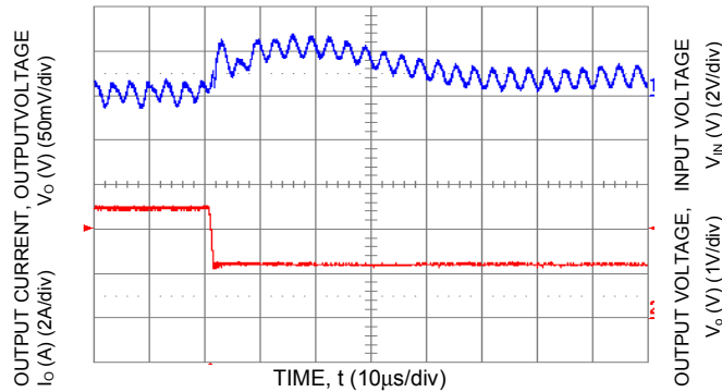
Figure 14. Transient Response to Dynamic Load Change from 100% of 50% full load ( V_o = 5.0 Vdc, C_{ext} = 2 \times 150 µF Polymer Capacitors).
