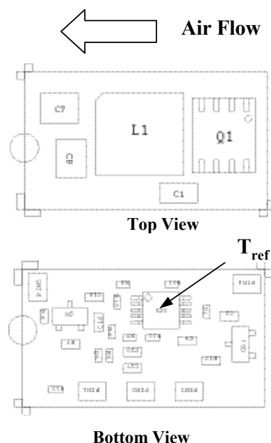
Figure 34. T_{\text{ref}} Temperature measurement location.
