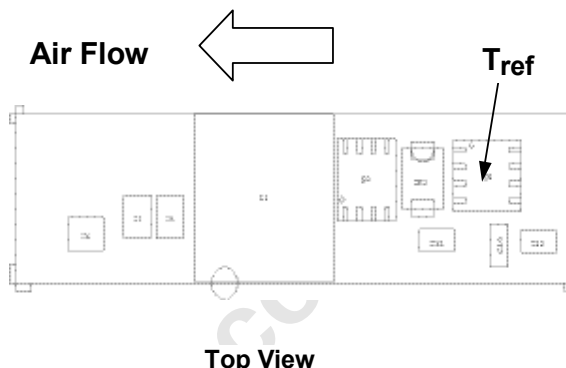
Figure 35. T_{ref} Temperature measurement location
