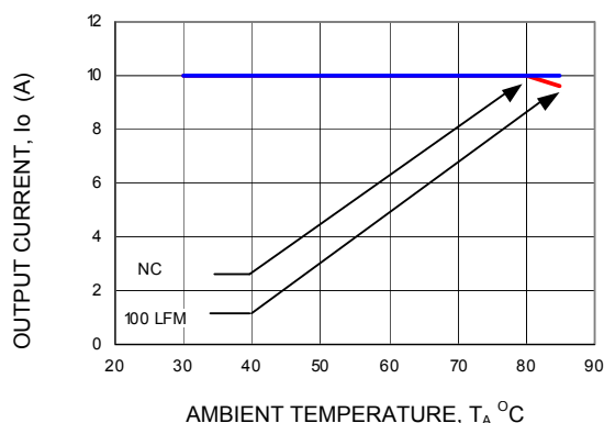
Figure 19. Derating Output Current versus Local Ambient Temperature and Airflow ( V_{in} = 5.0\text{Vdc} , V_o = 0.75\text{Vdc} ).
