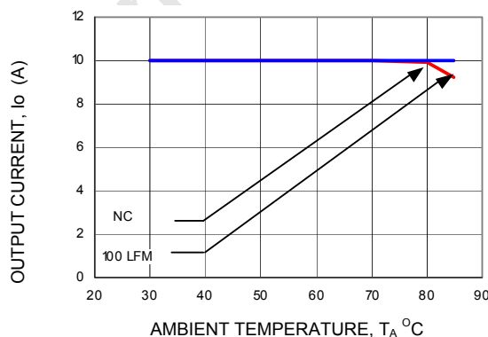
Figure 21. Derating Output Current versus Local Ambient Temperature and Airflow ( V_{in} = 5.0\text{Vdc} , V_o = 2.5\text{Vdc} ).
