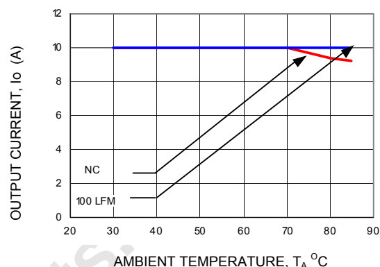
Figure 22. Derating Output Current versus Local Ambient Temperature and Airflow ( V_{in} = 5.0\text{Vdc} , V_o = 3.3\text{Vdc} ).
