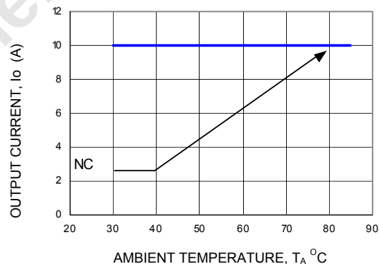
Figure 23. Derating Output Current versus Local Ambient Temperature and Airflow ( V_{in} = 3.3\text{Vdc} , V_o = 2.5\text{Vdc} ).
