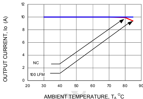
Figure 20. Derating Output Current versus Local Ambient Temperature and Airflow ( V_{in} = 5.0\text{Vdc} , V_o = 1.8\text{Vdc} ).
