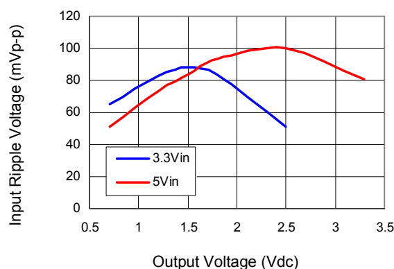
Figure 28. Input ripple voltage for various output with 3x150 \mu F polymer and 2x47 \mu F ceramic capacitors at the input (full load)
