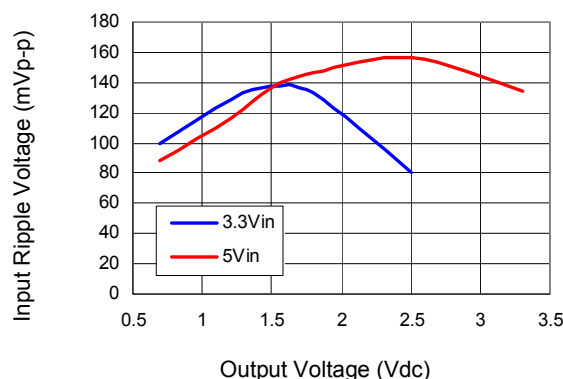
Figure 27. Input ripple voltage for various output with 1x150 \mu F polymer and 1x47 \mu F ceramic capacitors at the input (full load).
