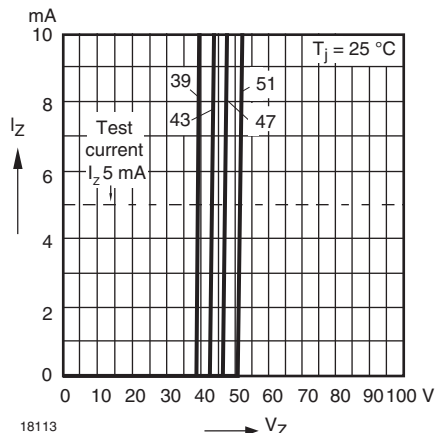
Fig. 14 - Breakdown Characteristics
