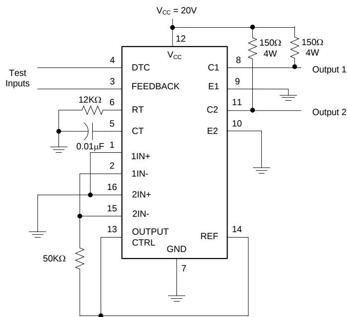
Test Circuit
